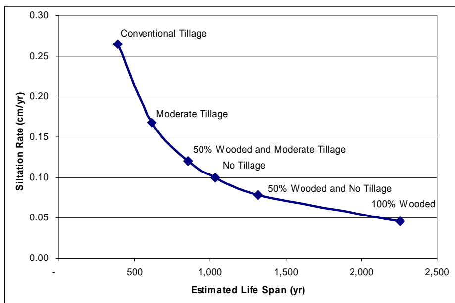
Figure 5-3. Estimated Life Span for Scenarios
