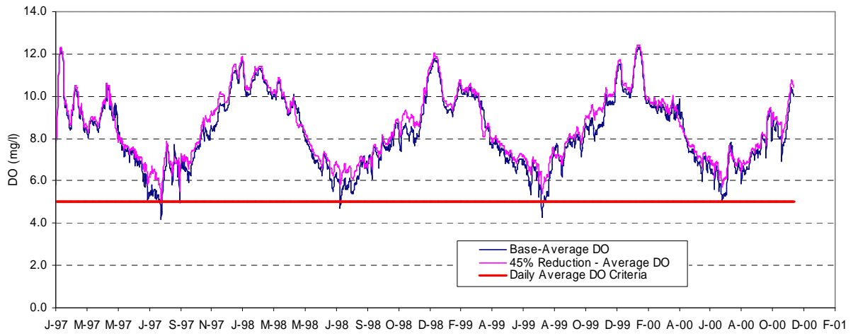
Figure 4-1. Daily Average DO in the Epilimnion.
