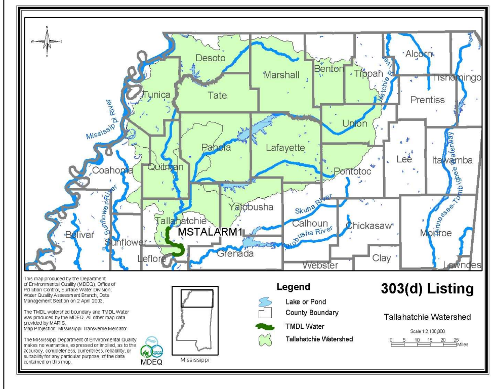
Figure 3. Tallahatchie River Watershed 303(d) Listed Segments (Complete Drainage Area)
