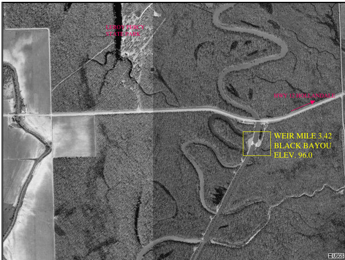
Photo 2. Aerial Photo of the Weir Located on Black Bayou Downstream of Highway 12
