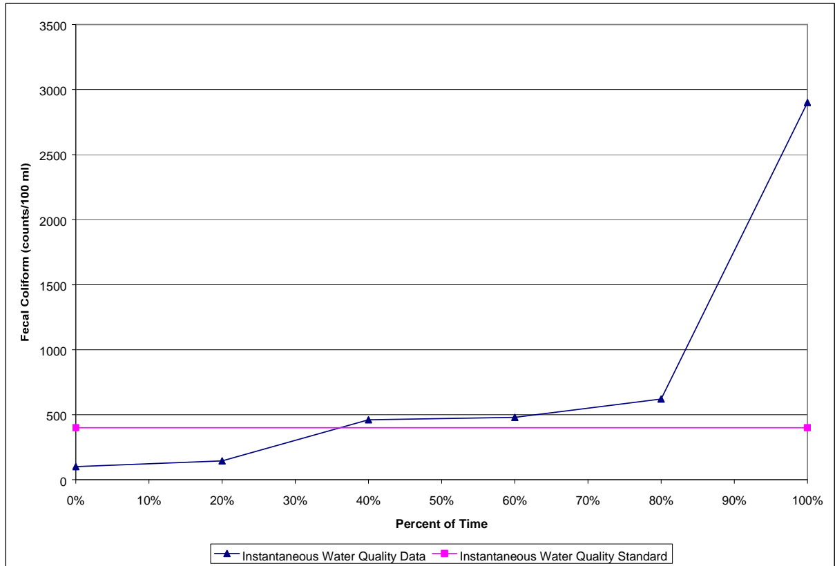
Figure 5. 10% Test Curve for Station FTN-37, Summer 2003
