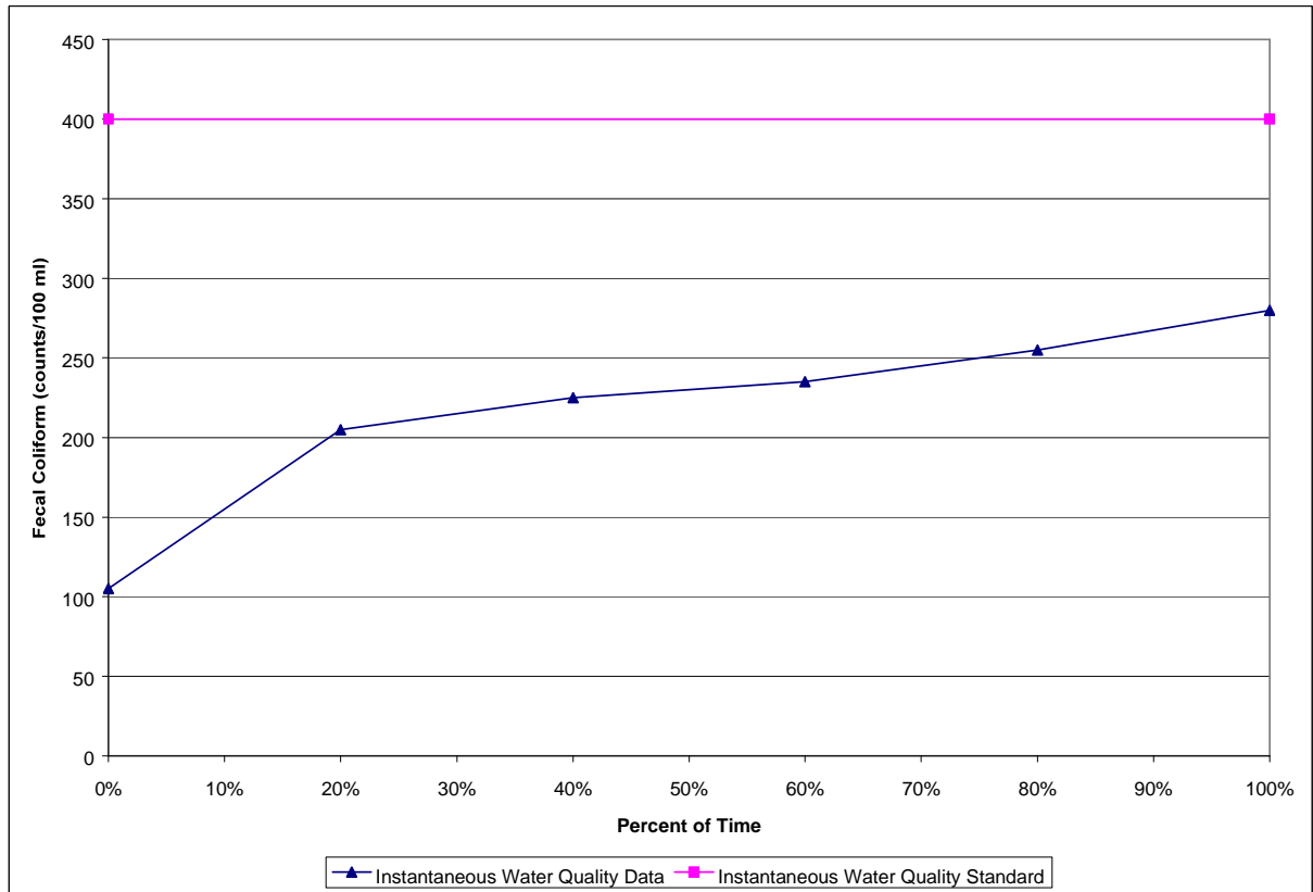
Figure 6. 10% Test Curve for Station FTN-37, Summer 2004
