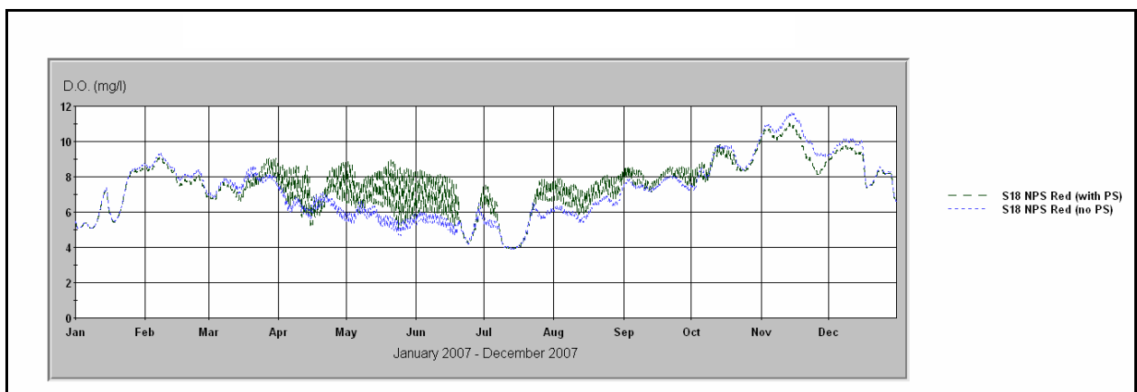
Figure 7. Model Output for DO – Quiver River Natural Conditions with and without PS
