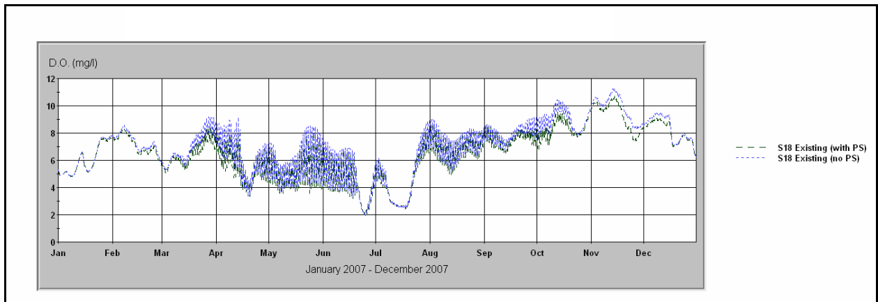
Figure 6. Model Output for DO –Quiver River Existing Conditions with and without PS
