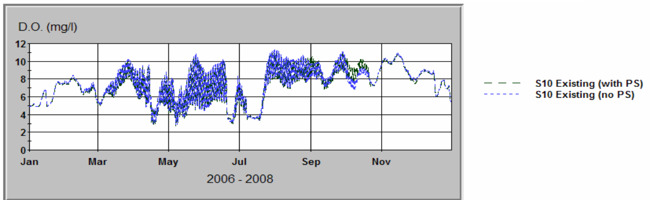
Figure 5. Model Output for DO – Porter Bayou Existing Conditions with and without PS
