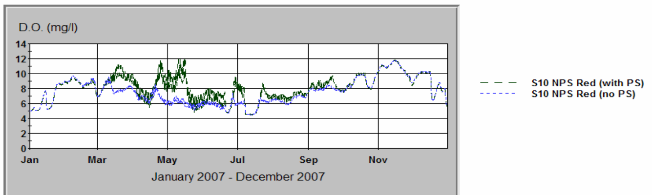
Figure 6. Model Output for DO – Porter Bayou Natural Conditions with and without PS
