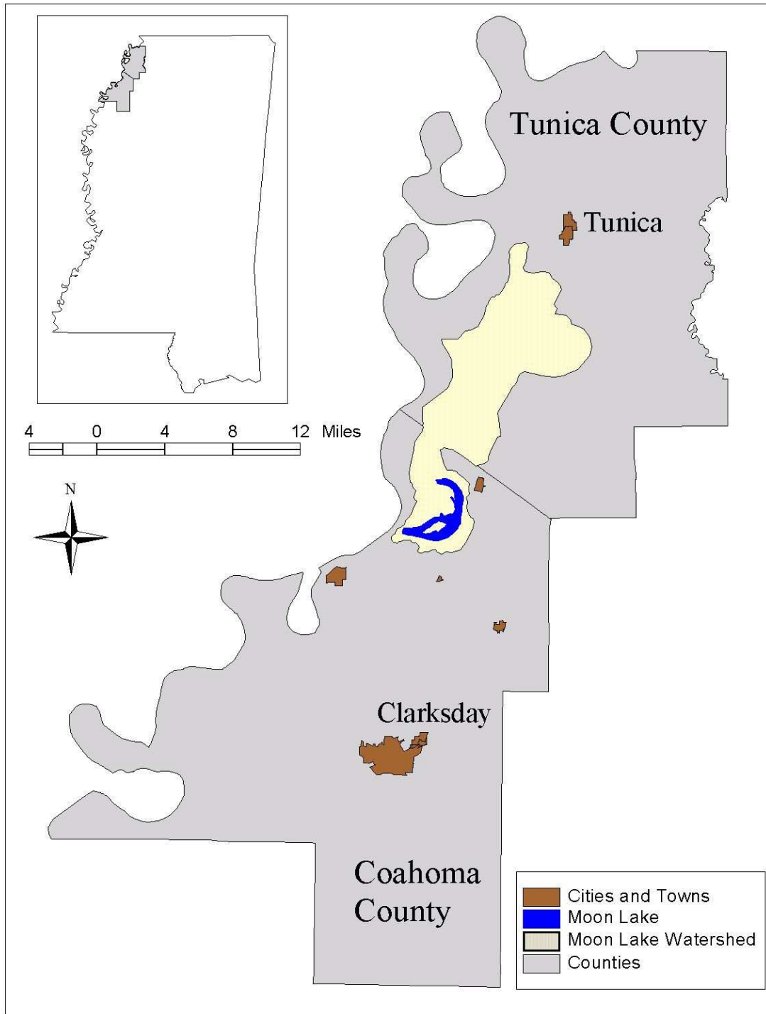
Figure 1-2. Watershed Location
