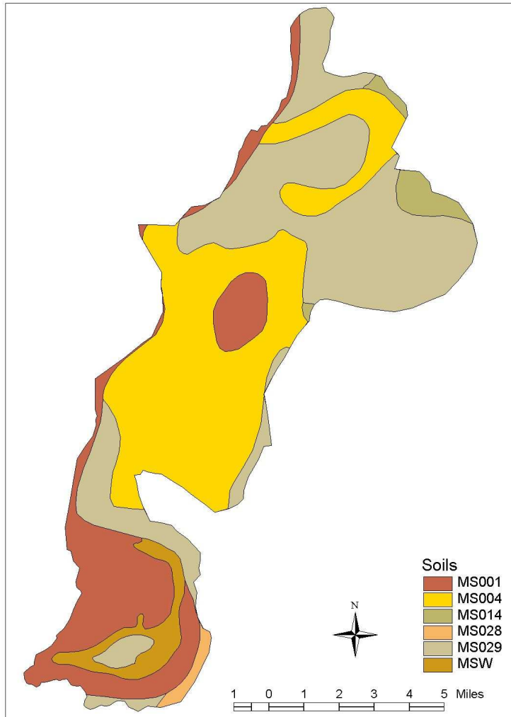
Figure 1-4. Soil Type
