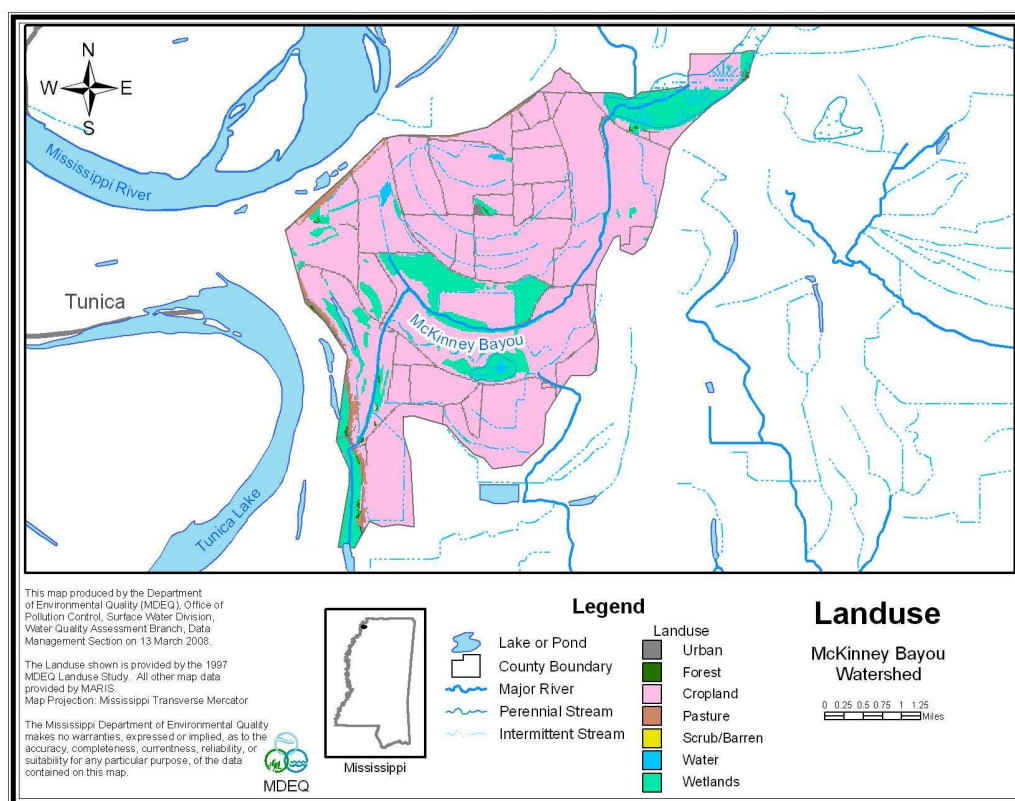
Figure 3. McKinney Bayou Watershed Landuse
