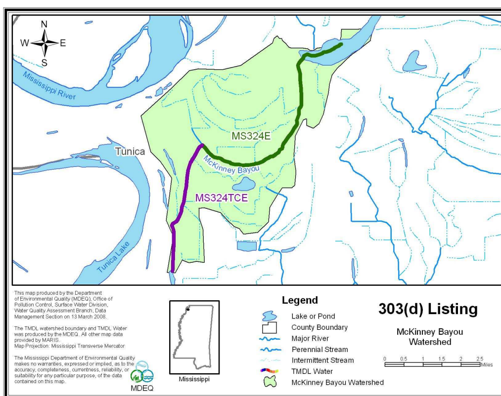
Figure 2. McKinney Bayou §303(d) Listed Segment
