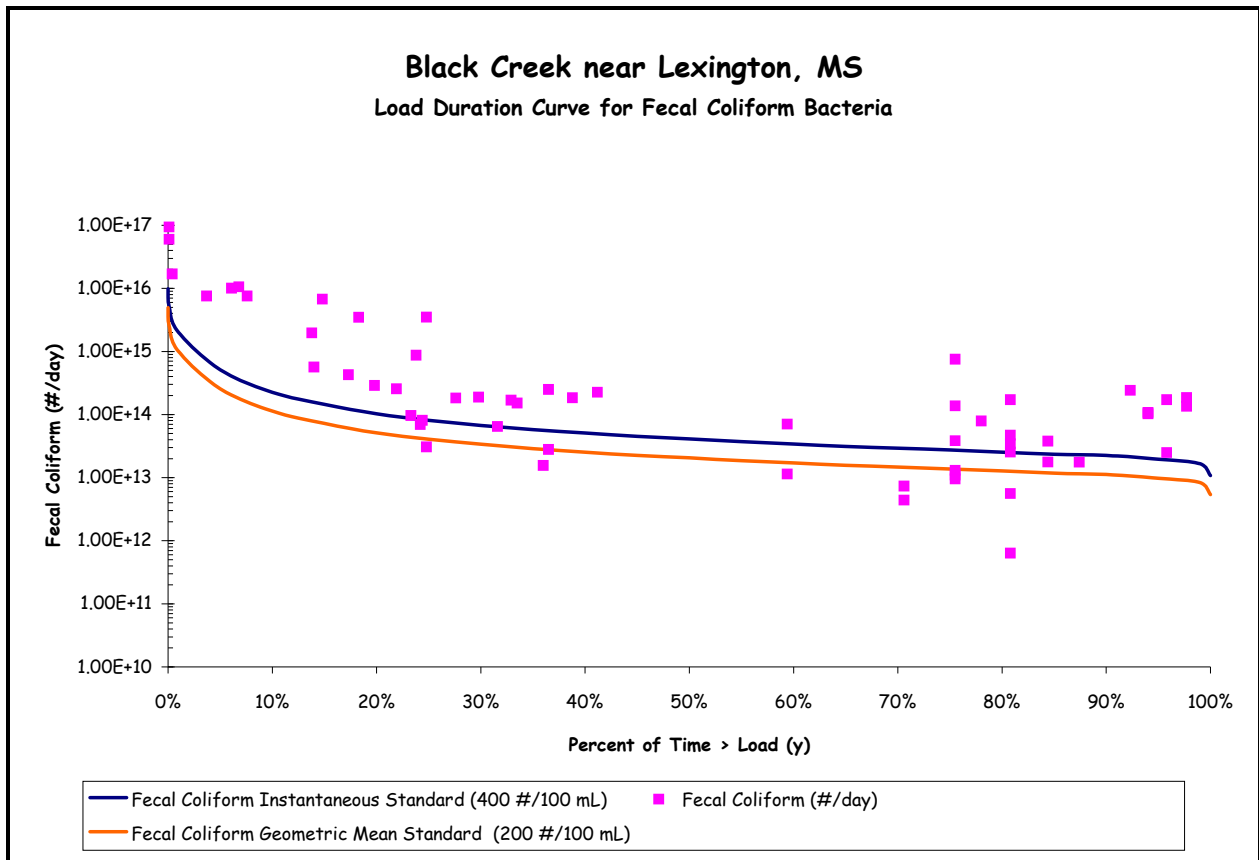
Figure 4. Load Duration Curve for Station 07287400
