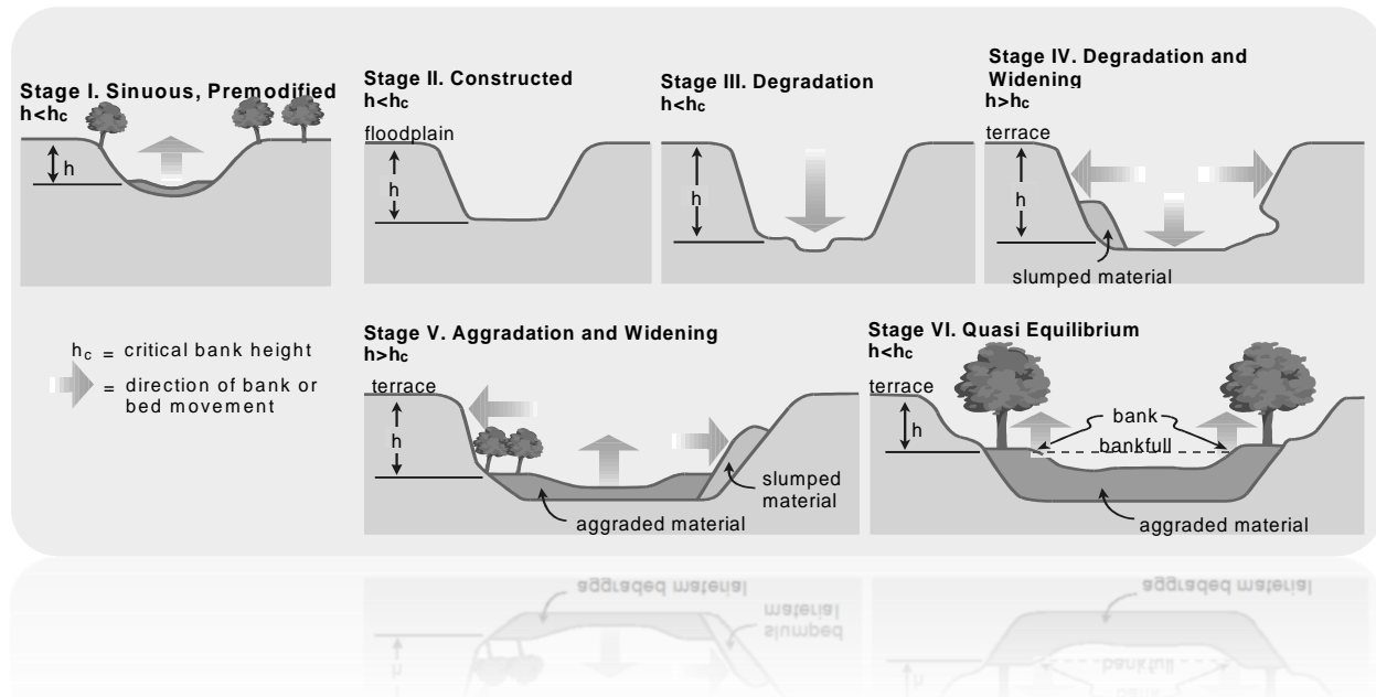
Figure 14. Six Stages of Channel Evolution (Simon and Hupp, 1986)
