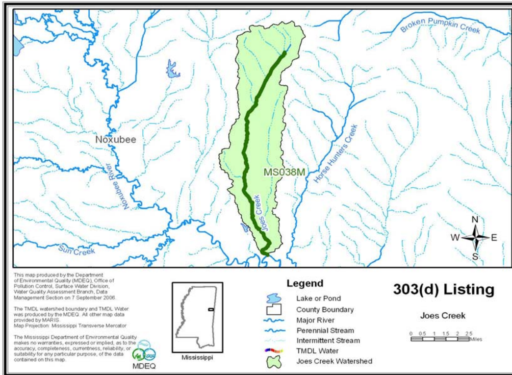
Figure 1. Joes Creek 303(d) segment
