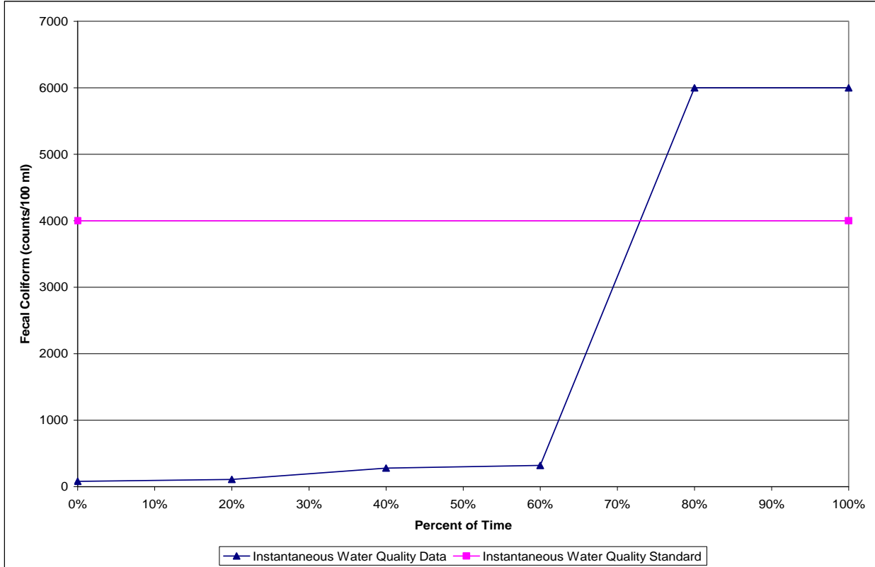
Figure 4. 10% Test Curve for Station 66, Winter 2003
