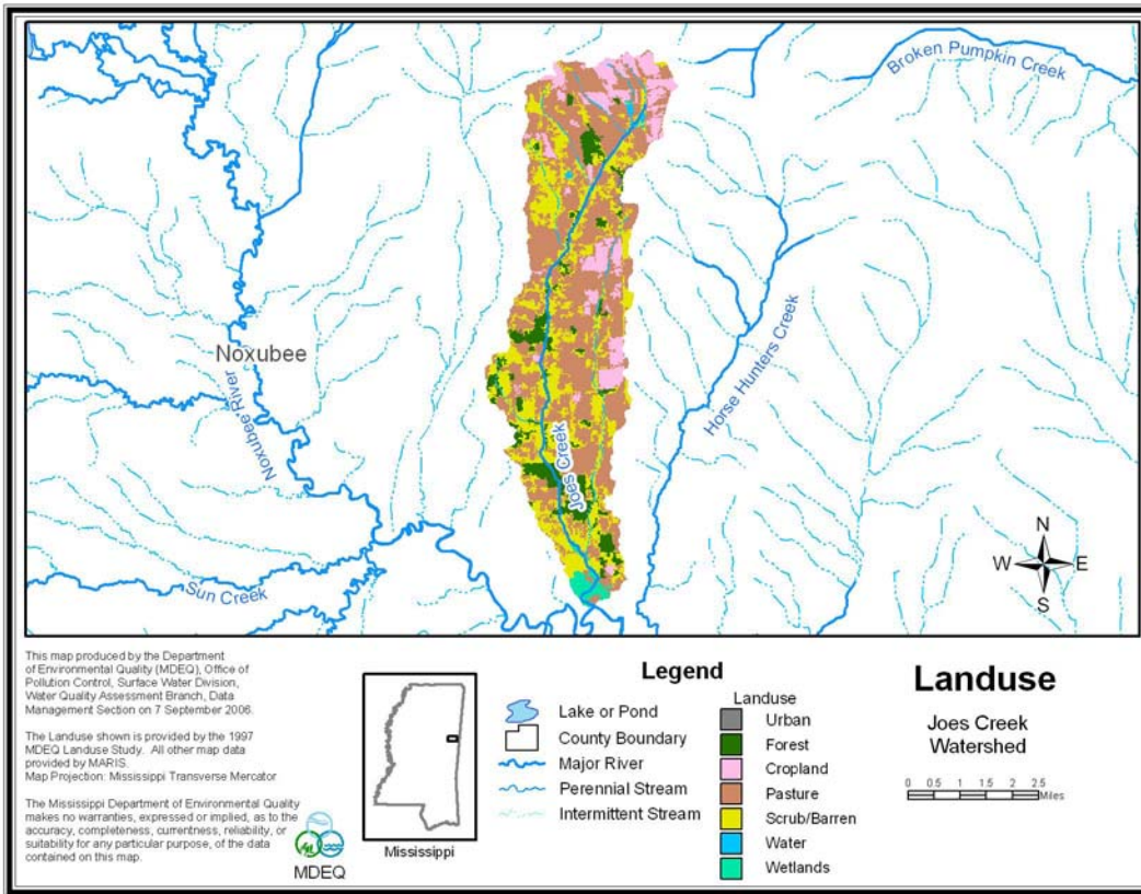
Figure 7. Landuse in Joes Creek Watershed
