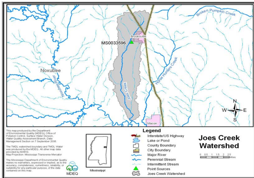
Figure 6. NPDES Dischargers in Joes Creek
