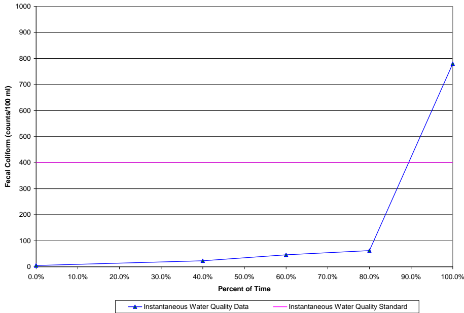
Figure 4. 10% Test Curve for Station 67, Summer 2002
