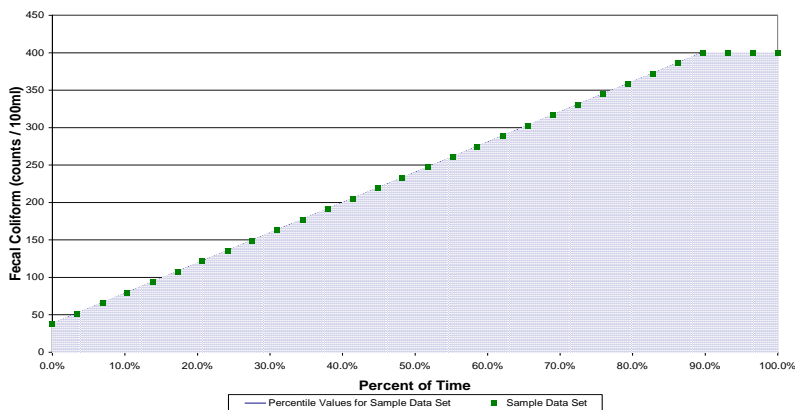
Figure 3. Theoretical Capacity Data Set Curve
