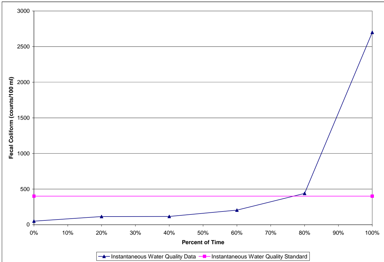
Figure 5. 10% Test Curve for Station A0570279, Summer 2004
