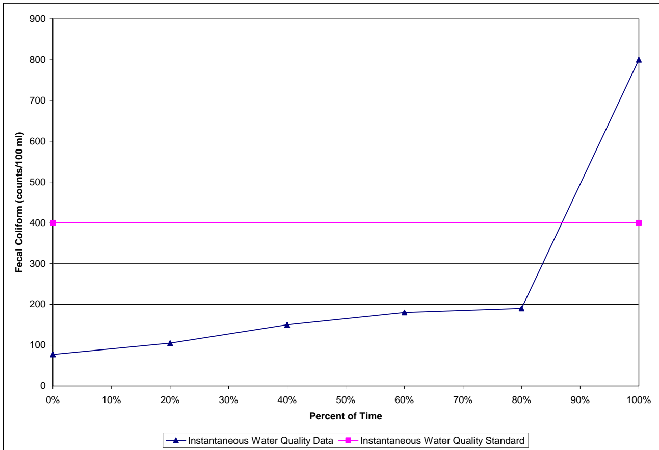
Figure 6. 10% Test Curve for Station A0570279, Summer 2005
