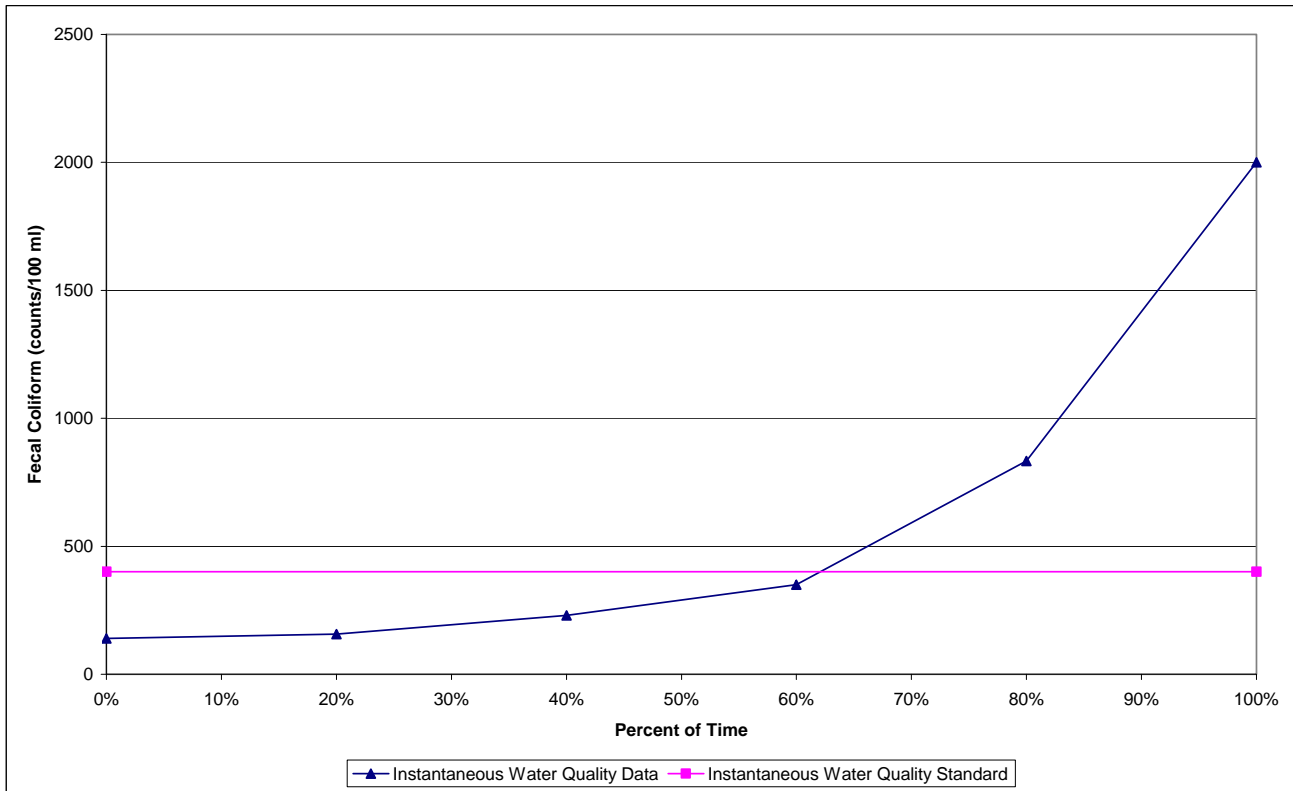
Figure 6. 10% Test Curve for Station PR-37, Summer 2003
