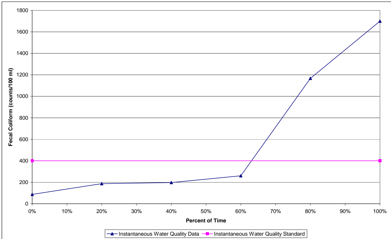
Figure 7. 10% Test Curve for Station PR-38, Summer 2003
