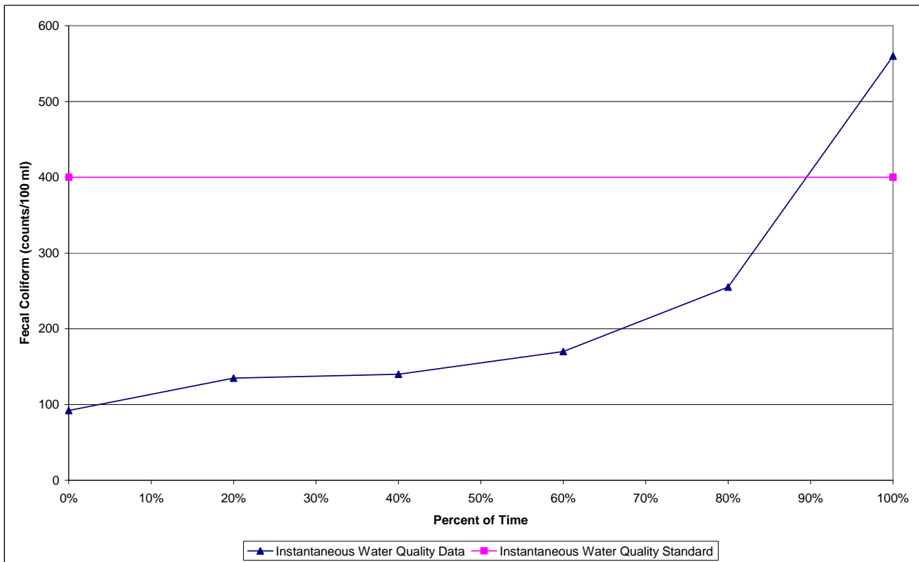
Figure 5. 10% Test Curve for Station PR-37, Summer 2001
