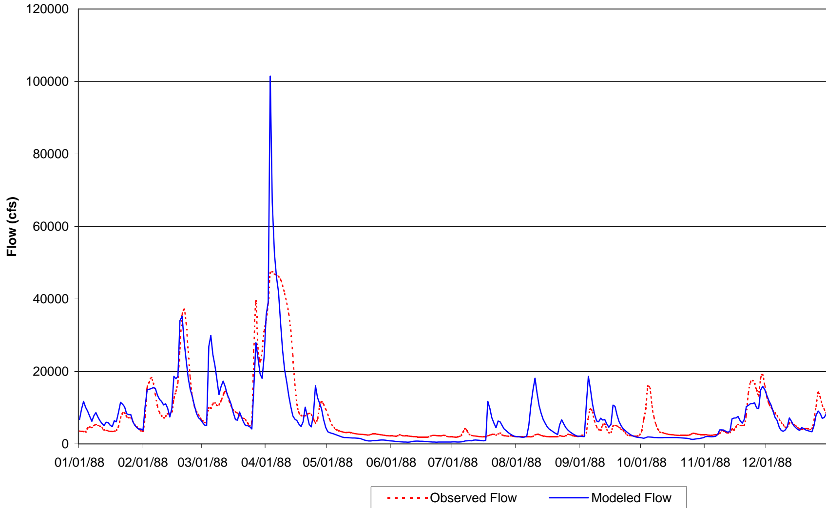
Graph A-1 Daily Flow Comparison between USGS Gage Station 02489500 and Reach 03180004010 for 01/01/1988 - 12/31/1988
