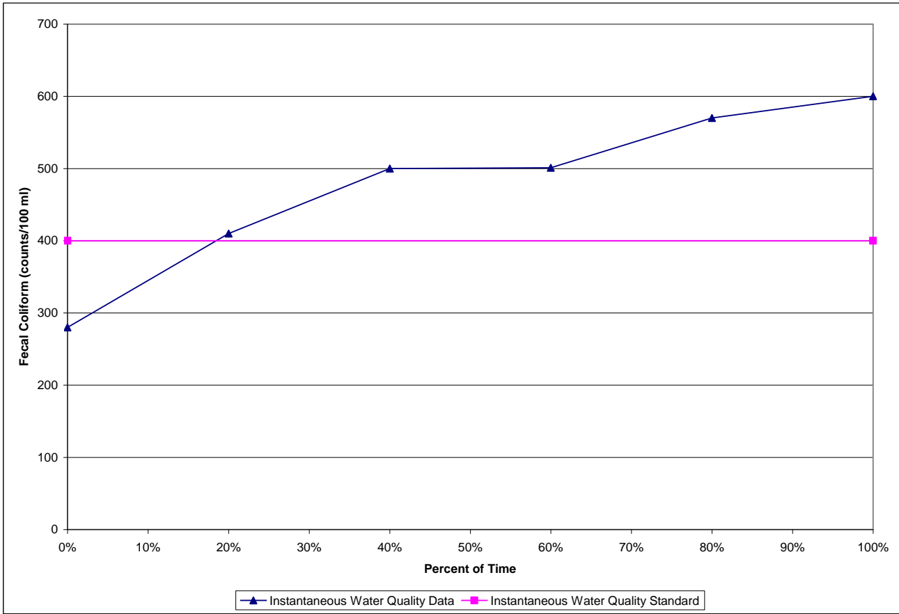
Figure 6. 10% Test Curve for Station PR-33, Summer 2003
