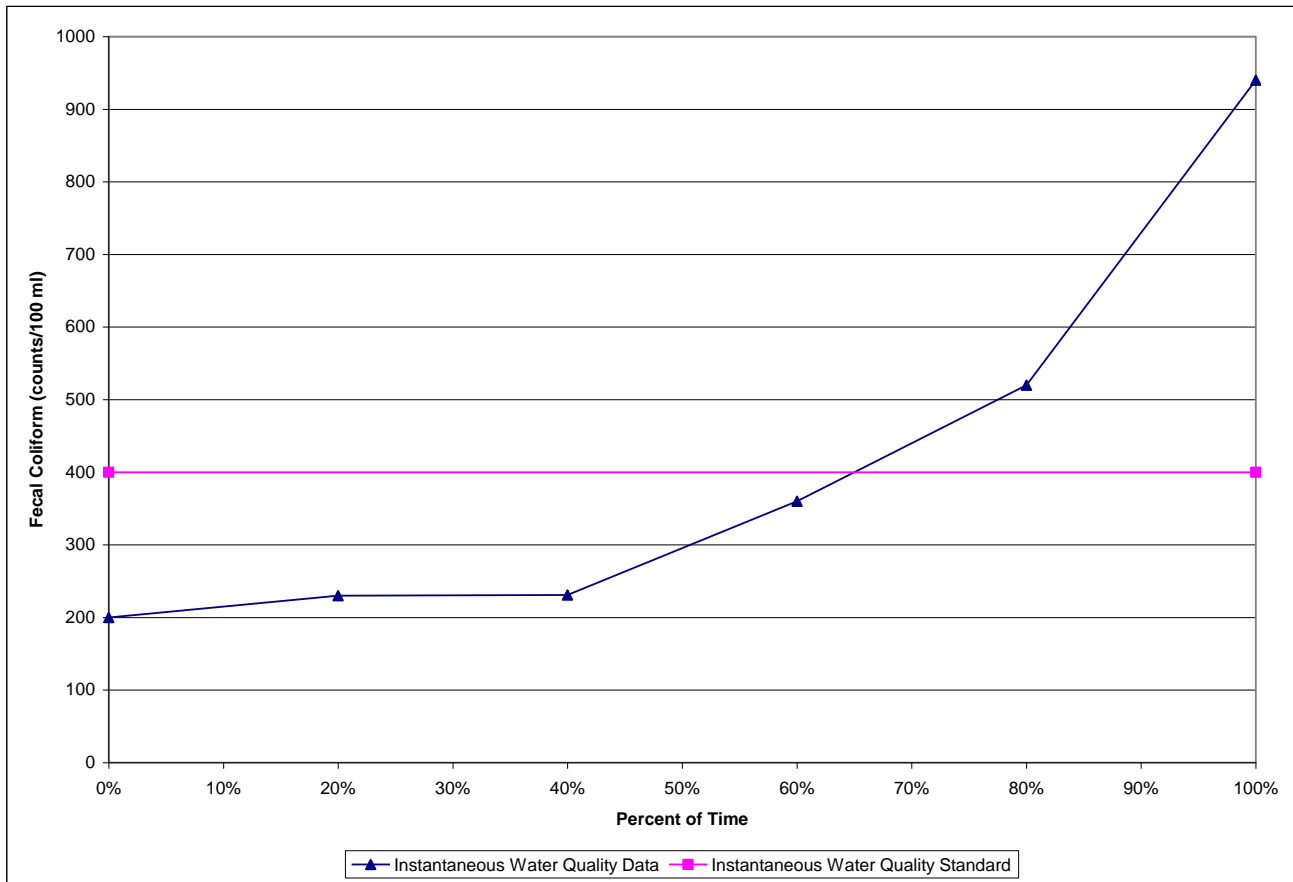
Figure 5. 10% Test Curve for Station PR-33, Summer 2001
