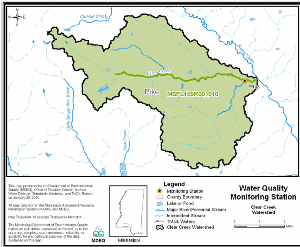
Figure 3. Clear Creek Segment with Water Quality Gage
