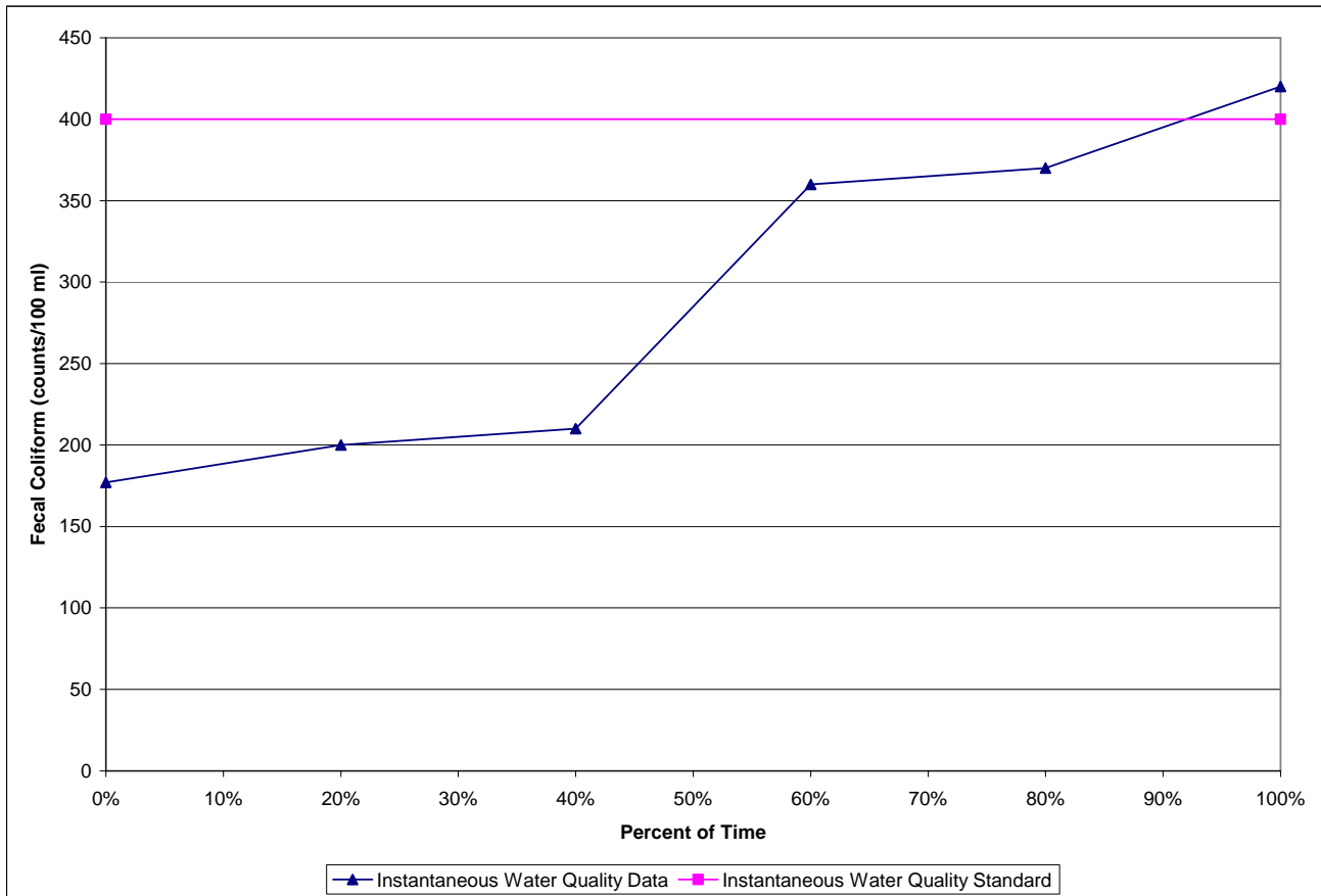
Figure 6. 10% Test Curve for Station PR43, Summer 2003
