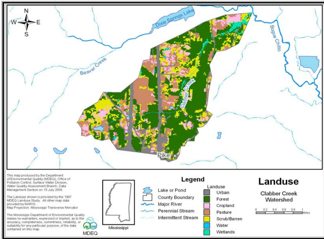
Figure 6. Land Use Distribution Map for the Clabber Creek Watershed
