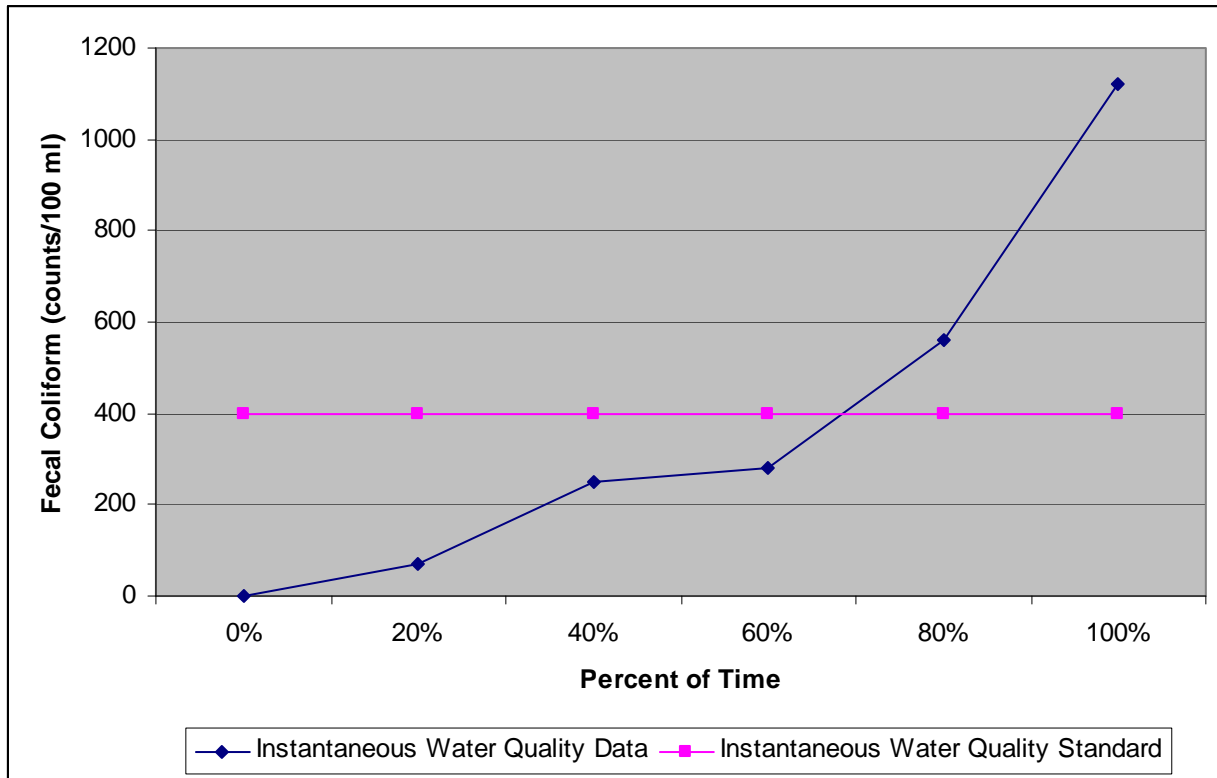
Figure 5. 10% Test Curve for Station A1130022, Summer 2006
