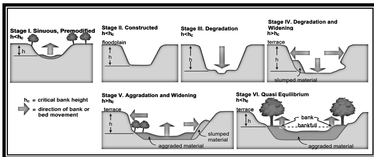
Figure 24: Six Stages of Channel Evolution (Simon and Hupp, 1986)
