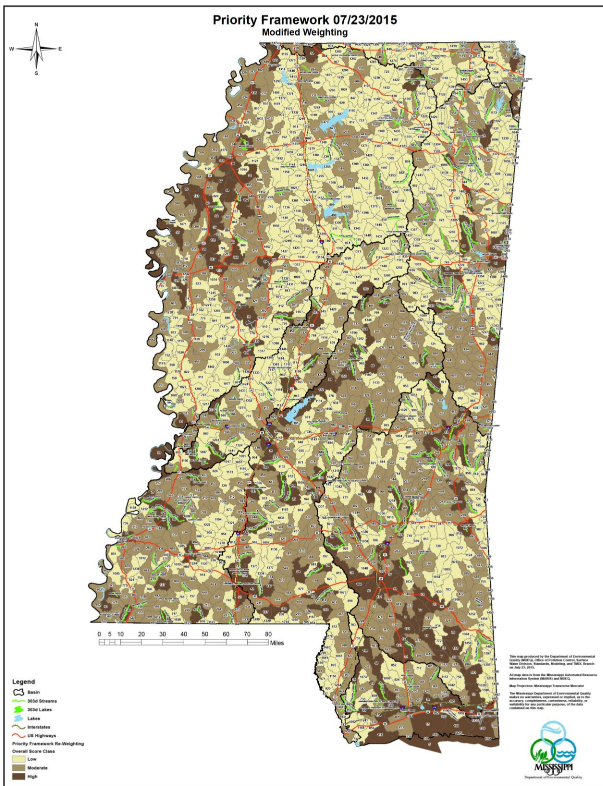
Figure 1. Watershed ranks based on factor profile weights
