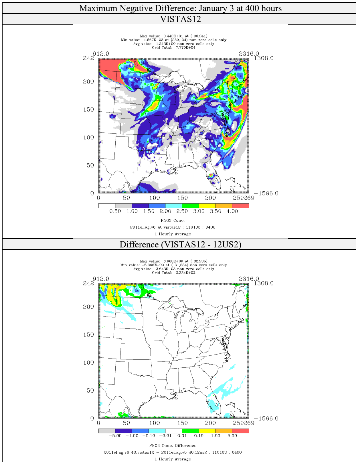
Figure 4-74: Comparison of Nitrate Concentrations ( \mu\text{g}/\text{m}^3 ) for CAMx 6.40 on VISTAS12 and 12US2 domains 2011el Simulations (Maximum Negative Difference)
