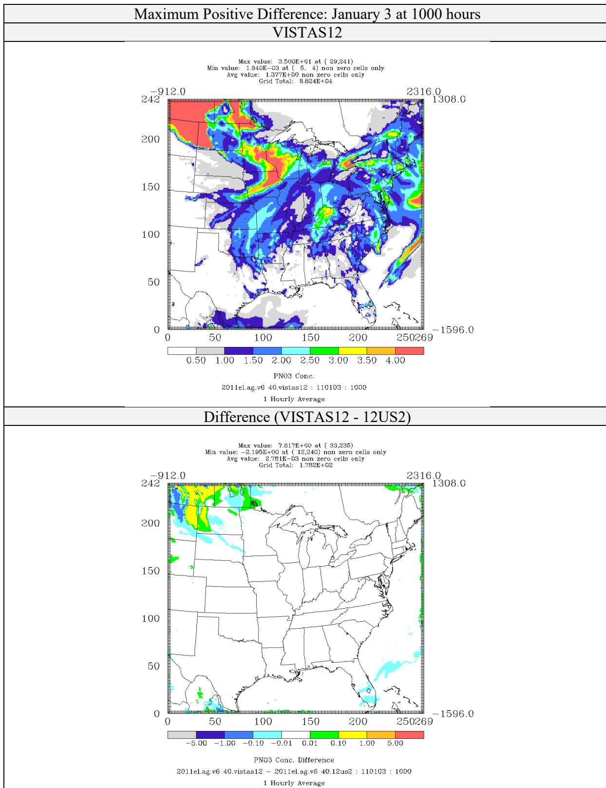
Figure 4-64: Comparison of Nitrate Concentrations ( \mu\text{g}/\text{m}^3 ) for CAMx 6.40 on VISTAS12 and 12US2 domains 2011el Simulations (Maximum Positive Difference)
