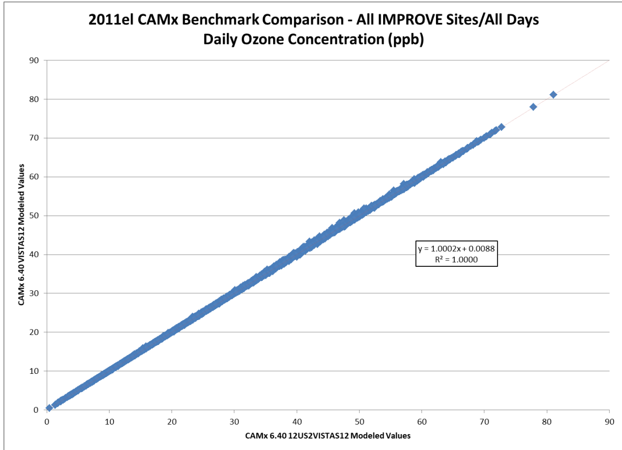
Figure 4-21: Scatterplot Comparing 24-hour Average Predicted Ozone Concentrations (ppb) for All Days at all IMPROVE Monitor Locations for CAMx 6.40 on VISTAS12 and 12US2 domains 2011el Simulations Performed by VISTAS (Alpine).
