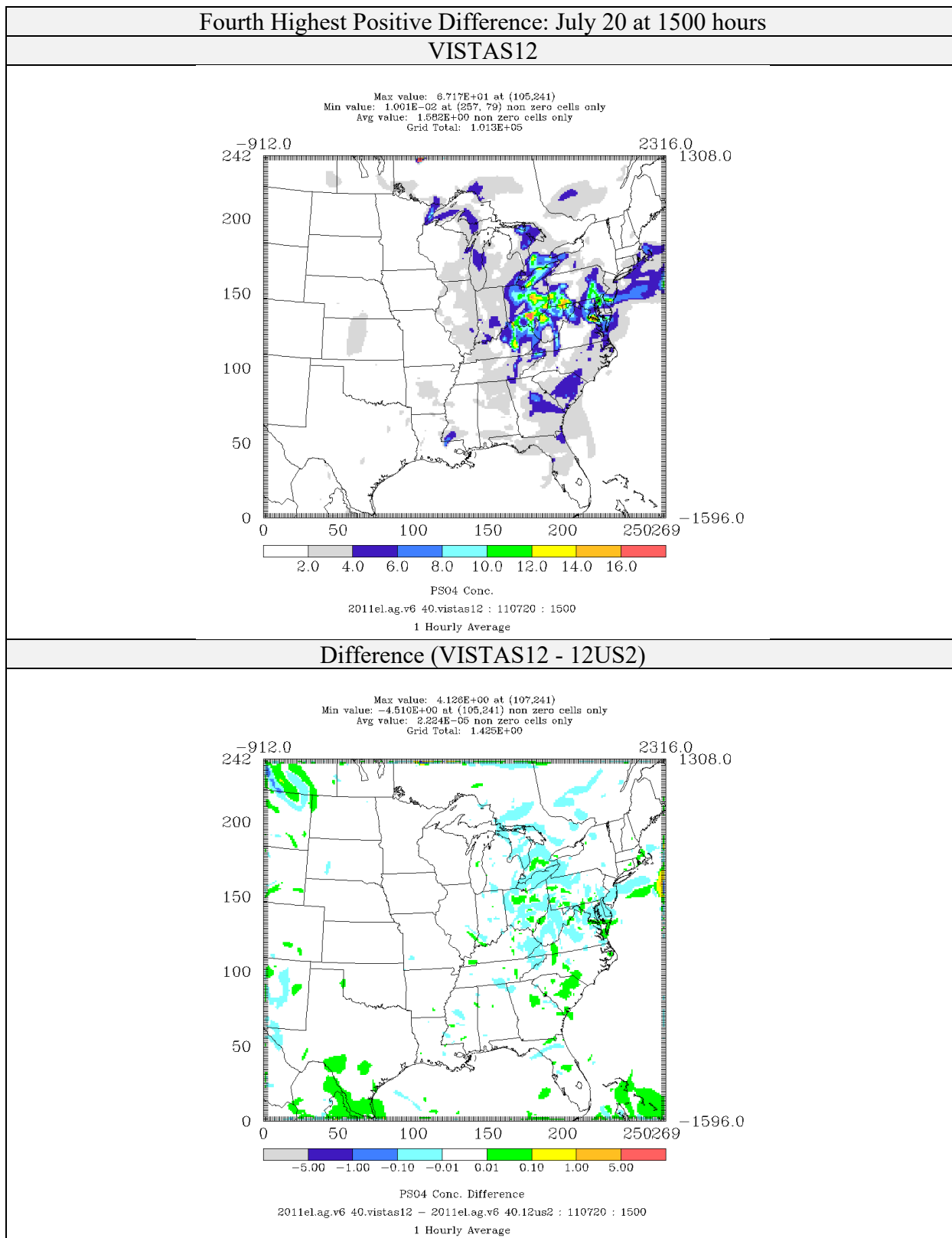
Figure 4-46: Comparison of Sulfate Concentrations ( \mu\text{g}/\text{m}^3 ) for CAMx 6.40 on VISTAS12 and 12US2 domains 2011el Simulations (Fourth Highest Positive Difference)
