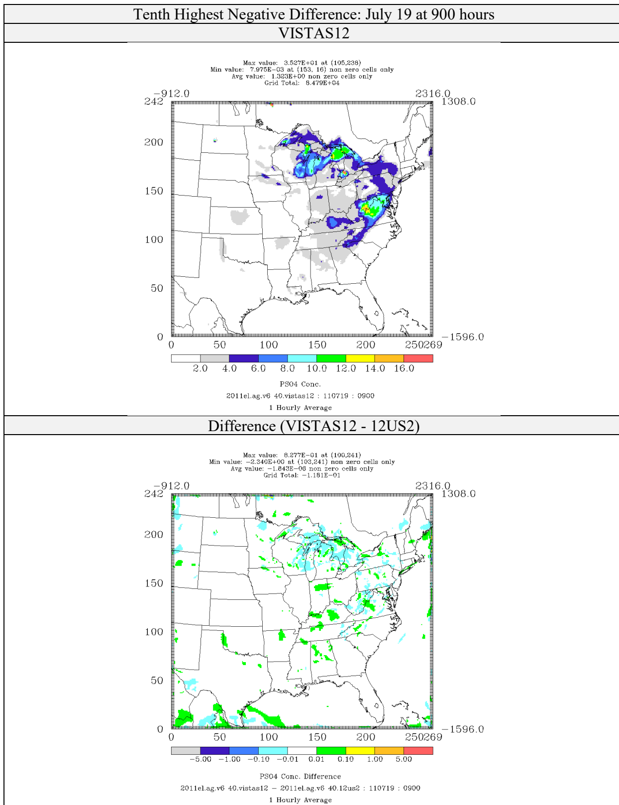
Figure 4-62: Comparison of Sulfate Concentrations ( \mu\text{g}/\text{m}^3 ) for CAMx 6.40 on VISTAS12 and 12US2 domains 2011el Simulations (Tenth Highest Negative Difference)
