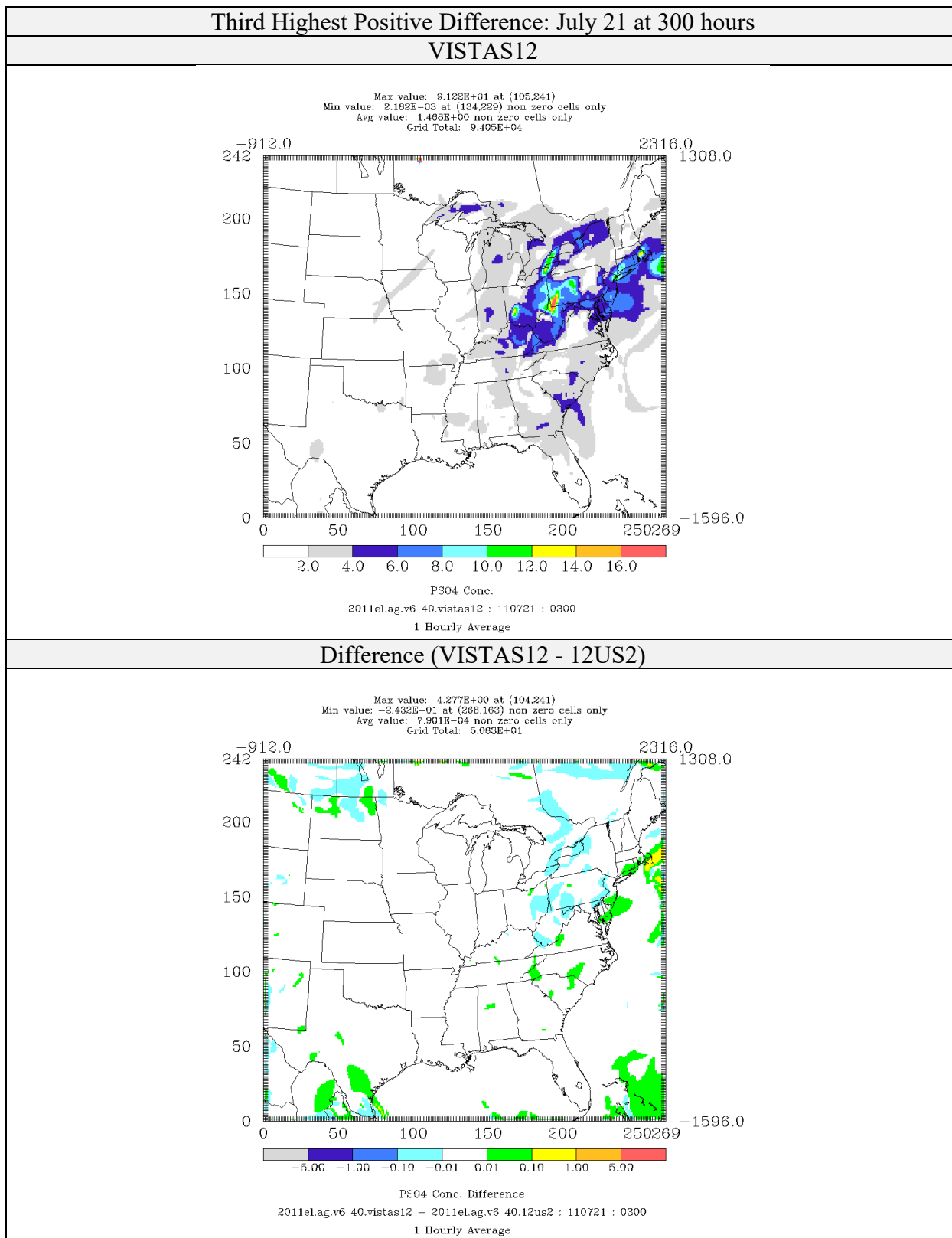
Figure 4-45: Comparison of Sulfate Concentrations ( \mu\text{g}/\text{m}^3 ) for CAMx 6.40 on VISTAS12 and 12US2 domains 2011el Simulations (Third Highest Positive Difference)
