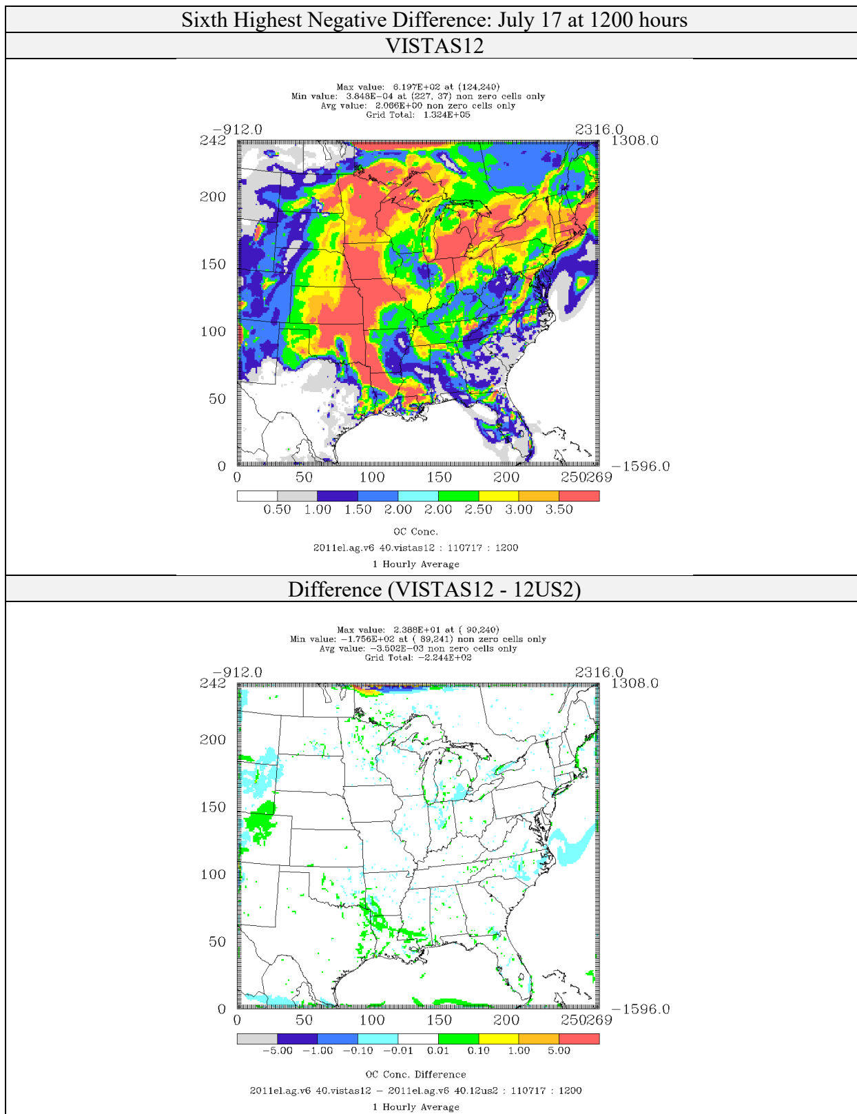
Figure 4-100: Comparison of Organic Matter Concentrations ( \mu\text{g}/\text{m}^3 ) for CAMx 6.40 on VISTAS12 and 12US2 domains 2011el Simulations (Sixth Highest Negative Difference)
