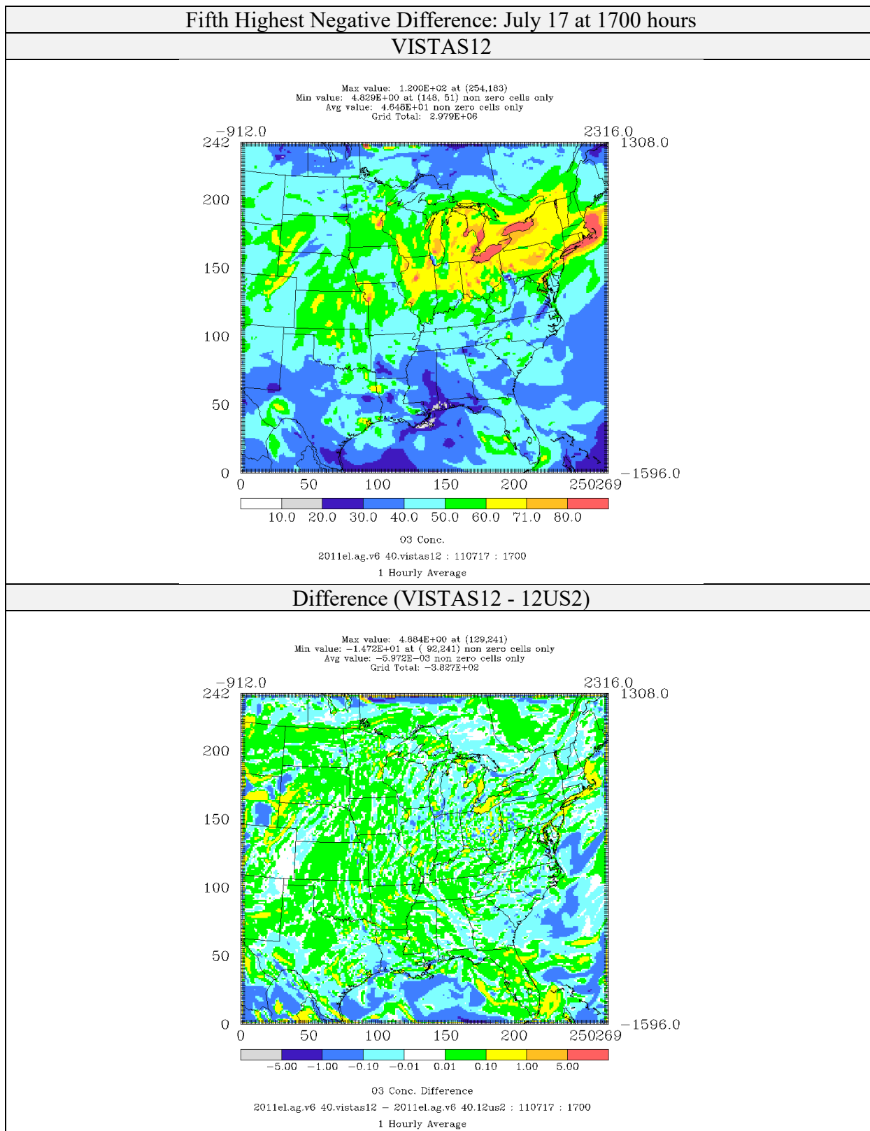
Figure 4-15: Comparison of Ozone Concentrations (ppb) for CAMx 6.40 on VISTAS12 and 12US2 domains 2011el Simulations (Fifth Highest Negative Difference)
