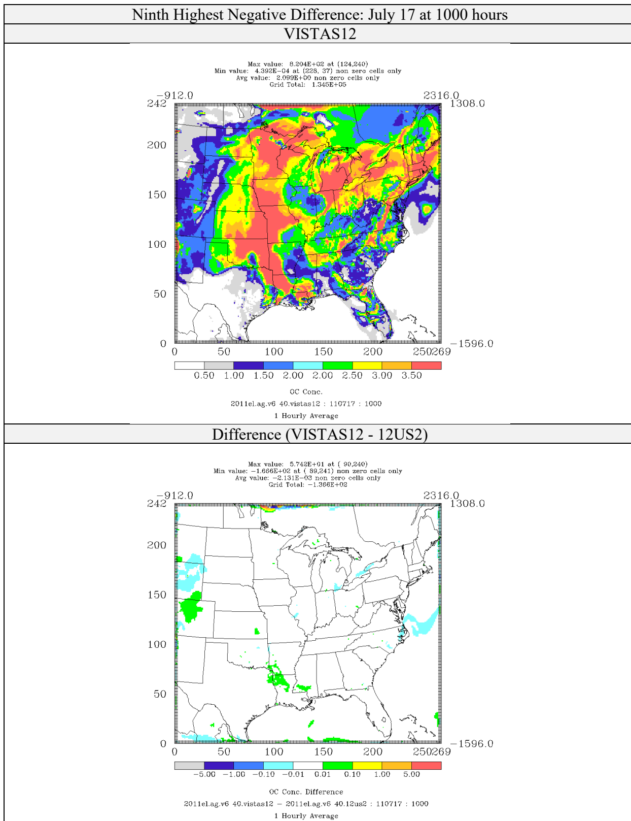
Figure 4-103: Comparison of Organic Matter Concentrations ( \mu\text{g}/\text{m}^3 ) for CAMx 6.40 on VISTAS12 and 12US2 domains 2011el Simulations (Ninth Highest Negative Difference)
