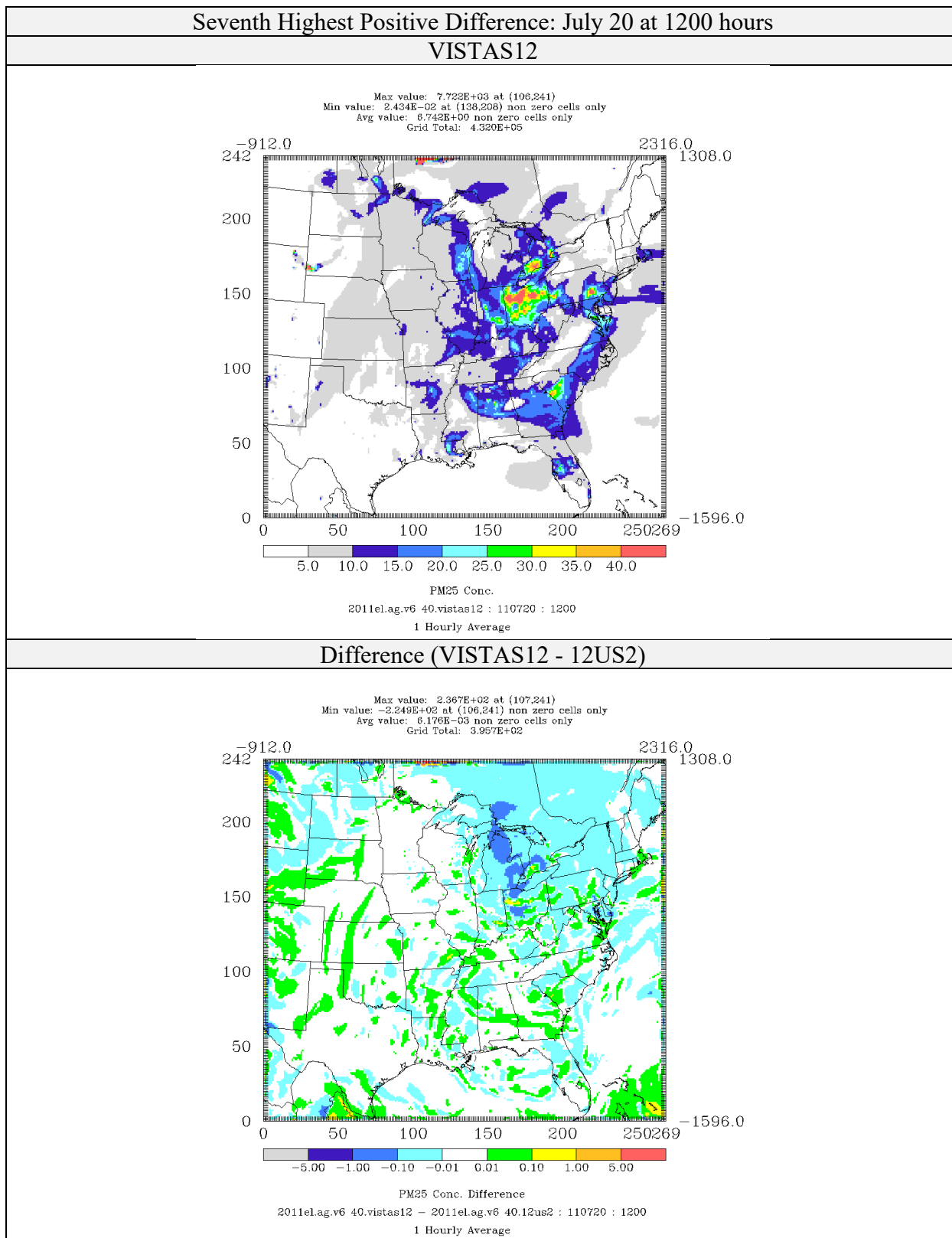
Figure 4-28: Comparison of PM 2.5 Concentrations ( \mu\text{g}/\text{m}^3 ) for CAMx 6.40 on VISTAS12 and 12US2 domains 2011el Simulations (Seventh Highest Positive Difference)
