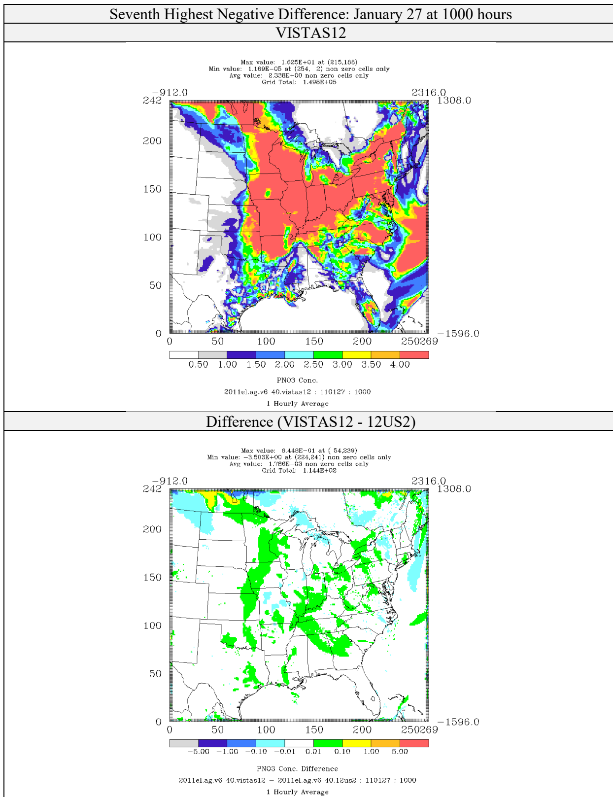
Figure 4-80: Comparison of Nitrate Concentrations ( \mu\text{g}/\text{m}^3 ) for CAMx 6.40 on VISTAS12 and 12US2 domains 2011el Simulations (Seventh Highest Negative Difference)
