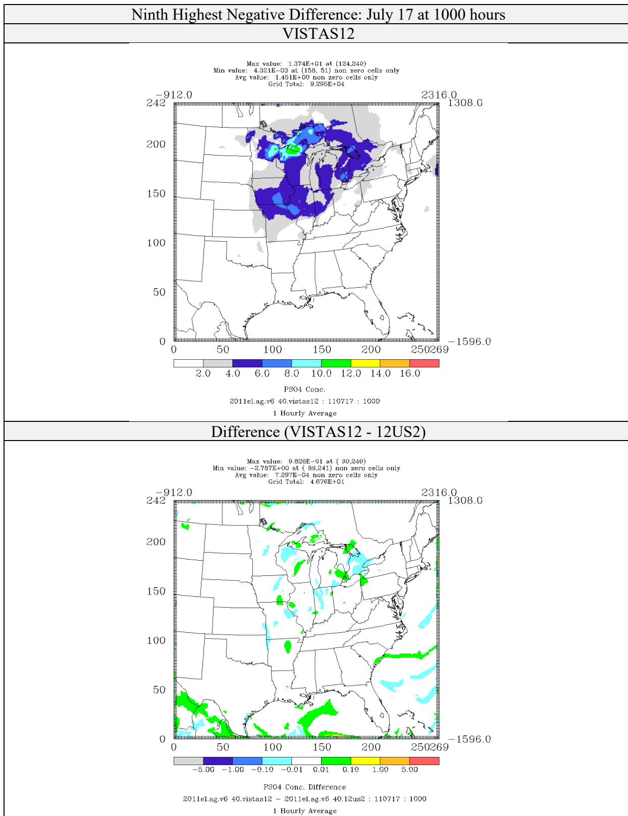
Figure 4-61: Comparison of Sulfate Concentrations ( \mu\text{g}/\text{m}^3 ) for CAMx 6.40 on VISTAS12 and 12US2 domains 2011el Simulations (Ninth Highest Negative Difference)
