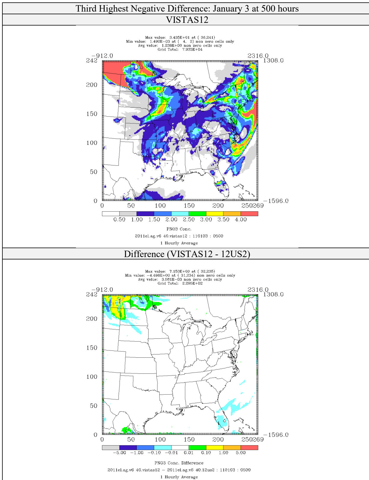
Figure 4-76: Comparison of Nitrate Concentrations ( \mu\text{g}/\text{m}^3 ) for CAMx 6.40 on VISTAS12 and 12US2 domains 2011el Simulations (Third Highest Negative Difference)
