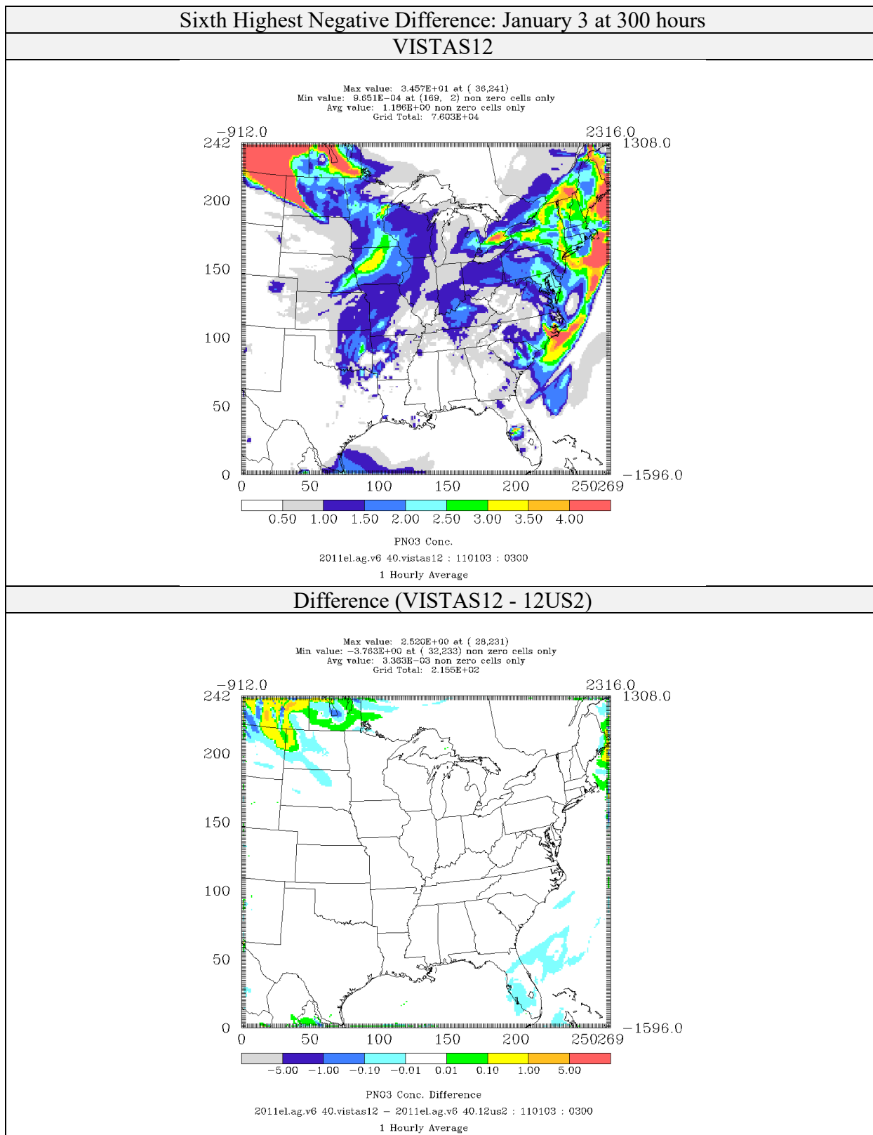
Figure 4-79: Comparison of Nitrate Concentrations ( \mu\text{g}/\text{m}^3 ) for CAMx 6.40 on VISTAS12 and 12US2 domains 2011el Simulations (Sixth Highest Negative Difference)
