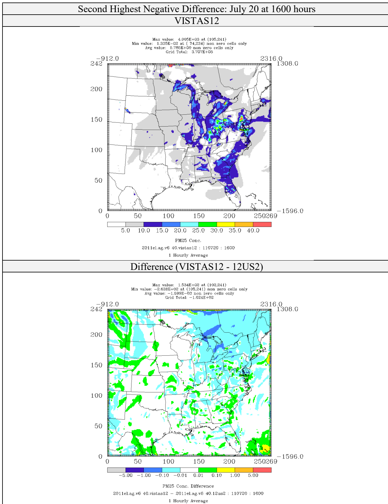
Figure 4-33: Comparison of PM 2.5 Concentrations ( \mu\text{g}/\text{m}^3 ) for CAMx 6.40 on VISTAS12 and 12US2 domains 2011el Simulations (Second Highest Negative Difference)
