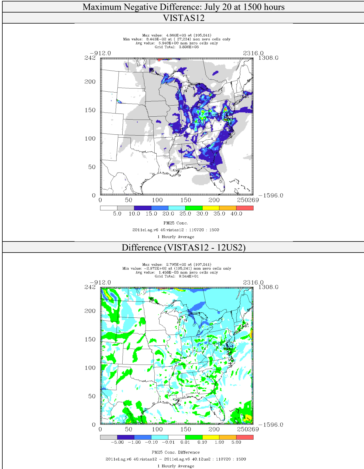
Figure 4-32: Comparison of PM 2.5 Concentrations ( \mu\text{g}/\text{m}^3 ) for CAMx 6.40 on VISTAS12 and 12US2 domains 2011el Simulations (Maximum Negative Difference)
