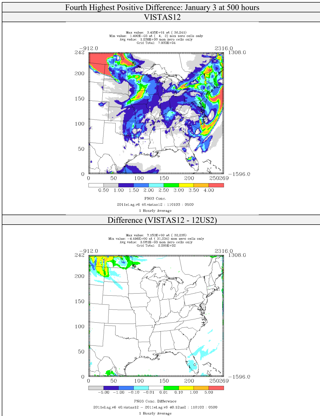
Figure 4-67: Comparison of Nitrate Concentrations ( \mu\text{g}/\text{m}^3 ) for CAMx 6.40 on VISTAS12 and 12US2 domains 2011el Simulations (Fourth Highest Positive Difference)
