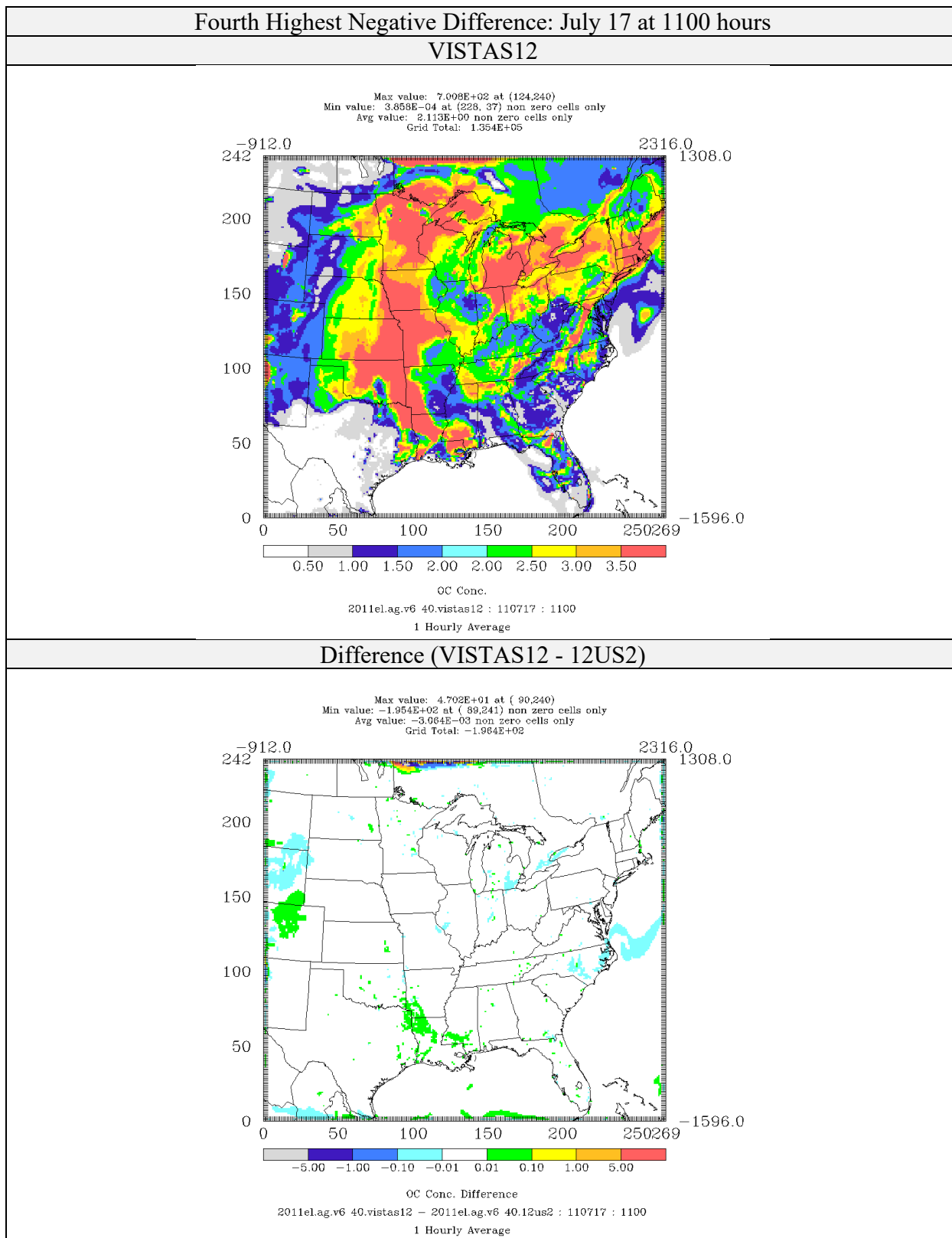
Figure 4-98: Comparison of Organic Matter Concentrations ( \mu\text{g}/\text{m}^3 ) for CAMx 6.40 on VISTAS12 and 12US2 domains 2011el Simulations (Fourth Highest Negative Difference)
