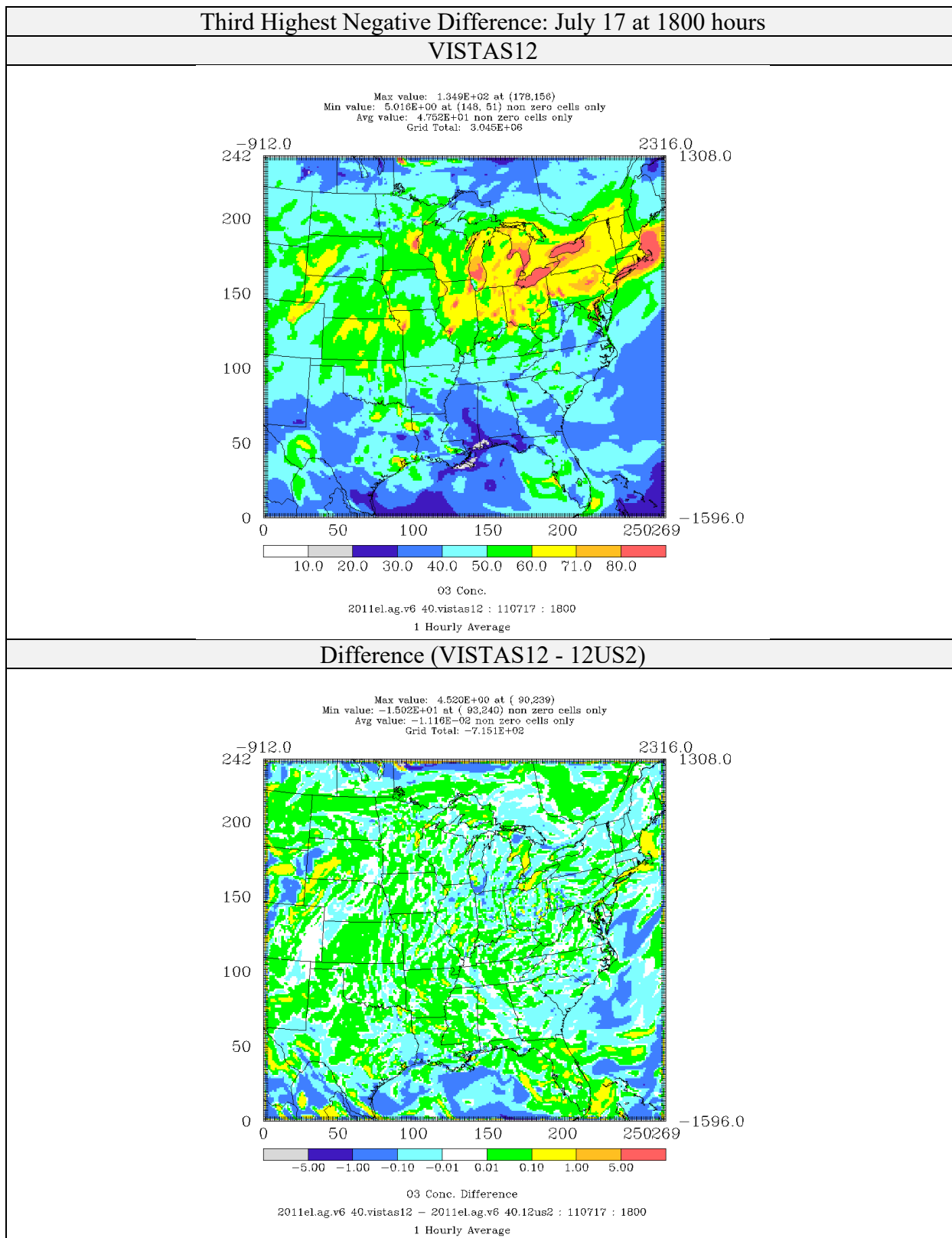
Figure 4-13: Comparison of Ozone Concentrations (ppb) for CAMx 6.40 on VISTAS12 and 12US2 domains 2011el Simulations (Third Highest Negative Difference)
