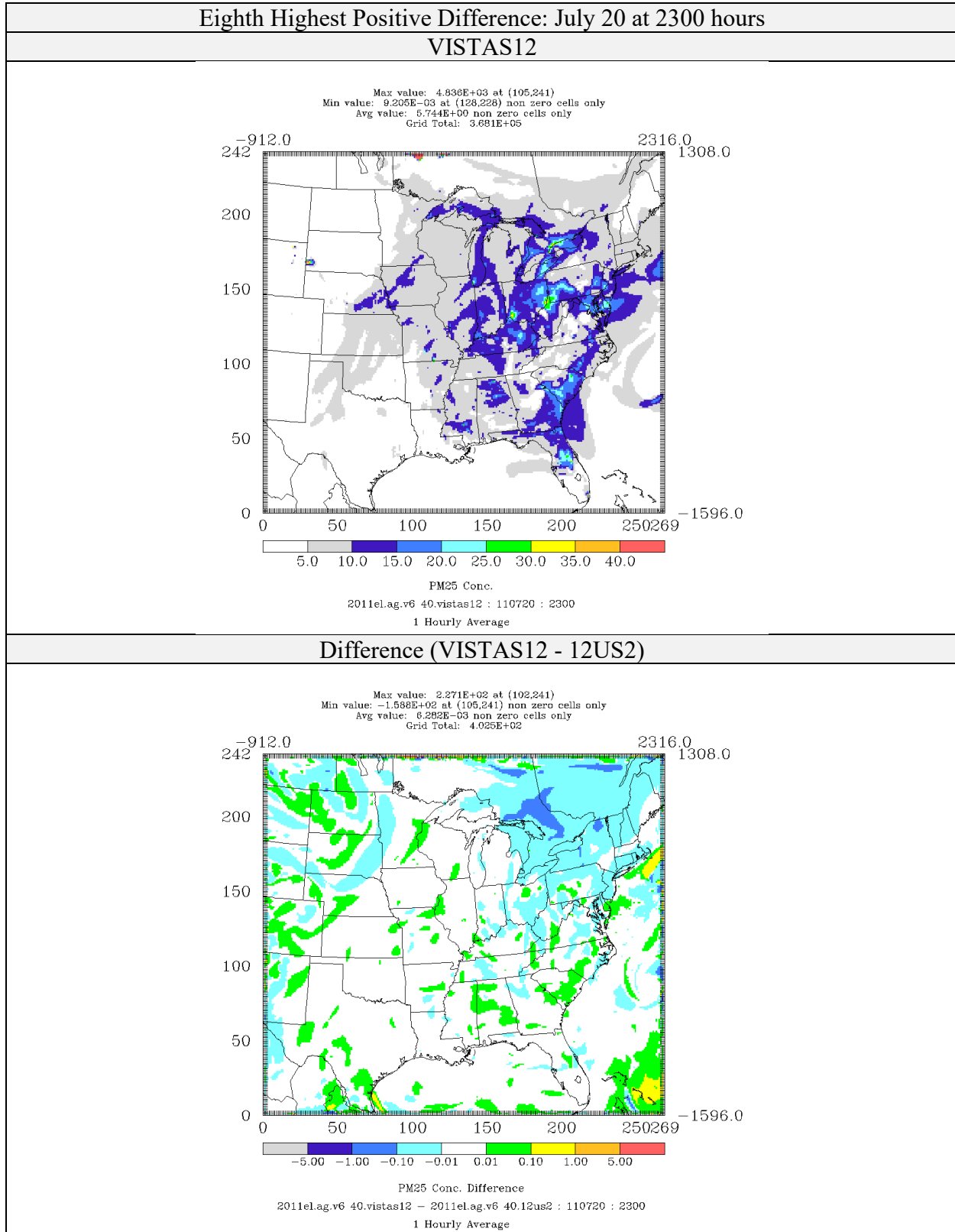
Figure 4-29: Comparison of PM 2.5 Concentrations ( \mu\text{g}/\text{m}^3 ) for CAMx 6.40 on VISTAS12 and 12US2 domains 2011el Simulations (Eighth Highest Positive Difference)
