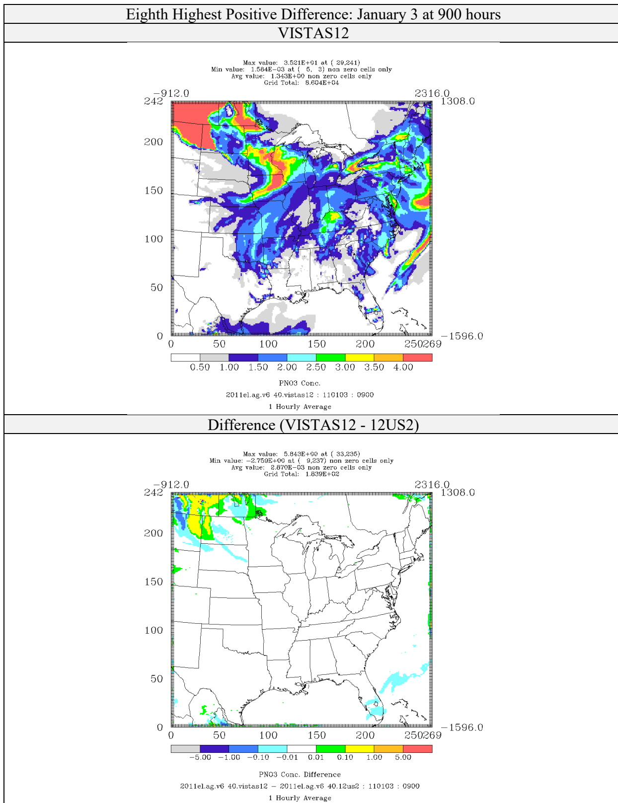
Figure 4-71: Comparison of Nitrate Concentrations ( \mu\text{g}/\text{m}^3 ) for CAMx 6.40 on VISTAS12 and 12US2 domains 2011el Simulations (Eighth Highest Positive Difference)
