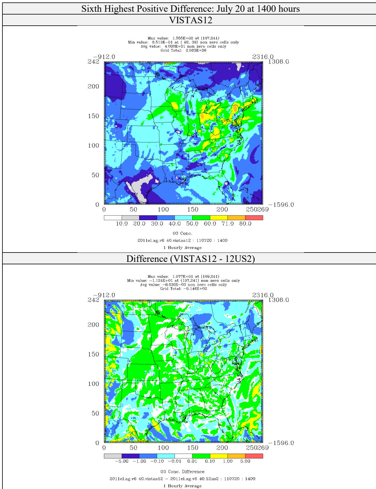
Figure 4-6: Comparison of Ozone Concentrations (ppb) for CAMx 6.40 on VISTAS12 and 12US2 domains 2011el Simulations (Sixth Highest Positive Difference)
