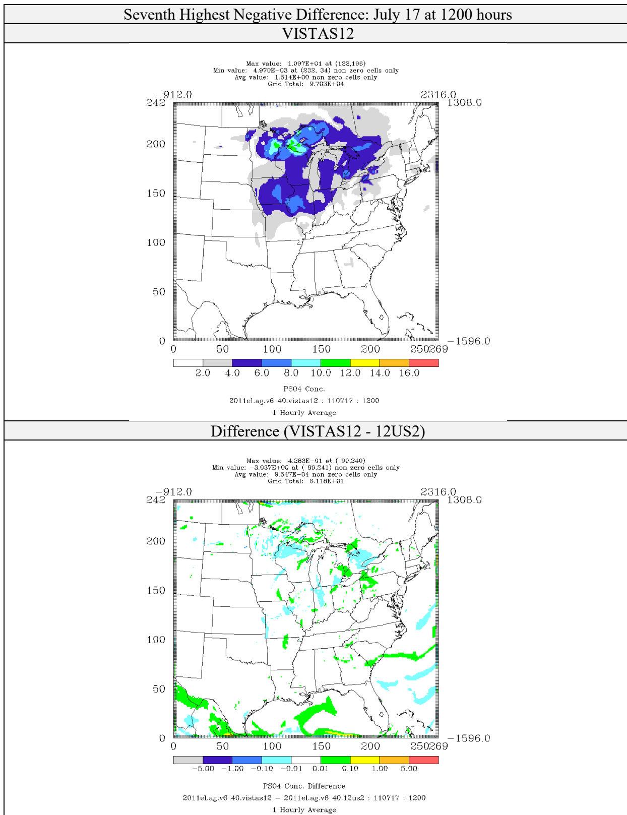
Figure 4-59: Comparison of Sulfate Concentrations ( \mu\text{g}/\text{m}^3 ) for CAMx 6.40 on VISTAS12 and 12US2 domains 2011el Simulations (Seventh Highest Negative Difference)
