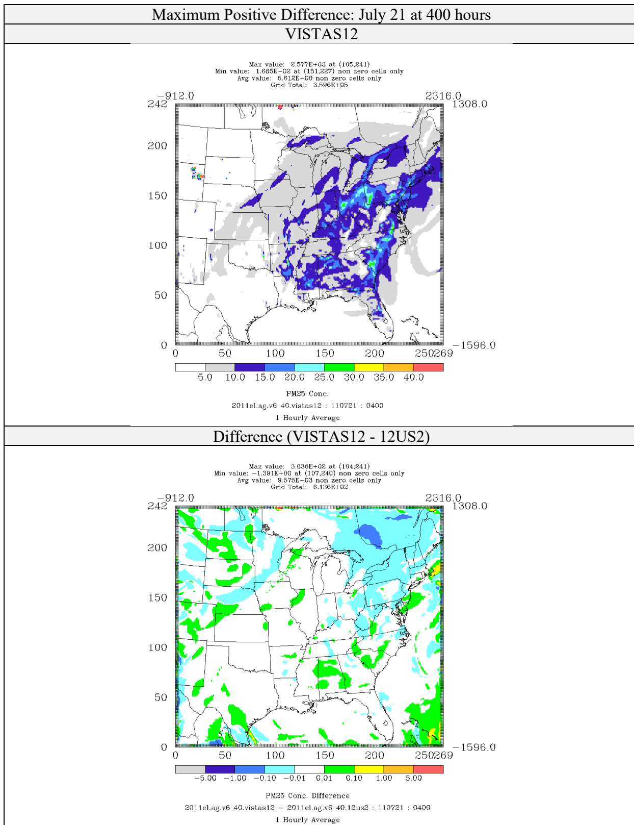
Figure 4-22: Comparison of PM 2.5 Concentrations ( \mu\text{g}/\text{m}^3 ) for CAMx 6.40 on VISTAS12 and 12US2 domains 2011el Simulations (Maximum Positive Difference)
