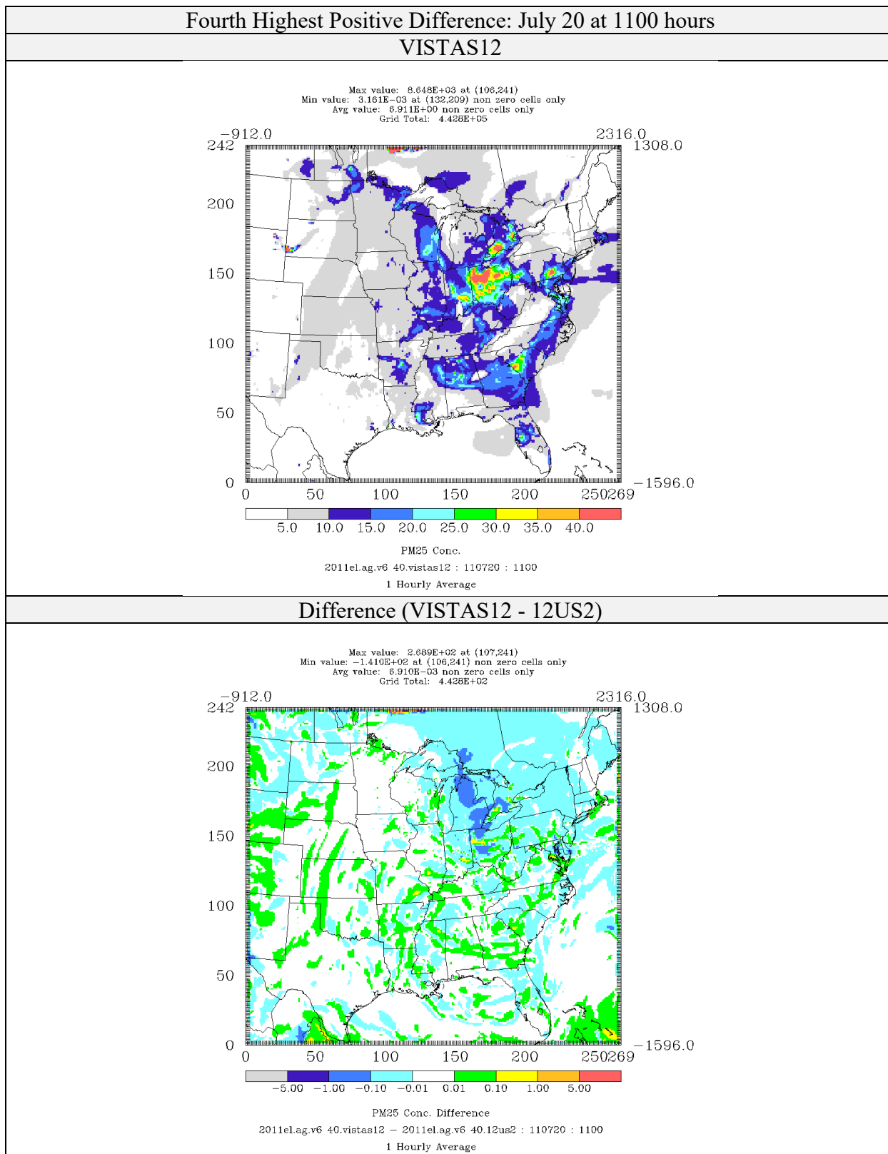
Figure 4-25: Comparison of PM 2.5 Concentrations ( \mu\text{g}/\text{m}^3 ) for CAMx 6.40 on VISTAS12 and 12US2 domains 2011el Simulations (Fourth Highest Positive Difference)
