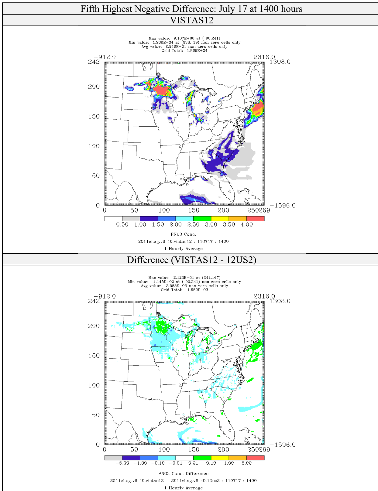
Figure 4-78: Comparison of Nitrate Concentrations ( \mu\text{g}/\text{m}^3 ) for CAMx 6.40 on VISTAS12 and 12US2 domains 2011el Simulations (Fifth Highest Negative Difference)
