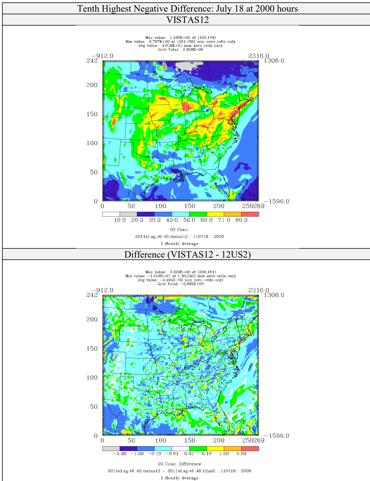
Figure 4-20: Comparison of Ozone Concentrations (ppb) for CAMx 6.40 on VISTAS12 and 12US2 domains 2011el Simulations (Tenth Highest Negative Difference)
