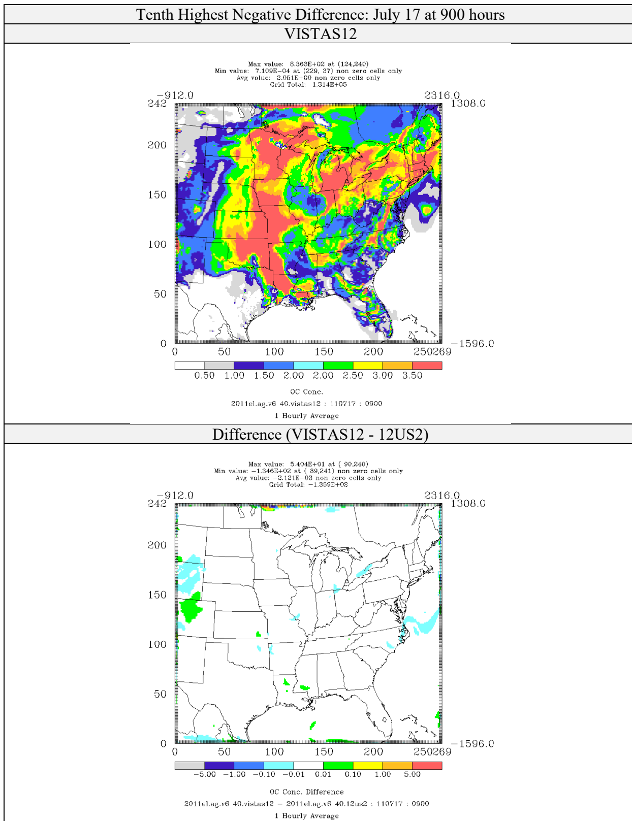
Figure 4-104: Comparison of Organic Matter Concentrations ( \mu\text{g}/\text{m}^3 ) for CAMx 6.40 on VISTAS12 and 12US2 domains 2011el Simulations (Tenth Highest Negative Difference)
