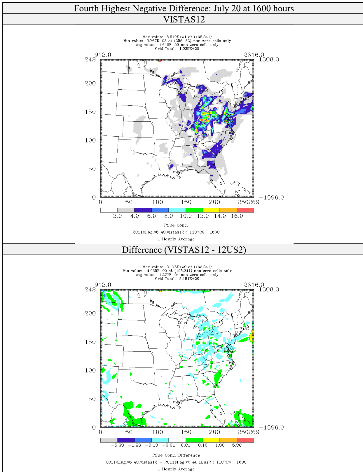
Figure 4-56: Comparison of Sulfate Concentrations ( \mu\text{g}/\text{m}^3 ) for CAMx 6.40 on VISTAS12 and 12US2 domains 2011el Simulations (Fourth Highest Negative Difference)
