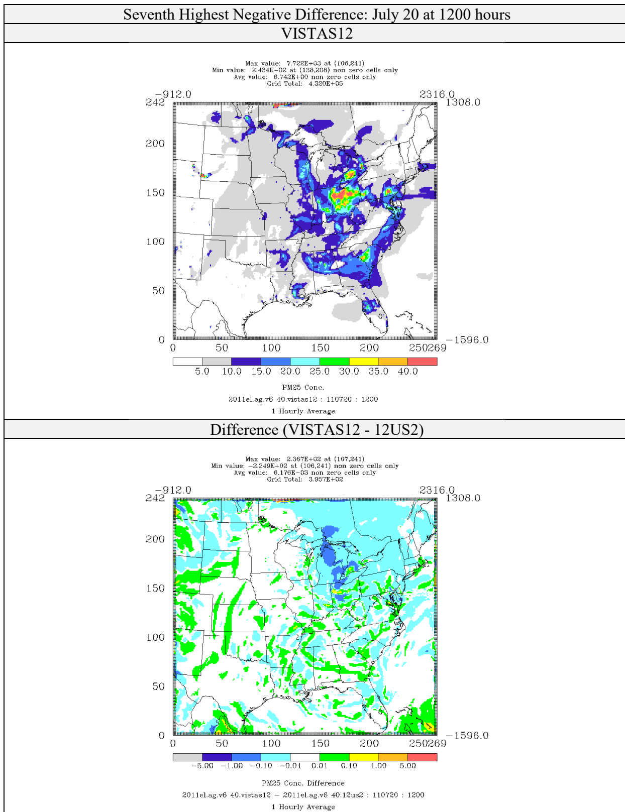
Figure 4-38: Comparison of PM 2.5 Concentrations ( \mu\text{g}/\text{m}^3 ) for CAMx 6.40 on VISTAS12 and 12US2 domains 2011el Simulations (Seventh Highest Negative Difference)
