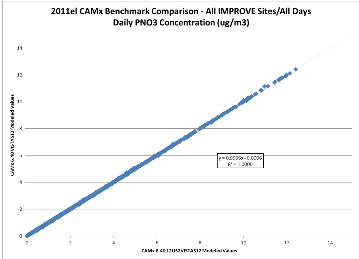
Figure 4-84: Scatterplot Comparing 24-hour Average Predicted Nitrate Concentrations ( \mu\text{g}/\text{m}^3 ) for All Days at all IMPROVE Monitor Locations for CAMx 6.40 on VISTAS12 and 12US2 domains 2011el Simulations Performed by VISTAS (Alpine).
