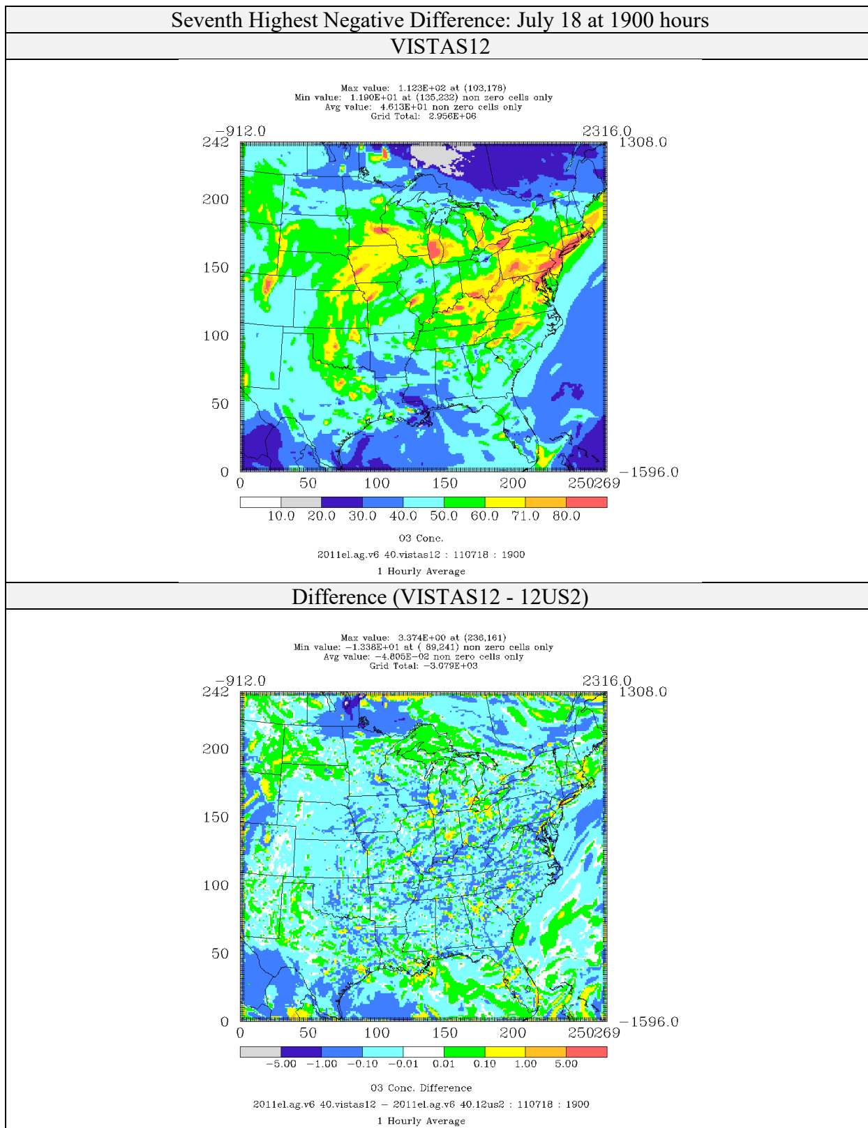
Figure 4-17: Comparison of Ozone Concentrations (ppb) for CAMx 6.40 on VISTAS12 and 12US2 domains 2011el Simulations (Seventh Highest Negative Difference)
