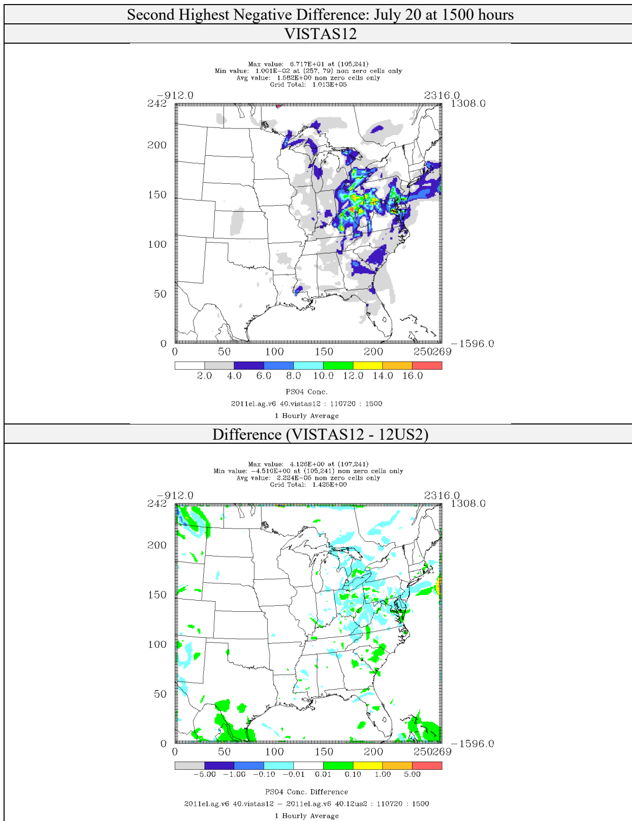
Figure 4-54: Comparison of Sulfate Concentrations ( \mu\text{g}/\text{m}^3 ) for CAMx 6.40 on VISTAS12 and 12US2 domains 2011el Simulations (Second Highest Negative Difference)
