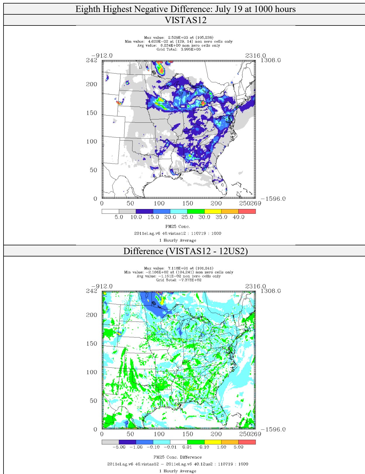
Figure 4-39: Comparison of PM 2.5 Concentrations ( \mu\text{g}/\text{m}^3 ) for CAMx 6.40 on VISTAS12 and 12US2 domains 2011el Simulations (Eighth Highest Negative Difference)
