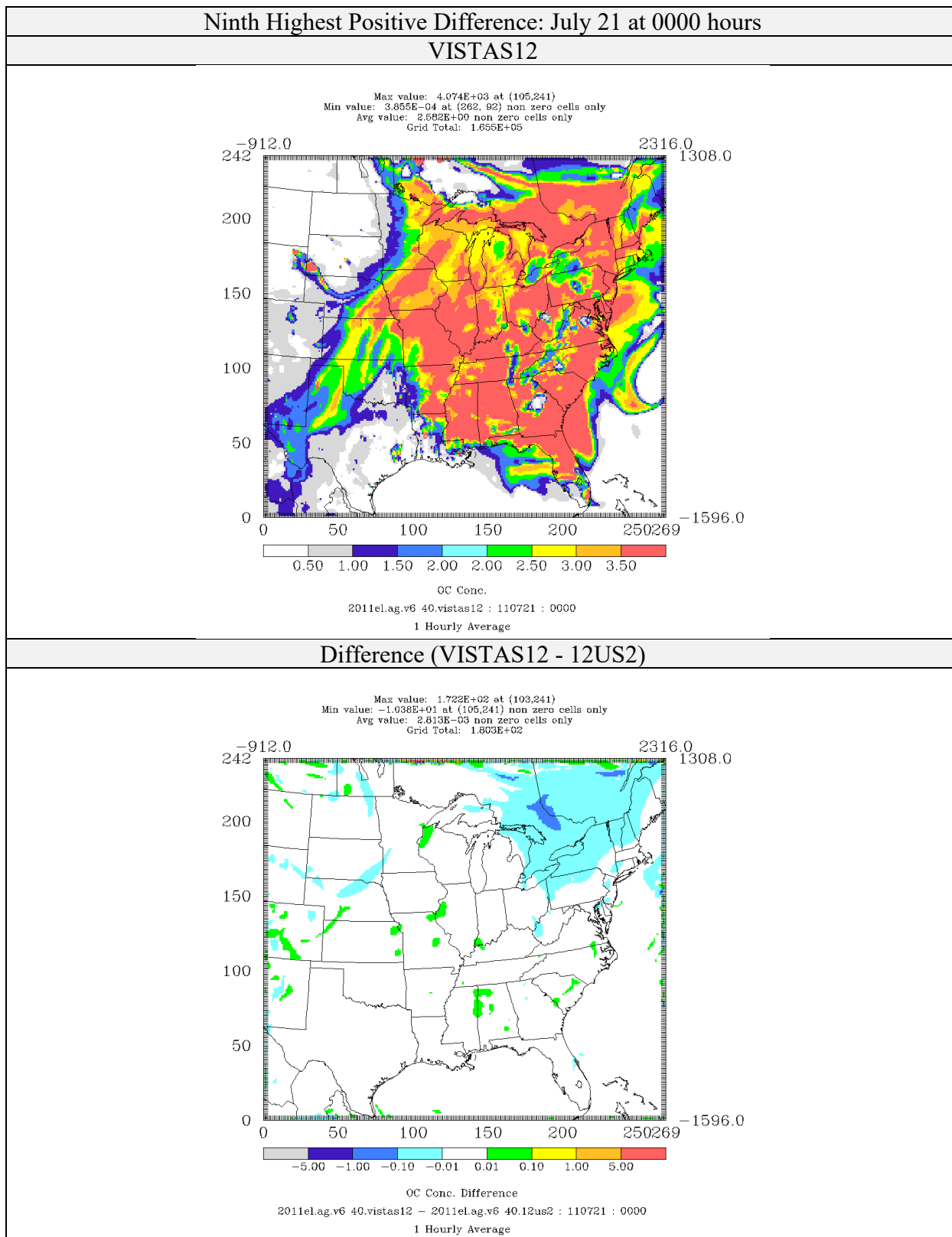
Figure 4-93: Comparison of Organic Matter Concentrations ( \mu\text{g}/\text{m}^3 ) for CAMx 6.40 on VISTAS12 and 12US2 domains 2011el Simulations (Ninth Highest Positive Difference)
