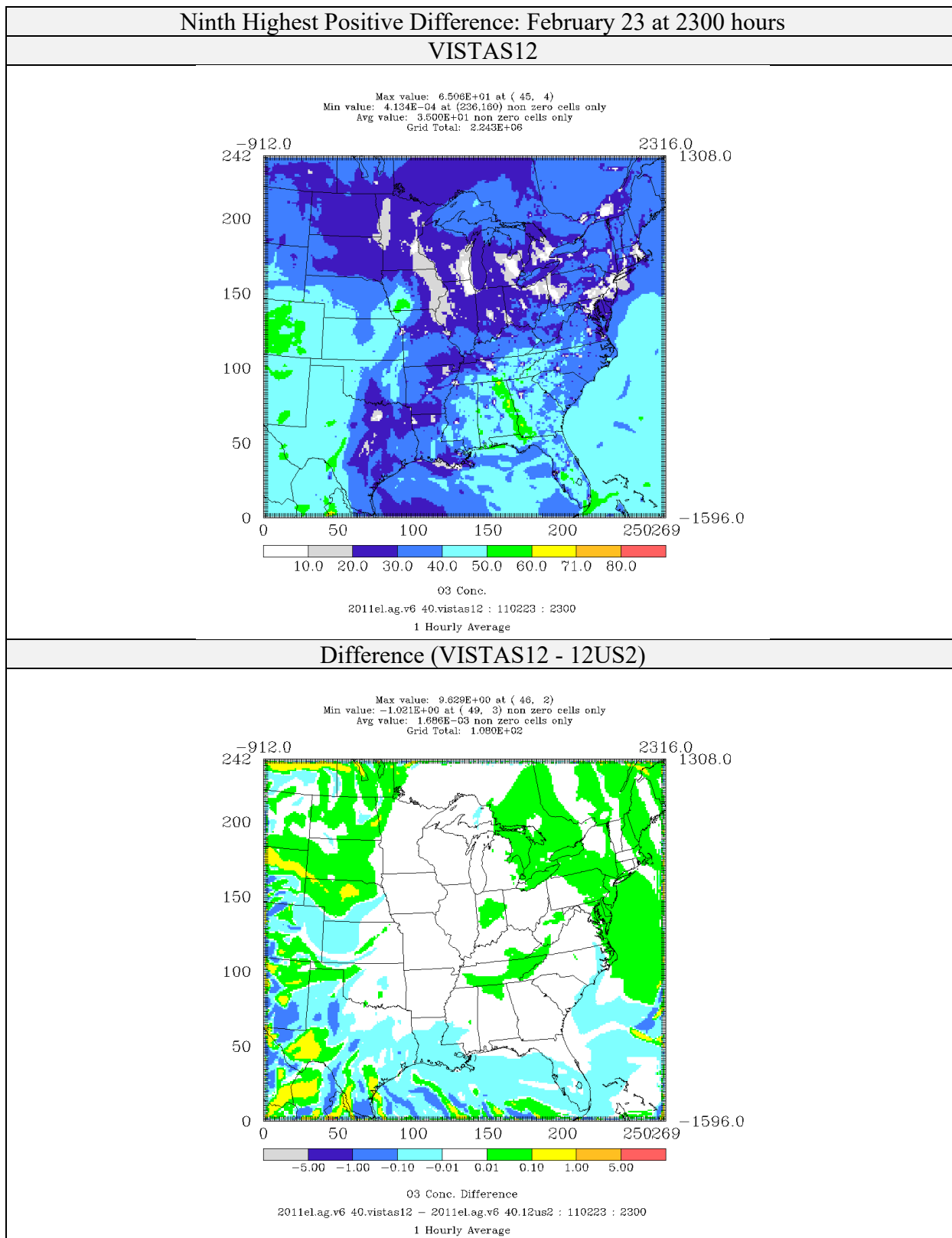
Figure 4-9: Comparison of Ozone Concentrations (ppb) for CAMx 6.40 on VISTAS12 and 12US2 domains 2011el Simulations (Ninth Highest Positive Difference)
