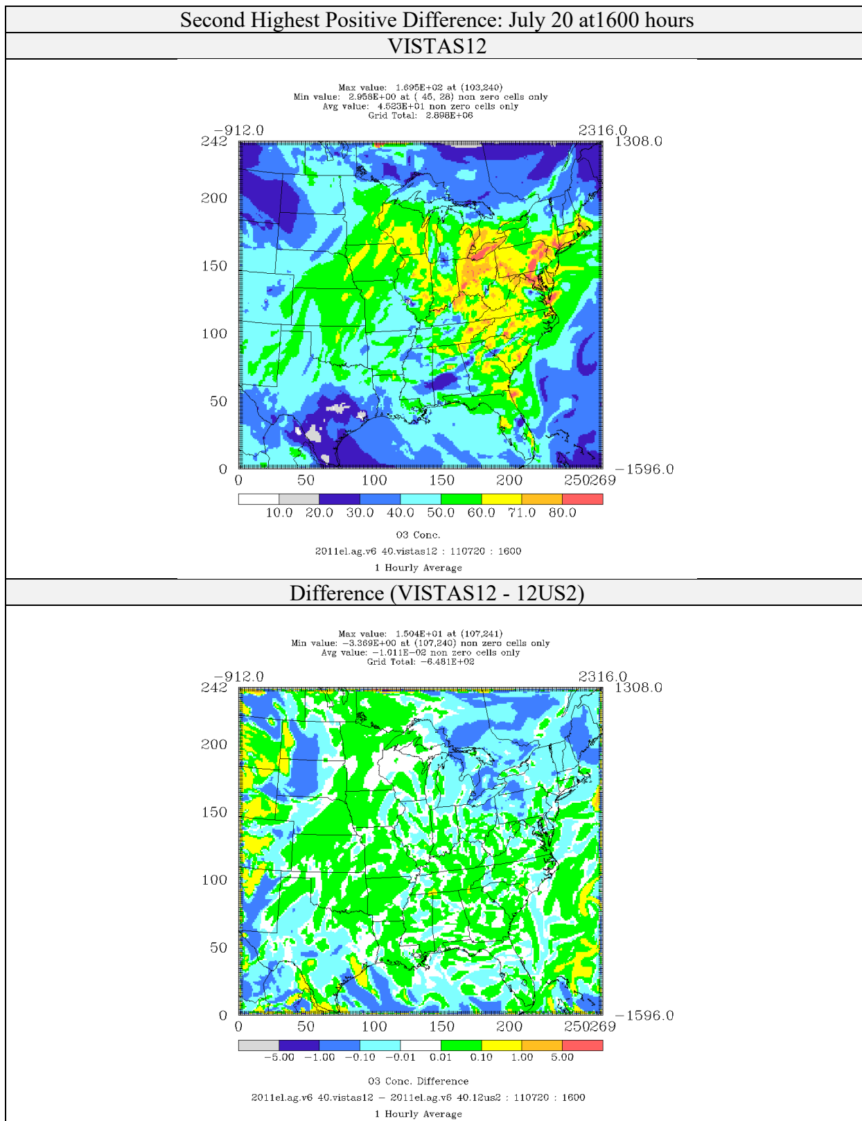
Figure 4-2: Comparison of Ozone Concentrations (ppb) for CAMx 6.40 on VISTAS12 and 12US2 domains 2011el Simulations (Second Highest Positive Difference)
