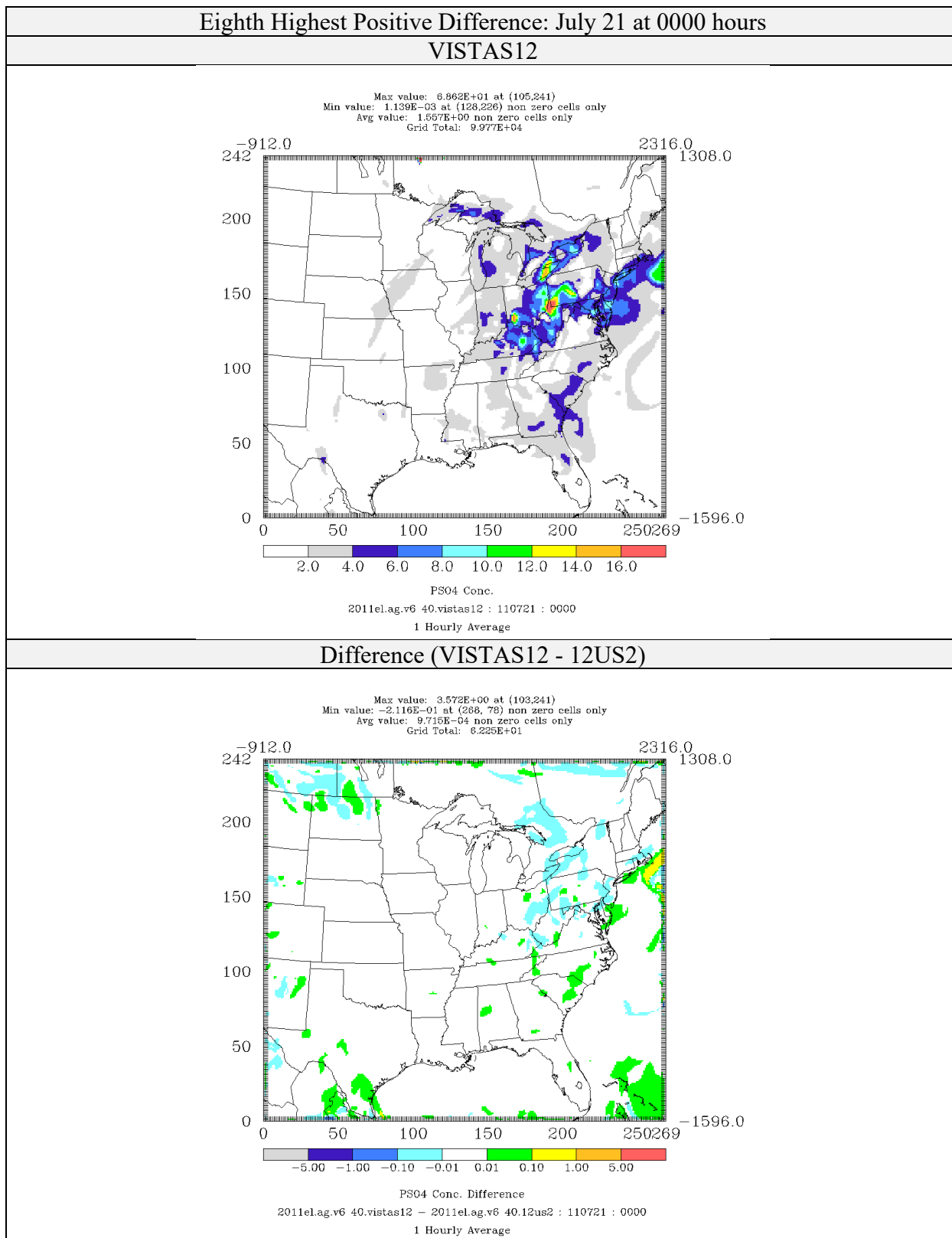
Figure 4-50: Comparison of Sulfate Concentrations ( \mu\text{g}/\text{m}^3 ) for CAMx 6.40 on VISTAS12 and 12US2 domains 2011el Simulations (Eighth Highest Positive Difference)
