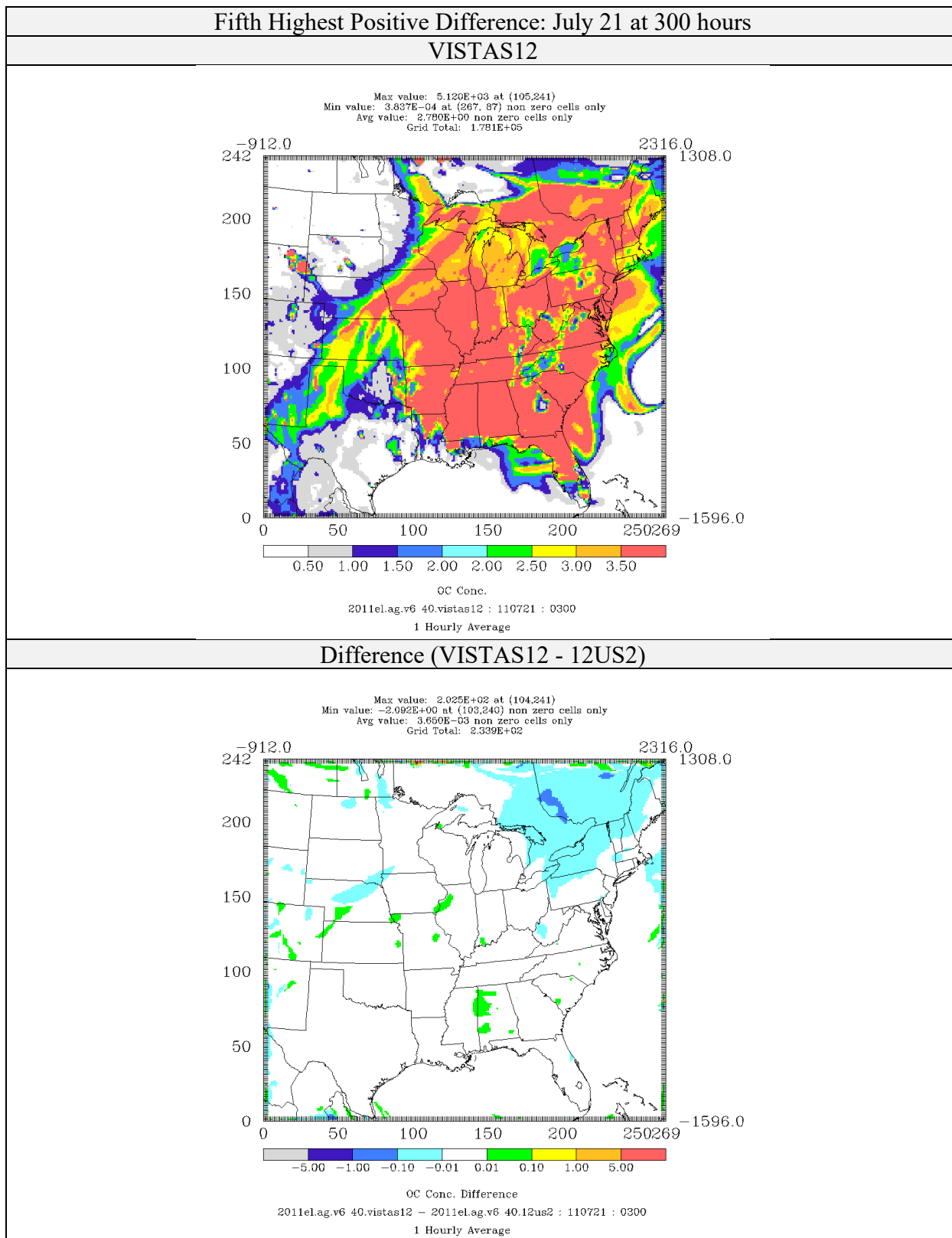
Figure 4-89: Comparison of Organic Matter Concentrations ( \mu\text{g}/\text{m}^3 ) for CAMx 6.40 on VISTAS12 and 12US2 domains 2011el Simulations (Fifth Highest Positive Difference)
