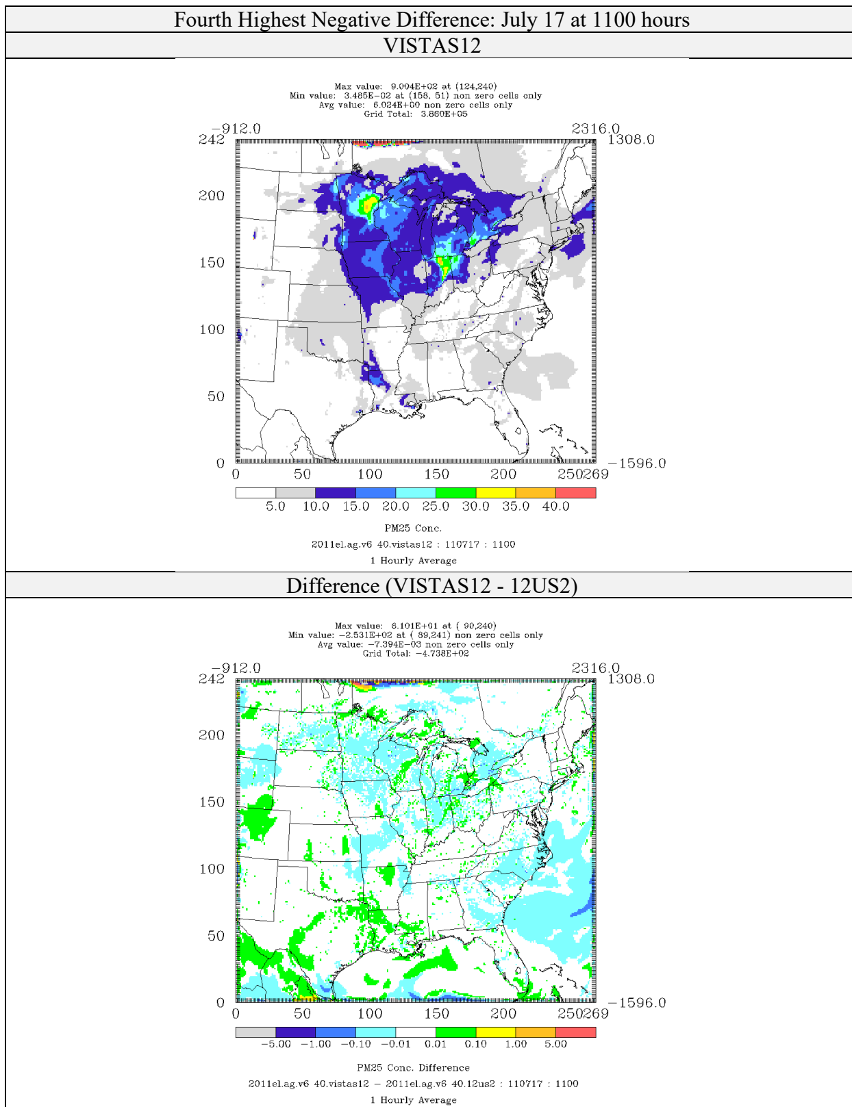
Figure 4-35: Comparison of PM 2.5 Concentrations ( \mu\text{g}/\text{m}^3 ) for CAMx 6.40 on VISTAS12 and 12US2 domains 2011el Simulations (Fourth Highest Negative Difference)
