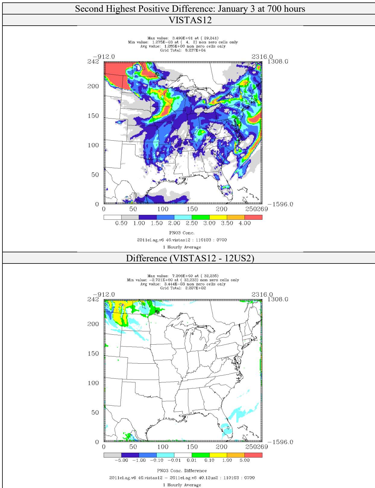
Figure 4-65: Comparison of Nitrate Concentrations ( \mu\text{g}/\text{m}^3 ) for CAMx 6.40 on VISTAS12 and 12US2 domains 2011el Simulations (Second Highest Positive Difference)
