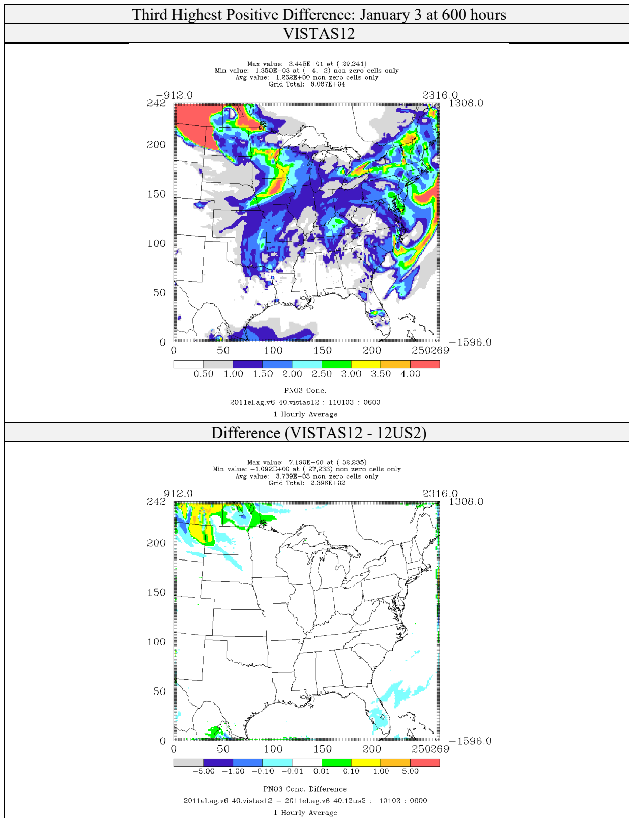
Figure 4-66: Comparison of Nitrate Concentrations ( \mu\text{g}/\text{m}^3 ) for CAMx 6.40 on VISTAS12 and 12US2 domains 2011el Simulations (Third Highest Positive Difference)
