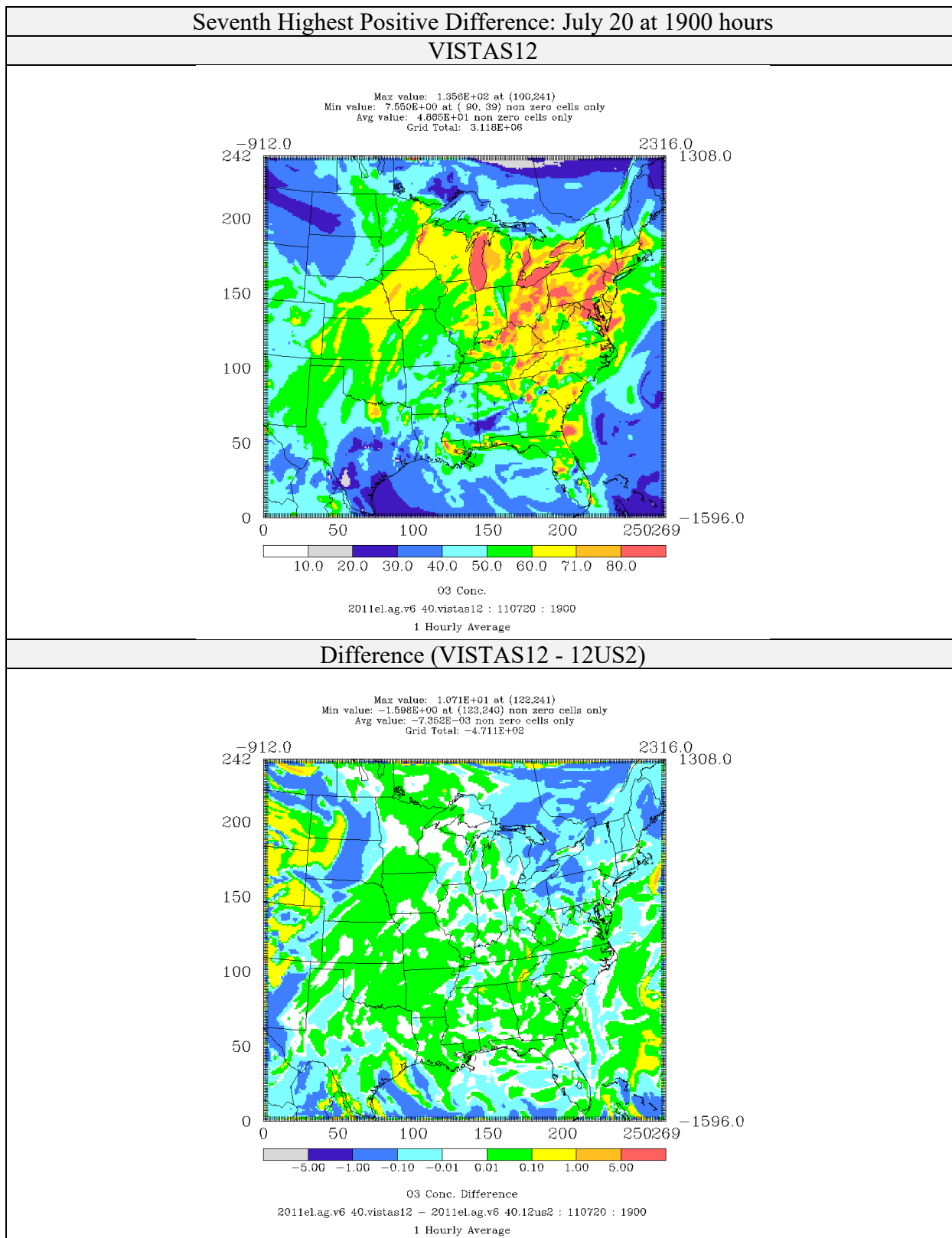
Figure 4-7: Comparison of Ozone Concentrations (ppb) for CAMx 6.40 on VISTAS12 and 12US2 domains 2011el Simulations (Seventh Highest Positive Difference)
