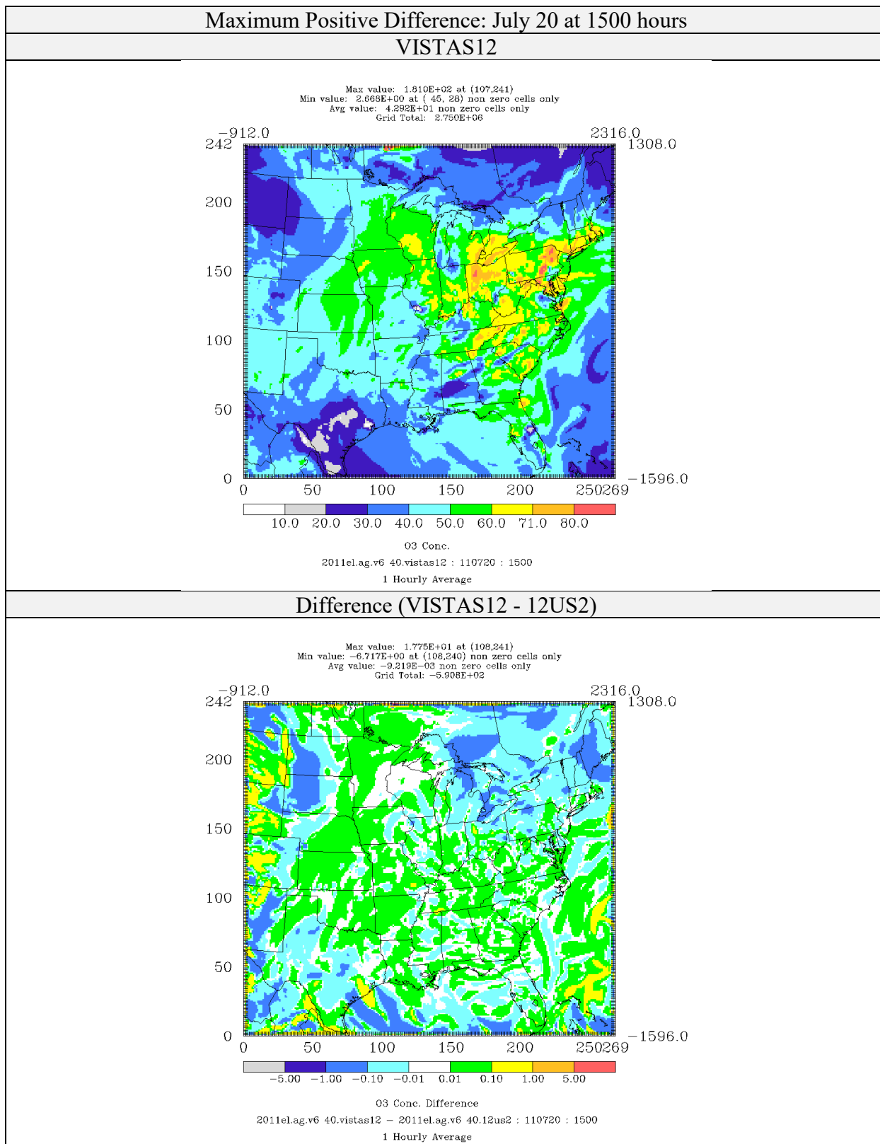
Figure 4-1: Comparison of Ozone Concentrations (ppb) for CAMx 6.40 on VISTAS12 and 12US2 domains 2011el Simulations (Maximum Positive Difference)
