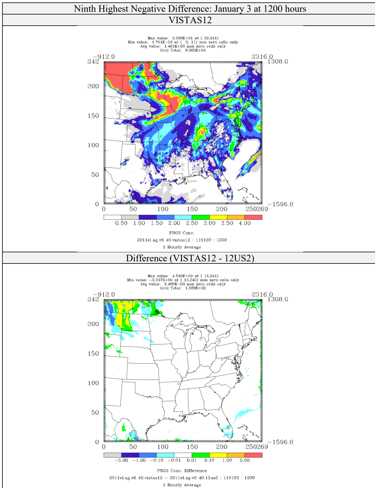
Figure 4-82: Comparison of Nitrate Concentrations ( \mu\text{g}/\text{m}^3 ) for CAMx 6.40 on VISTAS12 and 12US2 domains 2011el Simulations (Ninth Highest Negative Difference)
