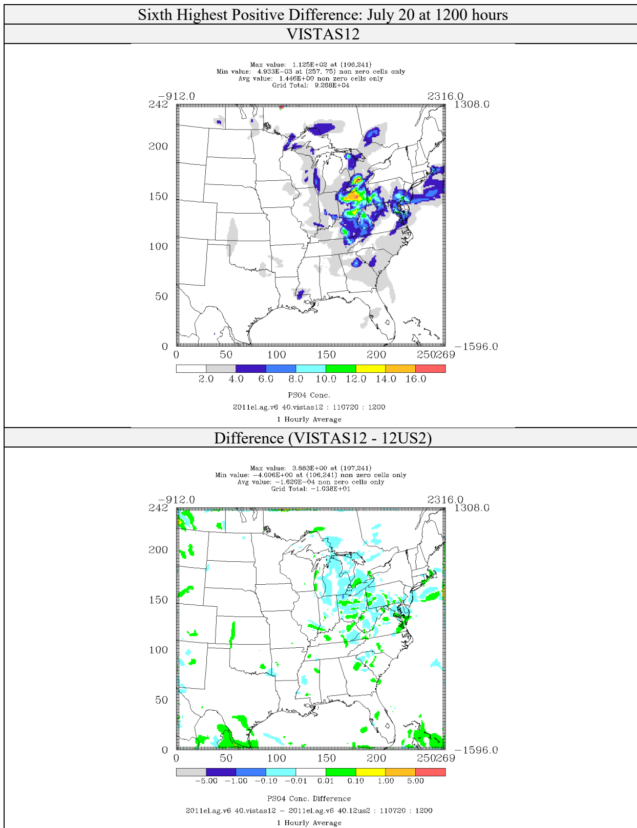
Figure 4-48: Comparison of Sulfate Concentrations ( \mu\text{g}/\text{m}^3 ) for CAMx 6.40 on VISTAS12 and 12US2 domains 2011el Simulations (Sixth Highest Positive Difference)
