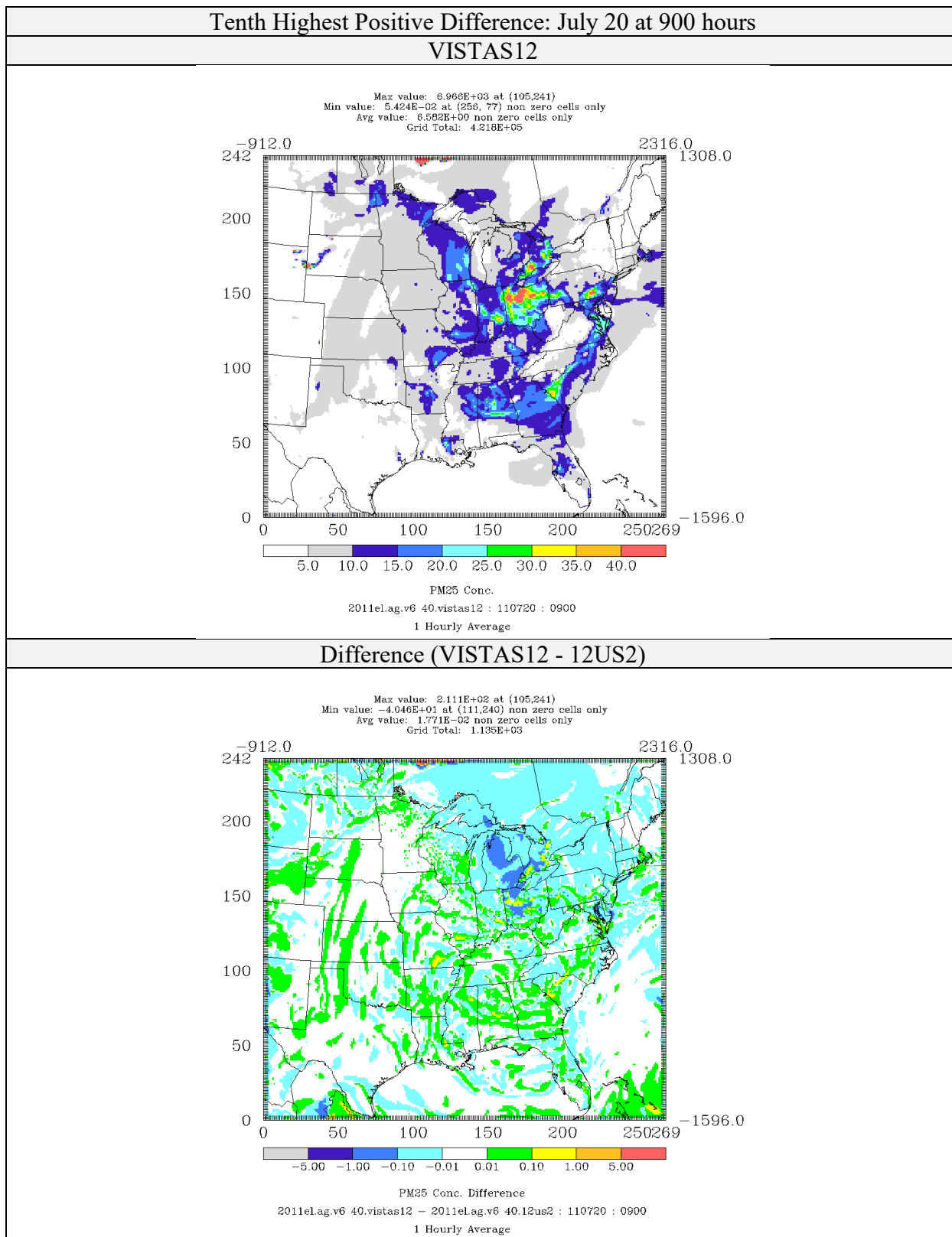
Figure 4-31: Comparison of PM 2.5 Concentrations ( \mu\text{g}/\text{m}^3 ) for CAMx 6.40 on VISTAS12 and 12US2 domains 2011el Simulations (Tenth Highest Positive Difference)
