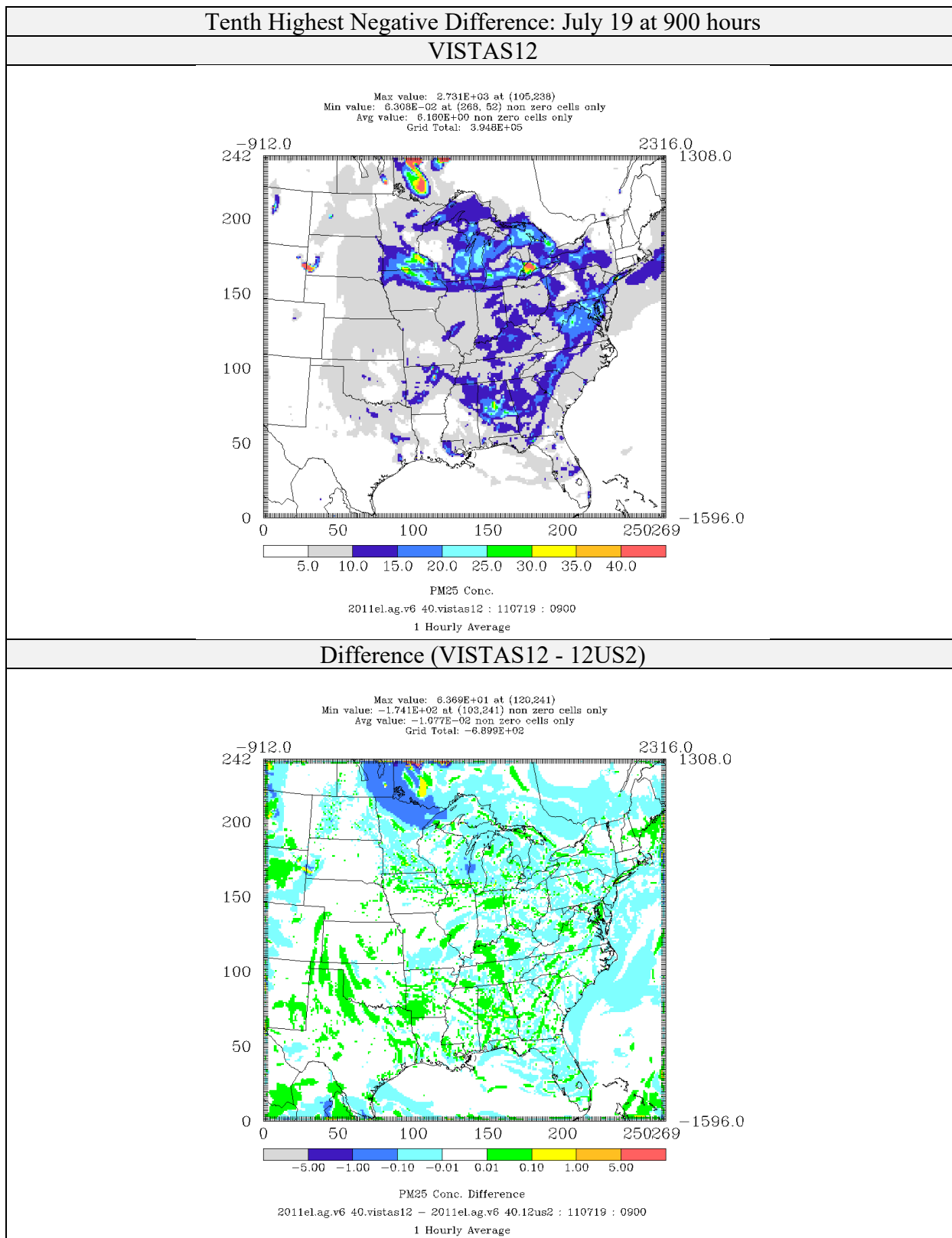
Figure 4-41: Comparison of PM 2.5 Concentrations ( \mu\text{g}/\text{m}^3 ) for CAMx 6.40 on VISTAS12 and 12US2 domains 2011el Simulations (Tenth Highest Negative Difference)
