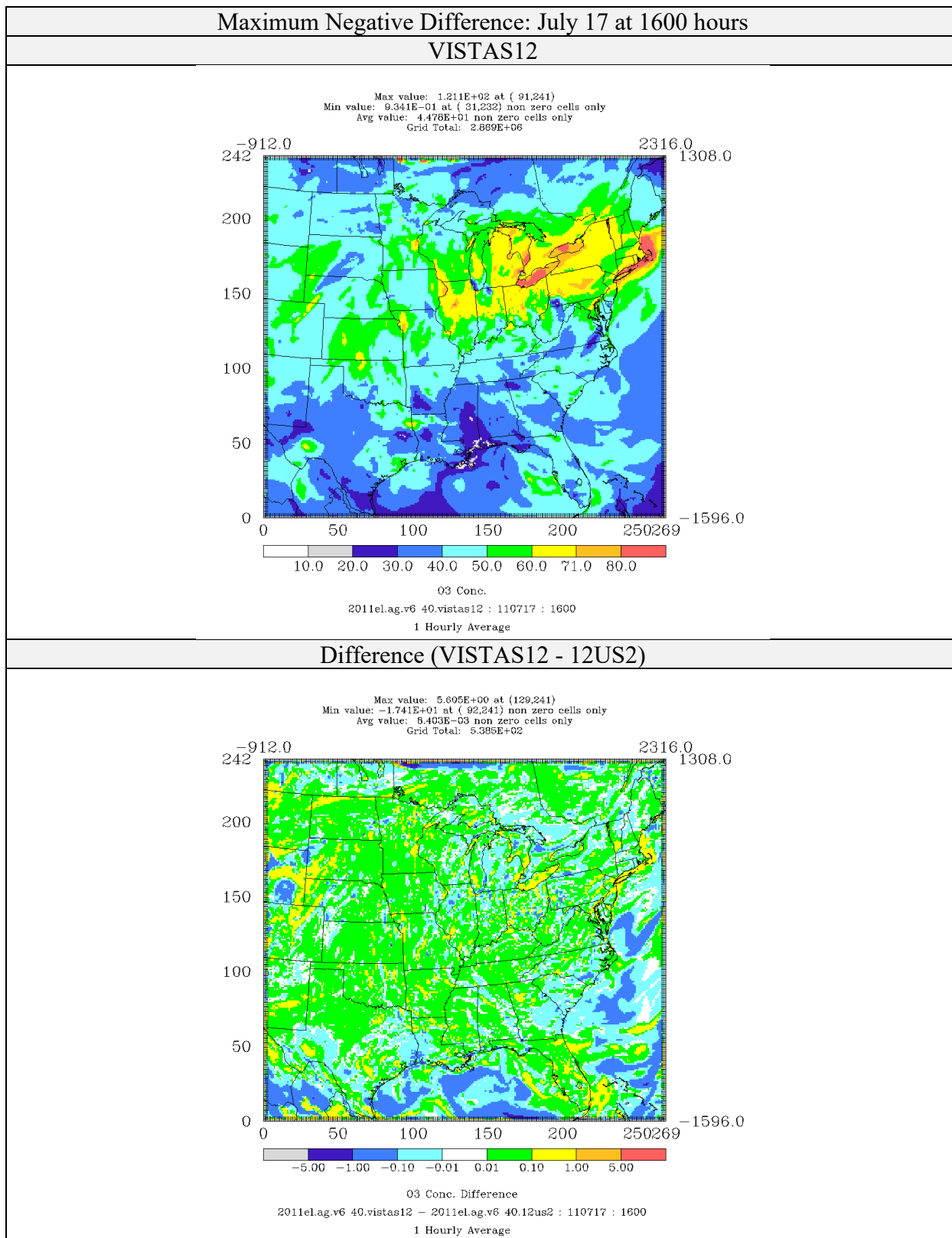
Figure 4-11: Comparison of Ozone Concentrations (ppb) for CAMx 6.40 on VISTAS12 and 12US2 domains 2011el Simulations (Maximum Negative Difference)
