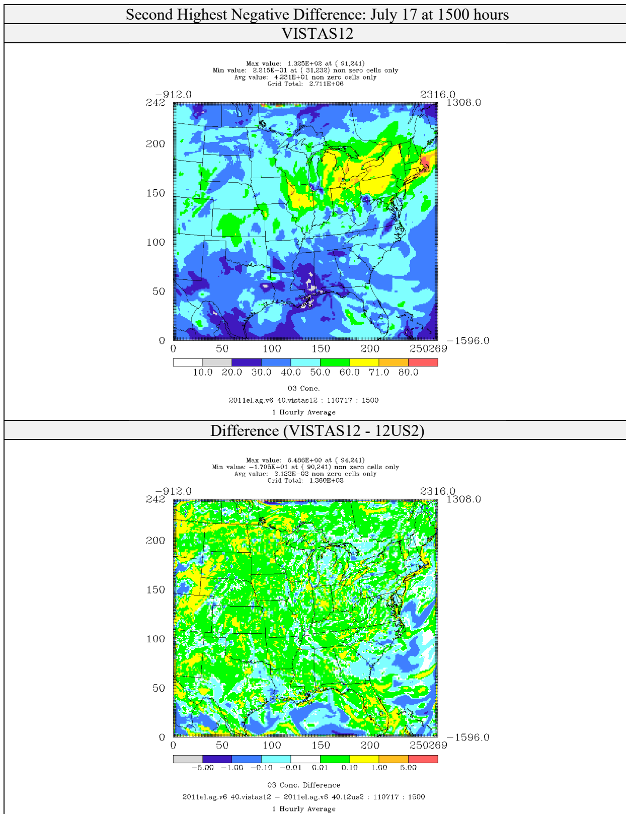
Figure 4-12: Comparison of Ozone Concentrations (ppb) for CAMx 6.40 on VISTAS12 and 12US2 domains 2011el Simulations (Second Highest Negative Difference)
