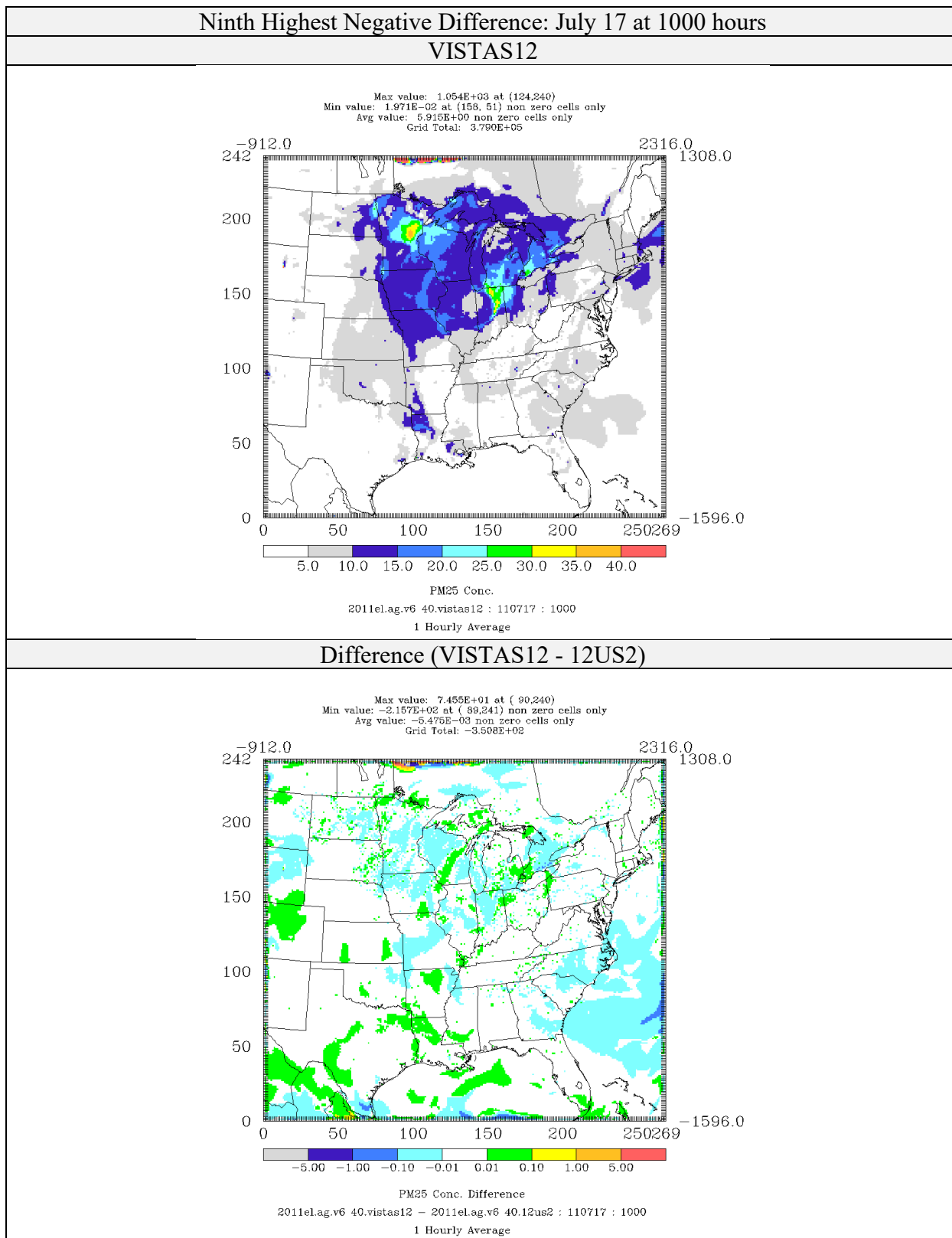
Figure 4-40: Comparison of PM 2.5 Concentrations ( \mu\text{g}/\text{m}^3 ) for CAMx 6.40 on VISTAS12 and 12US2 domains 2011el Simulations (Ninth Highest Negative Difference)
