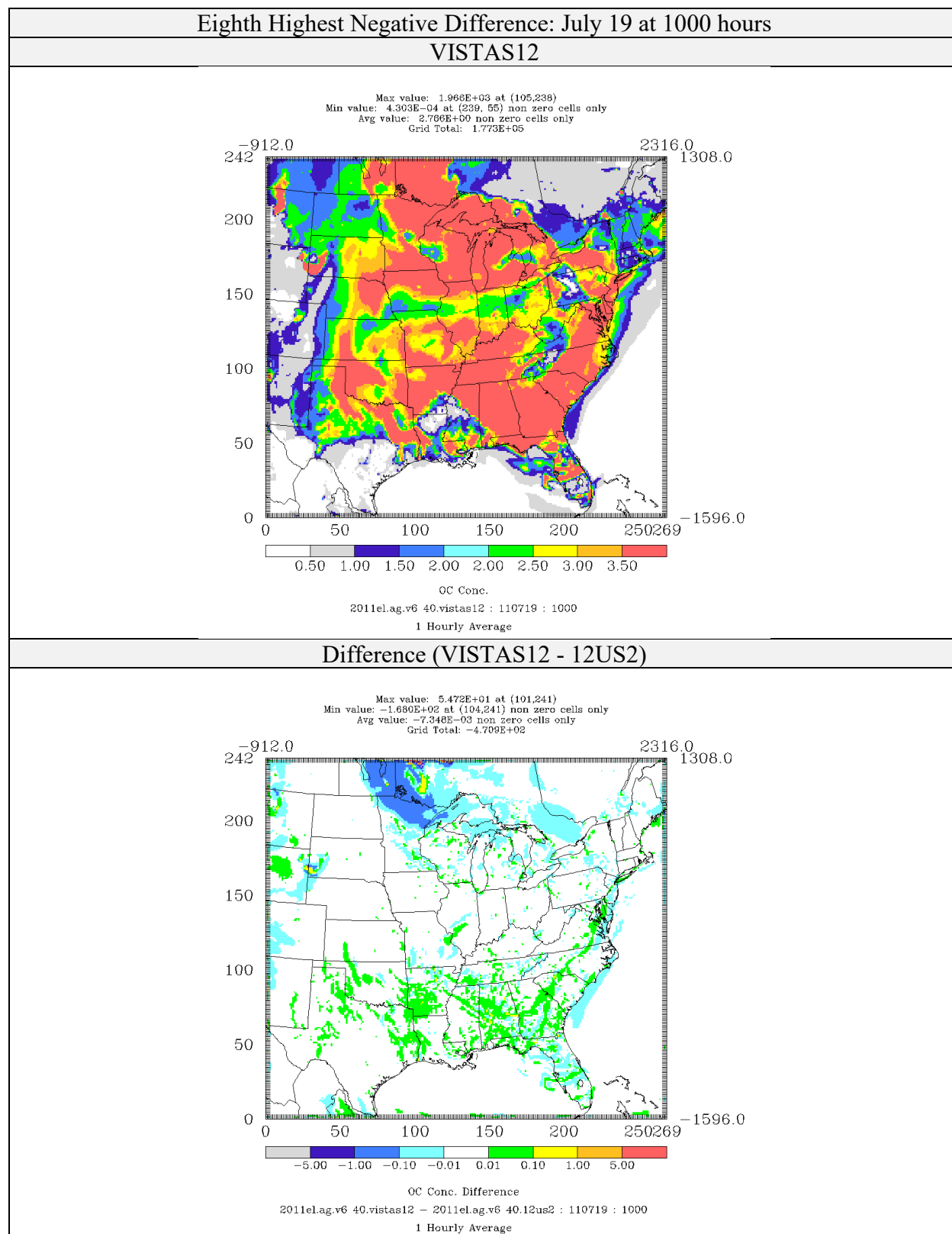
Figure 4-102: Comparison of Organic Matter Concentrations ( \mu\text{g}/\text{m}^3 ) for CAMx 6.40 on VISTAS12 and 12US2 domains 2011el Simulations (Eighth Highest Negative Difference)
