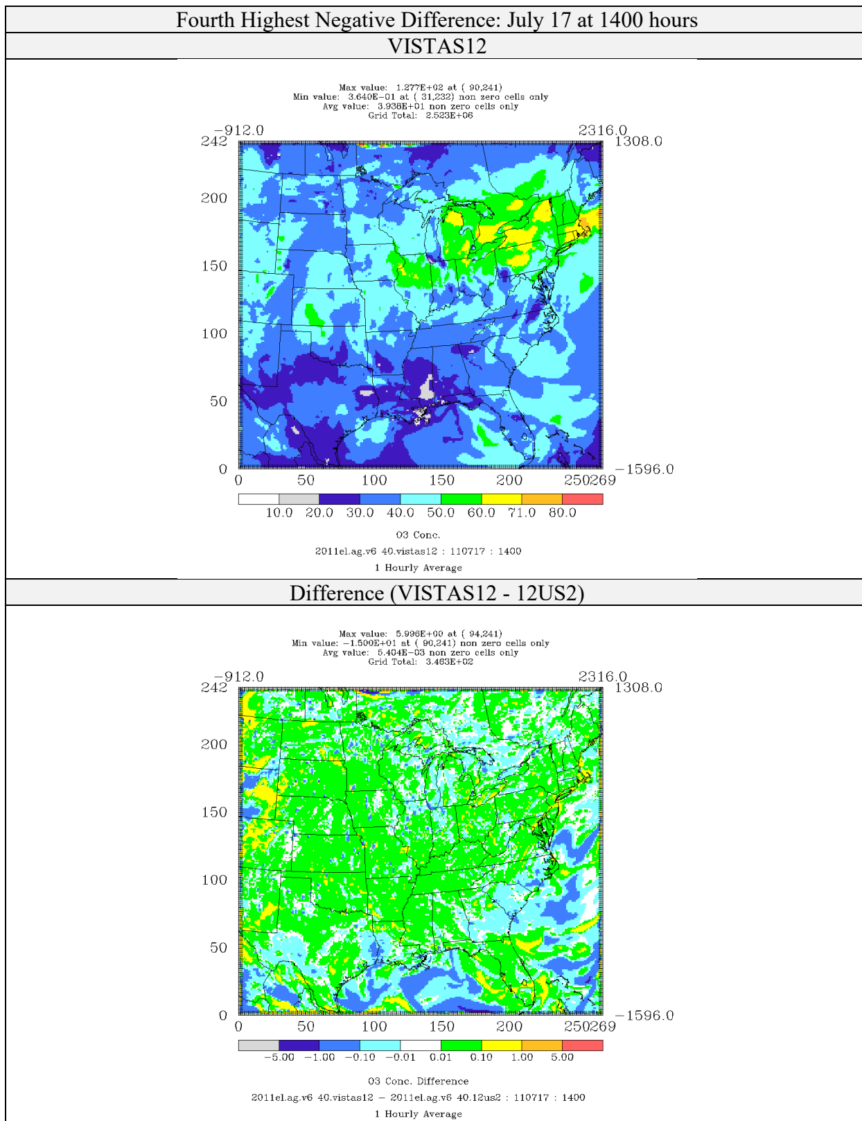
Figure 4-14: Comparison of Ozone Concentrations (ppb) for CAMx 6.40 on VISTAS12 and 12US2 domains 2011el Simulations (Fourth Highest Negative Difference)
