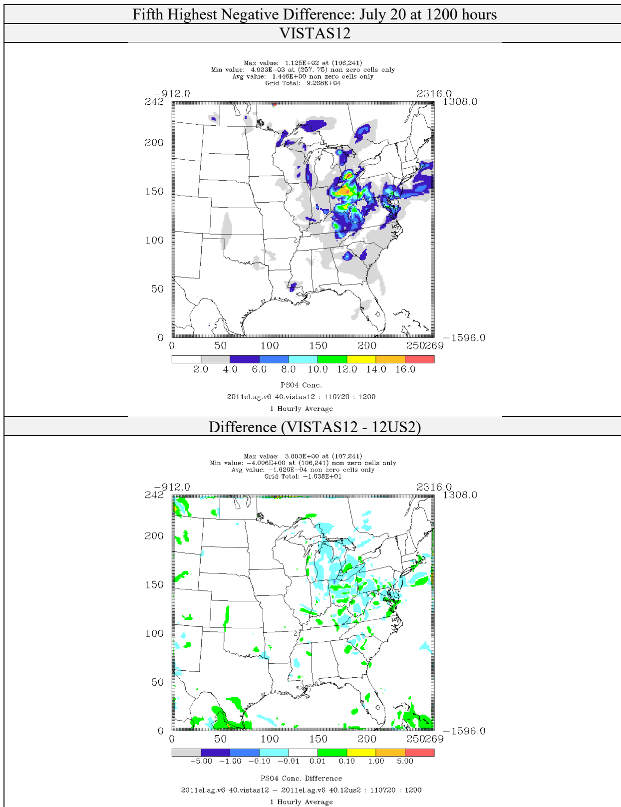
Figure 4-57: Comparison of Sulfate Concentrations ( \mu\text{g}/\text{m}^3 ) for CAMx 6.40 on VISTAS12 and 12US2 domains 2011el Simulations (Fifth Highest Negative Difference)
