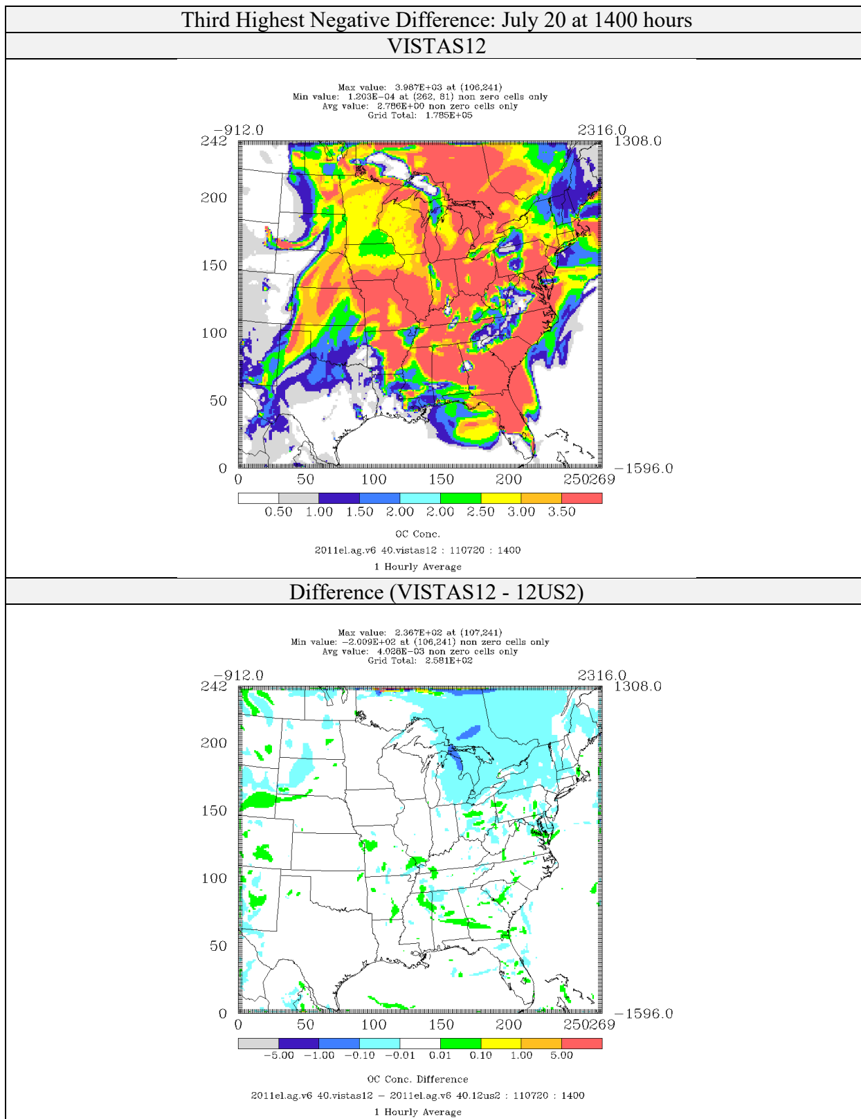
Figure 4-97: Comparison of Organic Matter Concentrations ( \mu\text{g}/\text{m}^3 ) for CAMx 6.40 on VISTAS12 and 12US2 domains 2011el Simulations (Third Highest Negative Difference)
