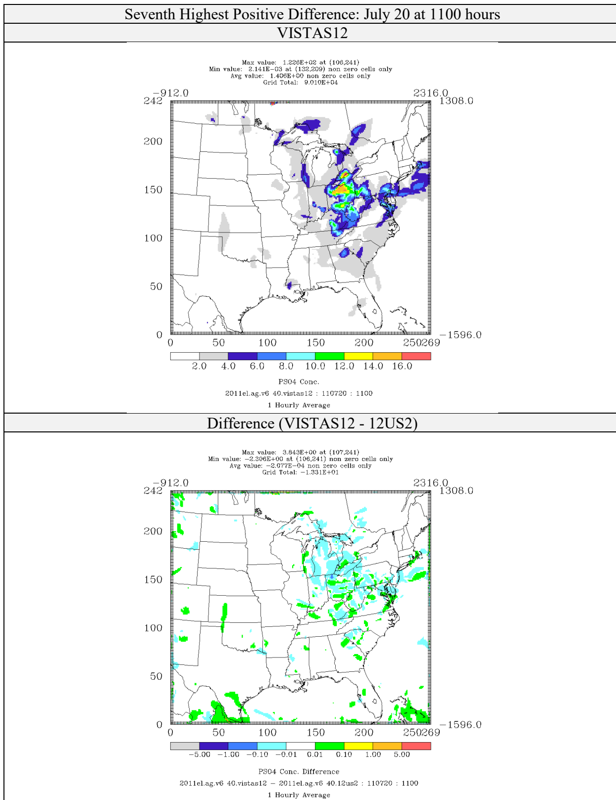
Figure 4-49: Comparison of Sulfate Concentrations ( \mu\text{g}/\text{m}^3 ) for CAMx 6.40 on VISTAS12 and 12US2 domains 2011el Simulations
