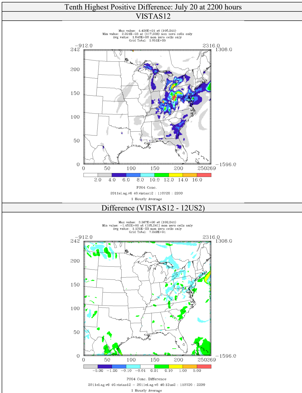
Figure 4-52: Comparison of Sulfate Concentrations ( \mu\text{g}/\text{m}^3 ) for CAMx 6.40 on VISTAS12 and 12US2 domains 2011el Simulations (Tenth Highest Positive Difference)
