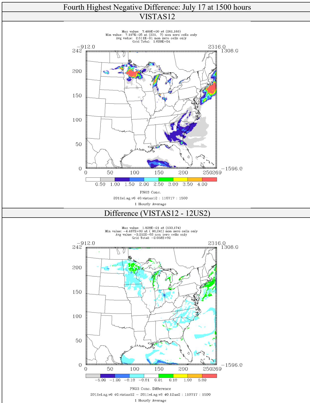
Figure 4-77: Comparison of Nitrate Concentrations ( \mu\text{g}/\text{m}^3 ) for CAMx 6.40 on VISTAS12 and 12US2 domains 2011el Simulations (Fourth Highest Negative Difference)
