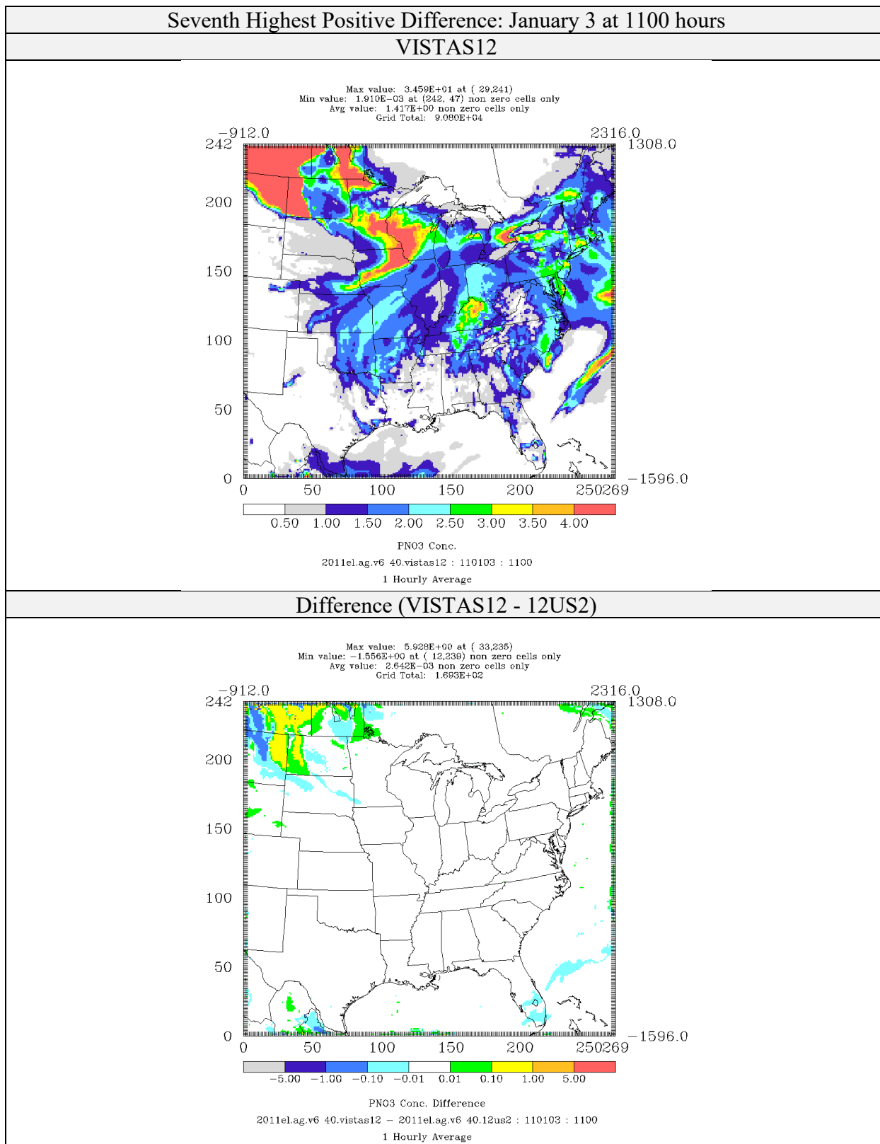
Figure 4-70: Comparison of Nitrate Concentrations ( \mu\text{g}/\text{m}^3 ) for CAMx 6.40 on VISTAS12 and 12US2 domains 2011el Simulations (Seventh Highest Positive Difference)
