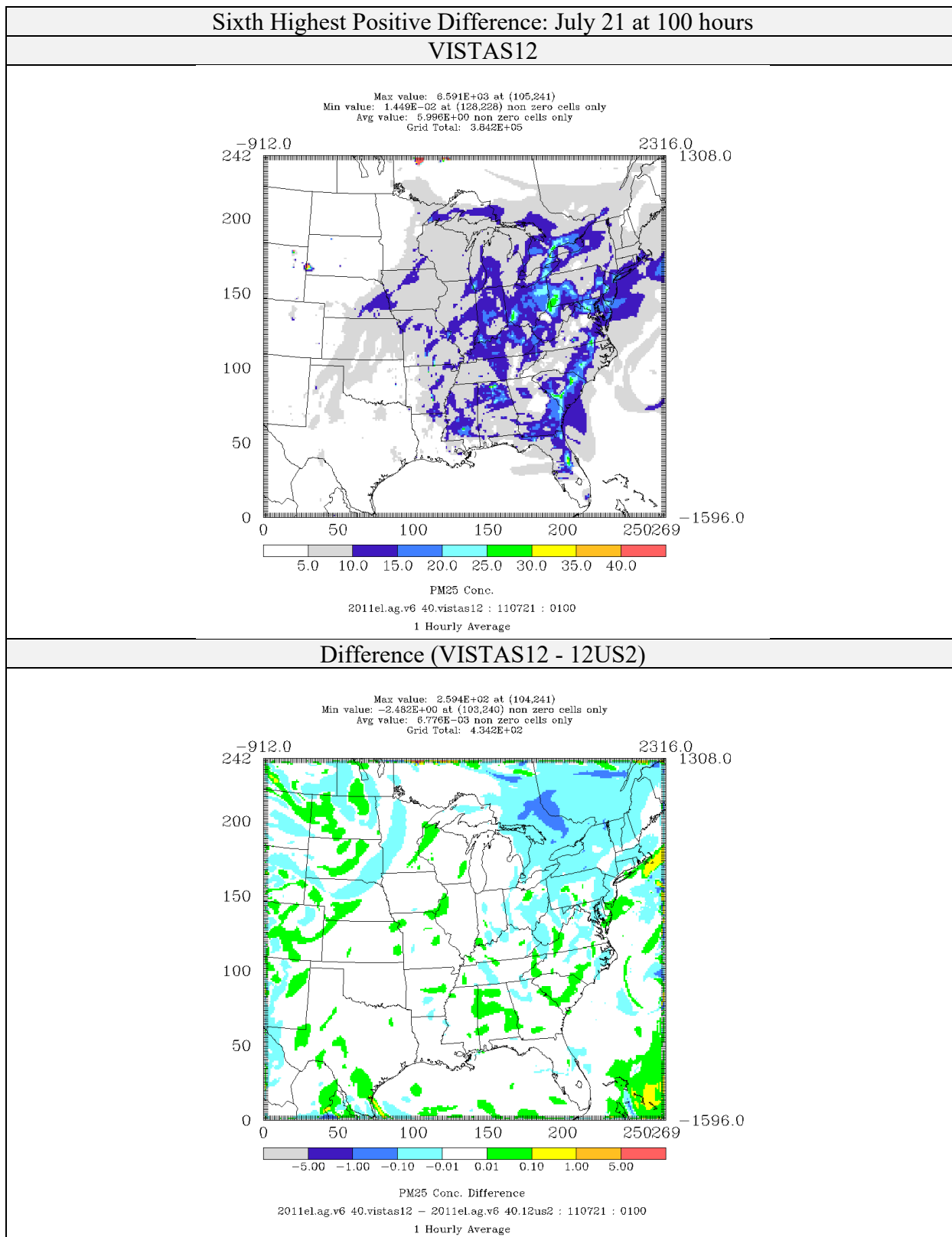
Figure 4-27: Comparison of PM 2.5 Concentrations ( \mu\text{g}/\text{m}^3 ) for CAMx 6.40 on VISTAS12 and 12US2 domains 2011el Simulations (Sixth Highest Positive Difference)
