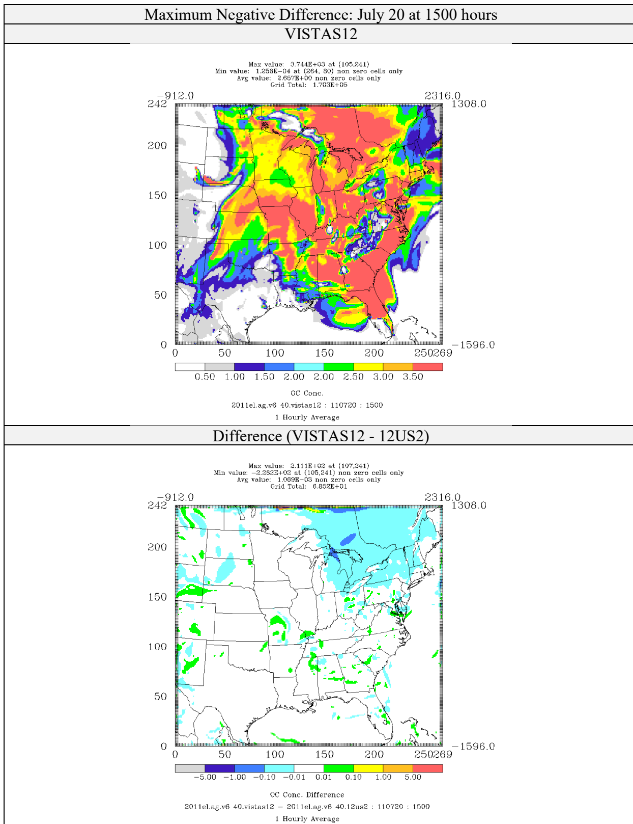
Figure 4-95: Comparison of Organic Matter Concentrations ( \mu\text{g}/\text{m}^3 ) for CAMx 6.40 on VISTAS12 and 12US2 domains 2011el Simulations (Maximum Negative Difference)
