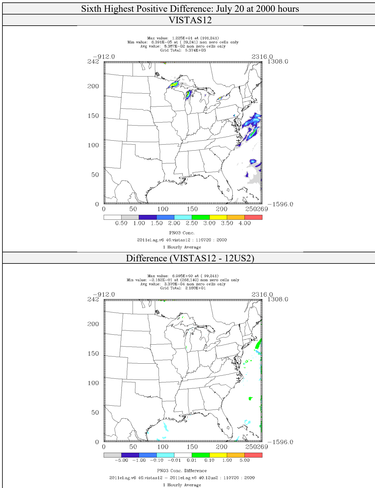
Figure 4-69: Comparison of Nitrate Concentrations ( \mu\text{g}/\text{m}^3 ) for CAMx 6.40 on VISTAS12 and 12US2 domains 2011el Simulations (Sixth Highest Positive Difference)
