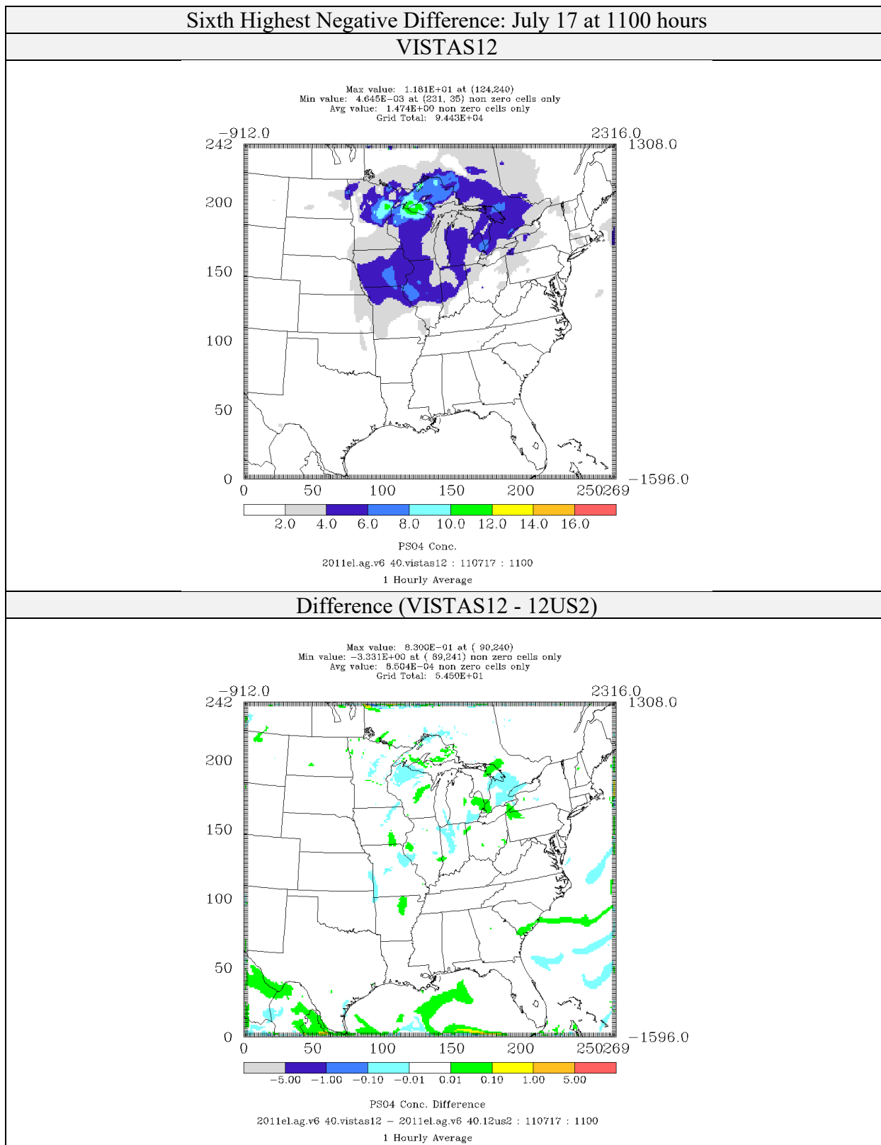
Figure 4-58: Comparison of Sulfate Concentrations ( \mu\text{g}/\text{m}^3 ) for CAMx 6.40 on VISTAS12 and 12US2 domains 2011el Simulations (Sixth Highest Negative Difference)
