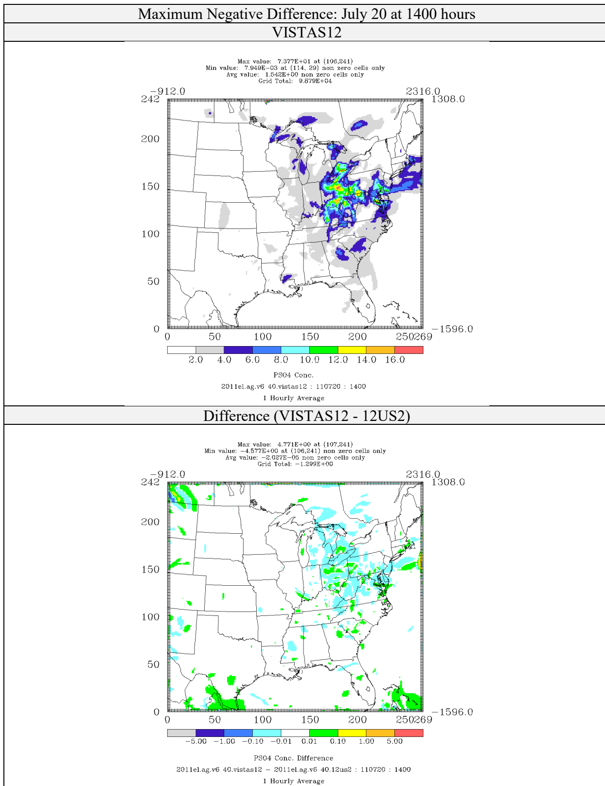
Figure 4-53: Comparison of Sulfate Concentrations ( \mu\text{g}/\text{m}^3 ) for CAMx 6.40 on VISTAS12 and 12US2 domains 2011el Simulations (Maximum Negative Difference)
