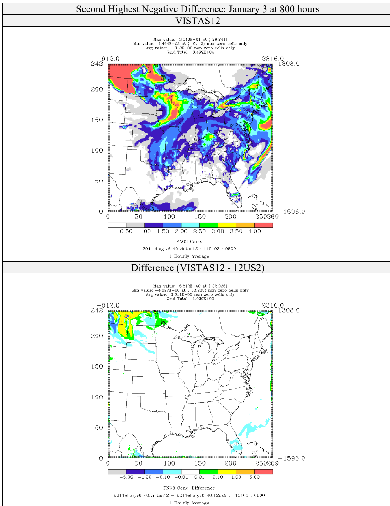
Figure 4-75: Comparison of Nitrate Concentrations ( \mu\text{g}/\text{m}^3 ) for CAMx 6.40 on VISTAS12 and 12US2 domains 2011el Simulations (Second Highest Negative Difference)
