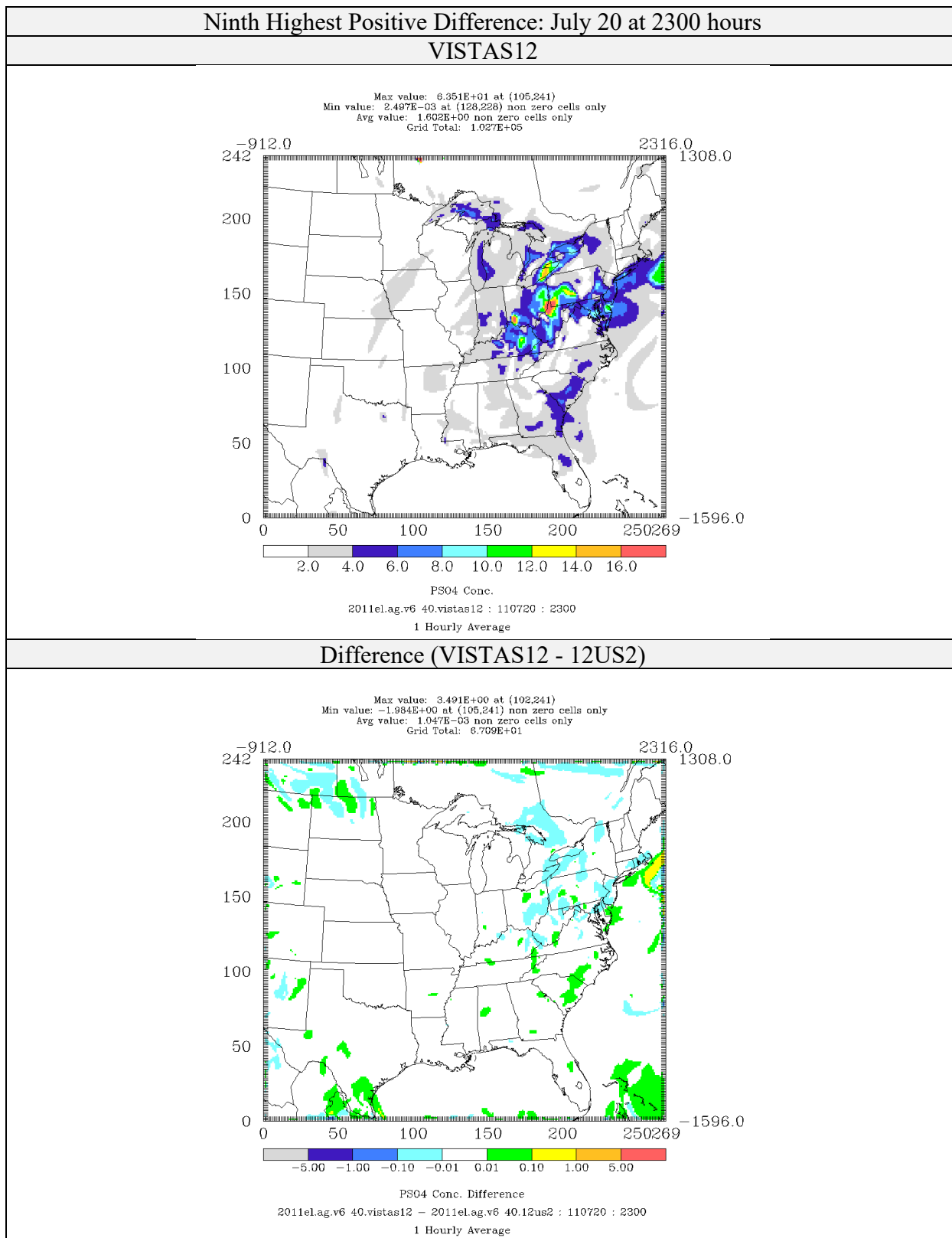
Figure 4-51: Comparison of Sulfate Concentrations ( \mu\text{g}/\text{m}^3 ) for CAMx 6.40 on VISTAS12 and 12US2 domains 2011el Simulations (Ninth Highest Positive Difference)
