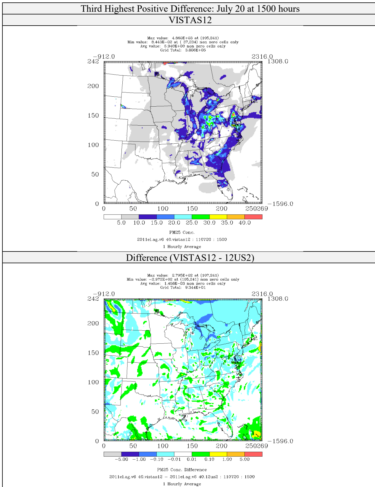
Figure 4-24: Comparison of PM 2.5 Concentrations ( \mu\text{g}/\text{m}^3 ) for CAMx 6.40 on VISTAS12 and 12US2 domains 2011el Simulations (Third Highest Positive Difference)
