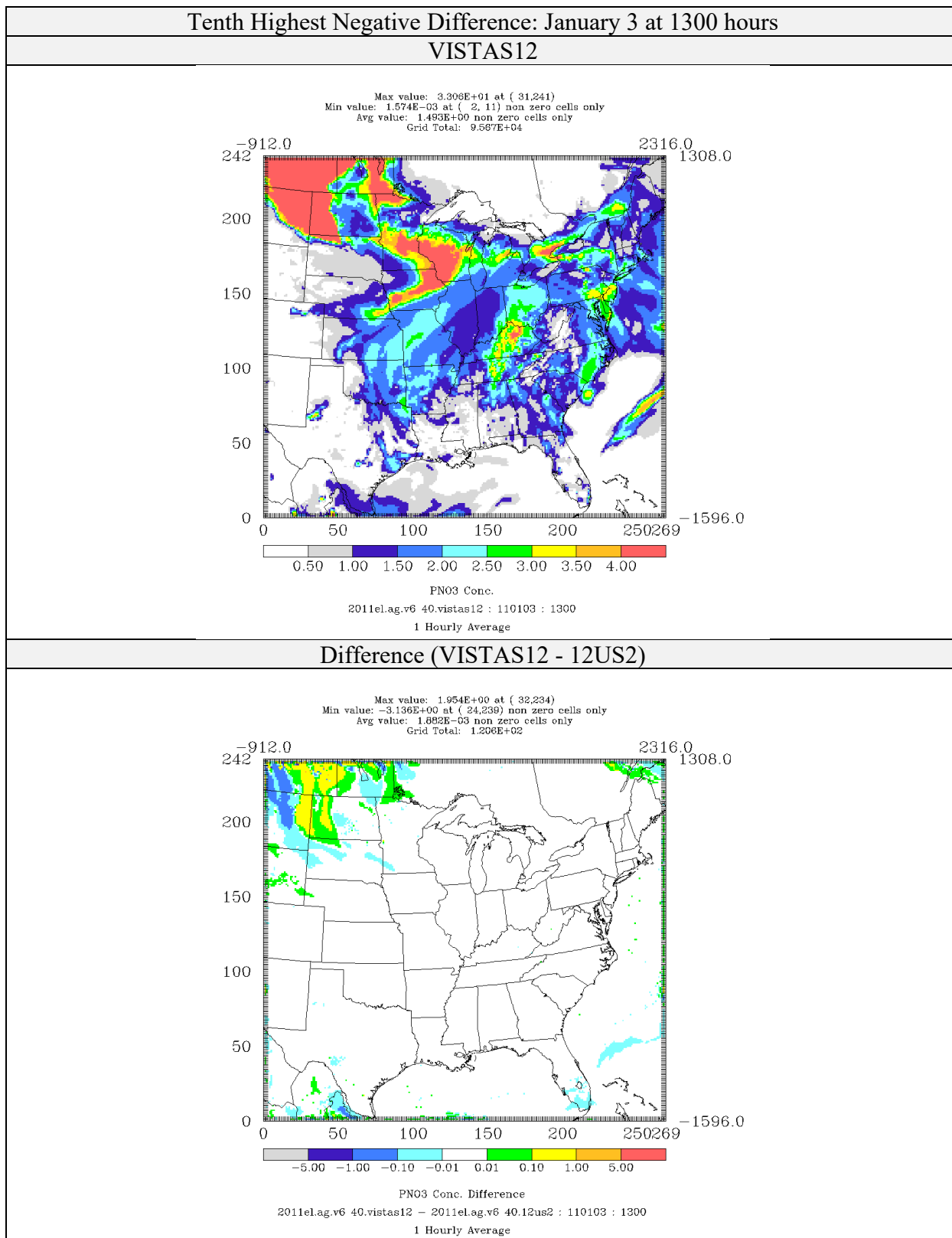
Figure 4-83: Comparison of Nitrate Concentrations ( \mu\text{g}/\text{m}^3 ) for CAMx 6.40 on VISTAS12 and 12US2 domains 2011el Simulations (Tenth Highest Negative Difference)
