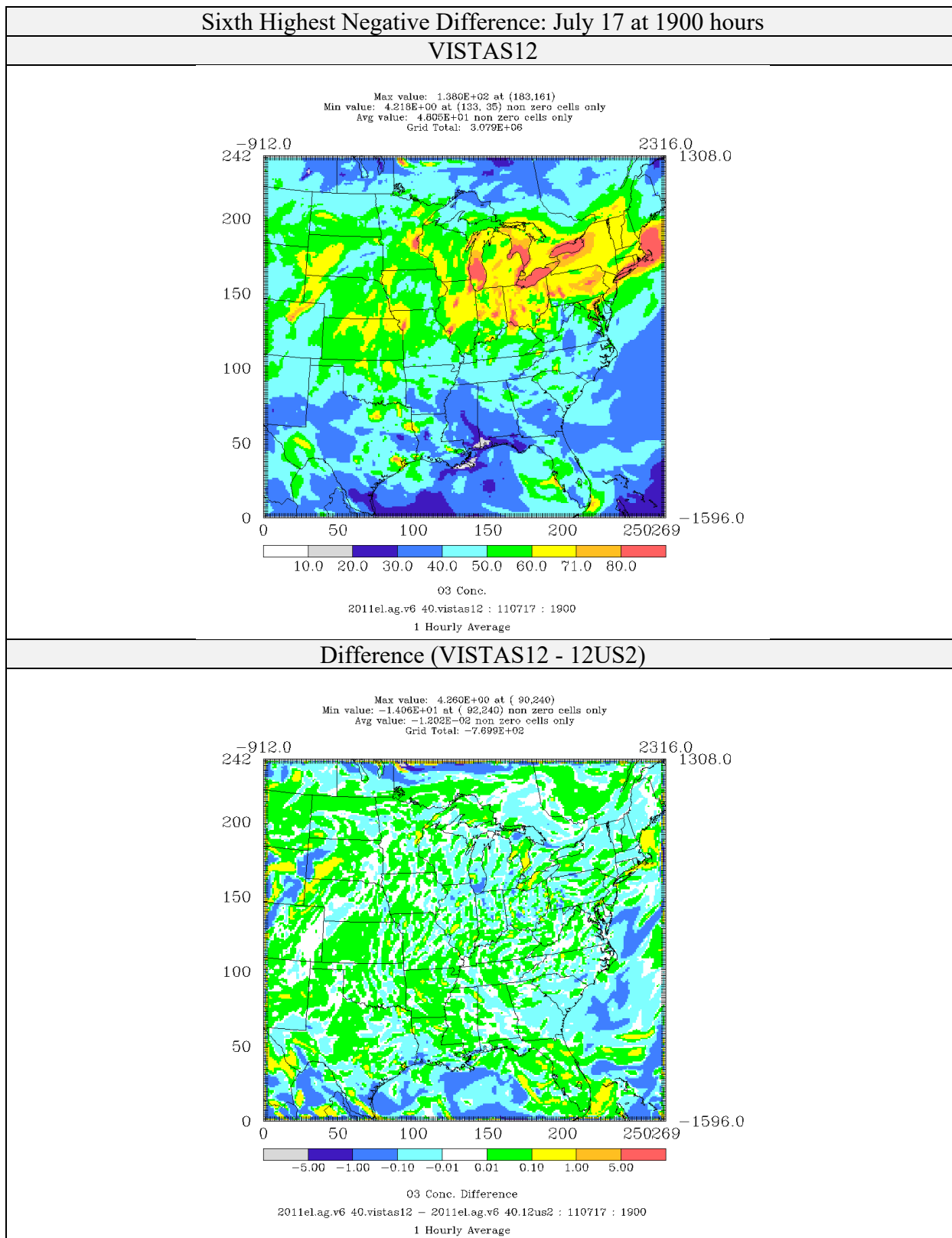
Figure 4-16: Comparison of Ozone Concentrations (ppb) for CAMx 6.40 on VISTAS12 and 12US2 domains 2011el Simulations (Sixth Highest Negative Difference)
