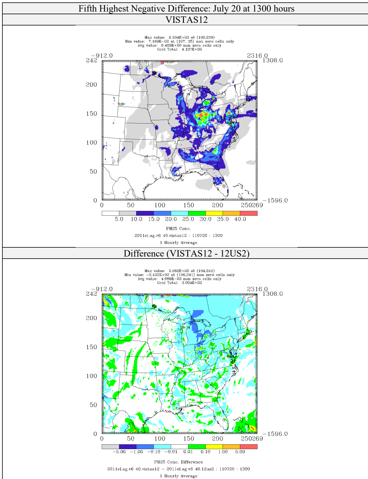
Figure 4-36: Comparison of PM 2.5 Concentrations ( \mu\text{g}/\text{m}^3 ) for CAMx 6.40 on VISTAS12 and 12US2 domains 2011el Simulations (Fifth Highest Negative Difference)
