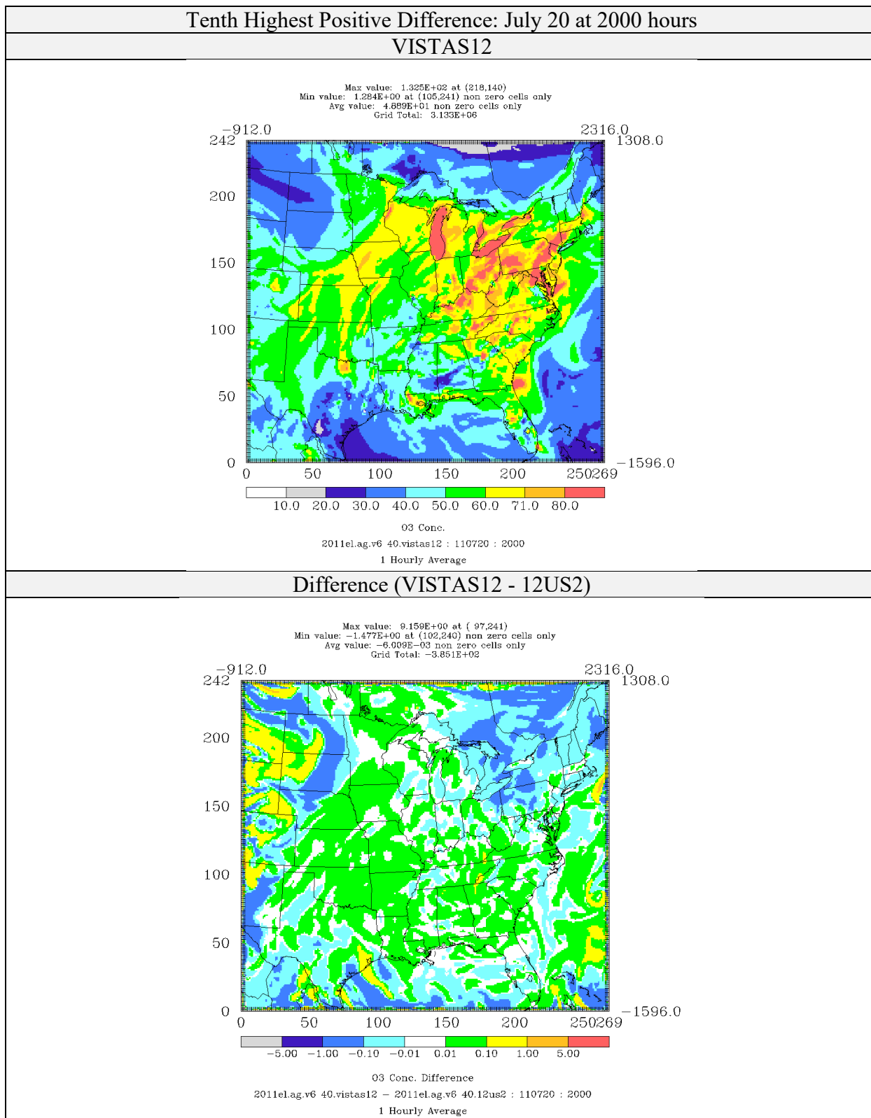
Figure 4-10: Comparison of Ozone Concentrations (ppb) for CAMx 6.40 on VISTAS12 and 12US2 domains 2011el Simulations (Tenth Highest Positive Difference)
