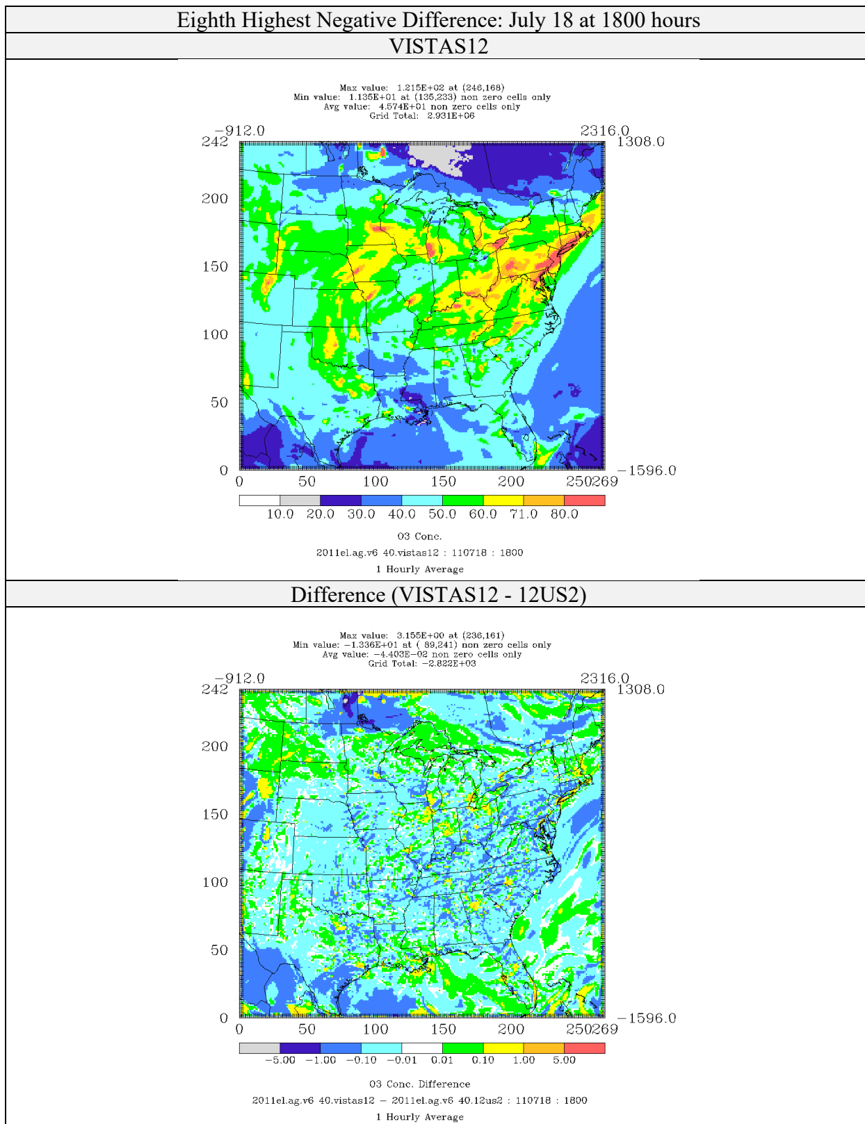
Figure 4-18: Comparison of Ozone Concentrations (ppb) for CAMx 6.40 on VISTAS12 and 12US2 domains 2011el Simulations (Eighth Highest Negative Difference)
