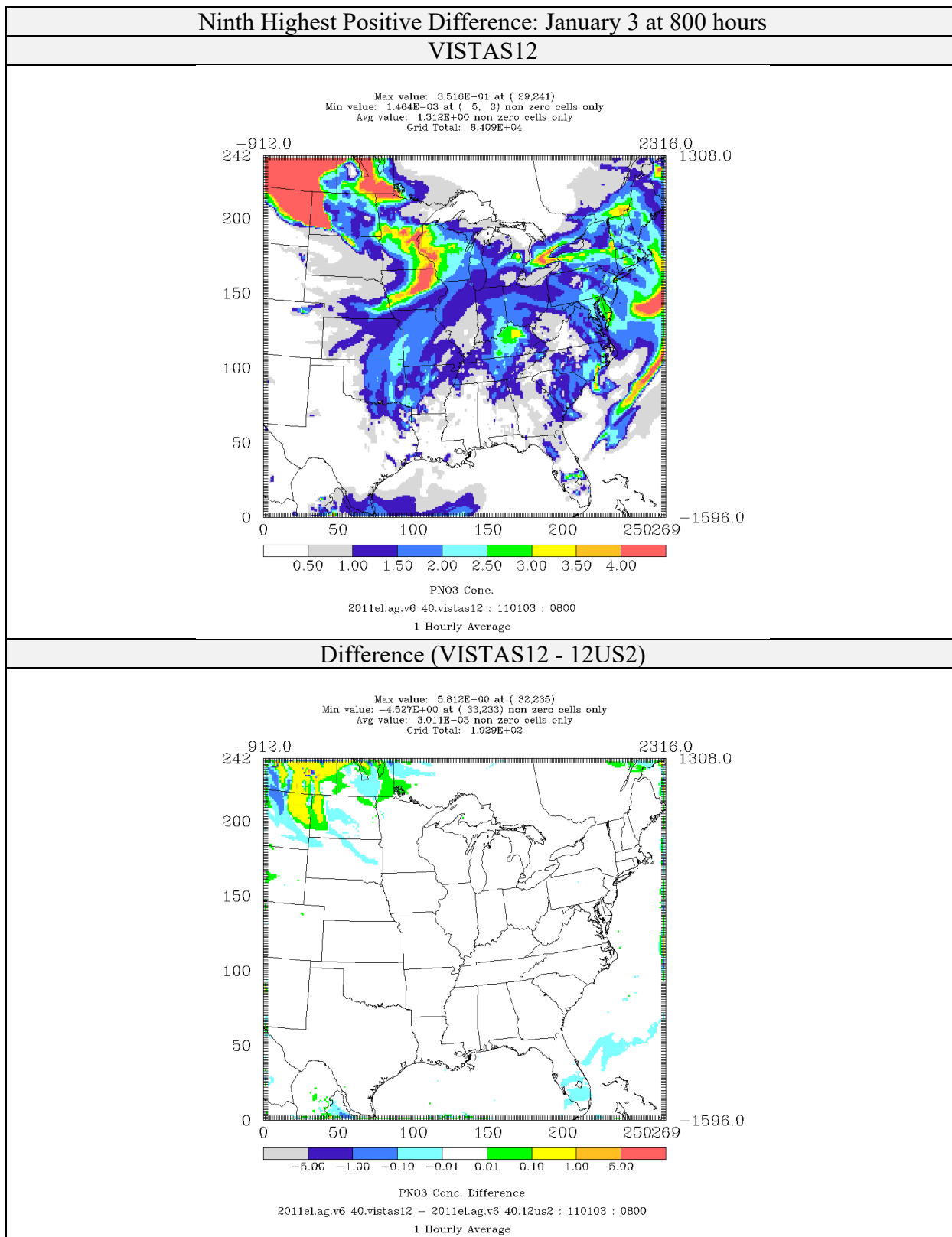
Figure 4-72: Comparison of Nitrate Concentrations ( \mu\text{g}/\text{m}^3 ) for CAMx 6.40 on VISTAS12 and 12US2 domains 2011el Simulations (Ninth Highest Positive Difference)
