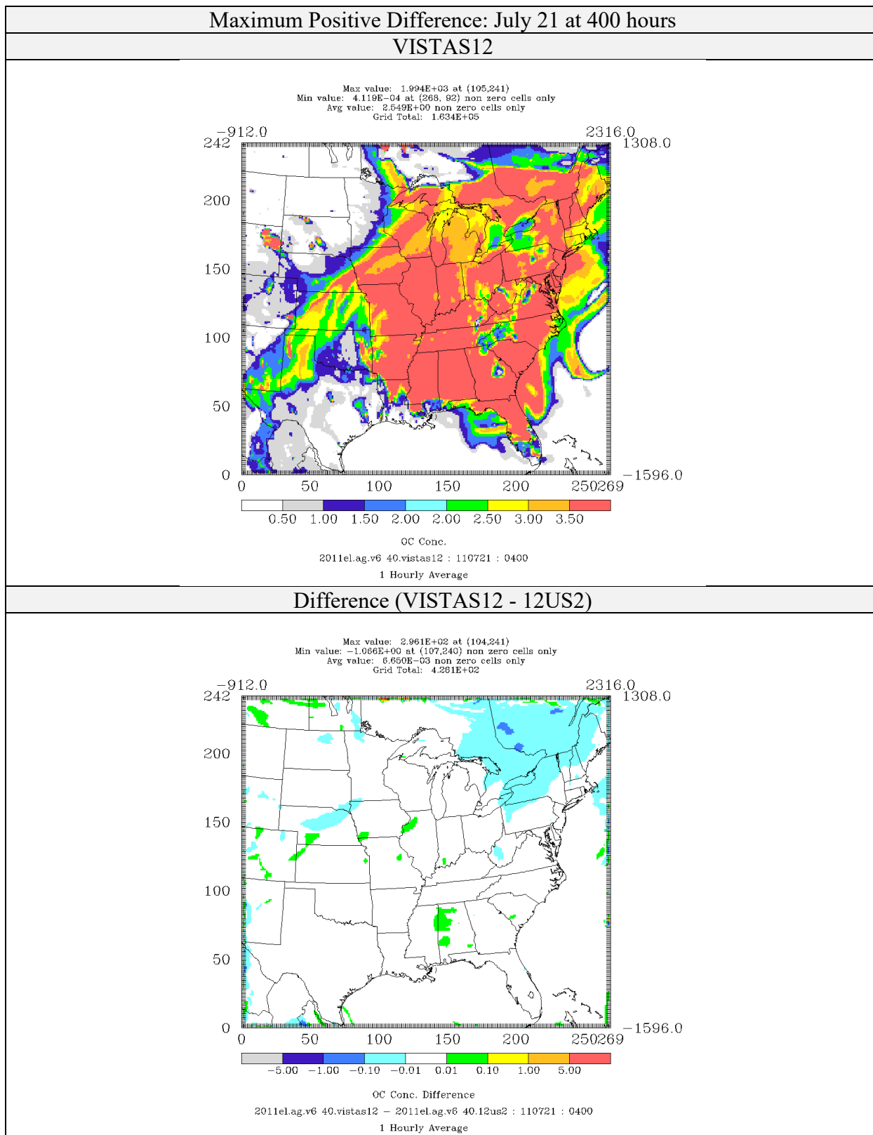
Figure 4-85: Comparison of Organic Matter Concentrations ( \mu\text{g}/\text{m}^3 ) for CAMx 6.40 on VISTAS12 and 12US2 domains 2011el Simulations (Maximum Positive Difference)
