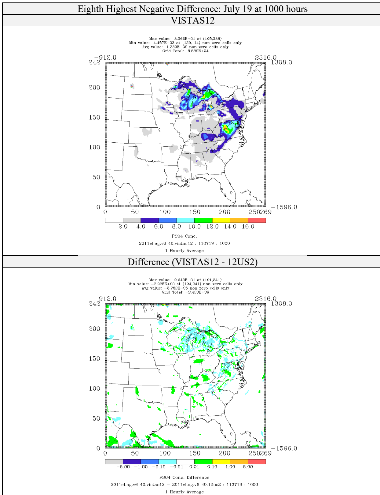
Figure 4-60: Comparison of Sulfate Concentrations ( \mu\text{g}/\text{m}^3 ) for CAMx 6.40 on VISTAS12 and 12US2 domains 2011el Simulations (Eighth Highest Negative Difference)
