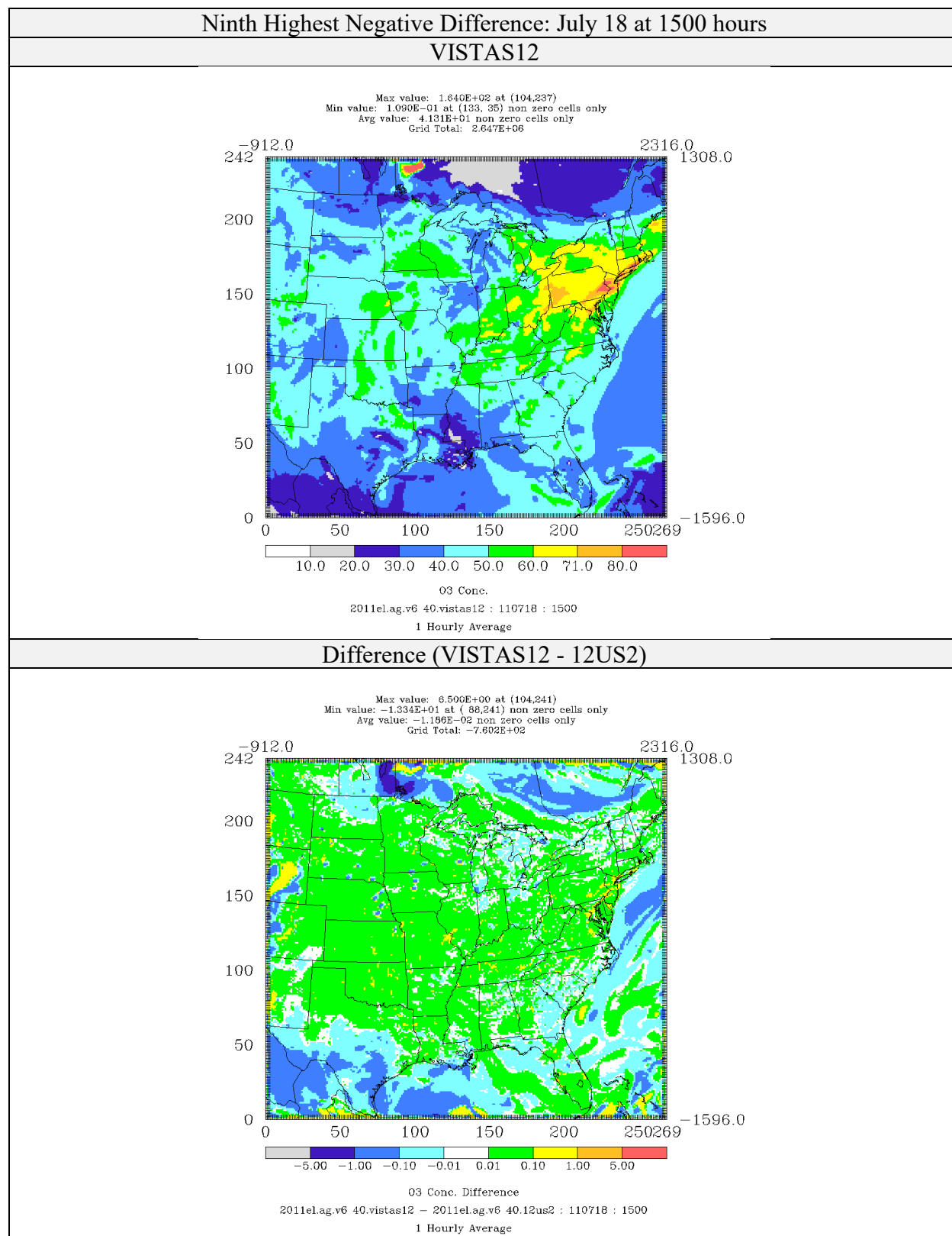
Figure 4-19: Comparison of Ozone Concentrations (ppb) for CAMx 6.40 on VISTAS12 and 12US2 domains 2011el Simulations (Ninth Highest Negative Difference)
