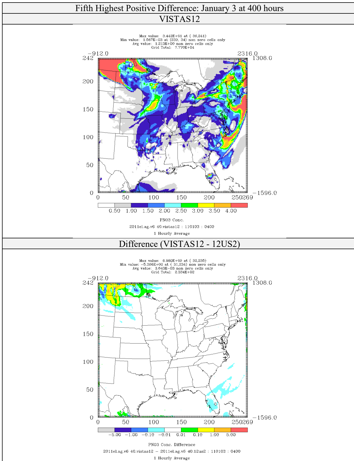
Figure 4-68: Comparison of Nitrate Concentrations ( \mu\text{g}/\text{m}^3 ) for CAMx 6.40 on VISTAS12 and 12US2 domains 2011el Simulations (Fifth Highest Positive Difference)
