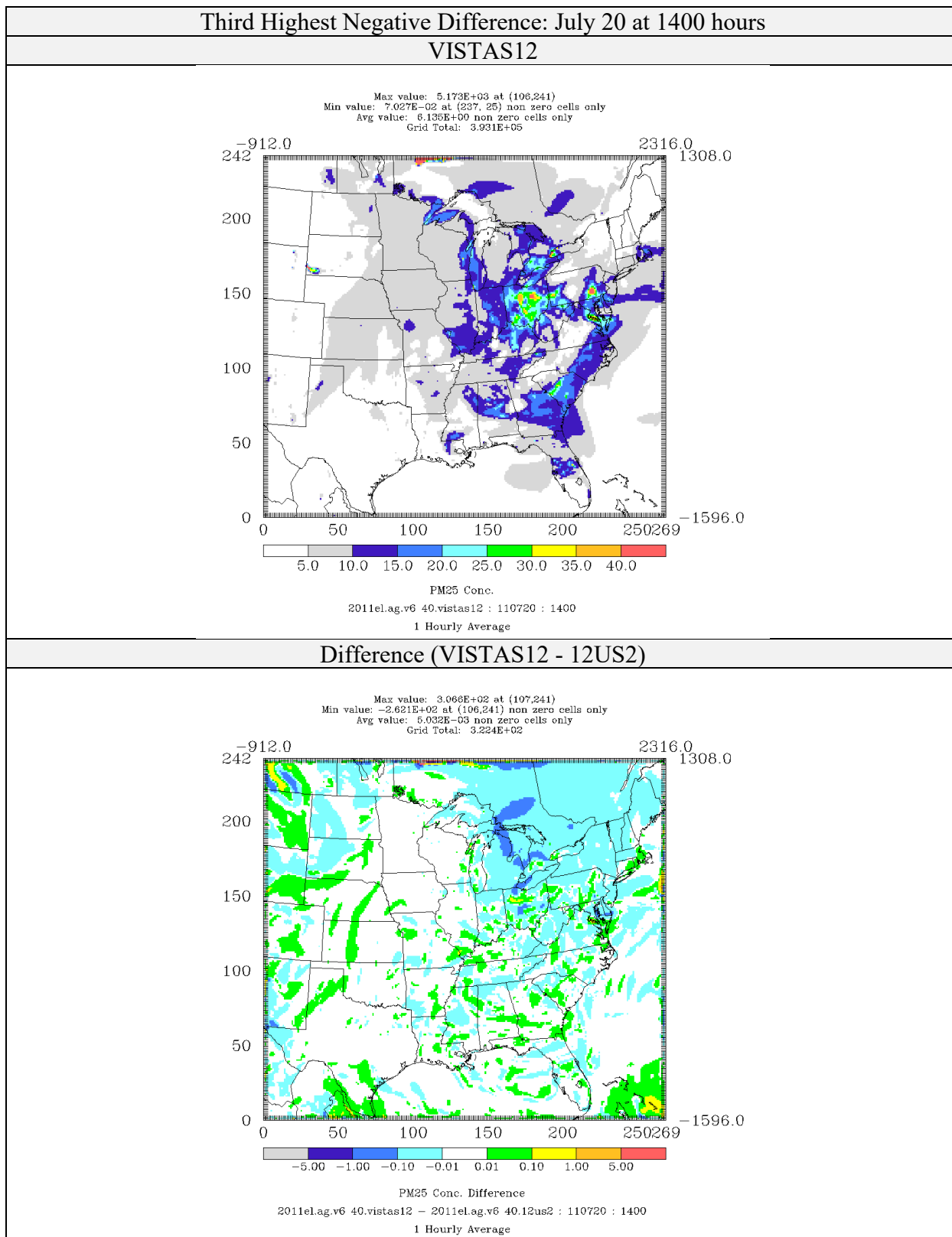
Figure 4-34: Comparison of PM 2.5 Concentrations ( \mu\text{g}/\text{m}^3 ) for CAMx 6.40 on VISTAS12 and 12US2 domains 2011el Simulations (Third Highest Negative Difference)
