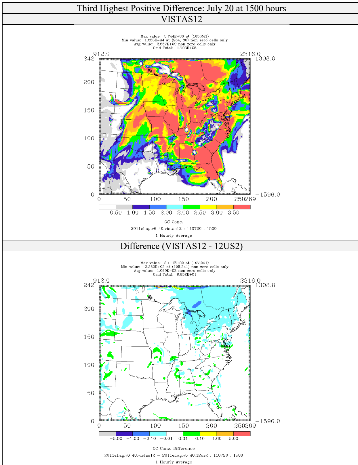
Figure 4-87: Comparison of Organic Matter Concentrations ( \mu\text{g}/\text{m}^3 ) for CAMx 6.40 on VISTAS12 and 12US2 domains 2011el Simulations (Third Highest Positive Difference)
