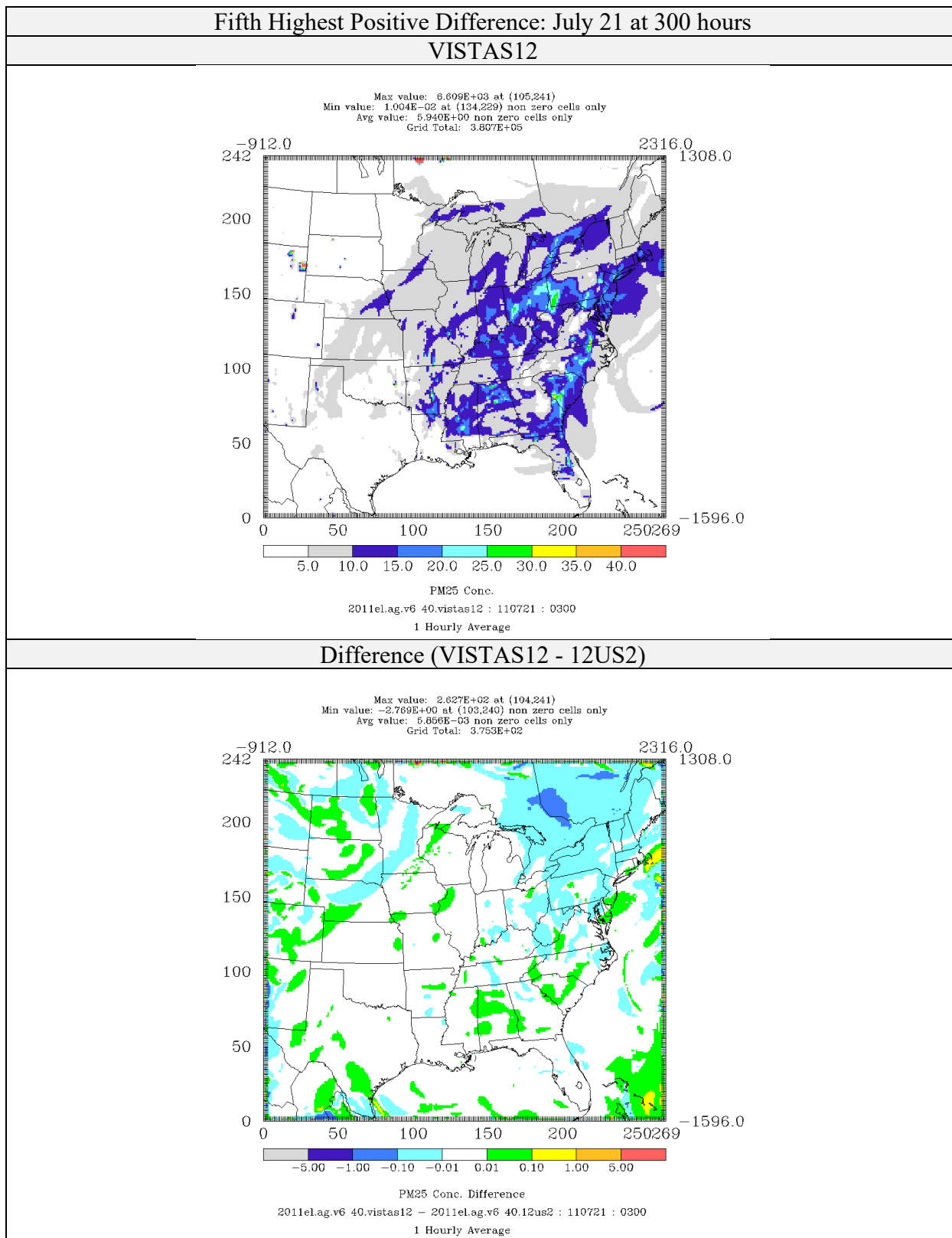
Figure 4-26: Comparison of PM 2.5 Concentrations ( \mu\text{g}/\text{m}^3 ) for CAMx 6.40 on VISTAS12 and 12US2 domains 2011el Simulations (Fifth Highest Positive Difference)
