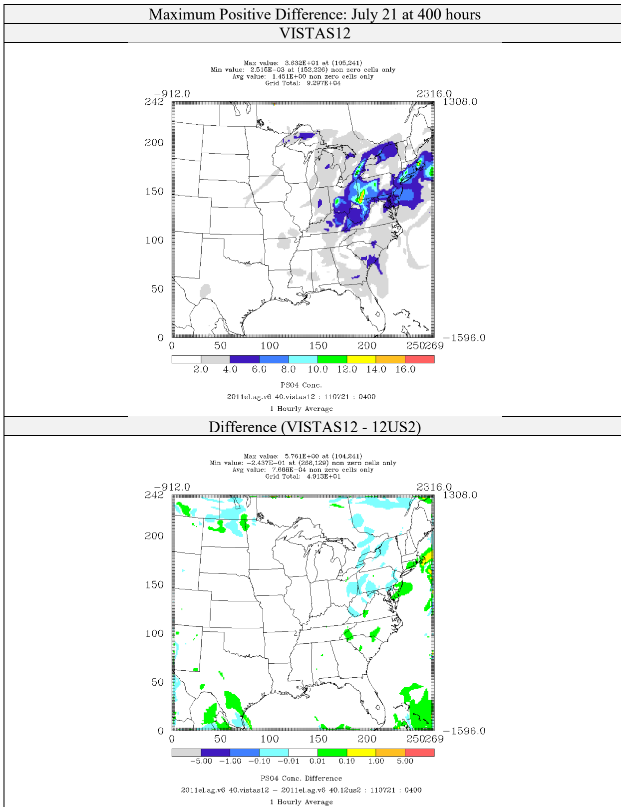
Figure 4-43: Comparison of Sulfate Concentrations ( \mu\text{g}/\text{m}^3 ) for CAMx 6.40 on VISTAS12 and 12US2 domains 2011el Simulations (Maximum Positive Difference)
