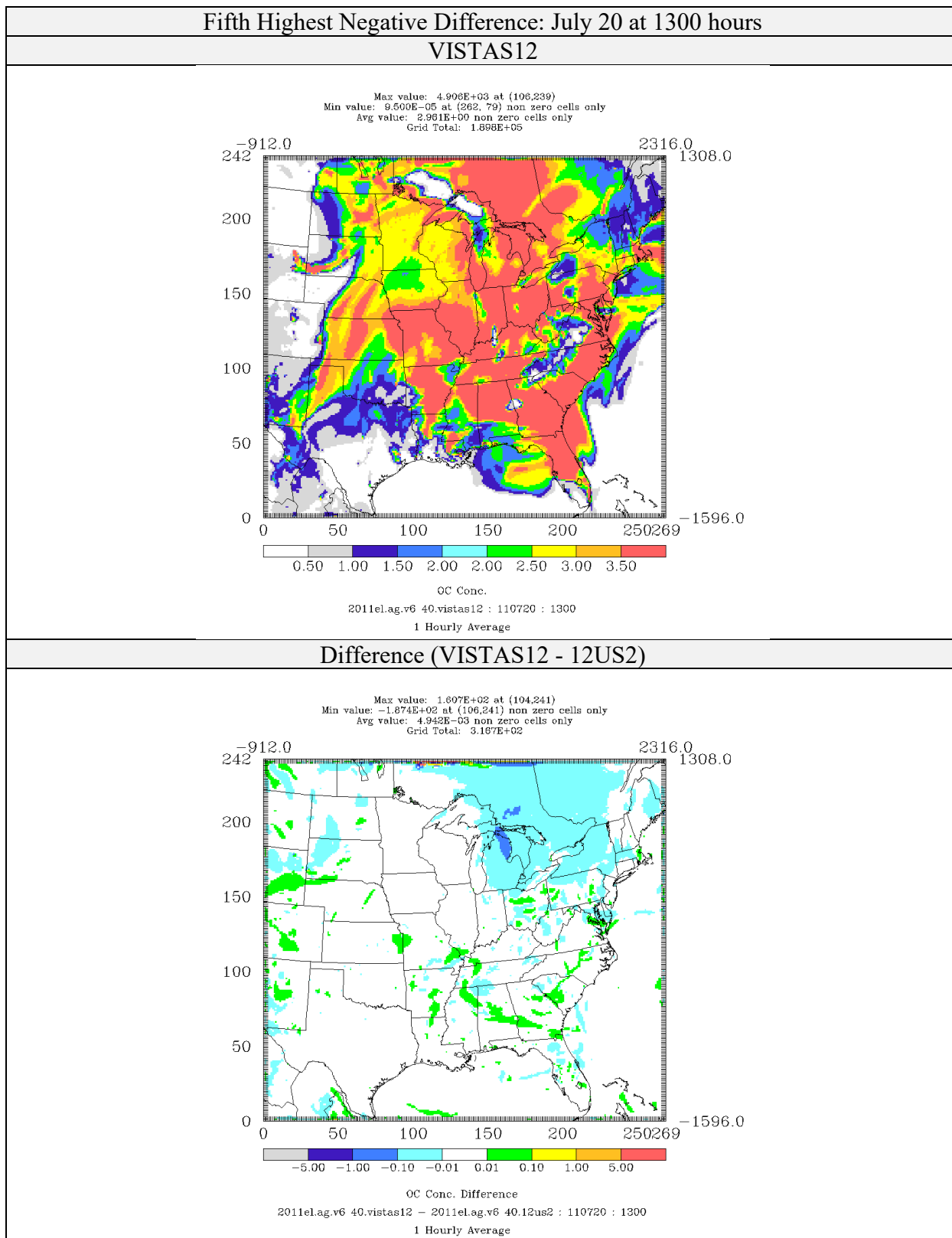
Figure 4-99: Comparison of Organic Matter Concentrations ( \mu\text{g}/\text{m}^3 ) for CAMx 6.40 on VISTAS12 and 12US2 domains 2011el Simulations (Fifth Highest Negative Difference)
