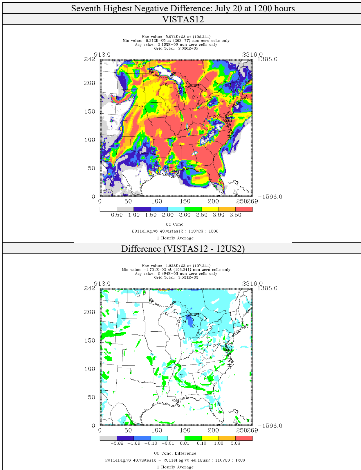
Figure 4-101: Comparison of Organic Matter Concentrations ( \mu\text{g}/\text{m}^3 ) for CAMx 6.40 on VISTAS12 and 12US2 domains 2011el Simulations (Seventh Highest Negative Difference)
