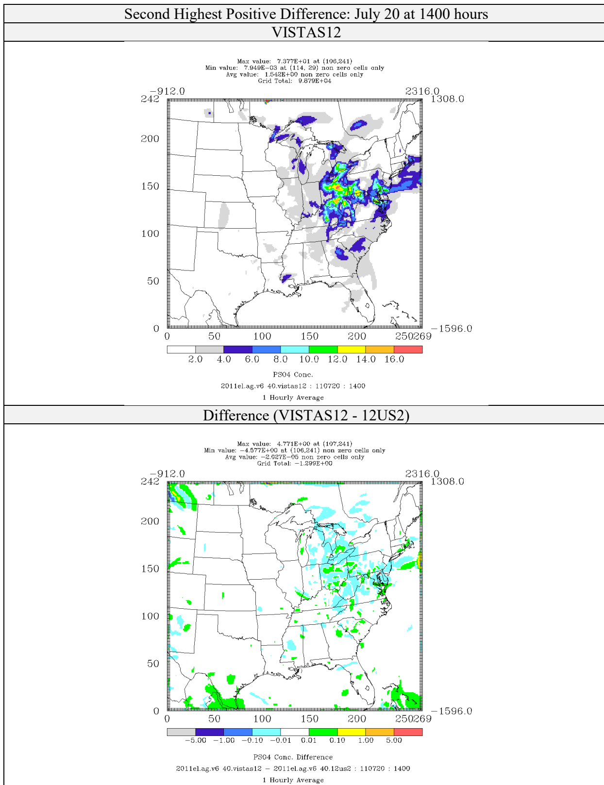
Figure 4-44: Comparison of Sulfate Concentrations ( \mu\text{g}/\text{m}^3 ) for CAMx 6.40 on VISTAS12 and 12US2 domains 2011el Simulations (Second Highest Positive Difference)
