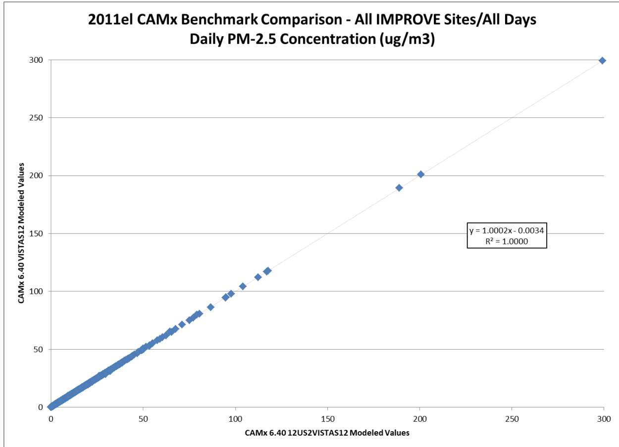
Figure 4-42: Scatterplot Comparing 24-hour Average Predicted PM 2.5 Concentrations (µg/m 3 ) for All Days at all IMPROVE Monitor Locations for CAMx 6.40 on VISTAS12 and 12US2 domains 2011el Simulations Performed by VISTAS (Alpine).
