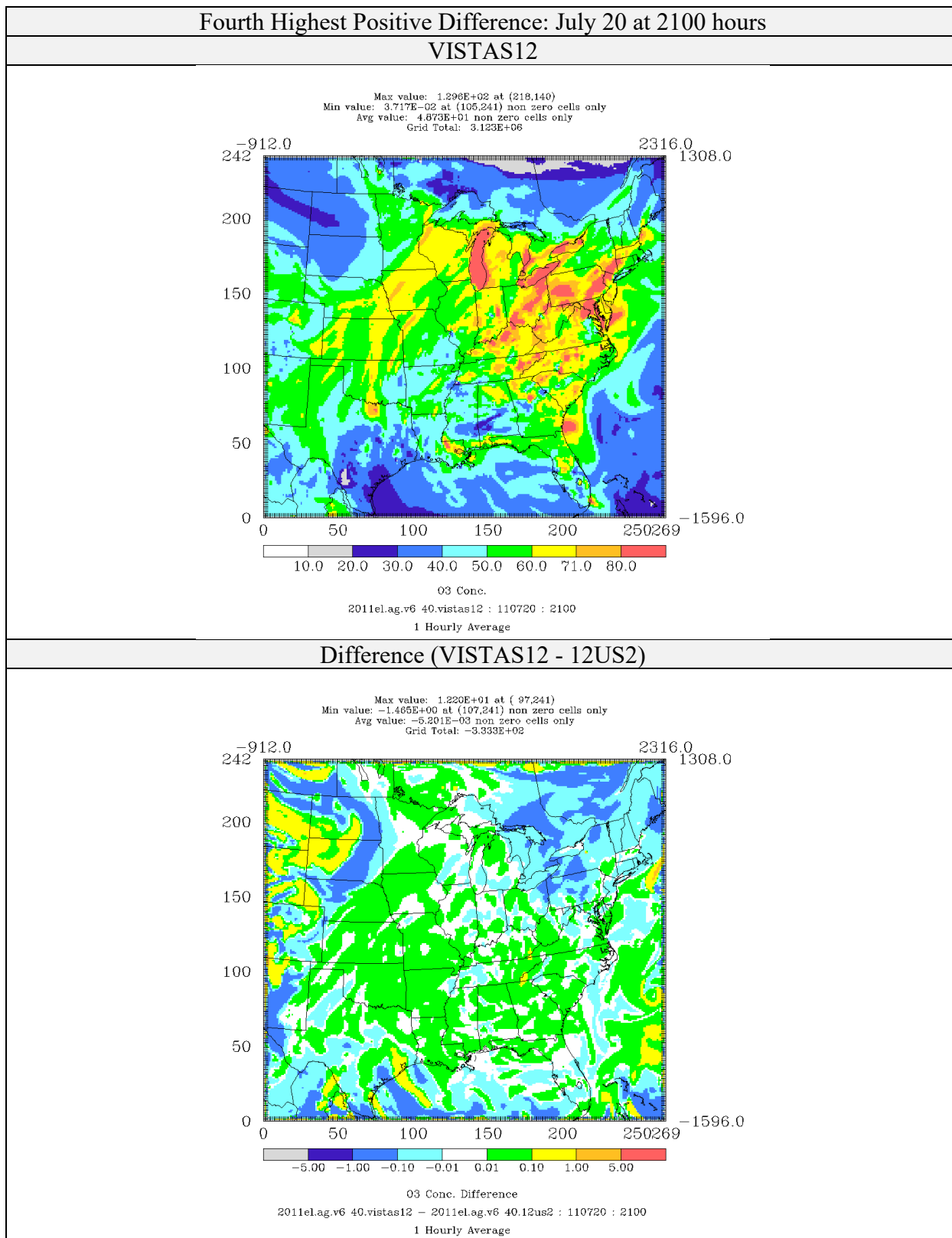
Figure 4-4: Comparison of Ozone Concentrations (ppb) for CAMx 6.40 on VISTAS12 and 12US2 domains 2011el Simulations (Fourth Highest Positive Difference)
