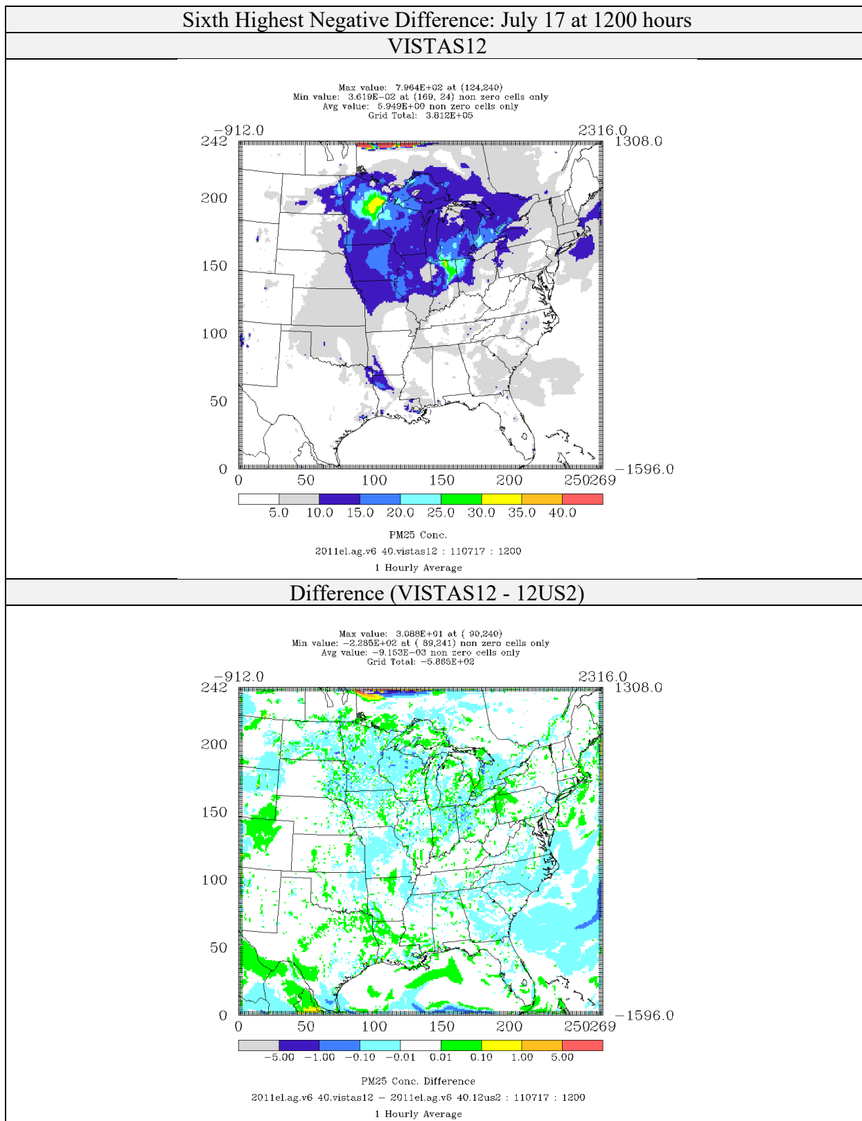
Figure 4-37: Comparison of PM 2.5 Concentrations ( \mu\text{g}/\text{m}^3 ) for CAMx 6.40 on VISTAS12 and 12US2 domains 2011el Simulations (Sixth Highest Negative Difference)
