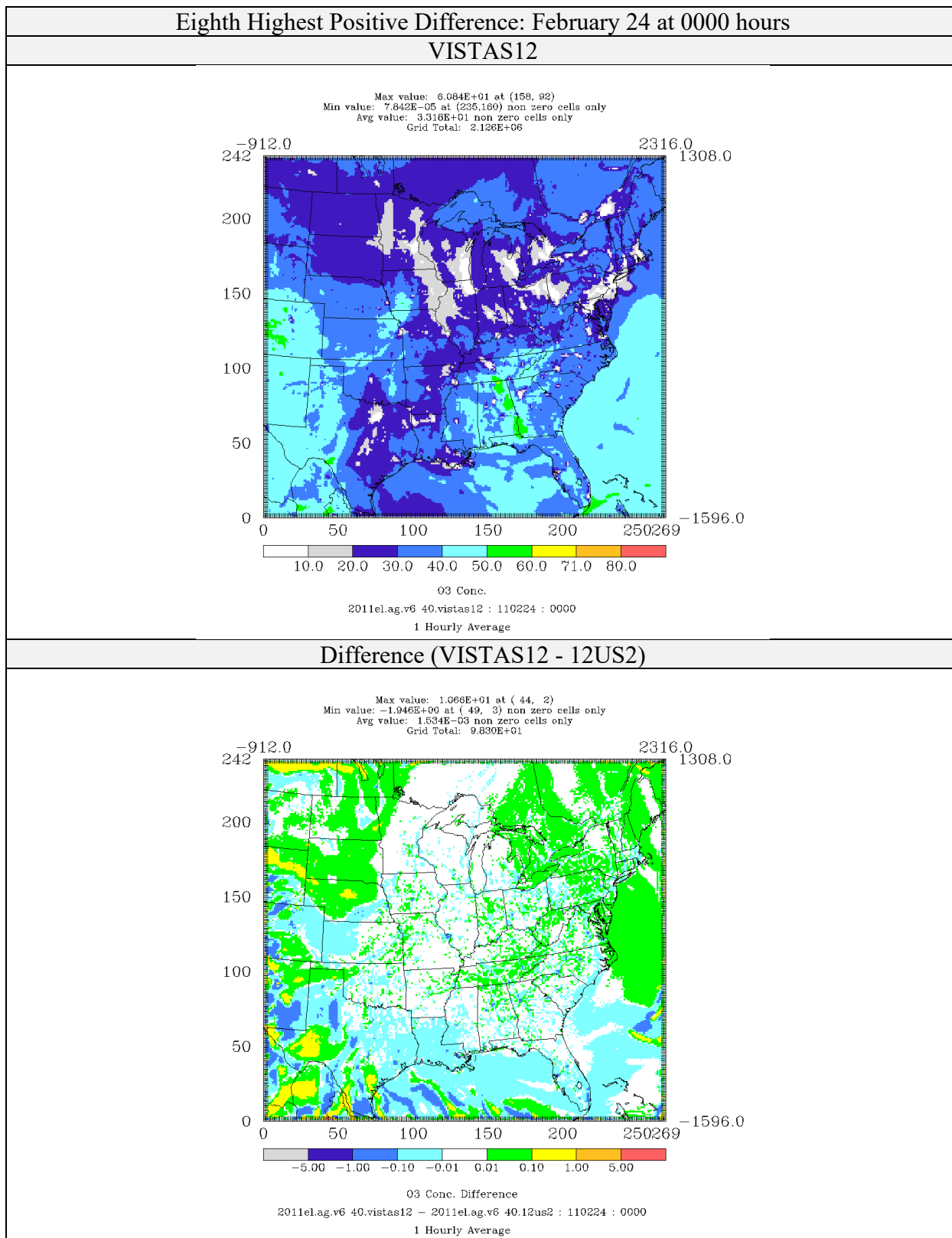
Figure 4-8: Comparison of Ozone Concentrations (ppb) for CAMx 6.40 on VISTAS12 and 12US2 domains 2011el Simulations (Eighth Highest Positive Difference)
