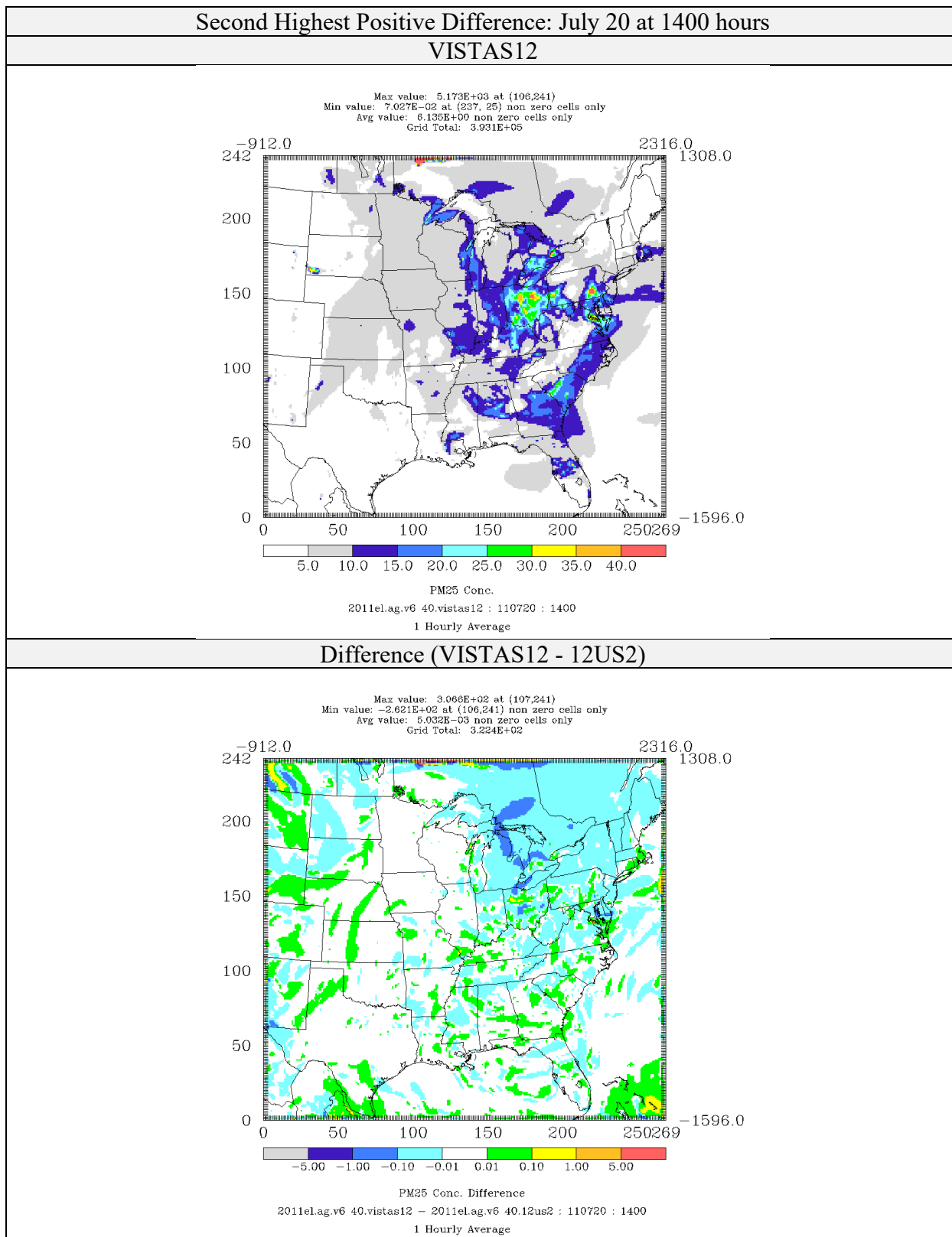
Figure 4-23: Comparison of PM 2.5 Concentrations ( \mu\text{g}/\text{m}^3 ) for CAMx 6.40 on VISTAS12 and 12US2 domains 2011el Simulations (Second Highest Positive Difference)
