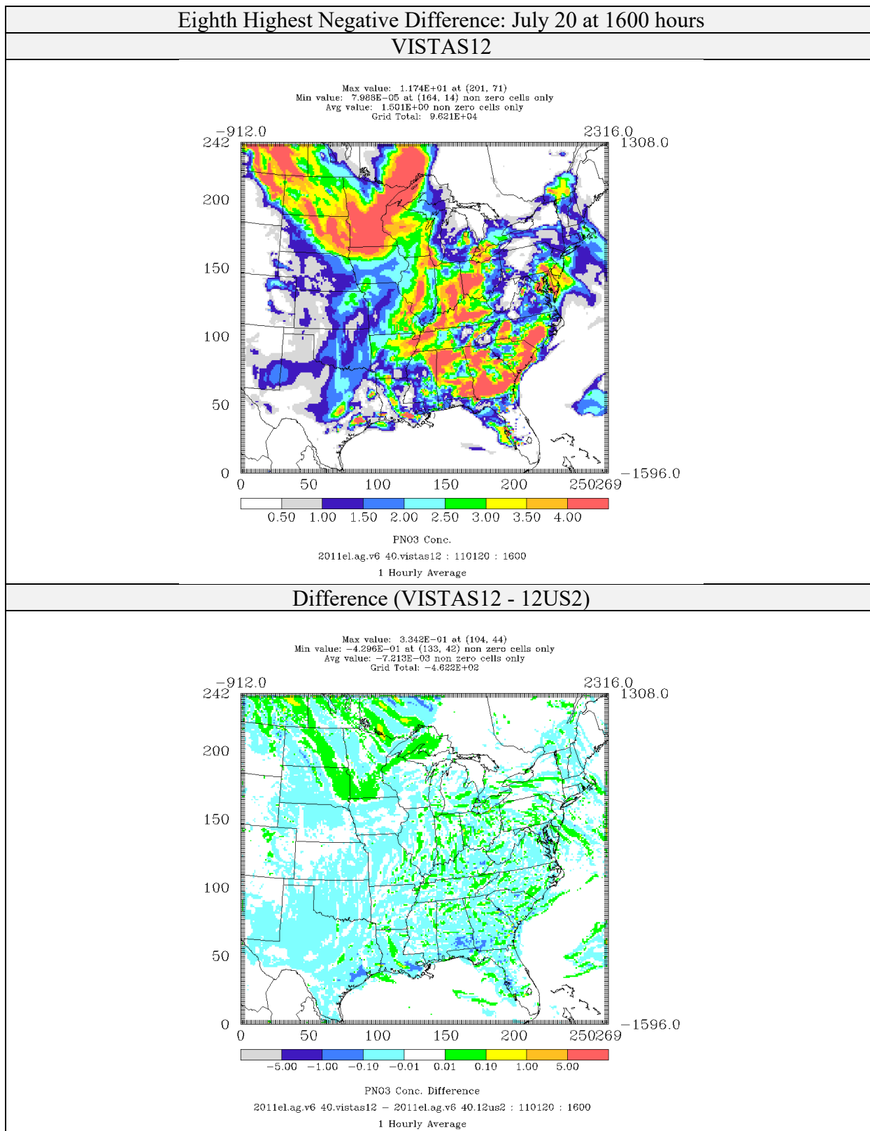
Figure 4-81: Comparison of Nitrate Concentrations ( \mu\text{g}/\text{m}^3 ) for CAMx 6.40 on VISTAS12 and 12US2 domains 2011el Simulations (Eighth Highest Negative Difference)
