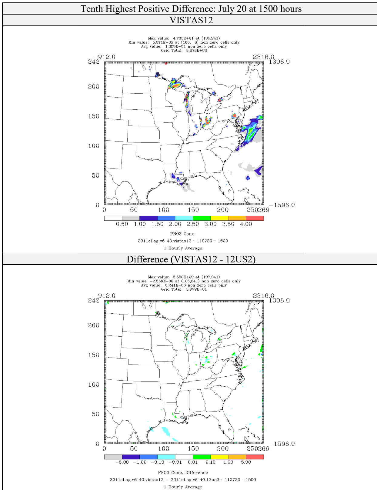
Figure 4-73: Comparison of Nitrate Concentrations ( \mu\text{g}/\text{m}^3 ) for CAMx 6.40 on VISTAS12 and 12US2 domains 2011el Simulations (Tenth Highest Positive Difference)
