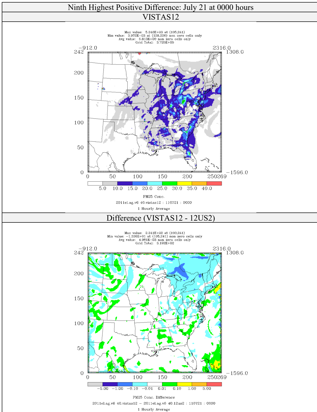
Figure 4-30: Comparison of PM 2.5 Concentrations ( \mu\text{g}/\text{m}^3 ) for CAMx 6.40 on VISTAS12 and 12US2 domains 2011el Simulations (Ninth Highest Positive Difference)
