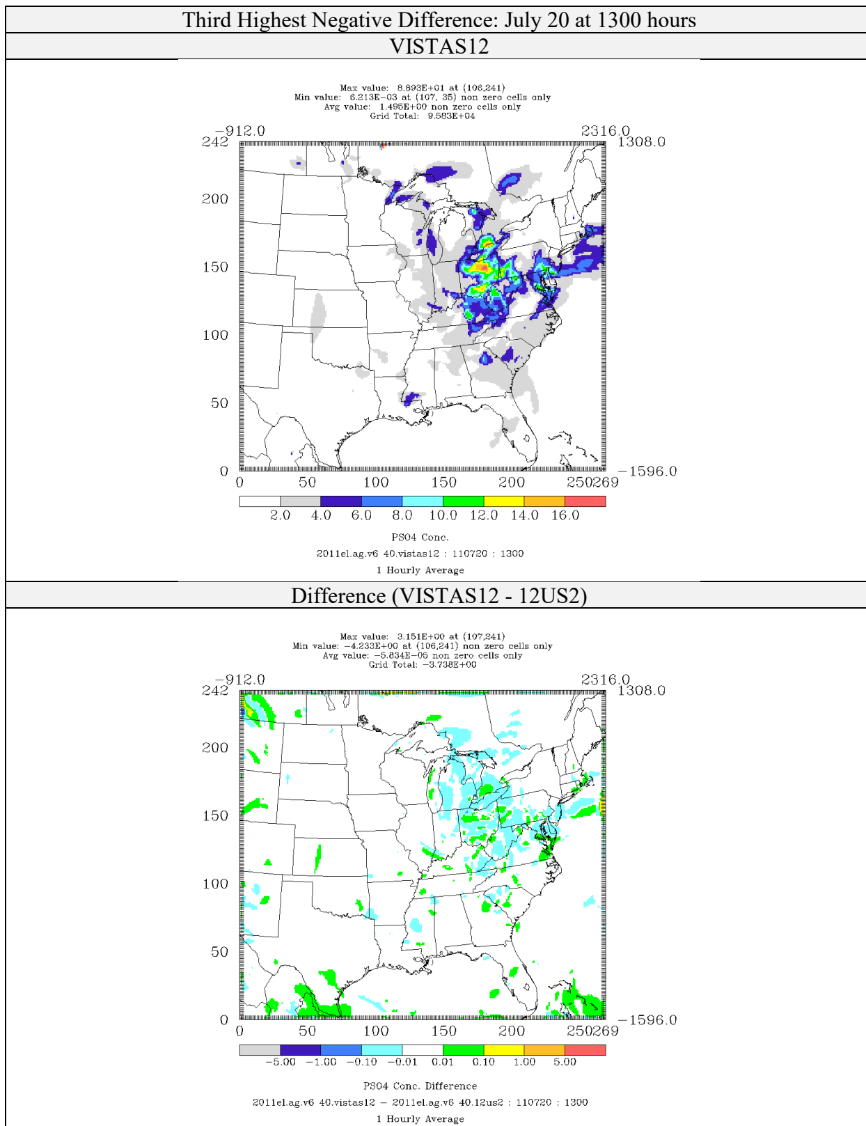
Figure 4-55: Comparison of Sulfate Concentrations ( \mu\text{g}/\text{m}^3 ) for CAMx 6.40 on VISTAS12 and 12US2 domains 2011el Simulations (Third Highest Negative Difference)
