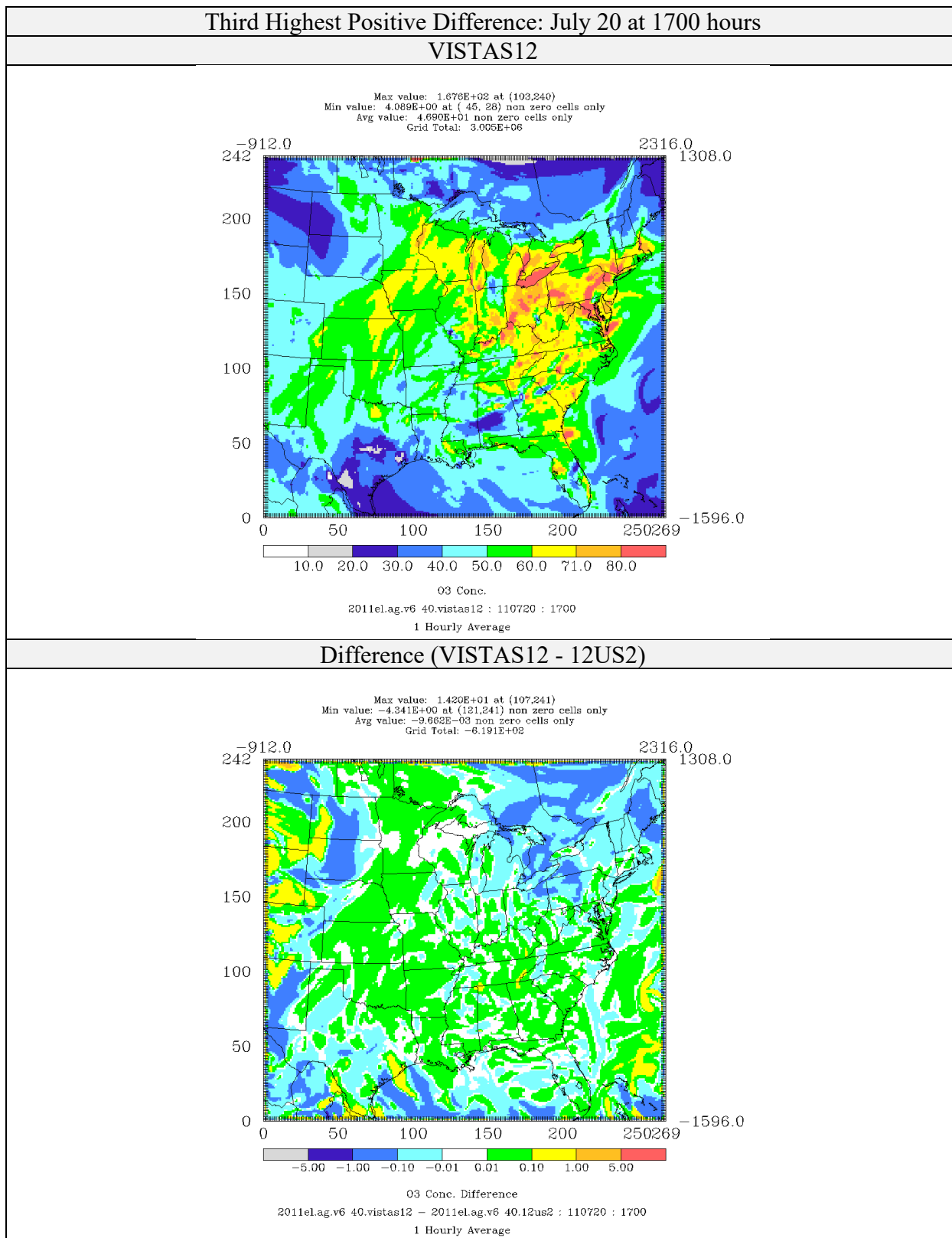
Figure 4-3: Comparison of Ozone Concentrations (ppb) for CAMx 6.40 on VISTAS12 and 12US2 domains 2011el Simulations (Third Highest Positive Difference)
