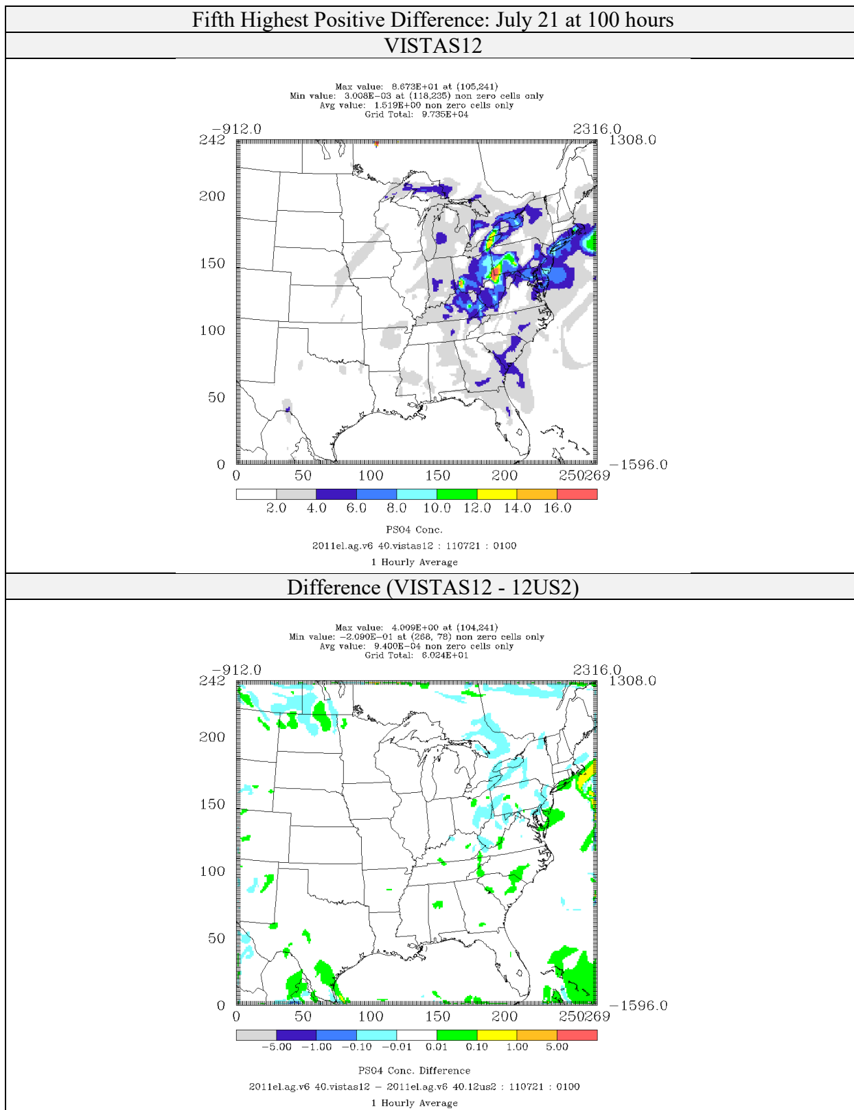
Figure 4-47: Comparison of Sulfate Concentrations ( \mu\text{g}/\text{m}^3 ) for CAMx 6.40 on VISTAS12 and 12US2 domains 2011el Simulations (Fifth Highest Positive Difference)
