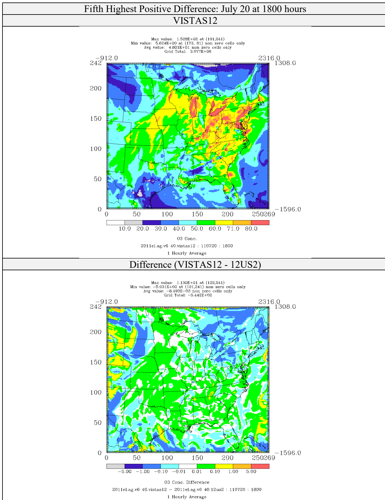
Figure 4-5: Comparison of Ozone Concentrations (ppb) for CAMx 6.40 on VISTAS12 and 12US2 domains 2011el Simulations (Fifth Highest Positive Difference)
