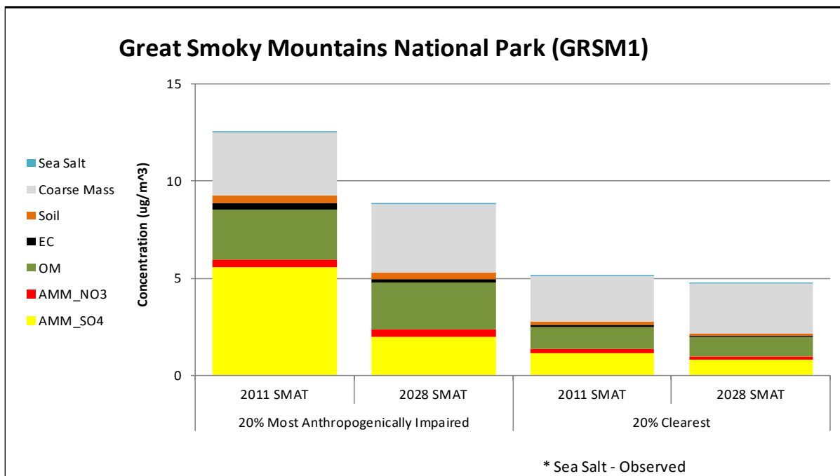
Figure 10-6. SMAT Concentrations (ug/m³) Great Smoky Mountains National Park on the Modeled 20% Clearest (Right) and 20% Most Anthropogenically Impaired (Left) Days.
