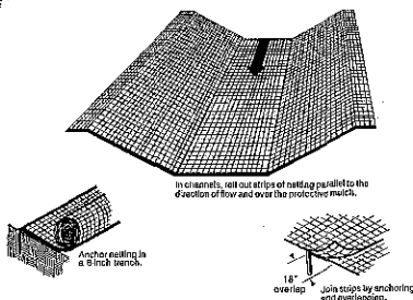
Installation of netting and mulch.
