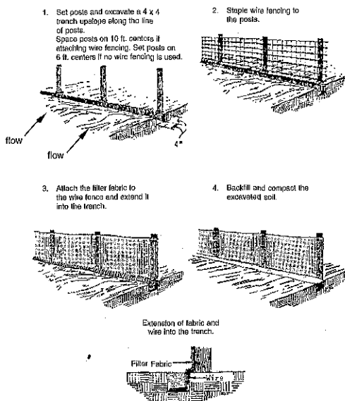
CONSTRUCTION OF A SILT FENCE
