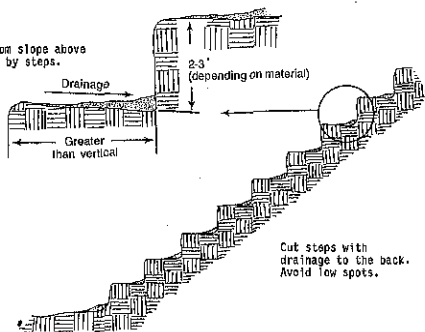
Stair stepping cut slopes
