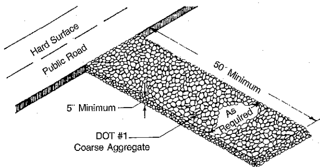
GRAVEL CONSTRUCTION ENTRANCE
