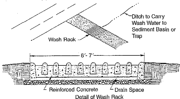
CONSTRUCTION ENTRANCE WITH WASH RACK
