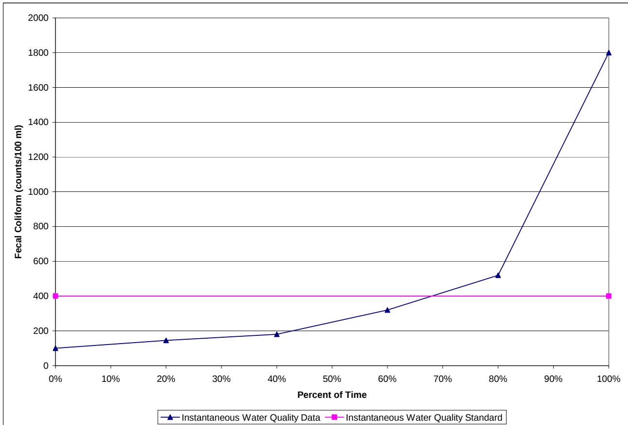
Figure 6. 10% Test Curve for Station PR-10, Summer 2001
