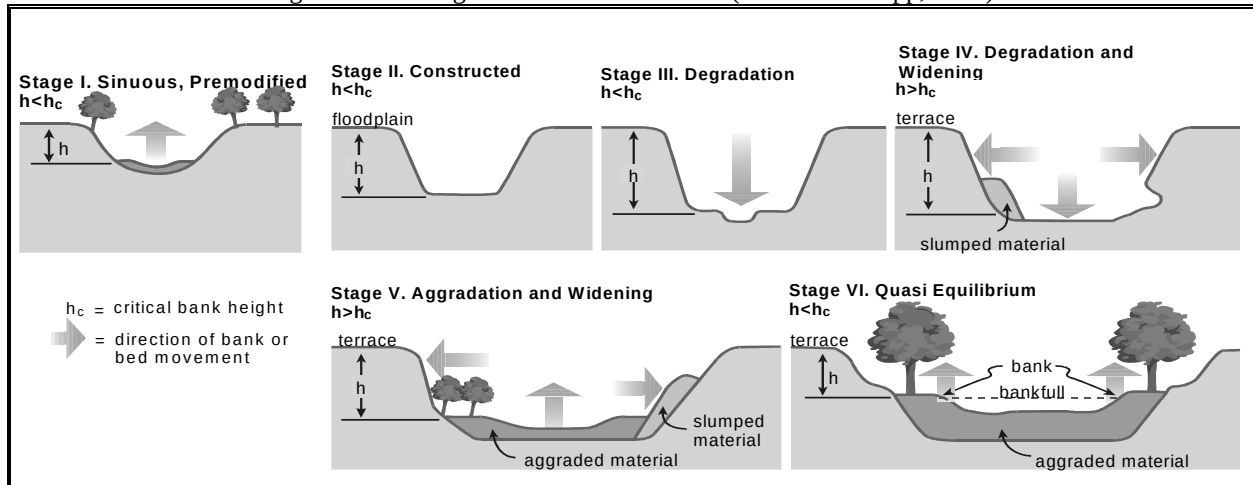
Figure 3. Six Stages of Channel Evolution (Simon and Hupp, 1986)
