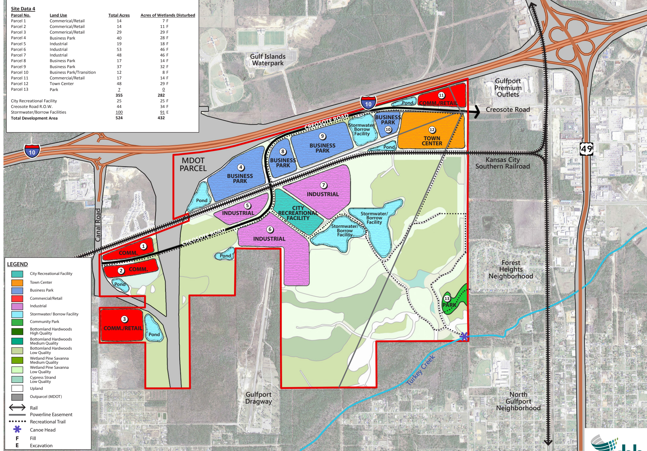
FIGURE A-15: PROPOSED PROJECT CONCEPT PLAN WARD-GULFPORT PROPERTY
