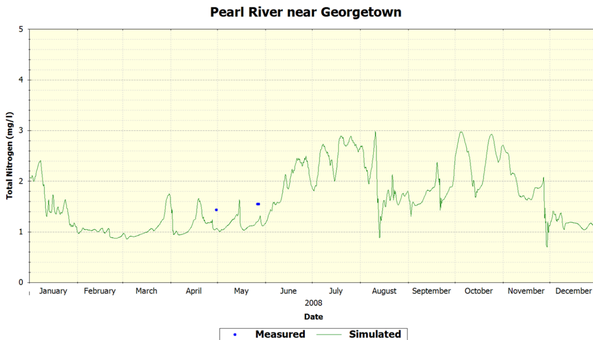
Figure 62 MDEQ Station Pearl River near Georgetown – Total Nitrogen
