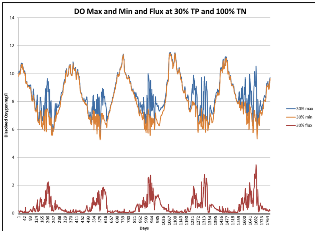
Figure 16 DO Flux at 30% TP Available
