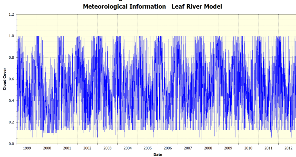
Figure 117 Cloud Cover
