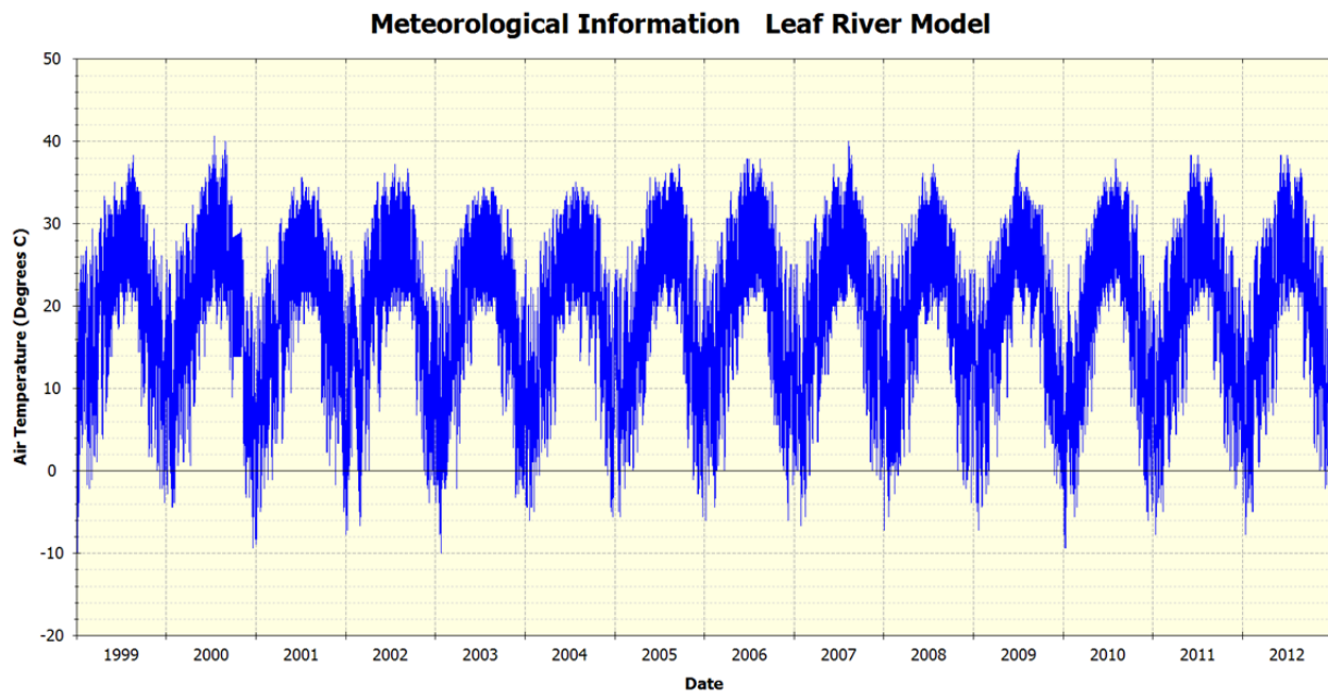
Figure 115 Air Temperature
