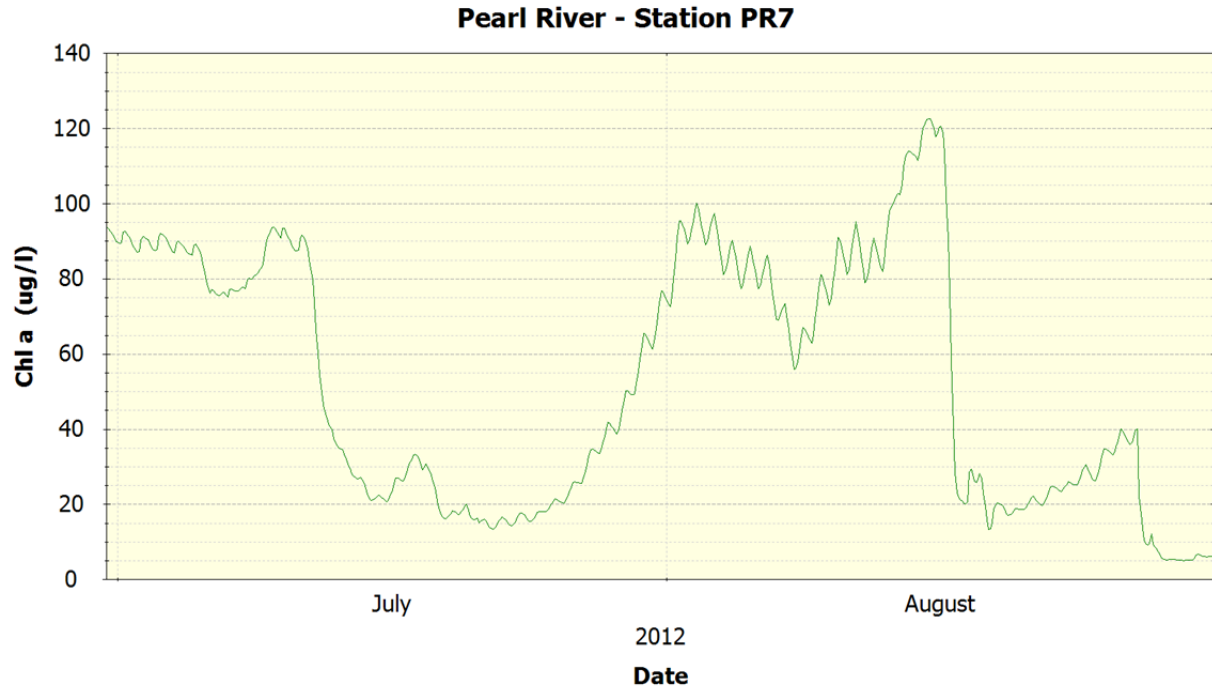
Figure 94 Pearl River Station PR7 – Chl a
