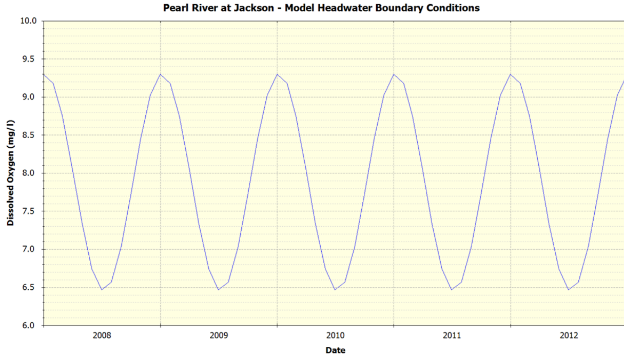
Figure 47 Model Headwater Conditions – Dissolved Oxygen
