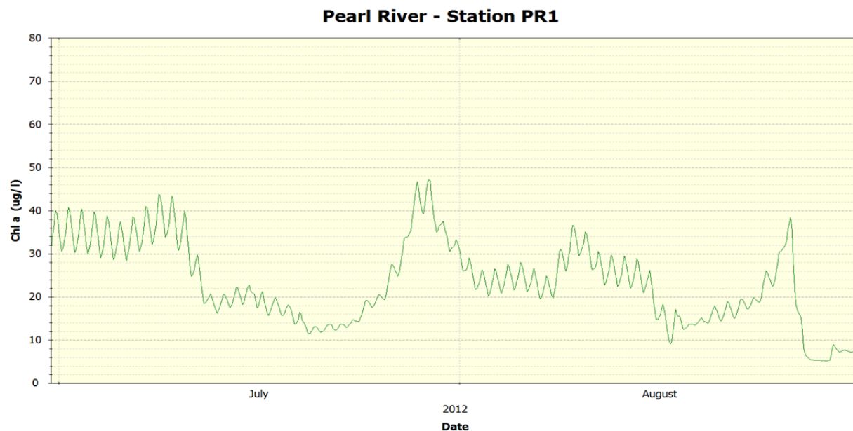
Figure 82 Pearl River Station PR1 – Chl a
