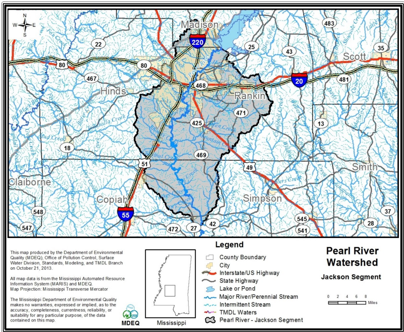
Figure 2 TMDL Segment of the Pearl River
