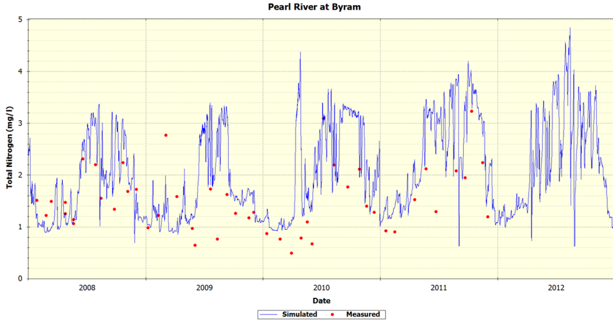
Figure 51 Pearl River at Byram – Simulated vs Measured Total Nitrogen
