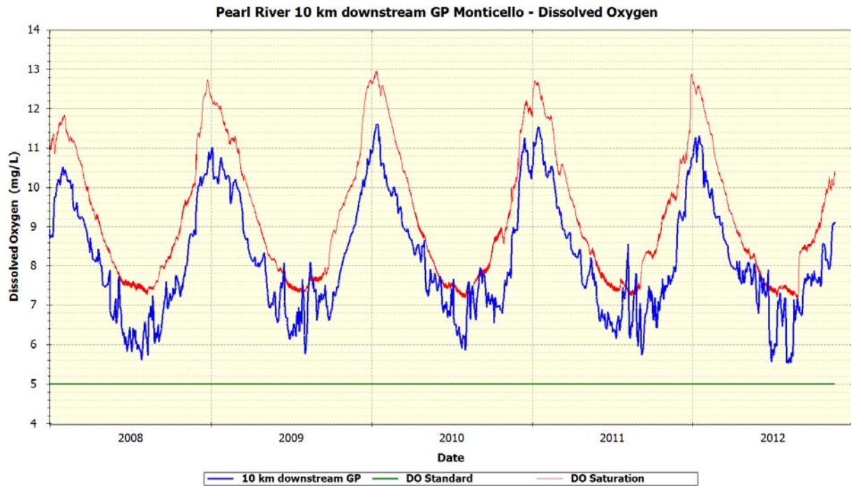
Figure 106 Pearl River 10 km downstream GP – Dissolved Oxygen
