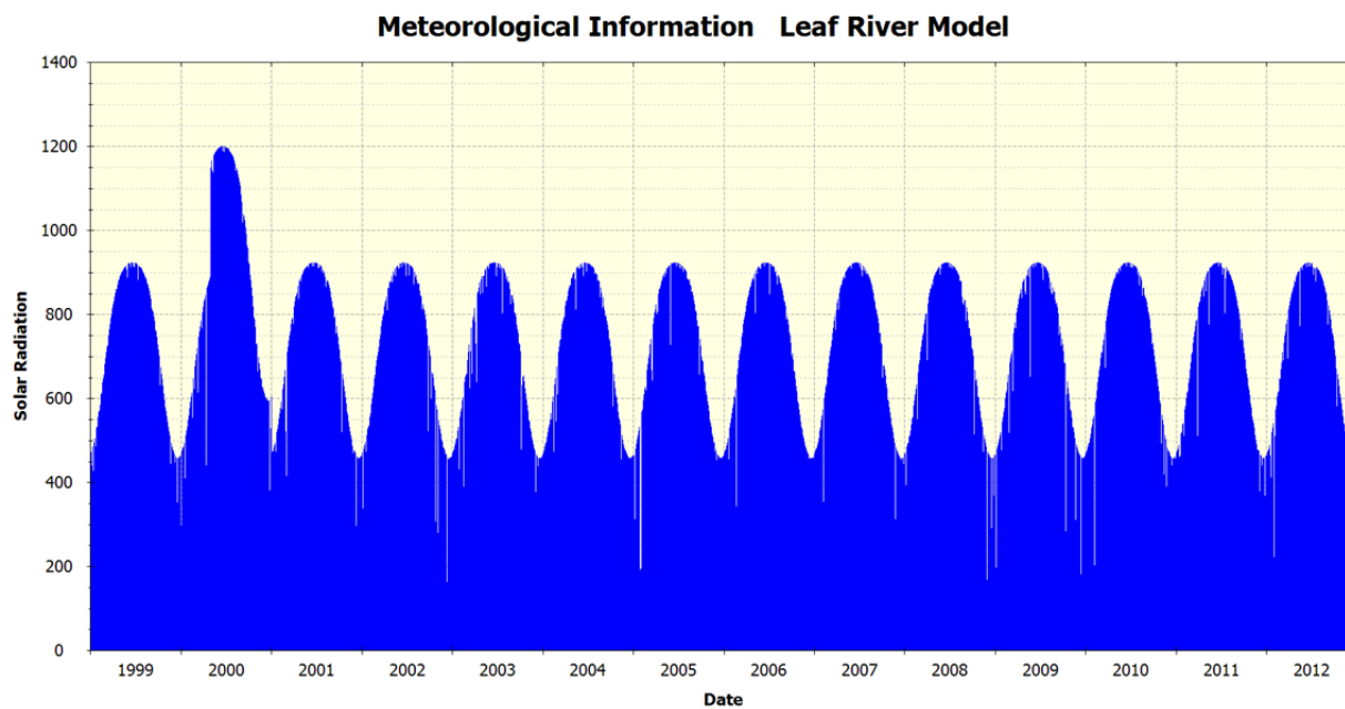
Figure 116 Solar Radiation
