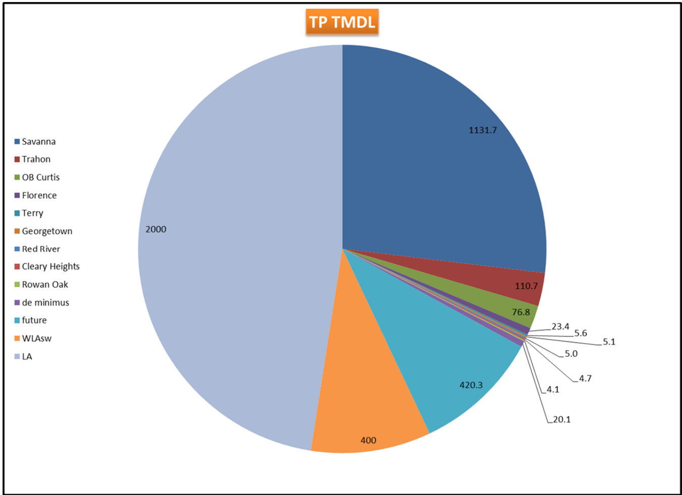
Figure 21 TP TMDL Allocations
