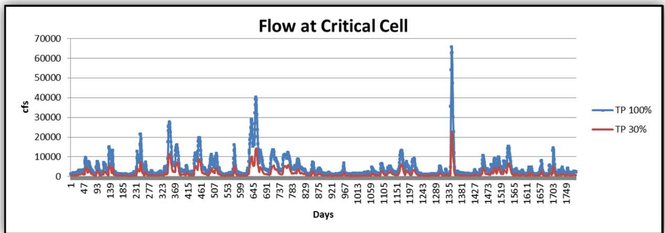
Figure 19 Flow at Model Cell 360
