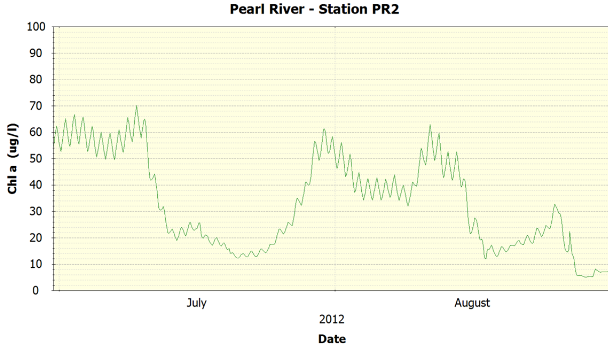
Figure 84 Pearl River Station PR2 – Chl a
