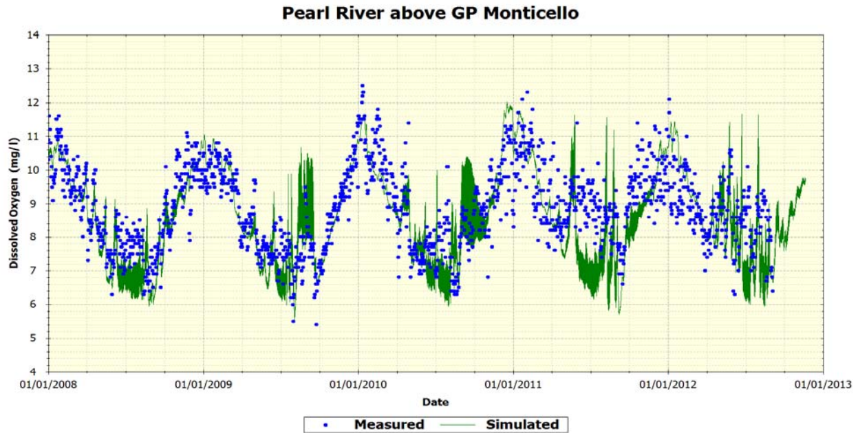
Figure 77 Pearl River above GP Monticello – Dissolved Oxygen
