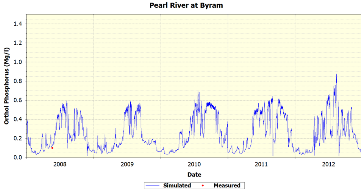
Figure 55 Pearl River at Byram – Simulated vs Measured Ortho-Phosphorous
