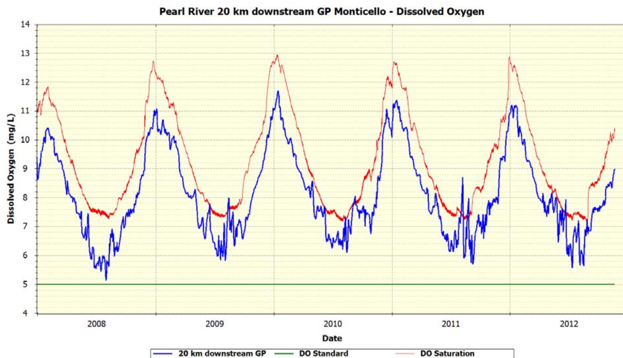
Figure 107 Pearl River 20 km downstream GP – Dissolved Oxygen
