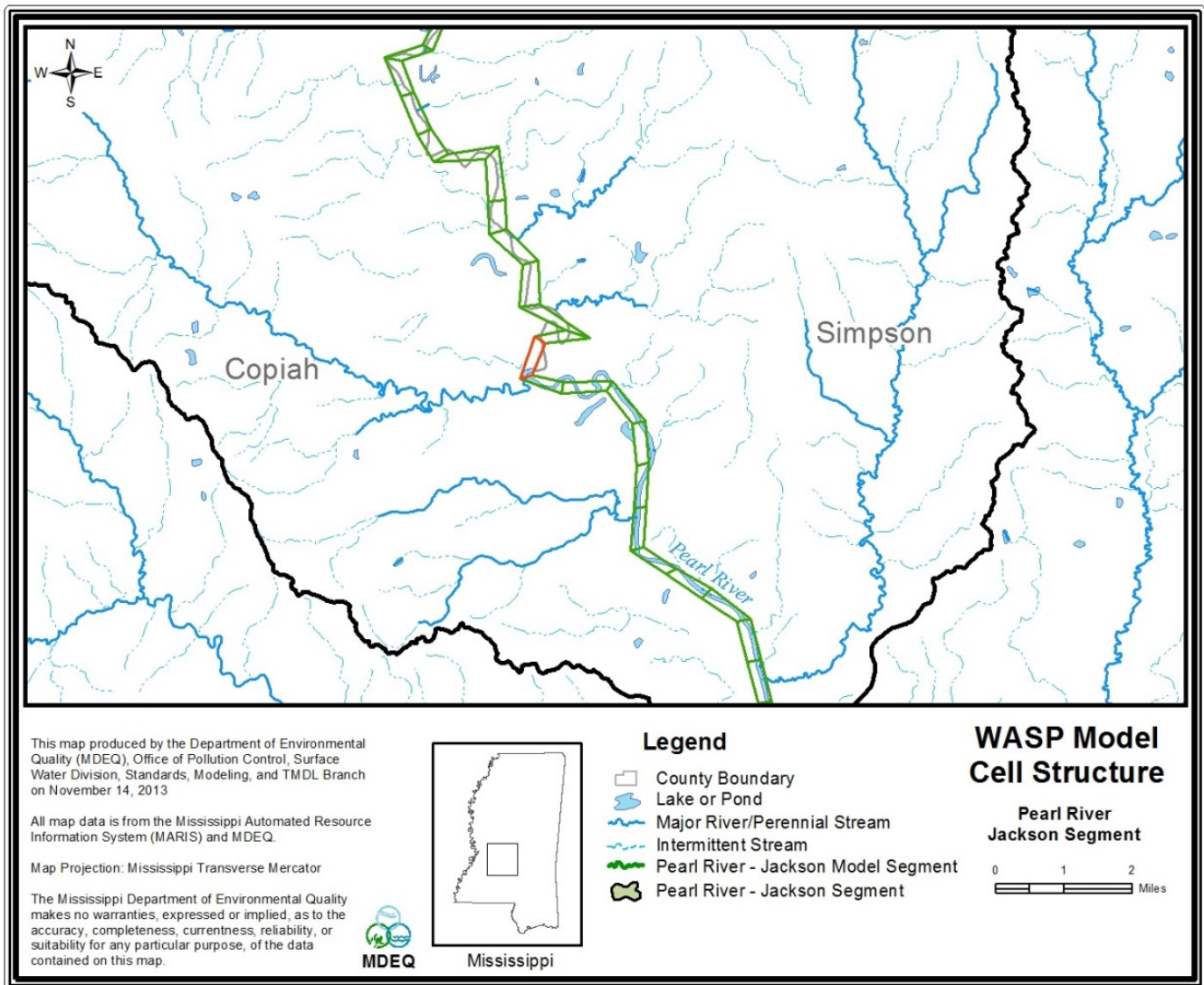
Figure 4 Critical Cell in WASP Model
