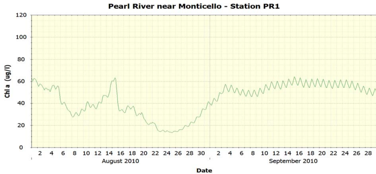
Figure 98 Pearl River near Monticello Station PR1 – Chl a
