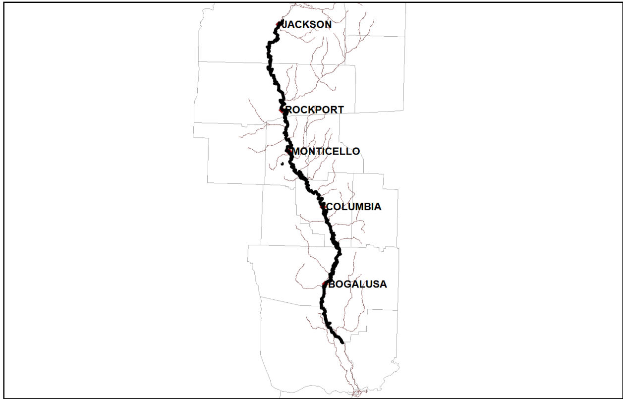
Figure 27 Pearl River Model Grid Full Extent
