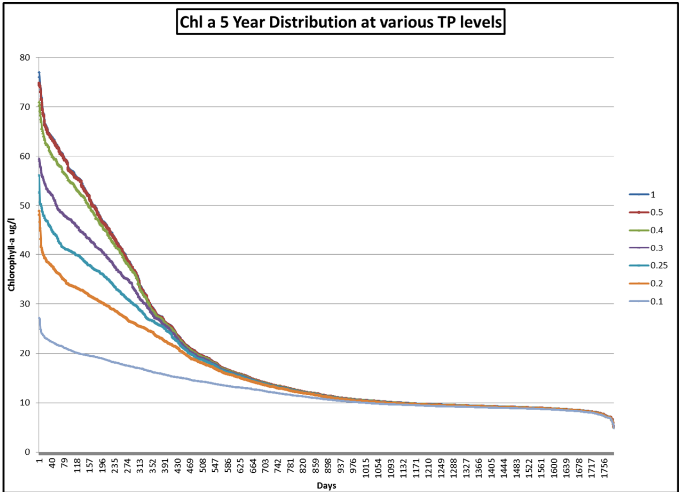
Figure 13 Regression of Chlorophyll-a Model Output at various TP Reductions Model Cell 360
