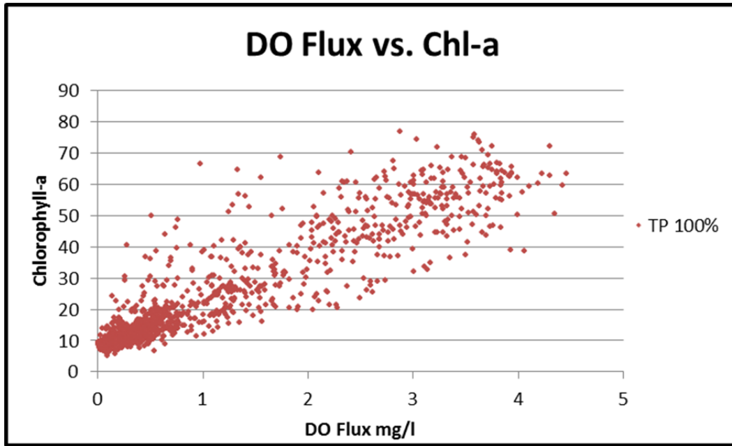
Figure 17 DO Flux vs. Chl-a TN and TP 100%
