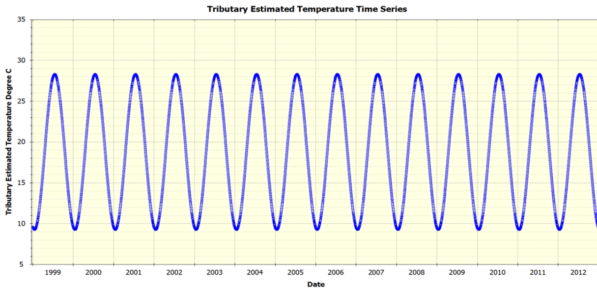
Figure 35 Tributary Temperatures
