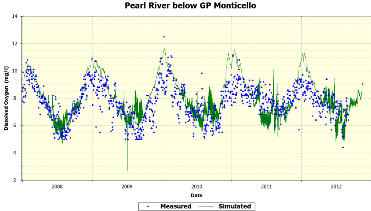
Figure 79 Pearl River below GP Monticello – Dissolved Oxygen
