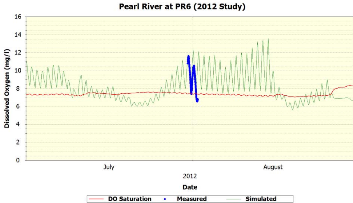
Figure 91 Pearl River Station PR6 – Dissolved Oxygen
