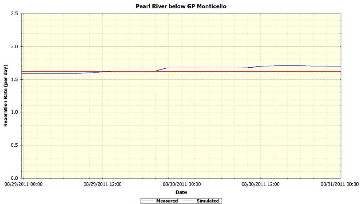
Figure 37 Simulated and Measured Reaeration Rates for Pearl River below GP Monticello
