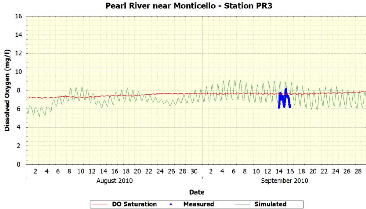
Figure 101 Pearl River near Monticello Station PR3 – Dissolved Oxygen
