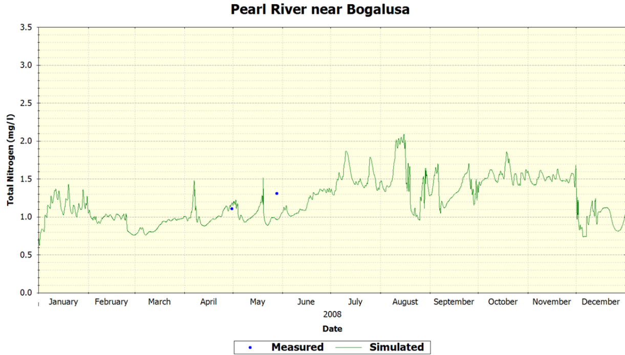
Figure 71 MDEQ Station Pearl River near Bogalusa – Total Nitrogen
