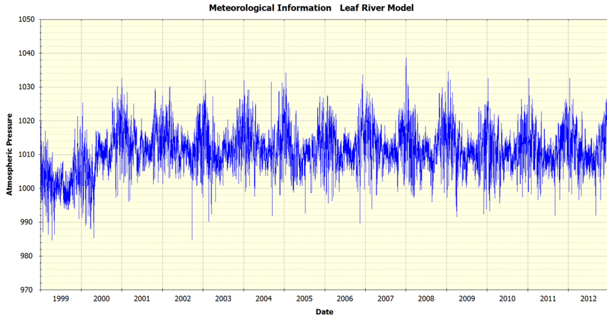
Figure 114 Atmospheric Pressure
