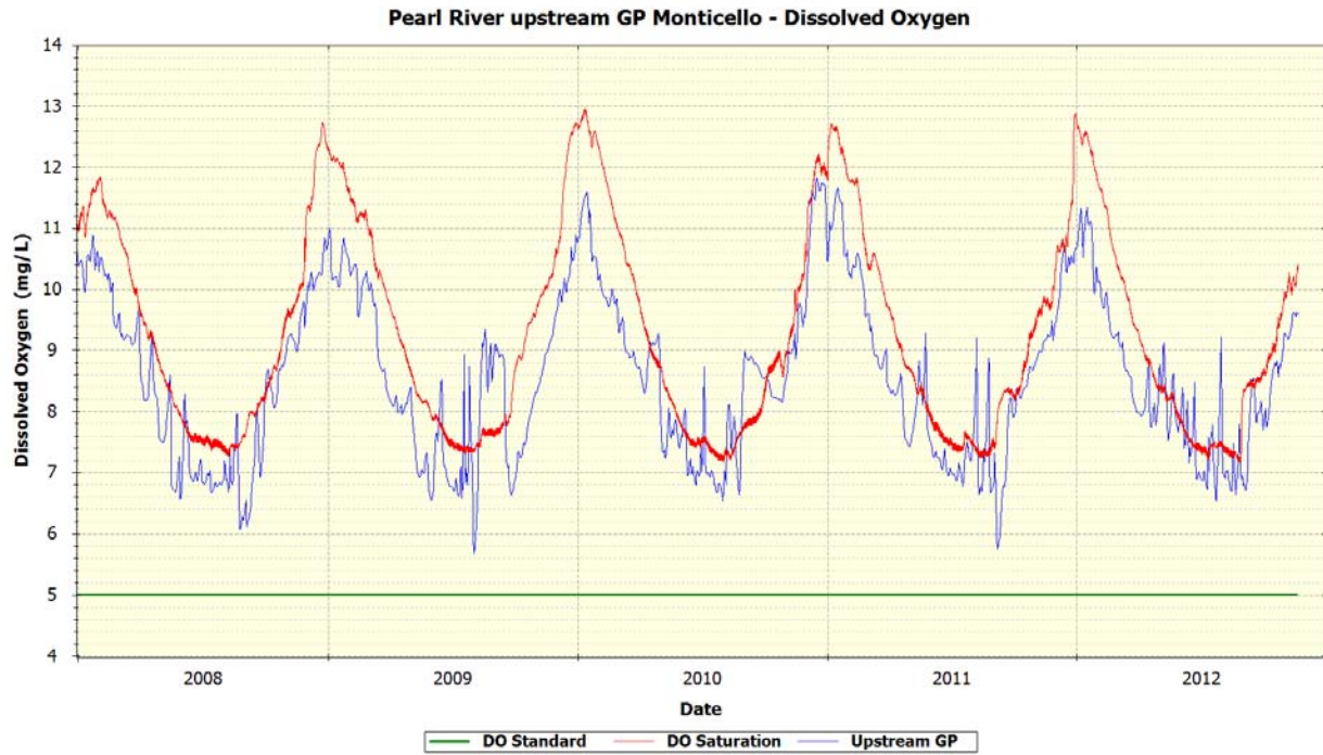
Figure 105 Pearl River upstream GP – Dissolved Oxygen
