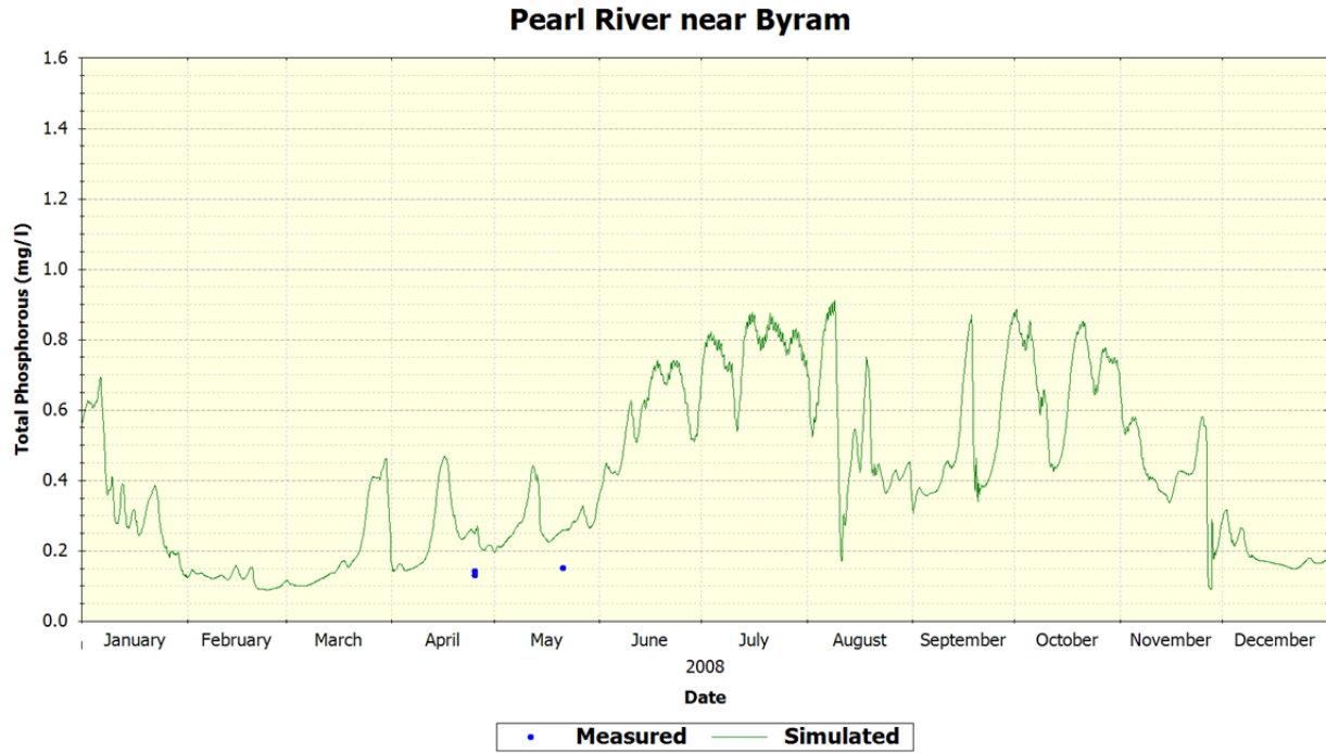
Figure 57 MDEQ Station Pearl River at Byram – Total Phosphorous
