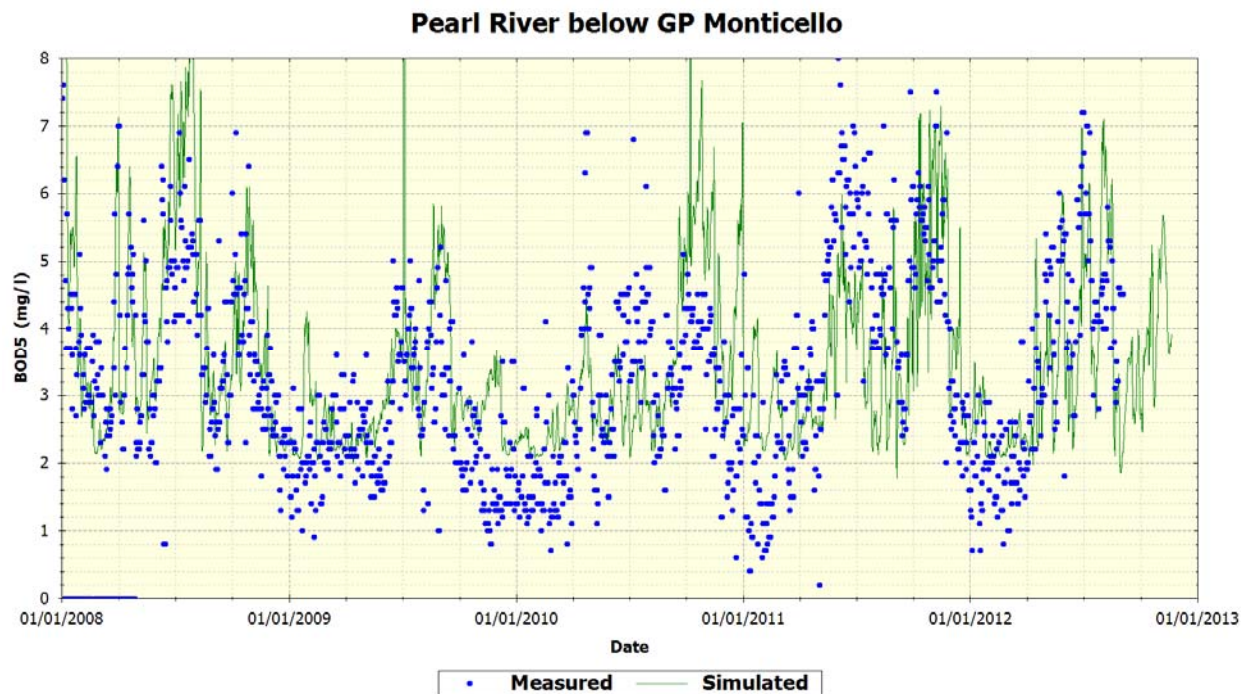
Figure 80 Pearl River below GP Monticello – BOD5
