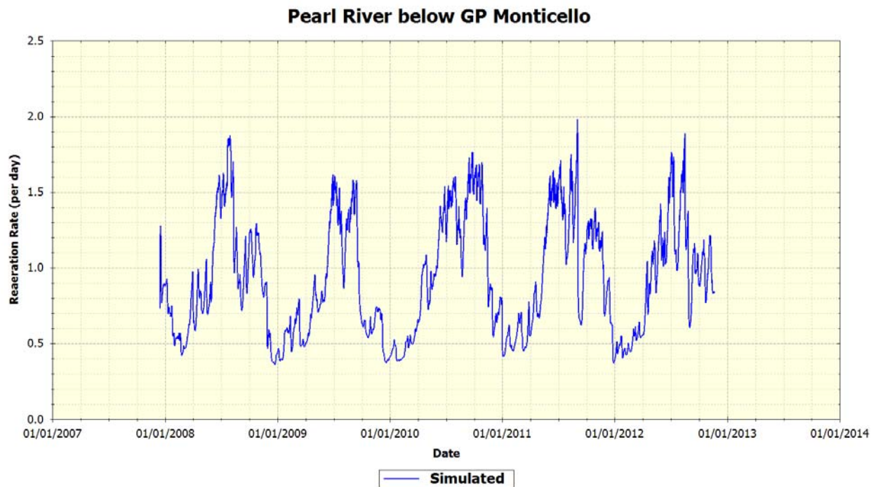
Figure 36 2008 – 2012 Simulated Reaeration Rates Pearl River below GP Monticello
