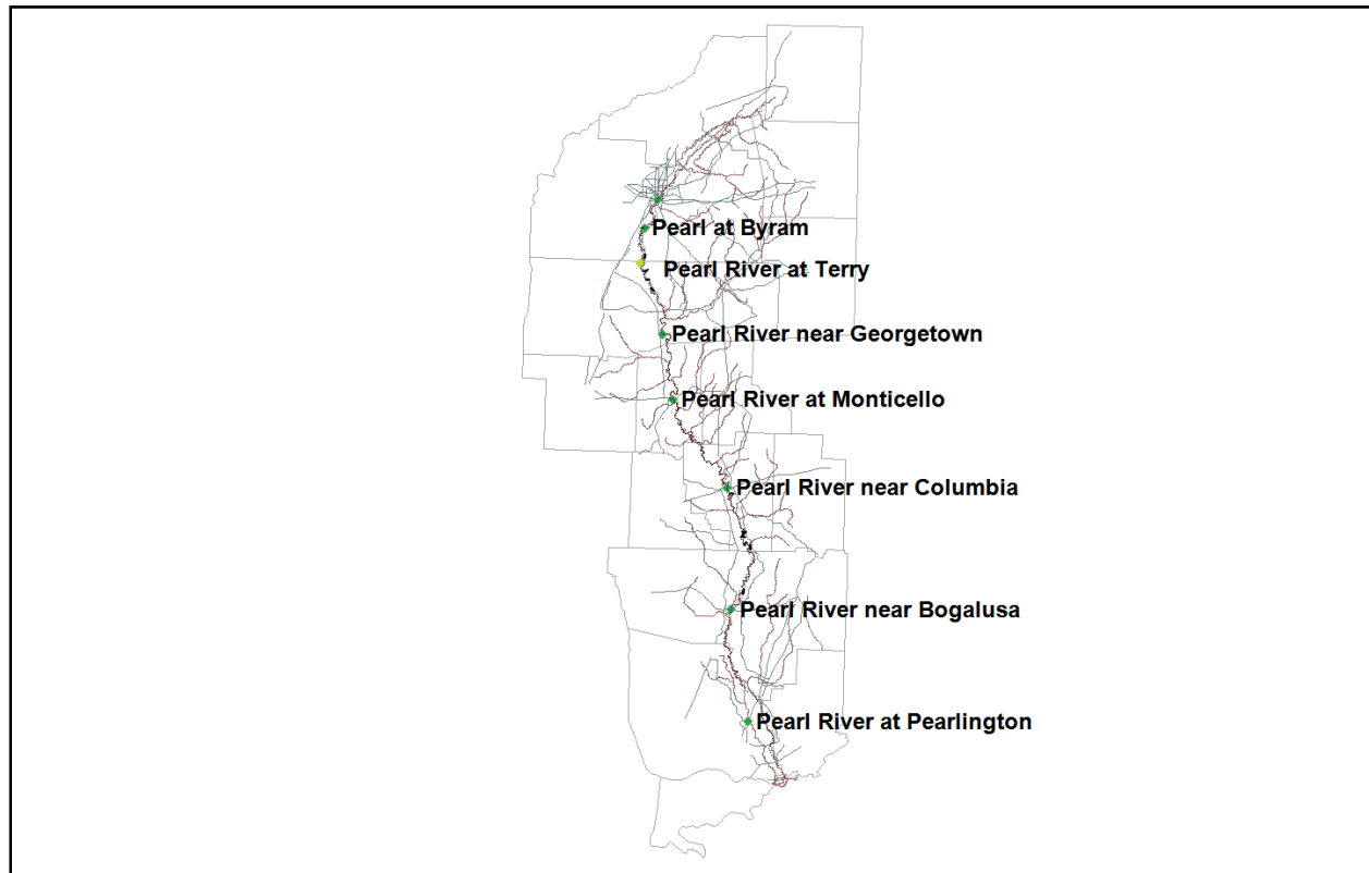
Figure 26 MDEQ 2008 TMDL Study Sampling Stations
