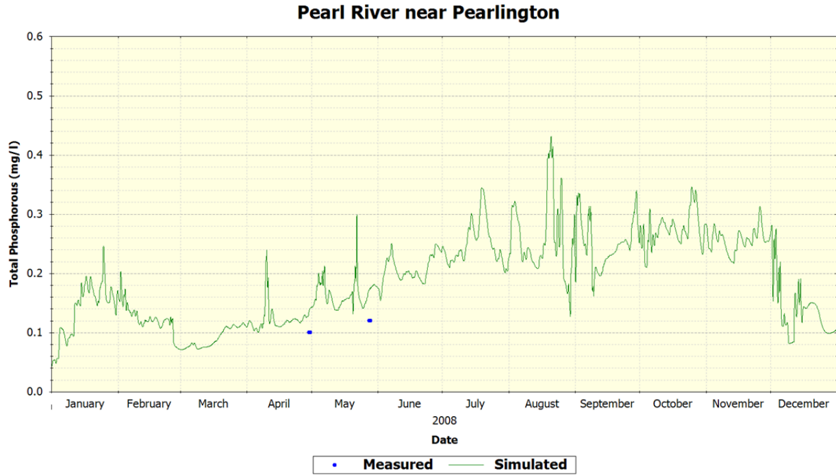
Figure 75 MDEQ Station Pearl River near Pearlington– Total Phosphorous
