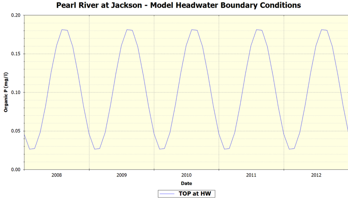
Figure 45 Model Headwater Conditions – Organic Phosphorus
