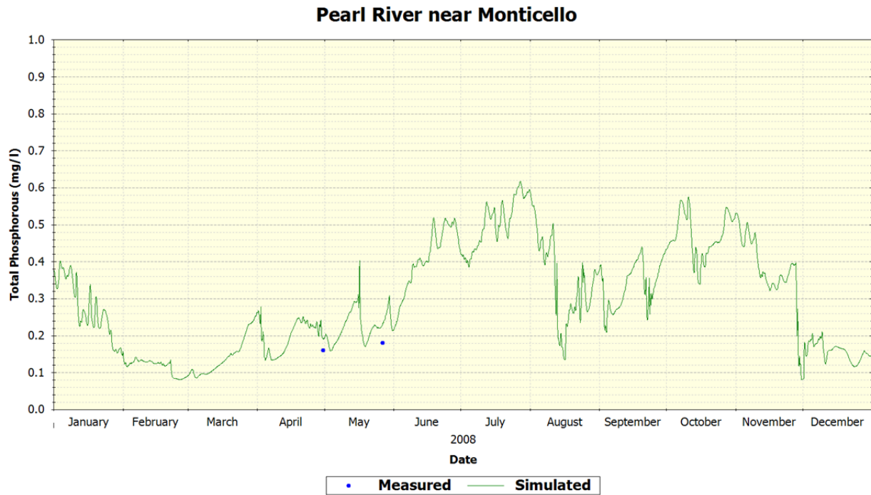
Figure 66 MDEQ Station Pearl River near Georgetown – Total Phosphorus
