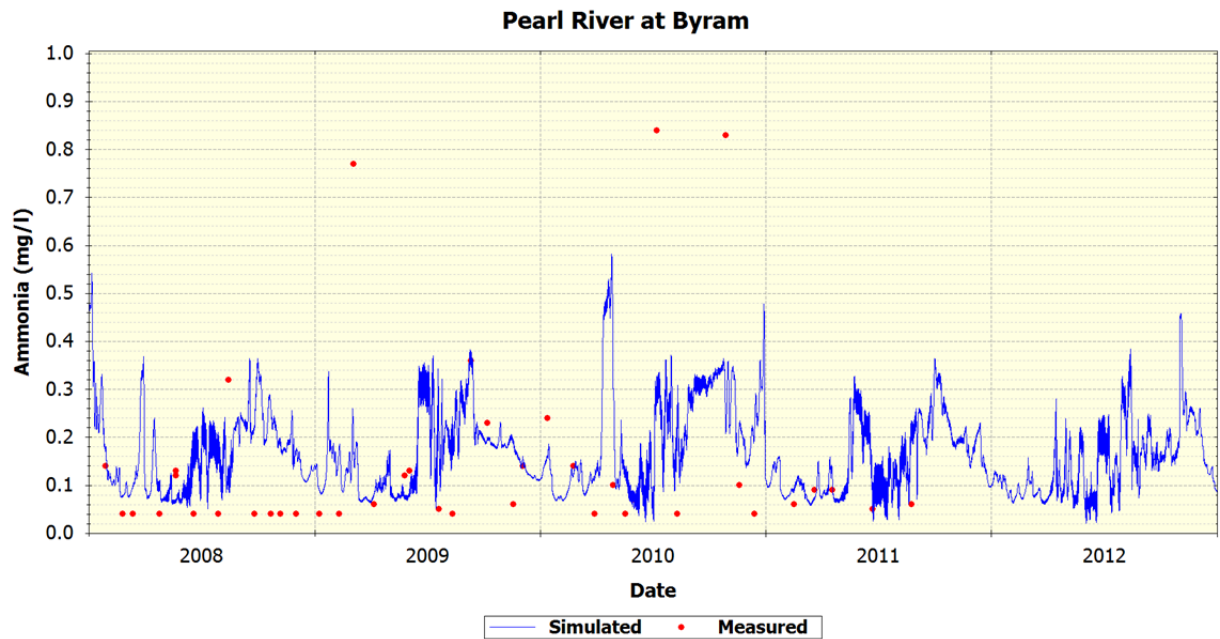
Figure 52 Pearl River at Byram – Simulated vs Measured Ammonia
