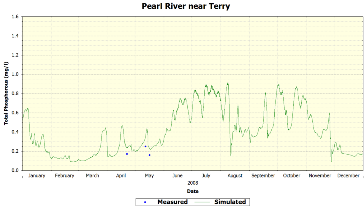
Figure 60 MDEQ Station Pearl River near Terry – Total Phosphorous
