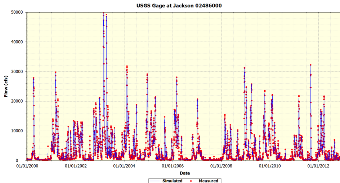
Figure 29 Simulated and Measured Flows – USGS Gage at Jackson
