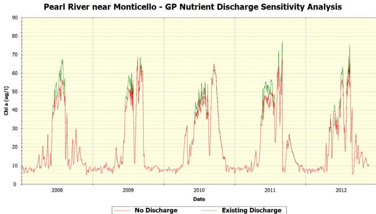
Figure 111 Pearl River Nutrient Sensitivity Analysis – Daily Average Chl a
