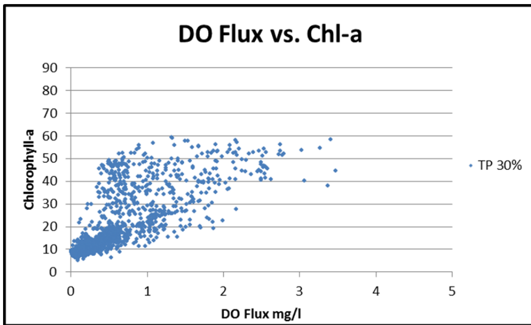
Figure 18 DO Flux vs. Chl-a TP 30%
