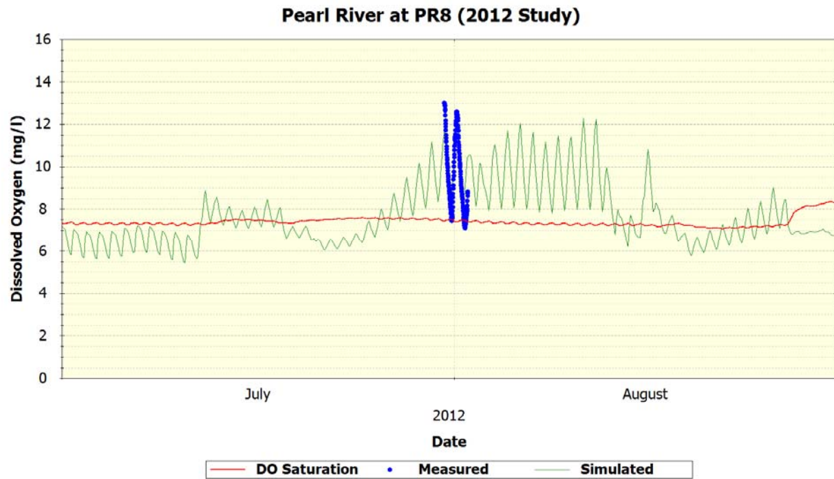
Figure 95 Pearl River Station PR8 – Dissolved Oxygen
