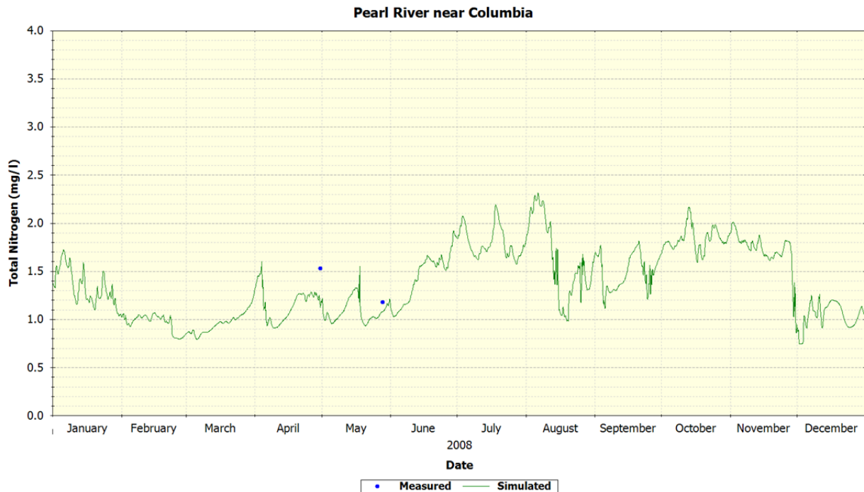
Figure 68 MDEQ Station Pearl River near Columbia – Total Nitrogen
