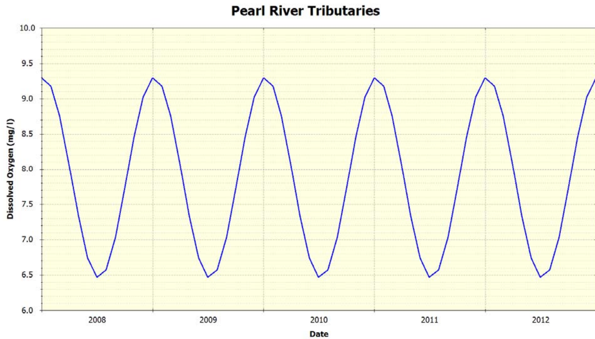
Figure 49 Pearl River Tributary – Dissolved Oxygen Series
