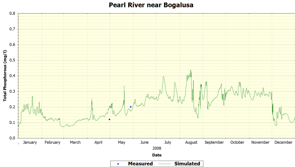
Figure 72 MDEQ Station Pearl River near Bogalusa – Total Phosphorus
