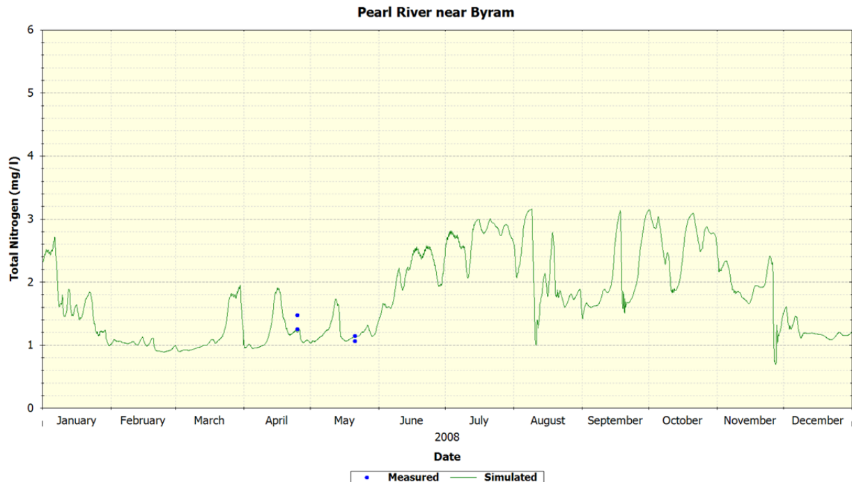
Figure 56 MDEQ Station Pearl River at Byram – Total Nitrogen
