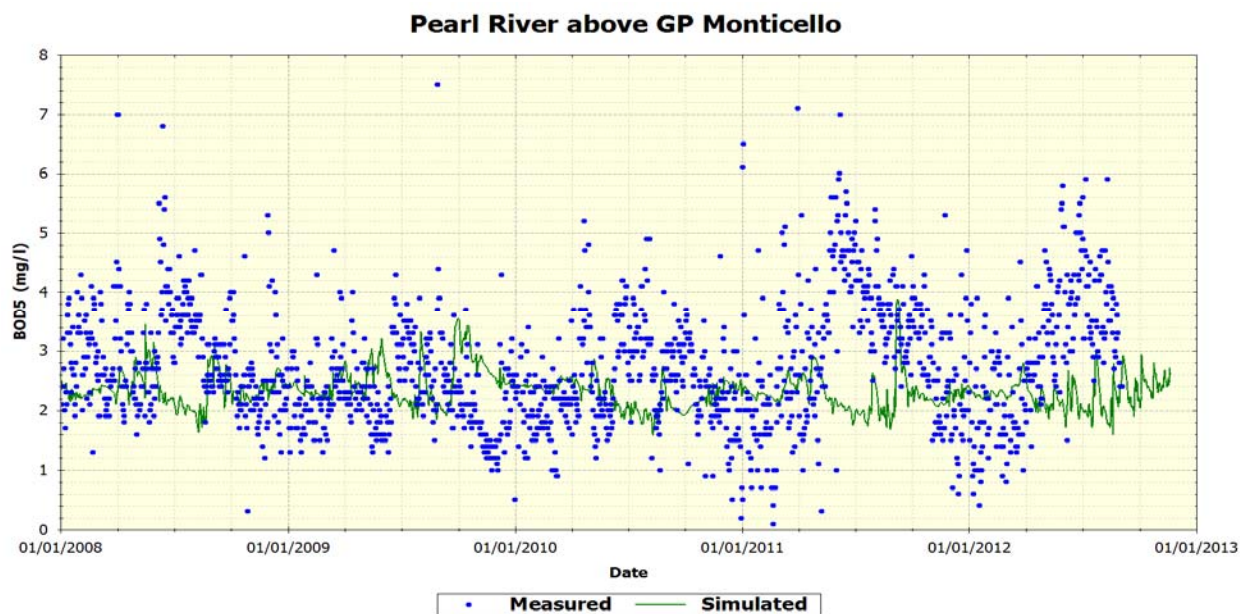
Figure 78 Pearl River above GP Monticello – BOD 5
