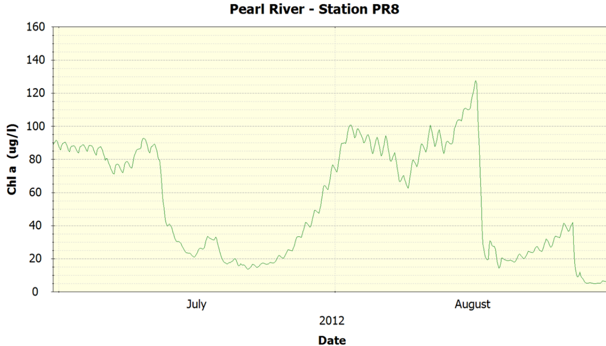
Figure 96 Pearl River Station PR8 – Chl a
