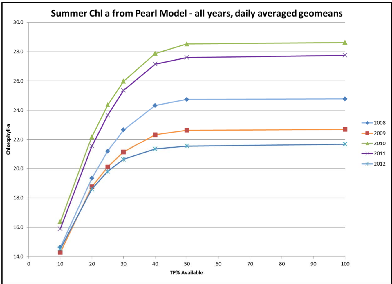
Figure 14 Geometric Means Chl-a at Various TP% Available
