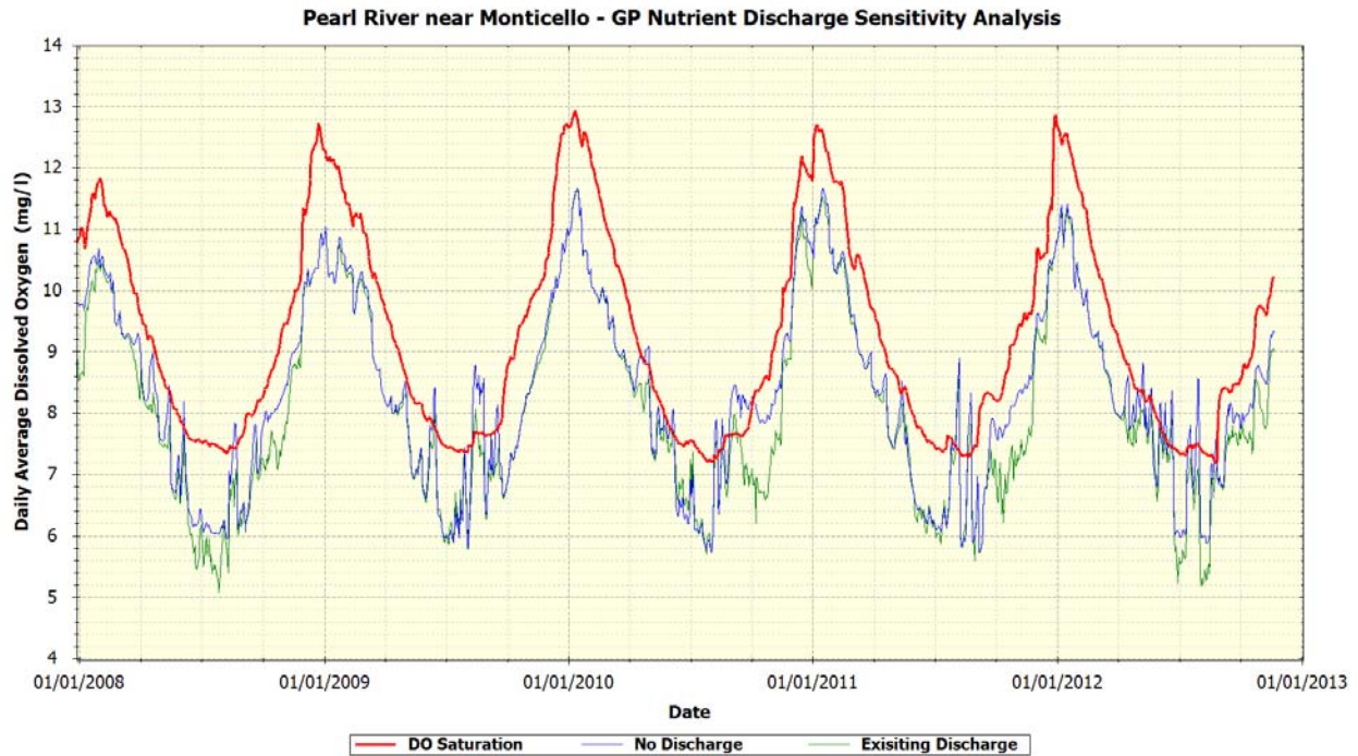
Figure 110 Pearl River Nutrient Sensitivity Analysis – Daily Average Dissolved Oxygen
