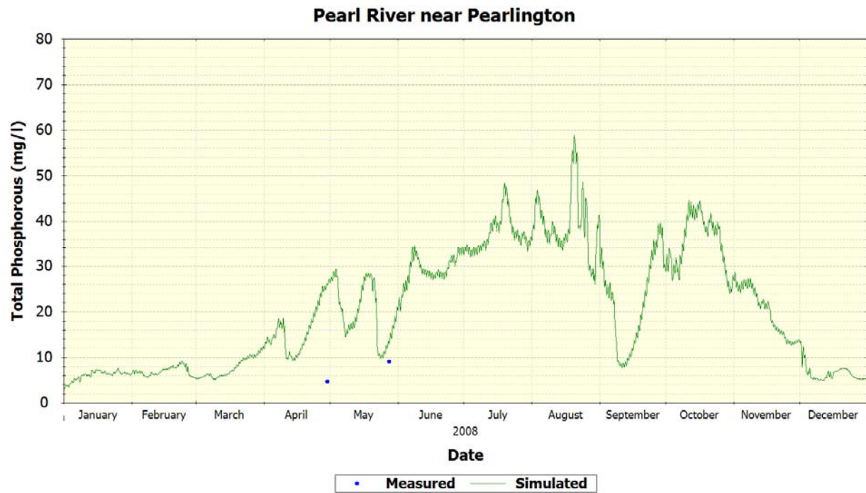
Figure 76 MDEQ Station Pearl River near Pearlington– Chl a
