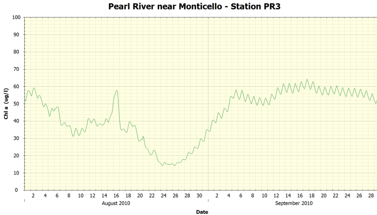
Figure 102 Pearl River near Monticello Station PR3 – Chl a
