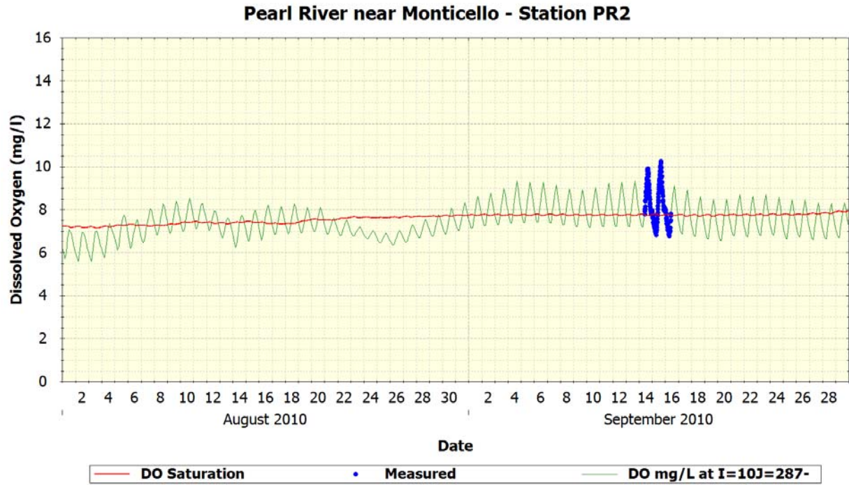
Figure 99 Pearl River near Monticello Station PR2 – Dissolved Oxygen
