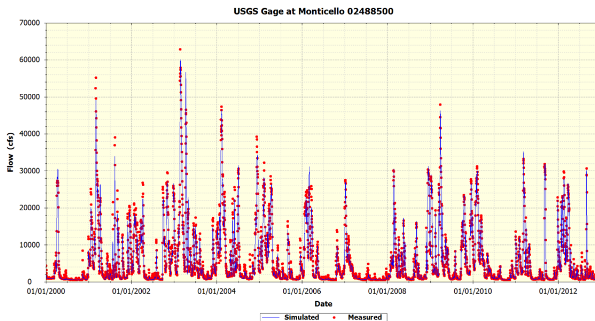
Figure 31 Simulated and Measured Flows – USGS Gage at Monticello
