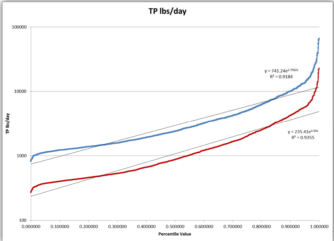
Figure 20 TP Load Regression
