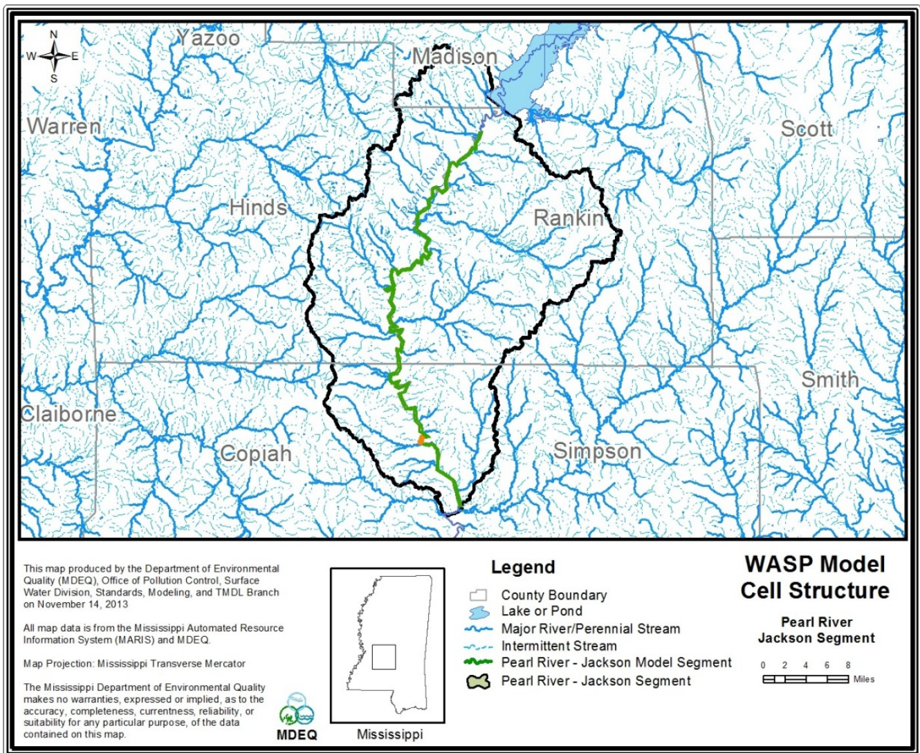
Figure 3 WASP Model Cell Structure (Critical Cell Highlighted)
