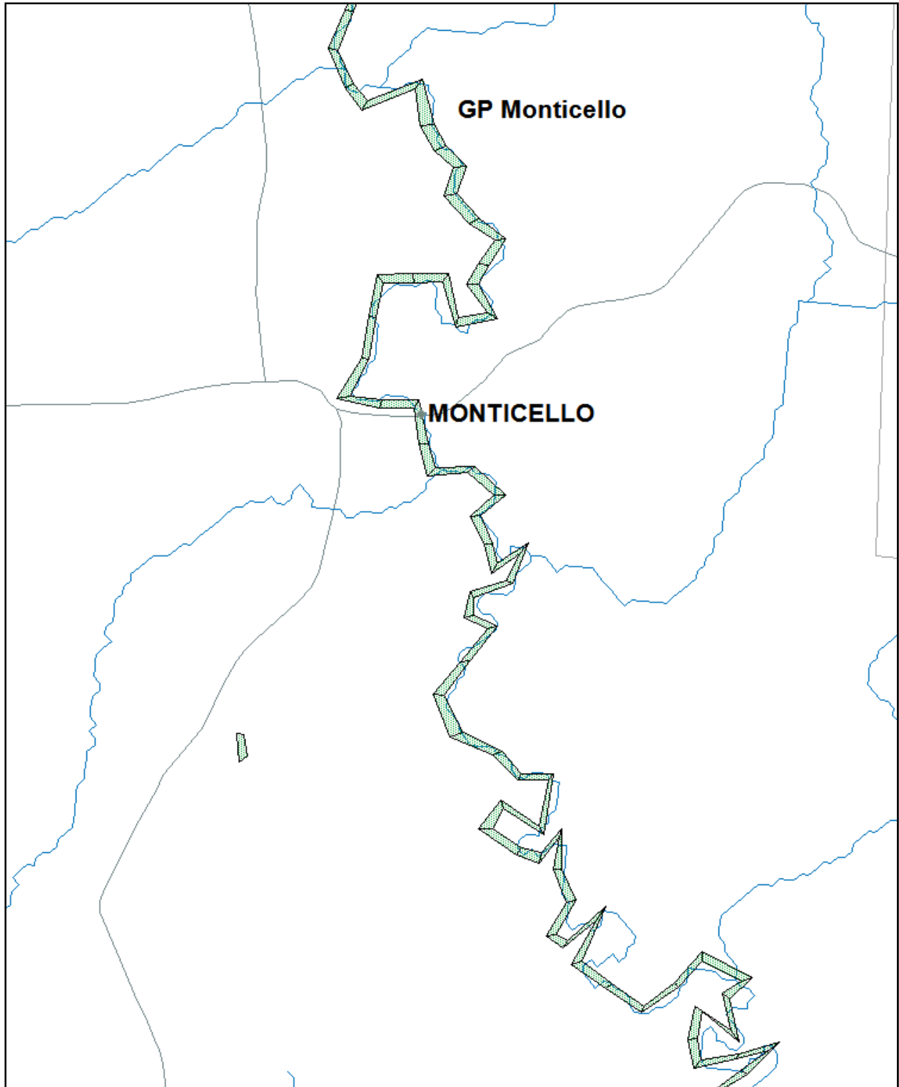
Figure 28 Model Grid near Monticello
