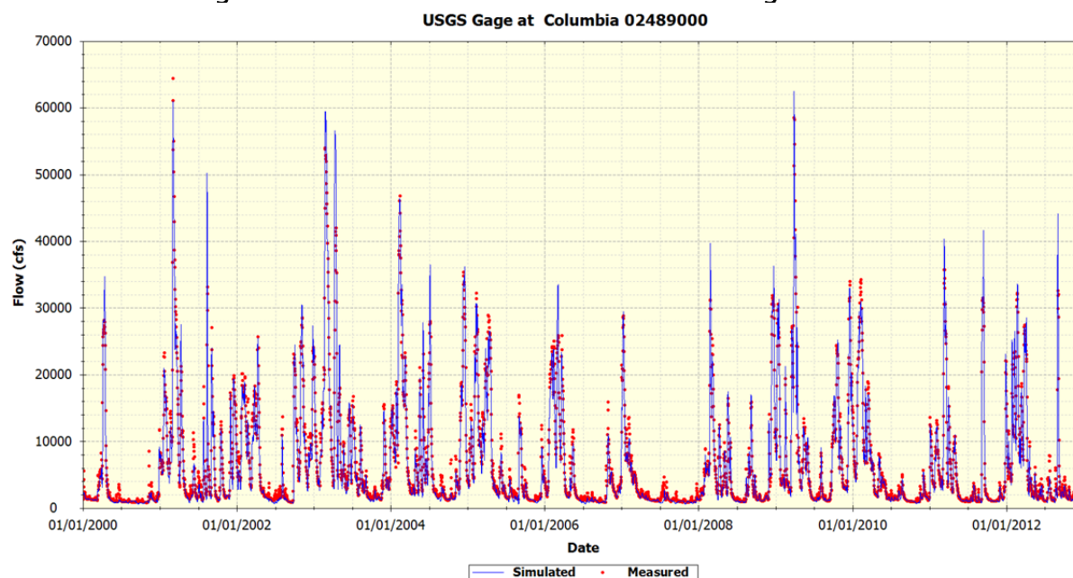
Figure 32 Simulated and Measured Flows – USGS Gage at Columbia
