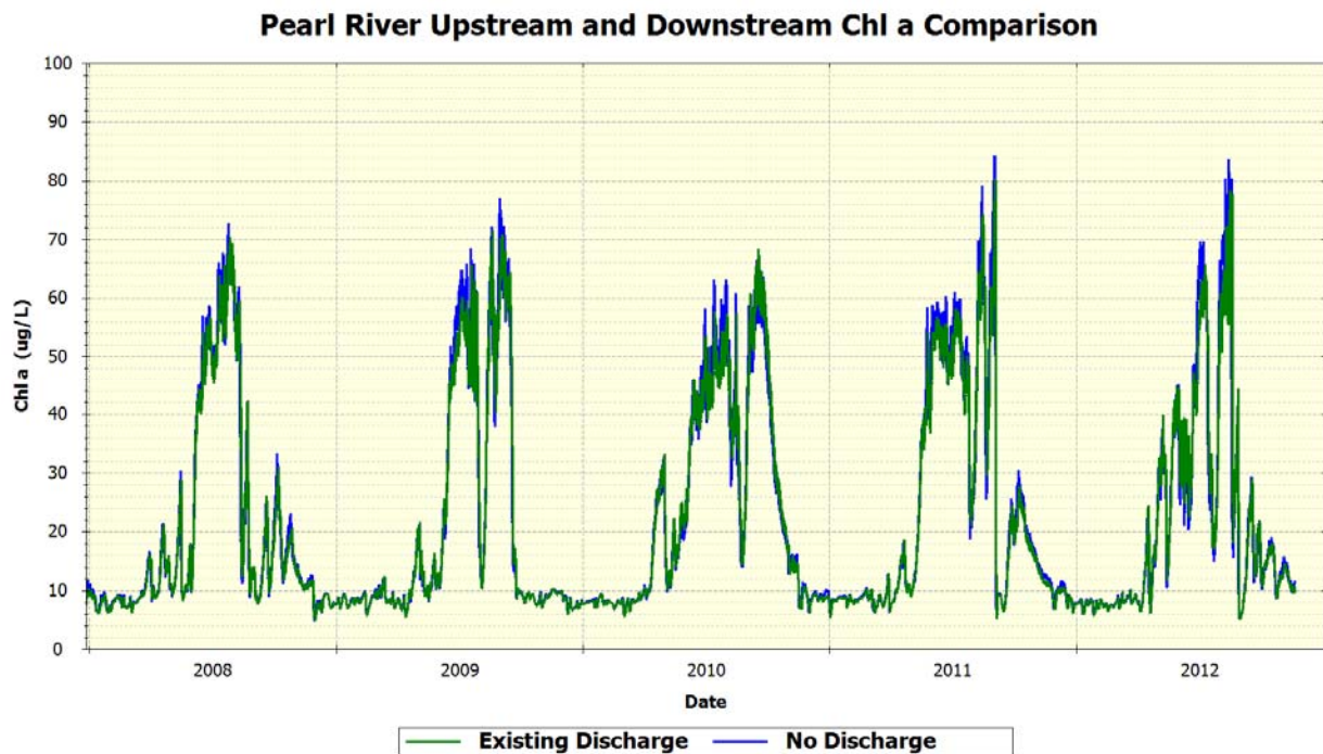
Figure 113 Pearl River Upstream and Downstream Analysis – Daily Average Chl a
