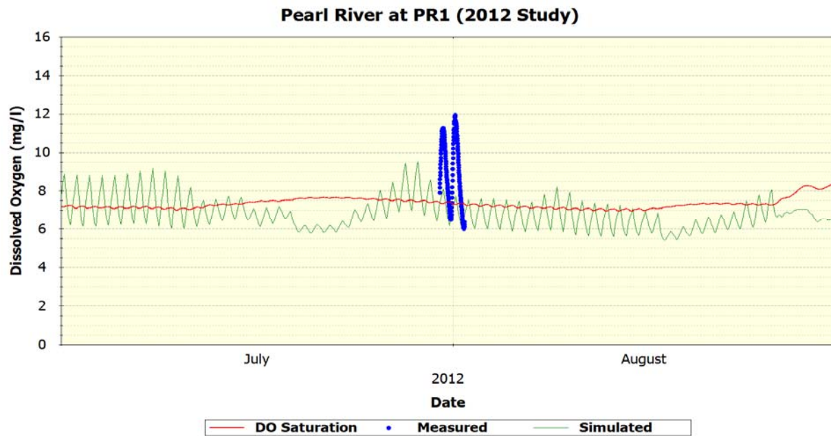
Figure 81 Pearl River Station PR1 – Dissolved Oxygen
