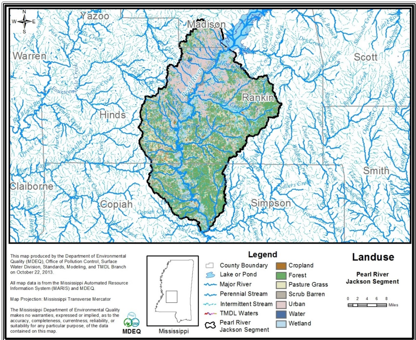
Figure 9 landuse in the Pearl River Jackson Segment (2006 image)
