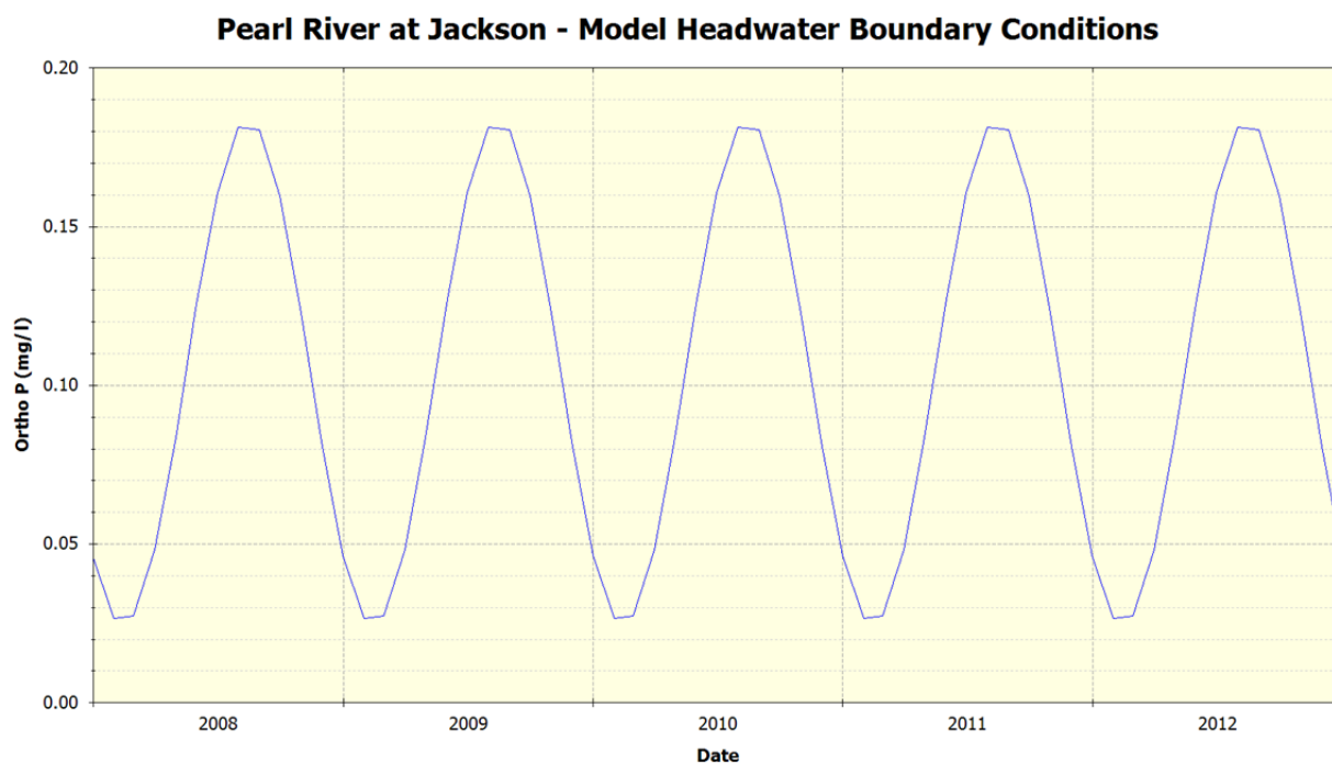
Figure 44 Model Headwater Conditions – Ortho-Phosphorous
