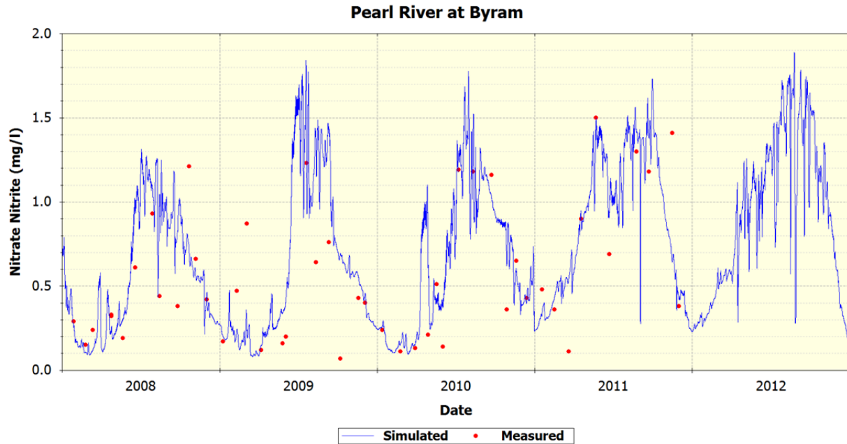
Figure 53 Pearl River at Byram – Simulated vs Measured Nitrate-Nitrite
