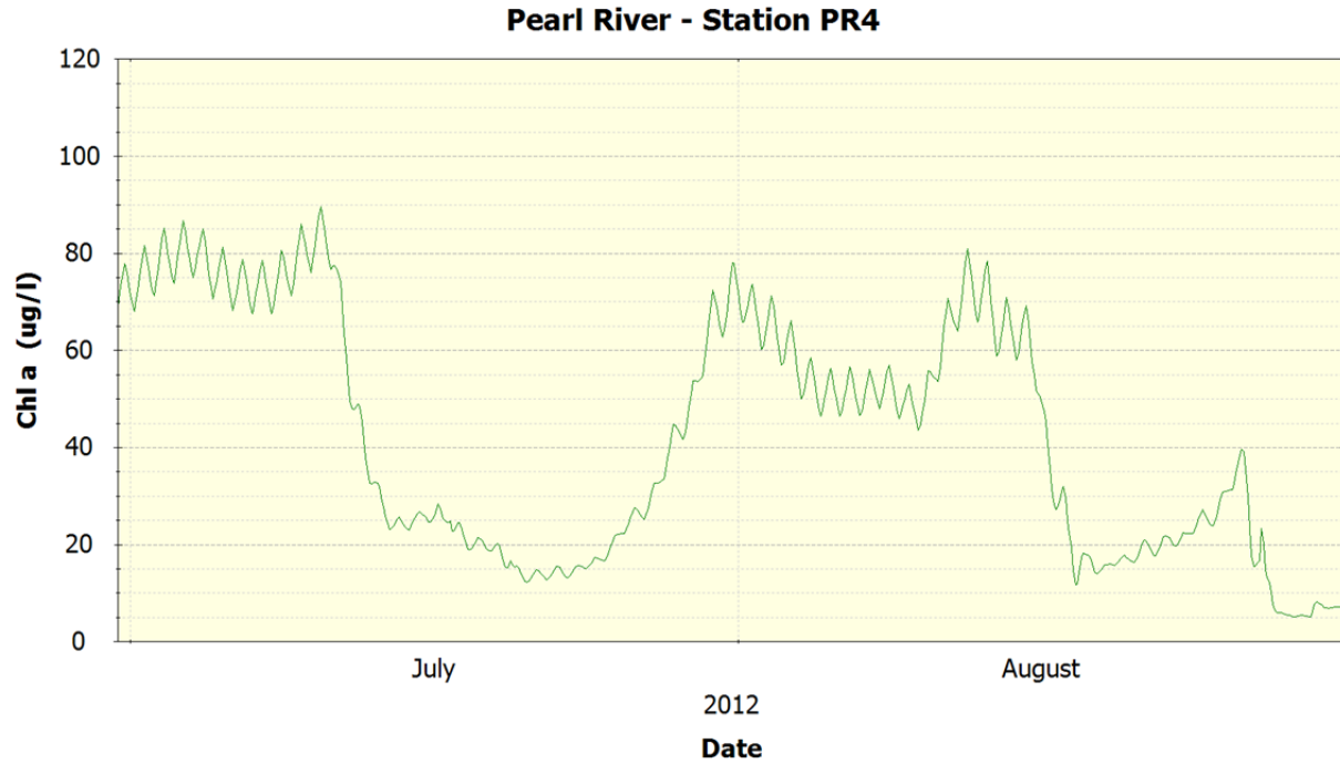
Figure 88 Pearl River Station PR4 – Chl a
