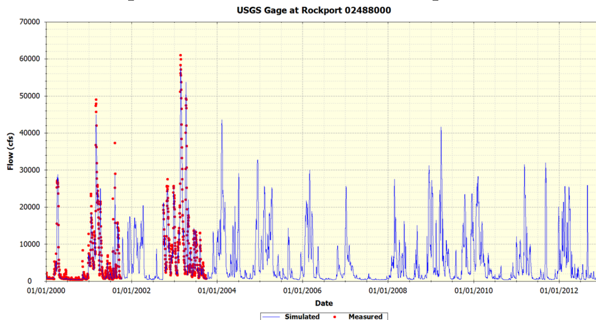
Figure 30 Simulated and Measured Flows – USGS Gage at Rockport
