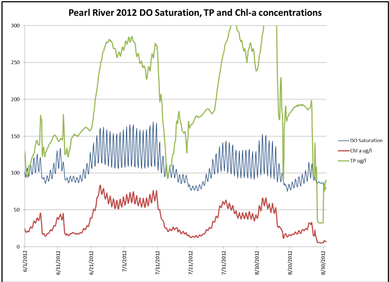
Figure 7 Calibrated Model Output Critical Cell Growing Season, 2012
