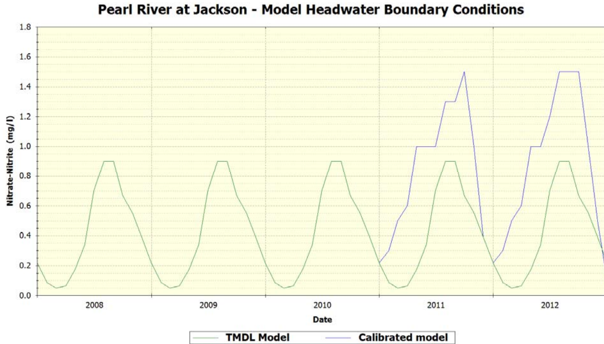
Figure 42 Model Headwater Conditions - Nitrate-Nitrite
