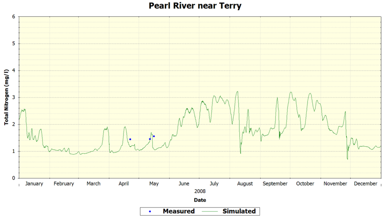
Figure 59 MDEQ Station Pearl River near Terry – Total Nitrogen
