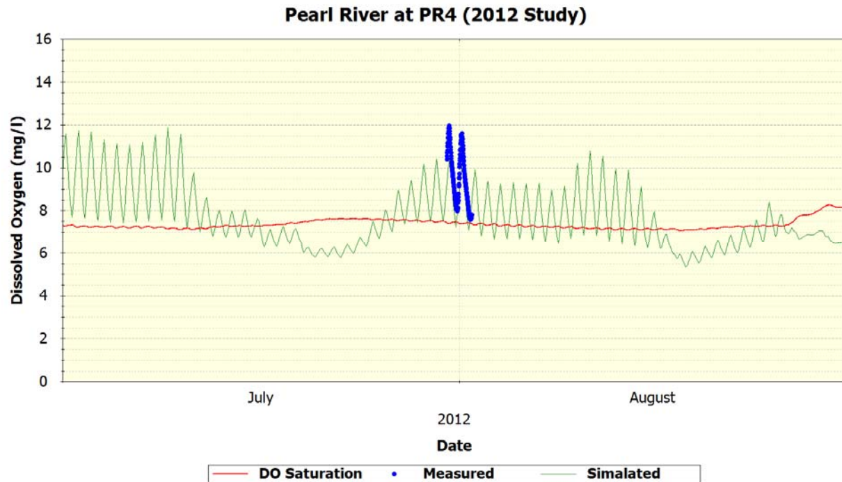
Figure 87 Pearl River Station PR4 – Dissolved Oxygen
