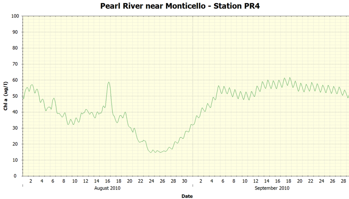
Figure 104 Pearl River near Monticello Station PR4 – Chl a
