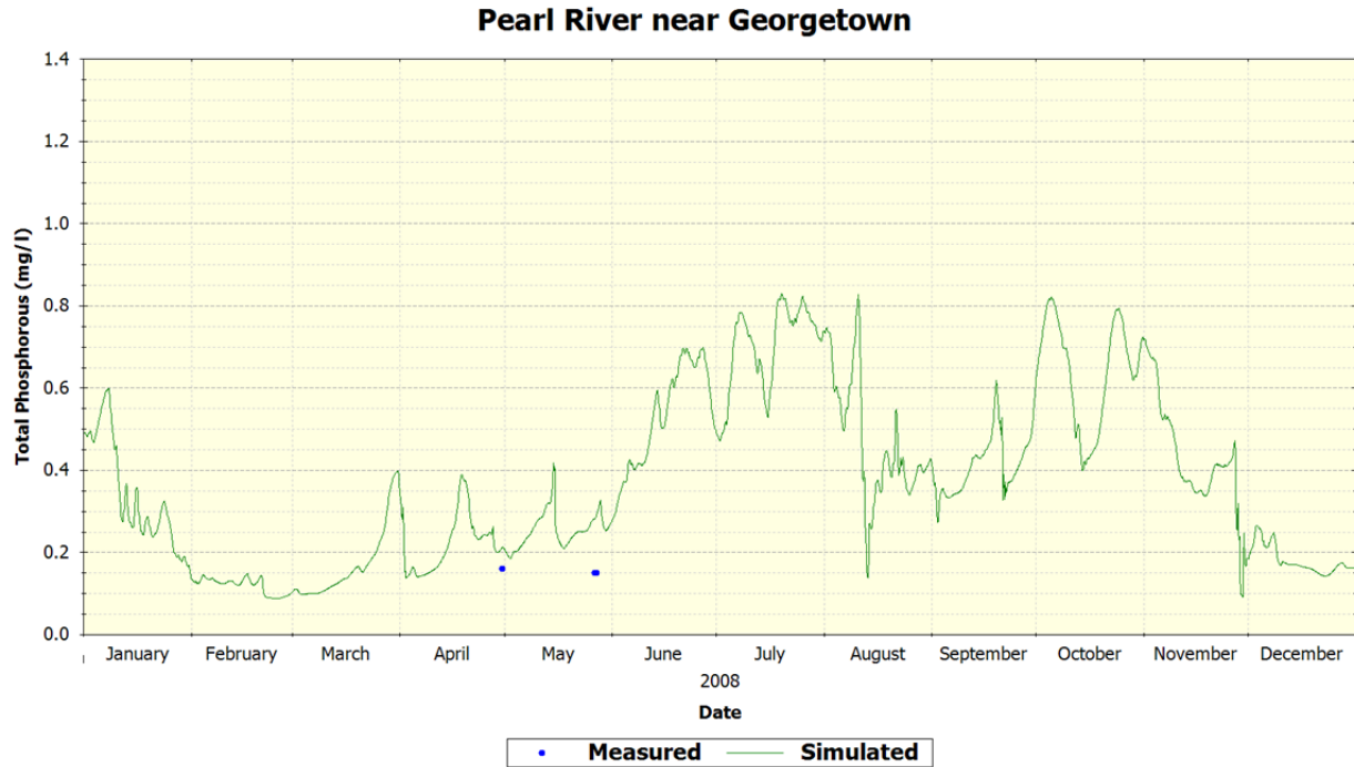
Figure 63 MDEQ Station Pearl River near Georgetown – Total Phosphorous
