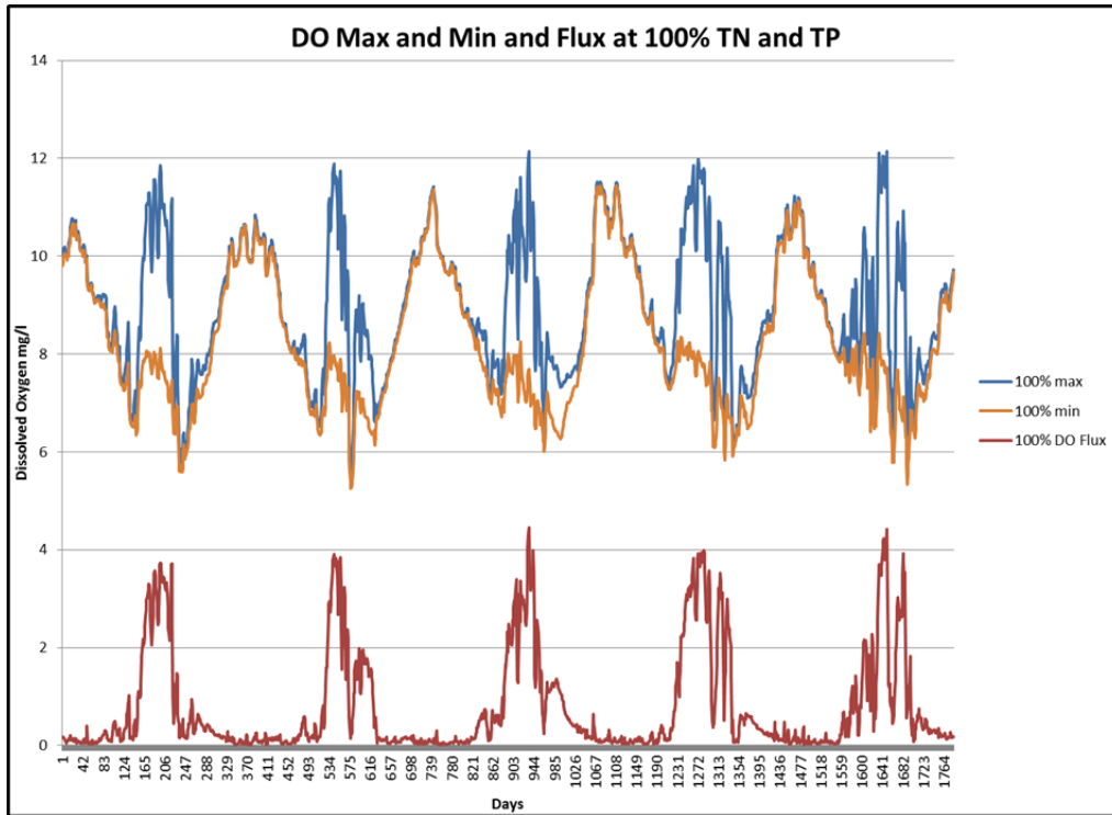
Figure 15 DO Flux at 100% TN and TP
