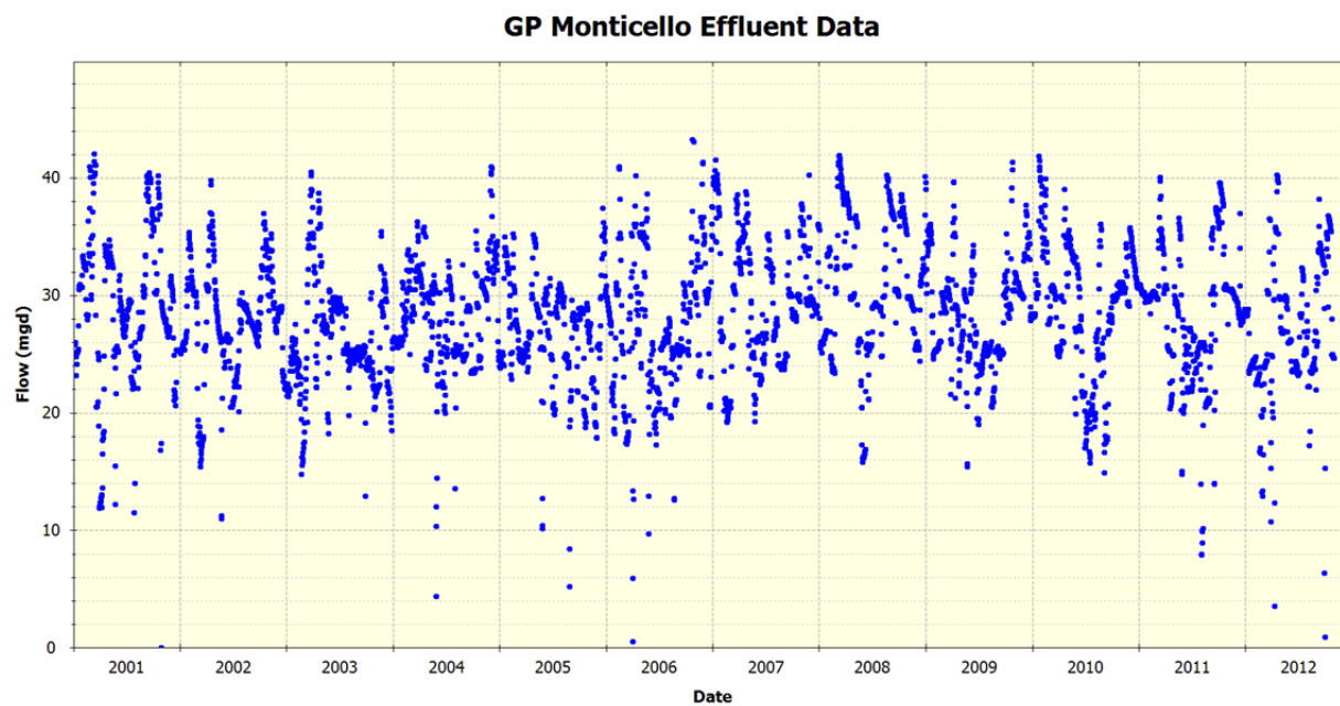
Figure 38 GP Monticello Effluent Discharge Flow Data
