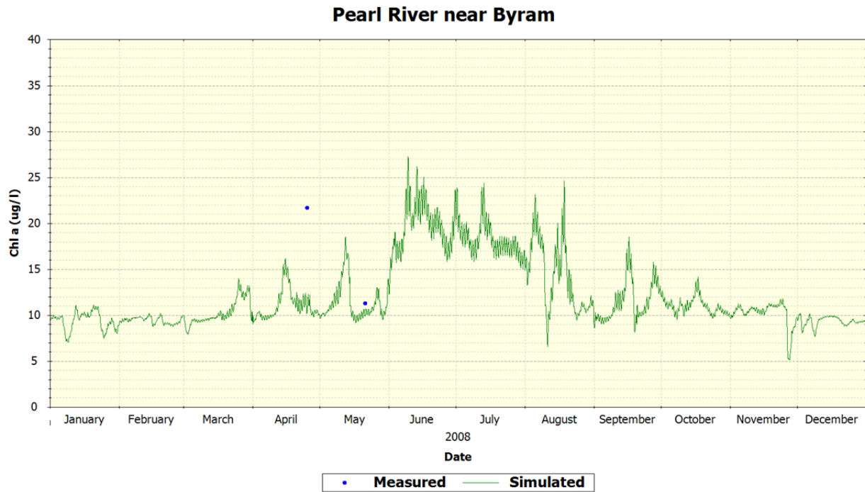
Figure 58 MDEQ Station Pearl River at Byram – Chl a
