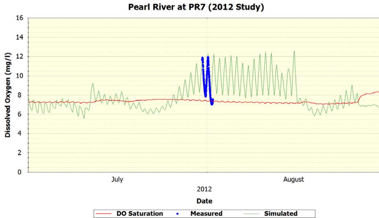
Figure 93 Pearl River Station PR7 – Dissolved Oxygen
