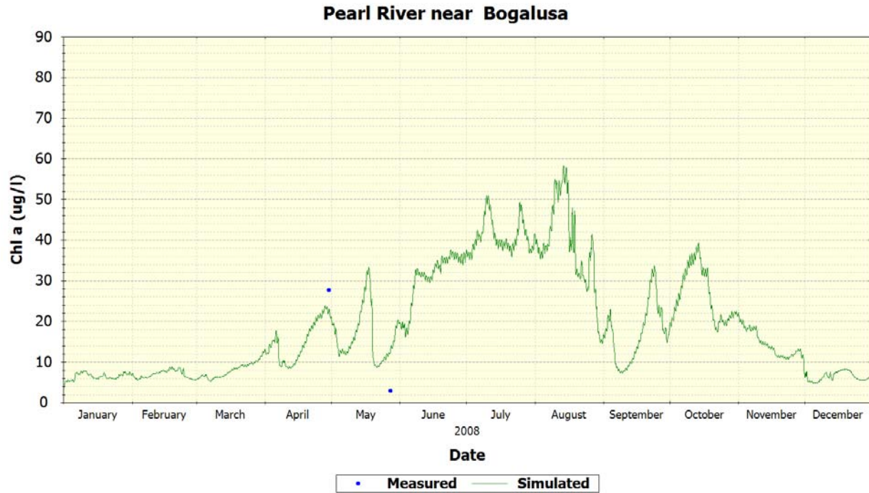
Figure 73 MDEQ Station Pearl River near Bogalusa – Chl a
