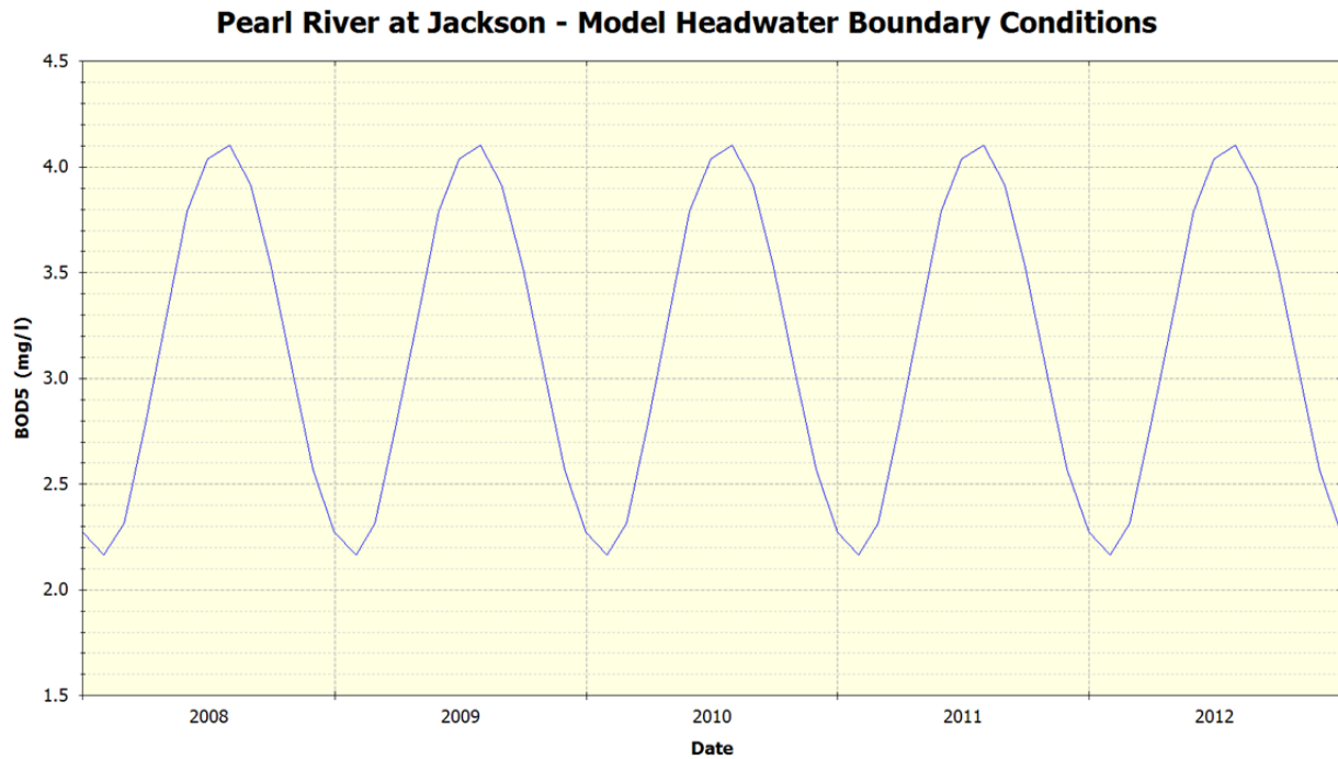
Figure 46 Model Headwater Conditions – BOD5
