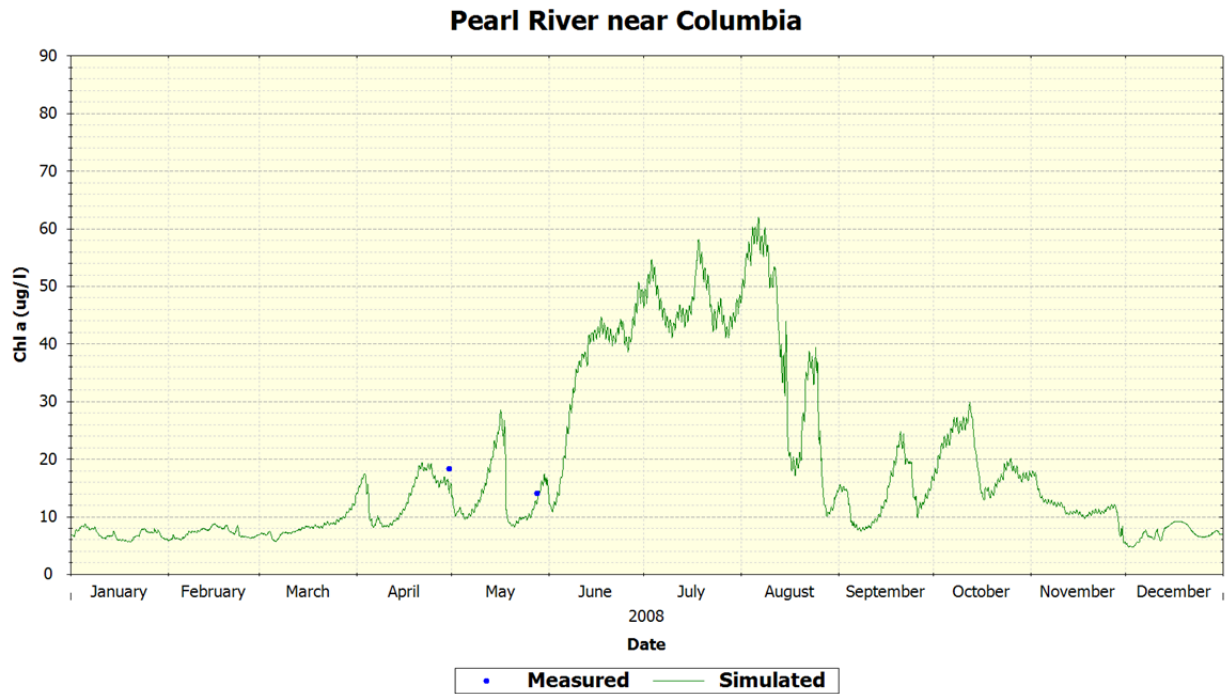
Figure 70 MDEQ Station Pearl River near Columbia – Chl a
