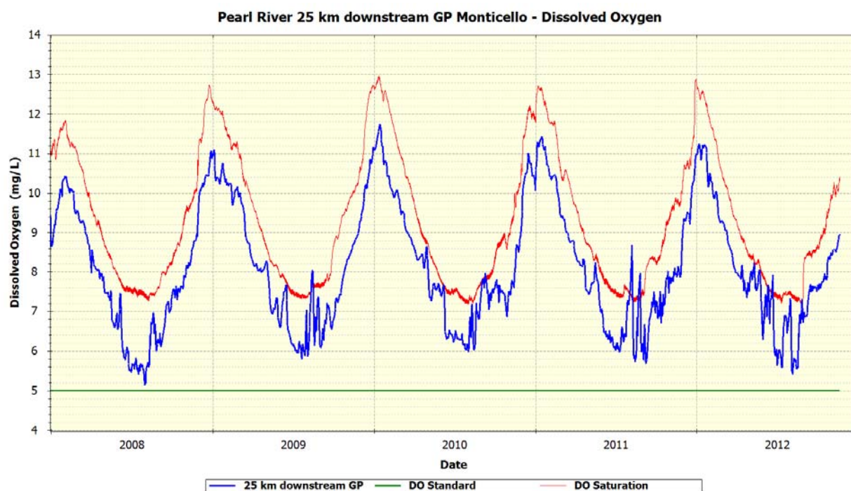
Figure 108 Pearl River 25 km downstream GP – Dissolved Oxygen – DO Sag Area
