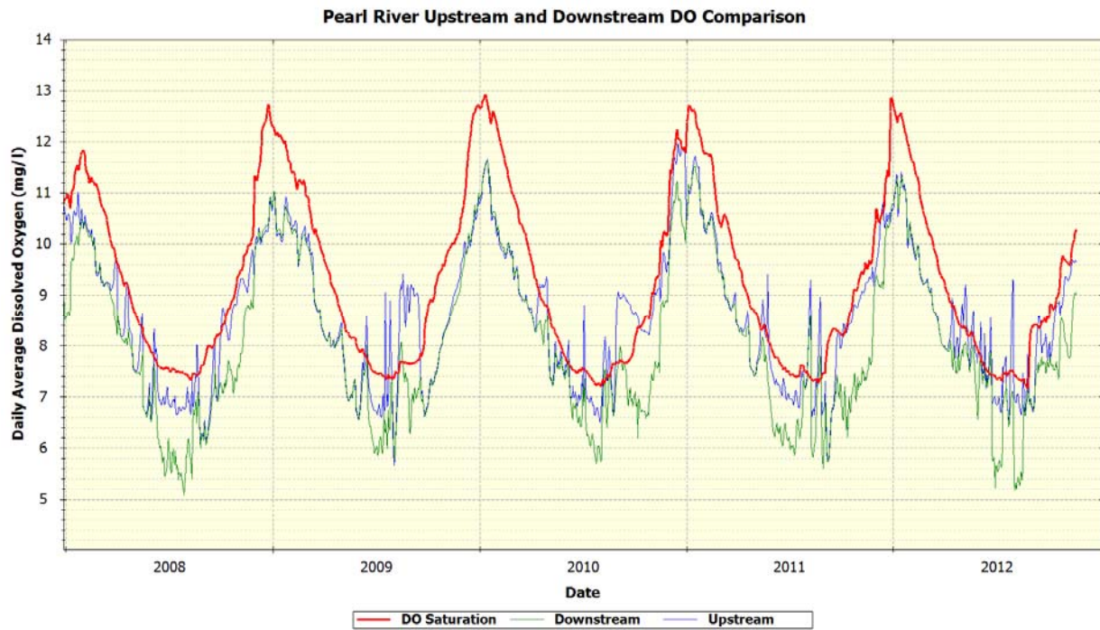
Figure 112 Pearl River Upstream and Downstream Analysis – Daily Average Dissolved Oxygen
