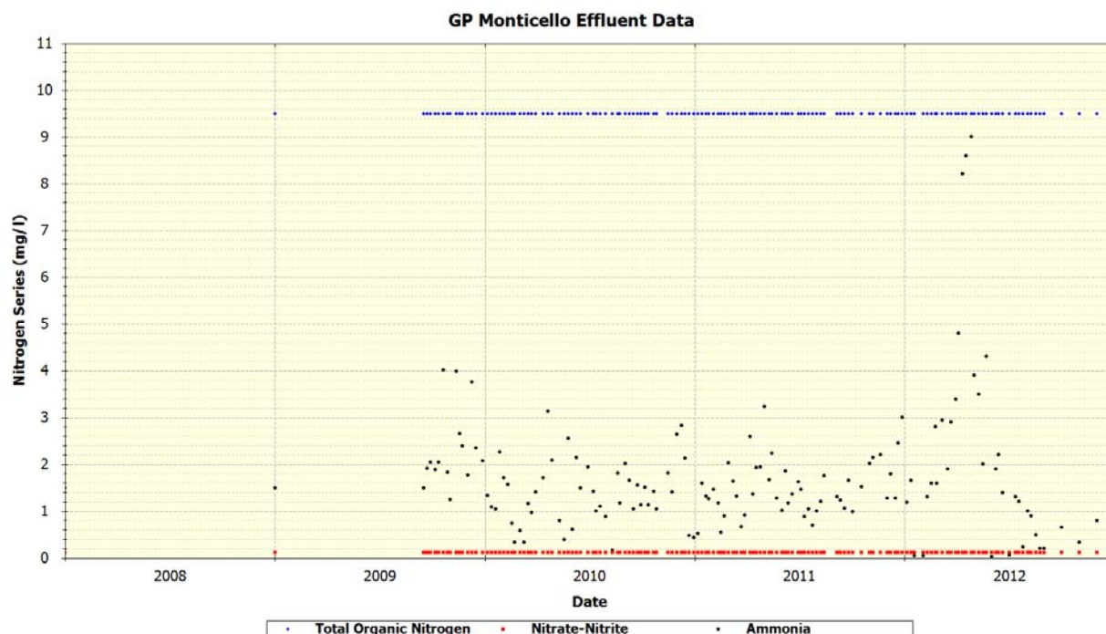
Figure 40 GP Monticello Effluent Discharge Nitrogen Series Data
