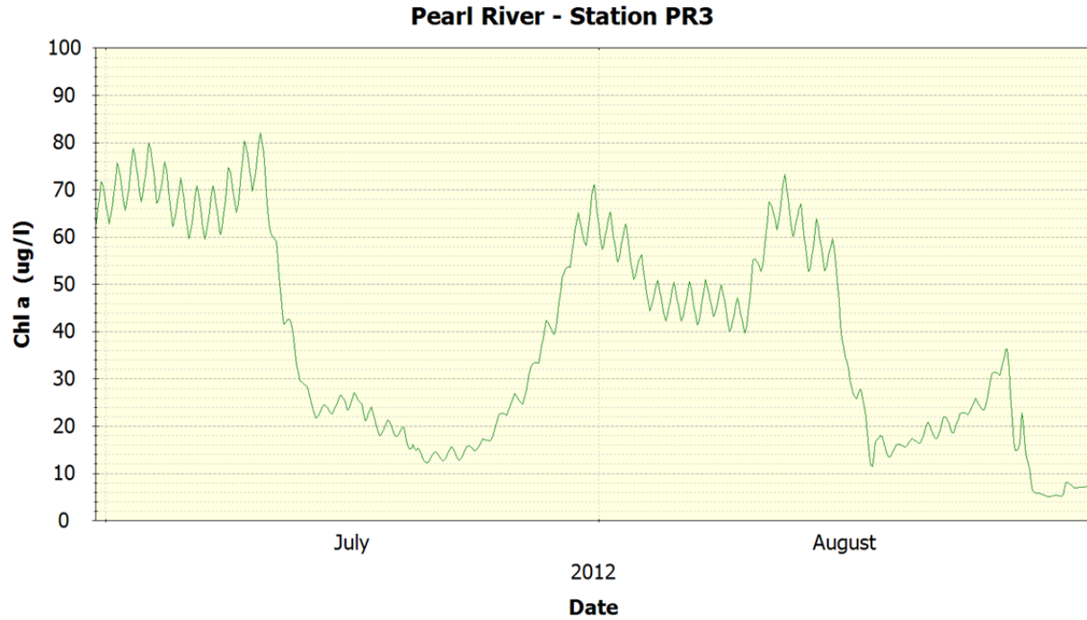
Figure 86 Pearl River Station PR3 – Chl a
