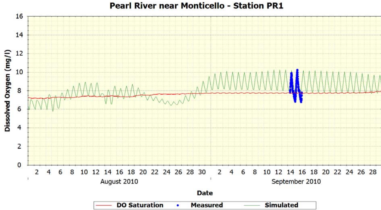
Figure 97 Pearl River near Monticello Station PR1 – Dissolved Oxygen
