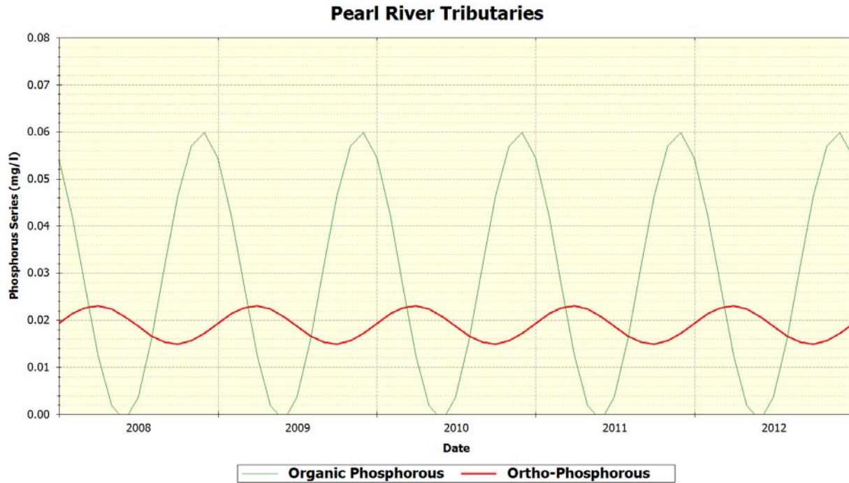
Figure 50 Pearl River Tributary – Phosphorous Series
