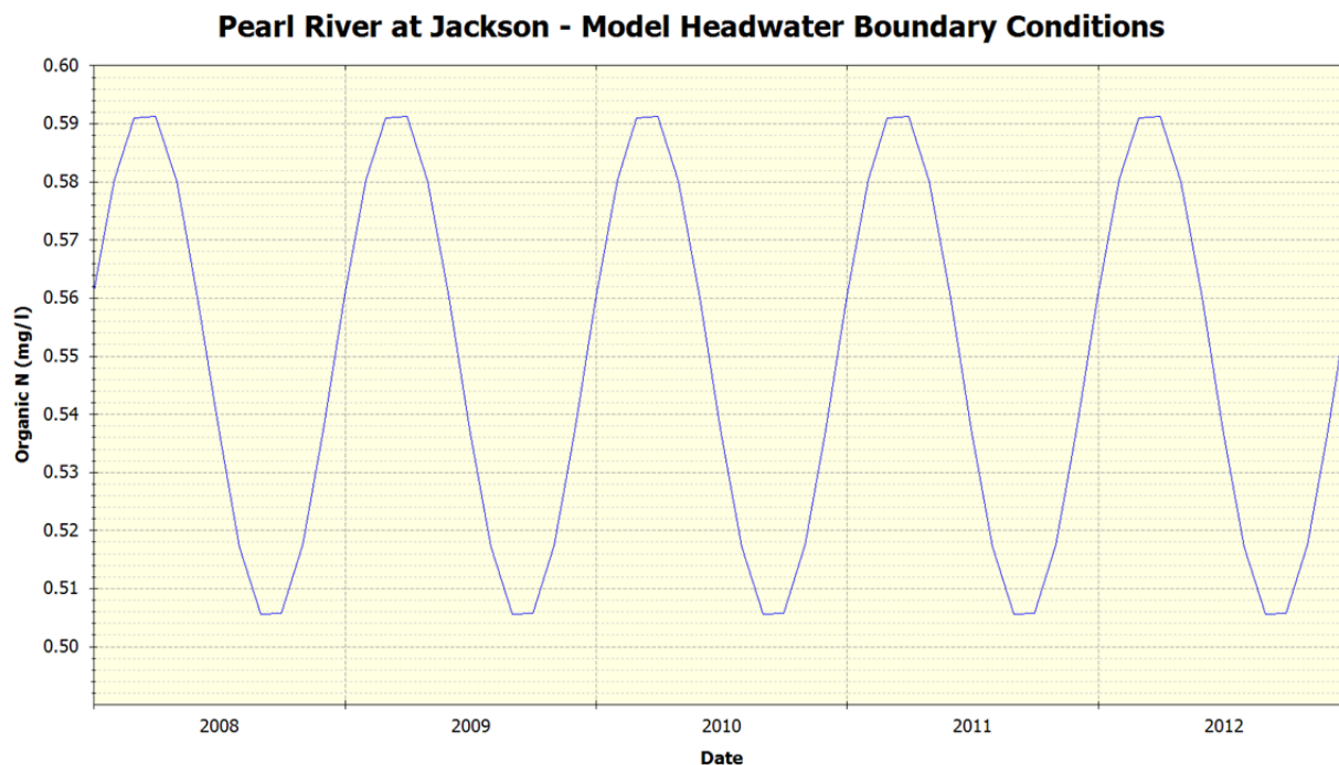
Figure 43 Model Headwater Conditions – Organic Nitrogen
