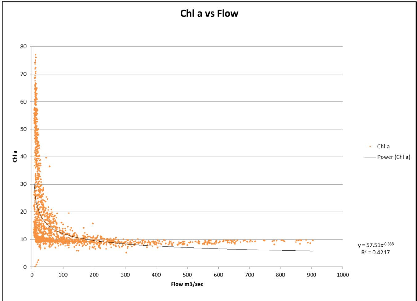
Figure 10 Model Output Chlorophyll-a vs. Flow Model Cell 360
