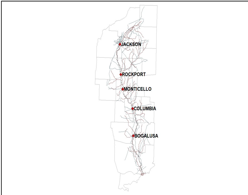
Figure 23 Pearl River USGS Gages
