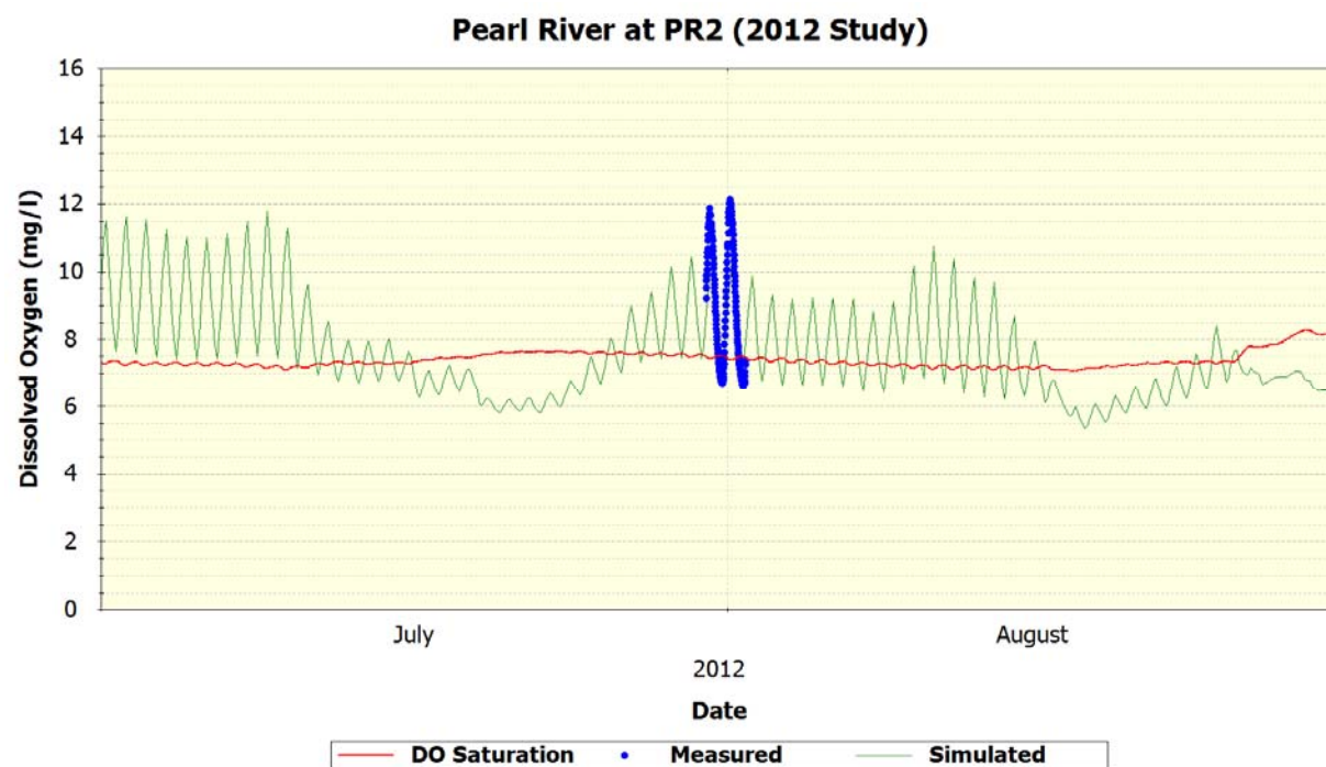
Figure 83 Pearl River Station PR2 – Dissolved Oxygen
