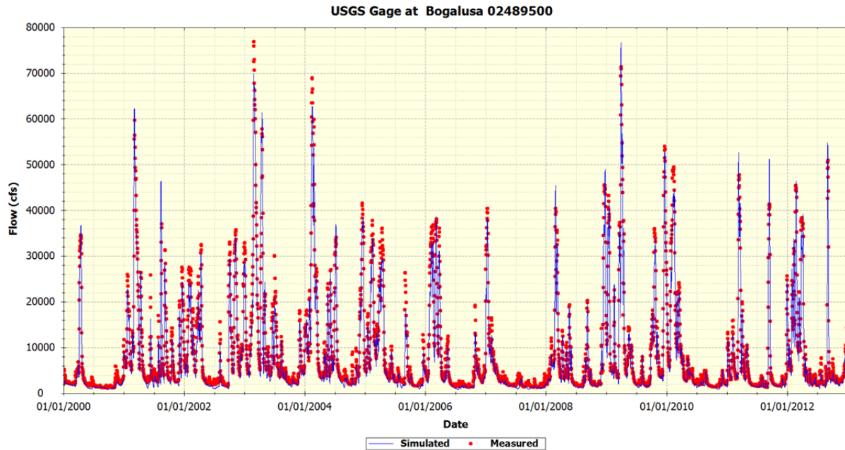
Figure 33 Simulated and Measured Flows – USGS Gage at Bogalusa
