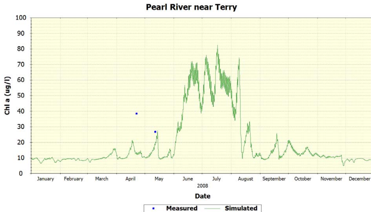
Figure 61 MDEQ Station Pearl River near Terry – Chl a
