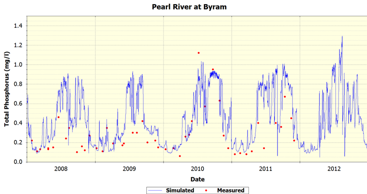
Figure 54 Pearl River at Byram – Simulated vs Measured Total Phosphorus
