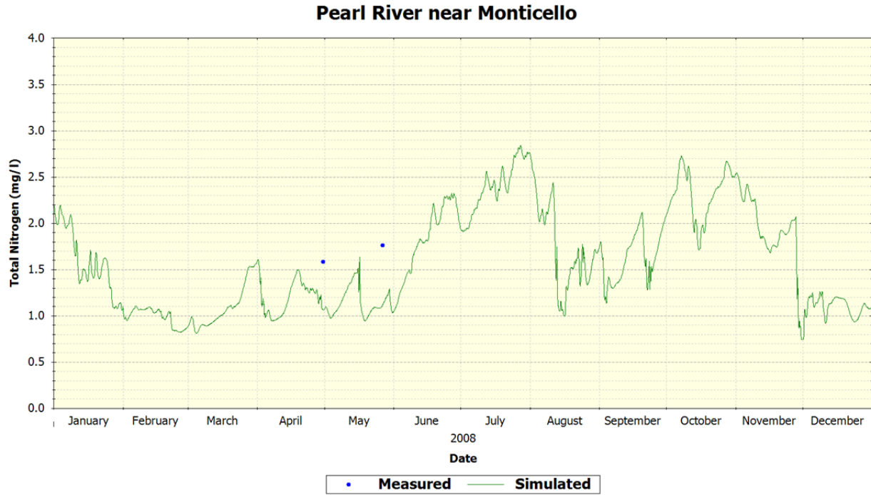
Figure 65 MDEQ Station Pearl River near Monticello – Total Nitrogen
