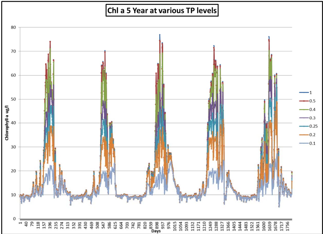
Figure 12 Model Output Chlorophyll-a at various TP reductions Model Cell 360, 2008 - 2012
