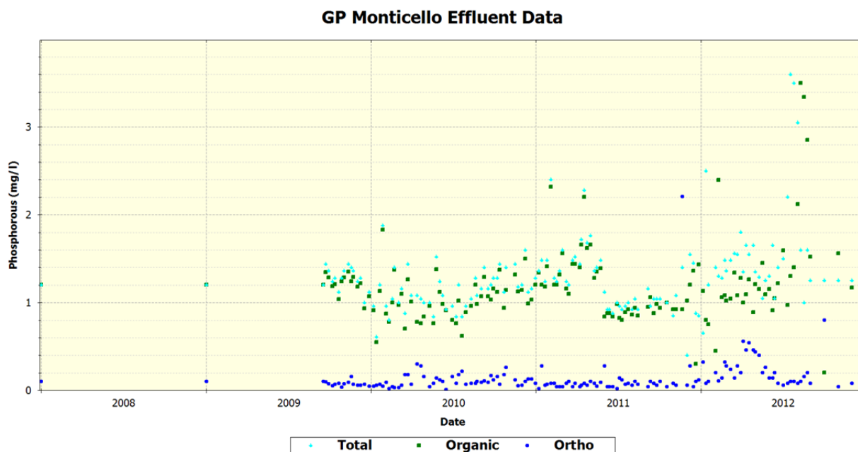
Figure 41 GP Monticello Effluent Discharge Phosphorous Series Data
