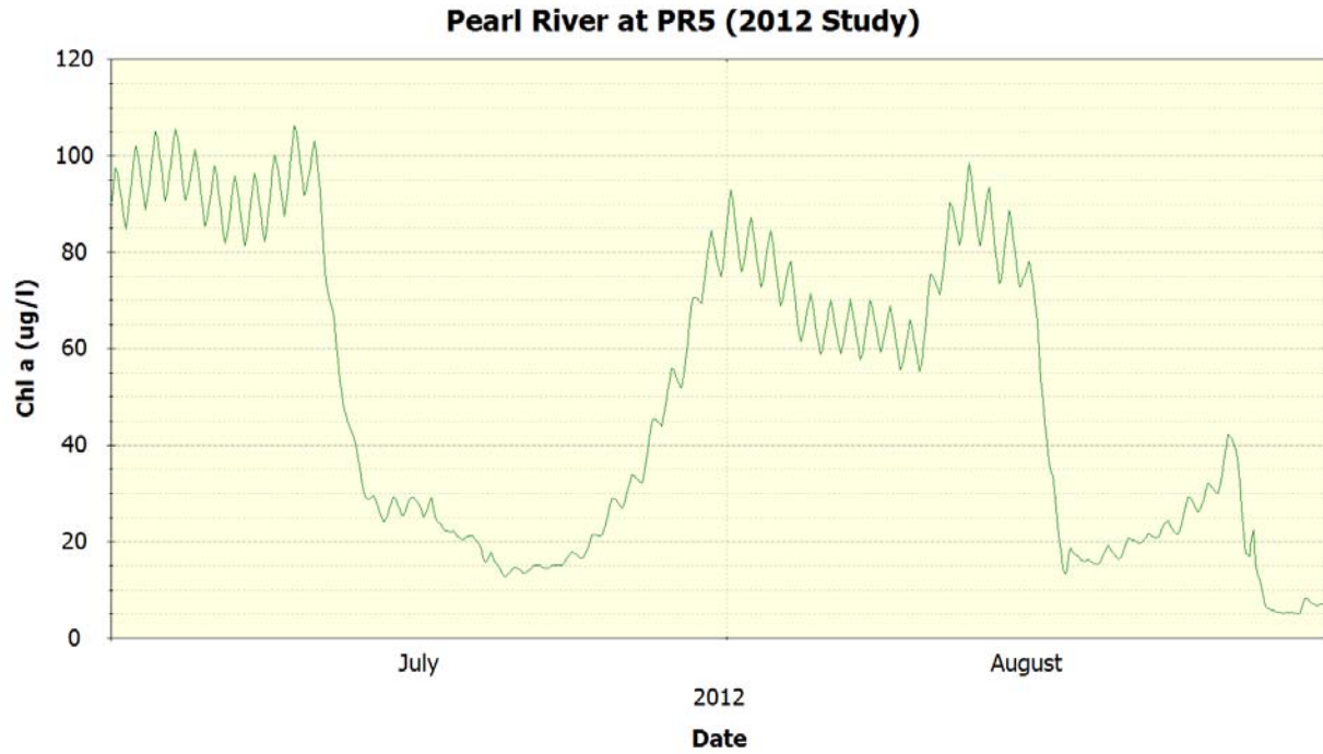
Figure 90 Pearl River Station PR5 – Chl a
