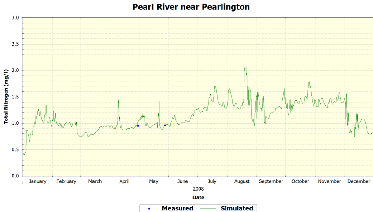
Figure 74 MDEQ Station Pearl River near Pearlington – Total Nitrogen
