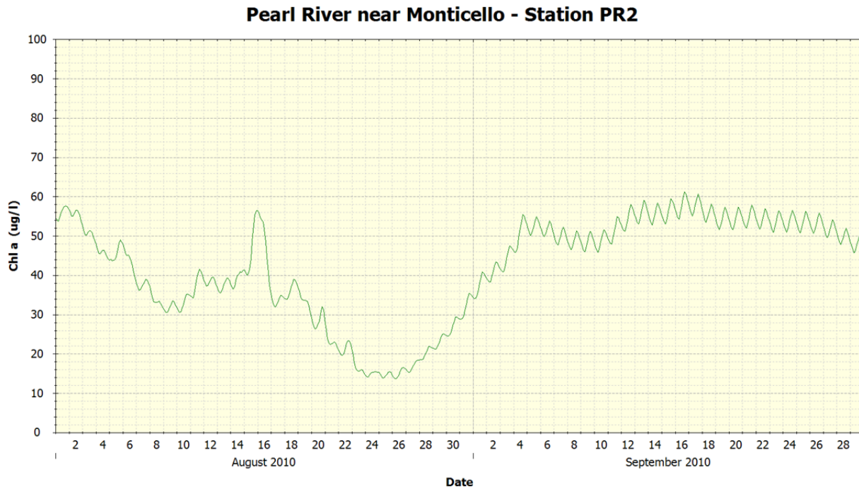
Figure 100 Pearl River near Monticello Station PR2 – Chl a
