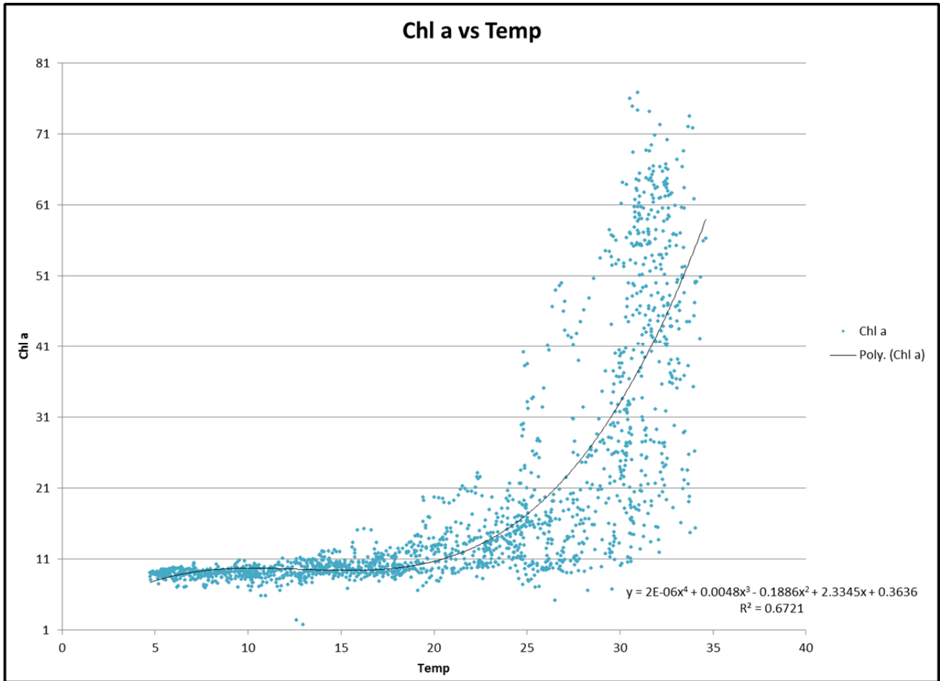
Figure 11 Model Output Chlorophyll-a vs. Temperature Model Cell 360
