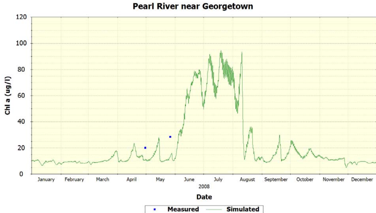
Figure 64 MDEQ Station Pearl River near Georgetown – Chl a
