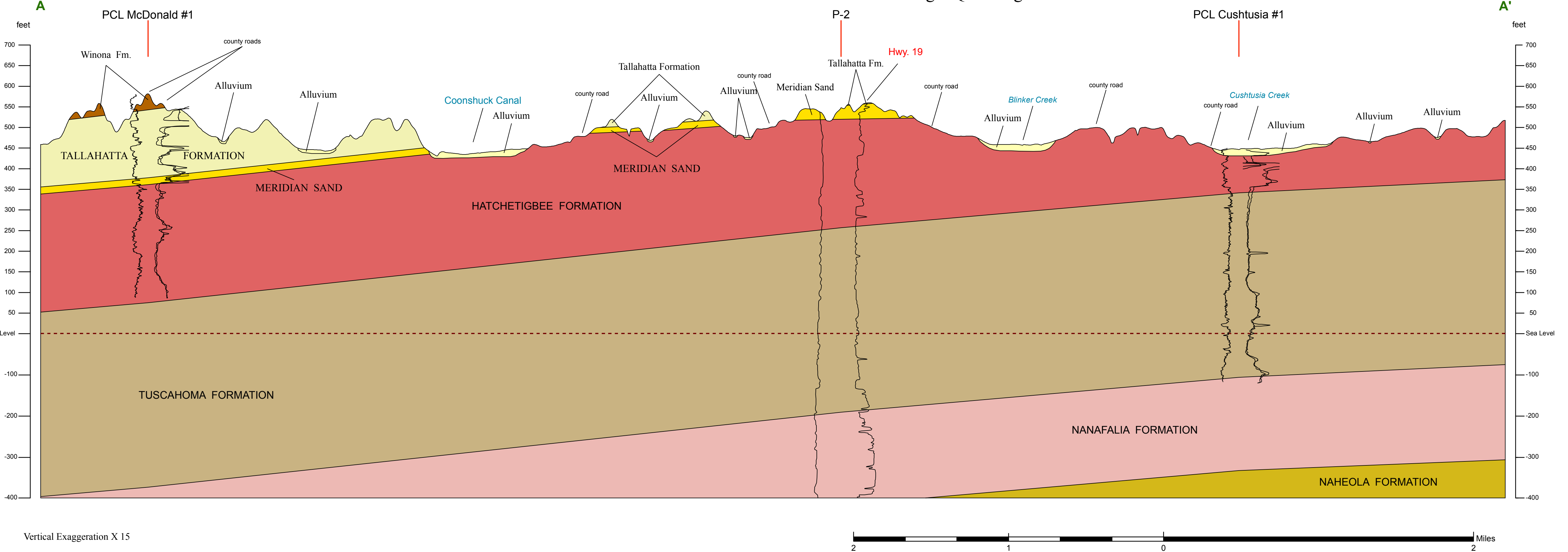
Structural Cross-Section of the Deemer 7.5-Minute Geologic Quadrangle
