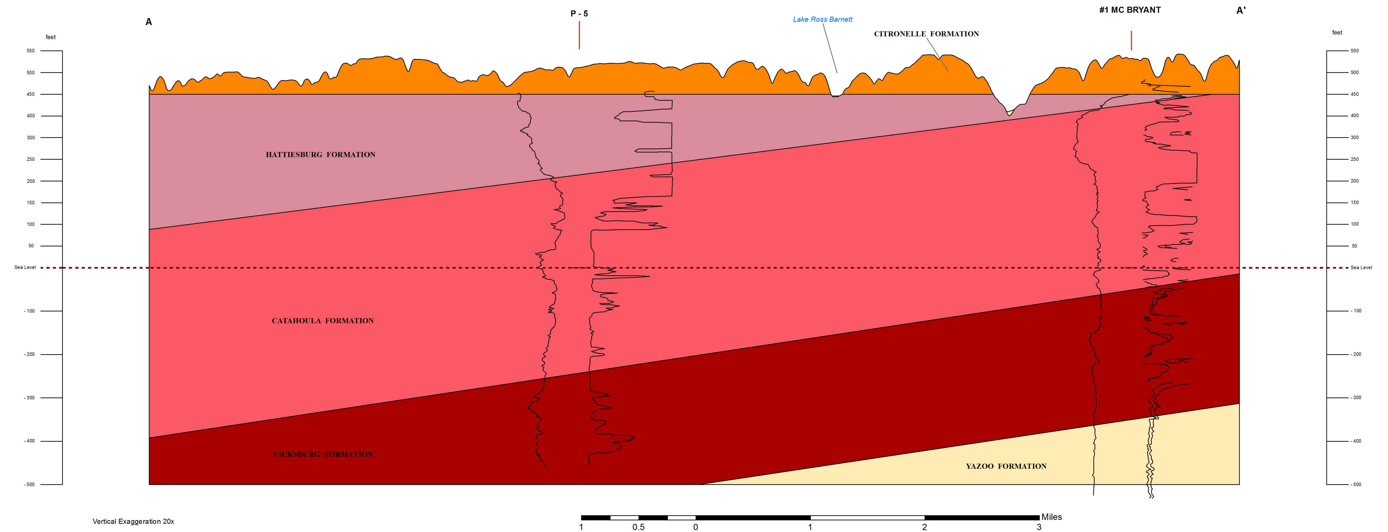
Structural Cross-Section of the Mize 7.5-Minute Geologic Quadrangle
