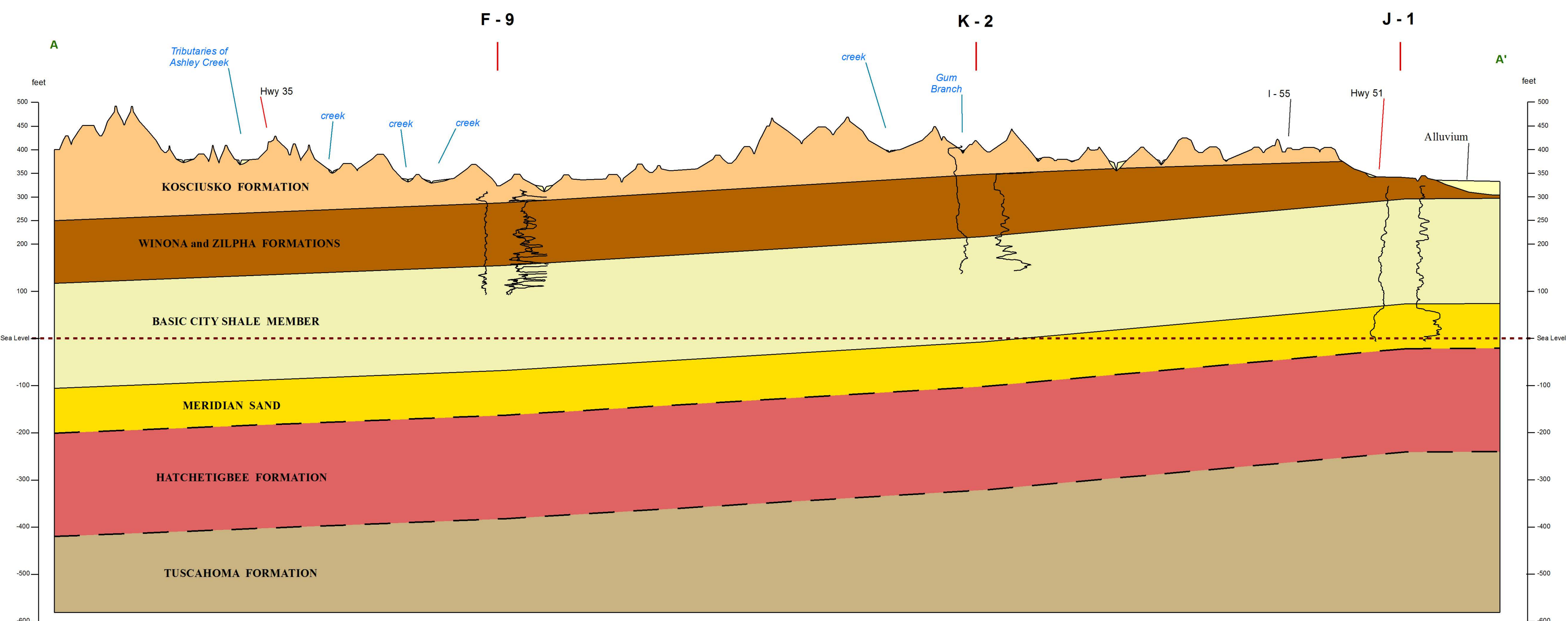
Structural Cross-Section of the Bailey Lake 7.5-Minute Geologic Quadrangle
