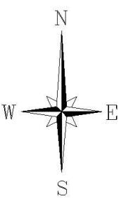
GEOLOGIC MAP BAILEY LAKE QUADRANGLE Carroll and Montgomery Counties, Mississippi
