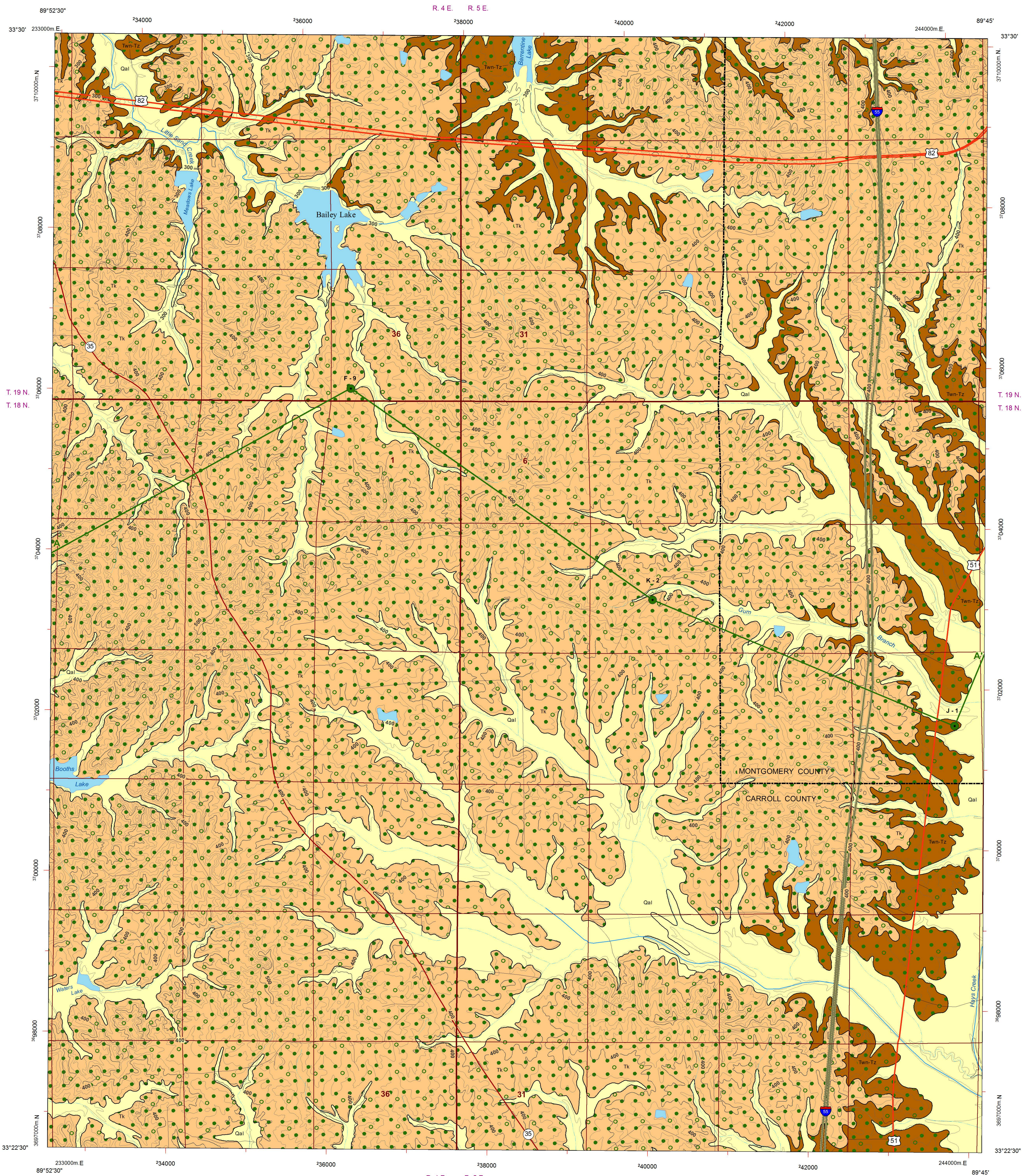
GEOLOGIC MAP BAILEY LAKE QUADRANGLE Carroll and Montgomery Counties, Mississippi
