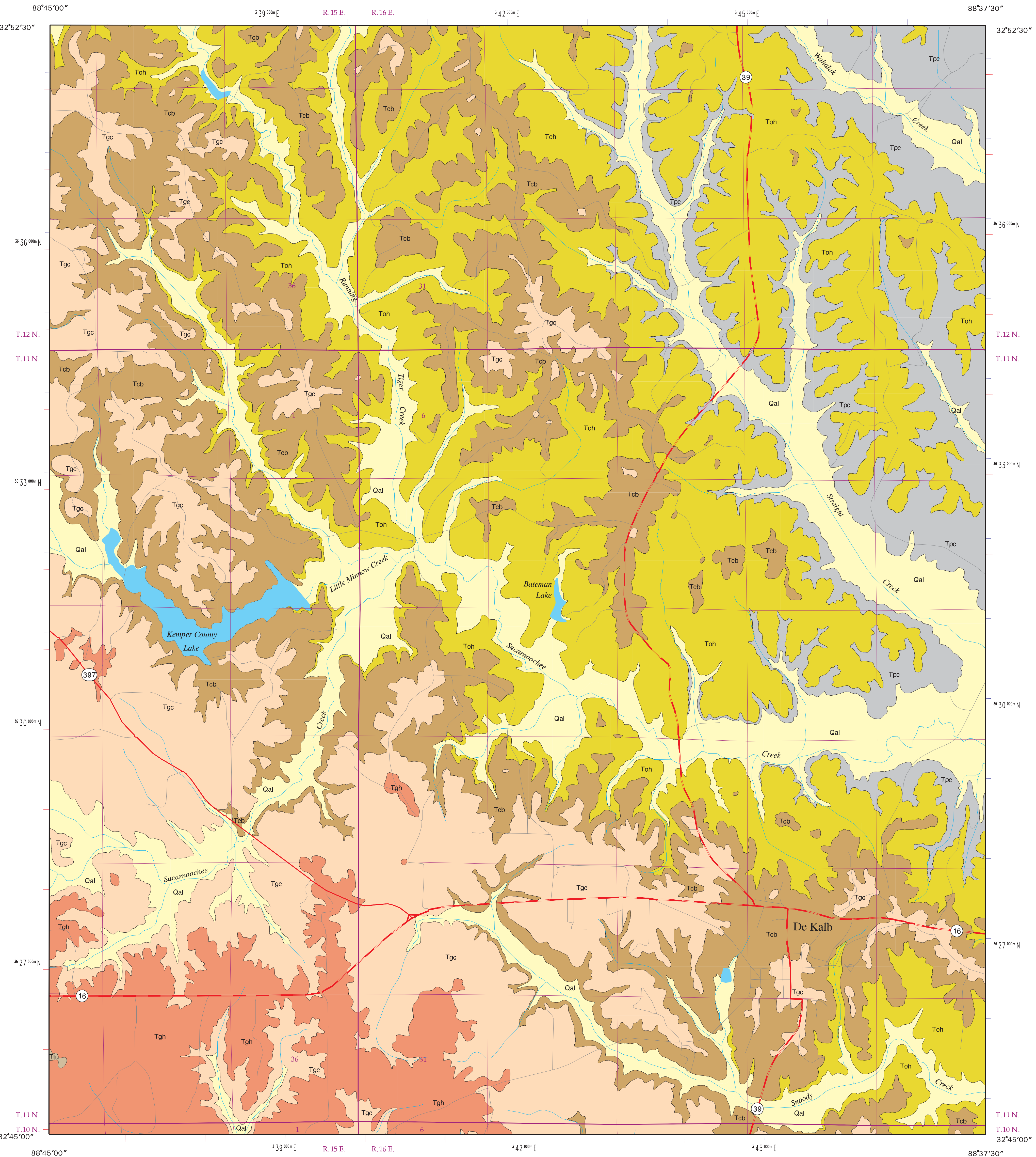
GEOLOGIC MAP DE KALB QUADRANGLE Kemper County, Mississippi
