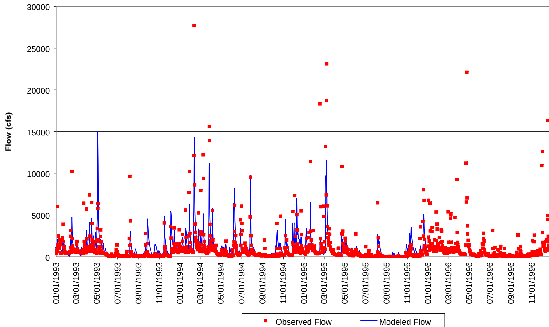
Graph A-1 Daily Flow Comparison between USGS Station 02436500 and Reach 03160102001 for 01/01/1993 - 12/31/1998
