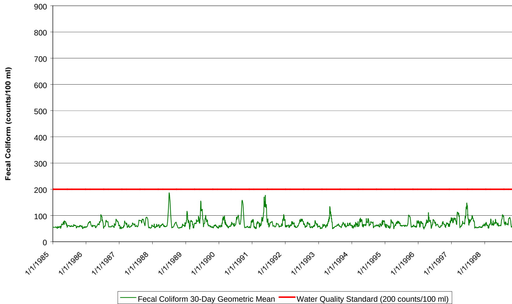
Graph A-4 Modeled Fecal Coliform Concentrations Under Existing Conditions for Reach 03160102001
