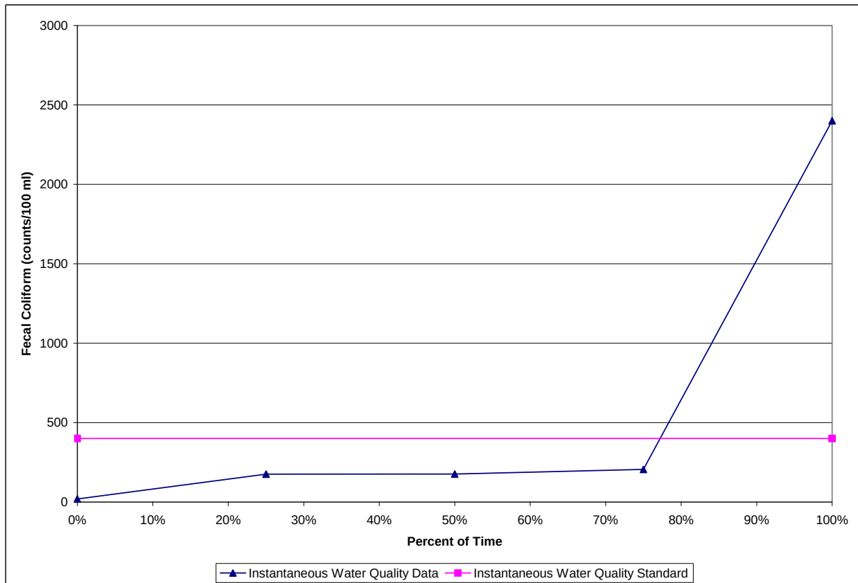
Figure 6. 10% Test Curve for Station 62, Summer 2003
