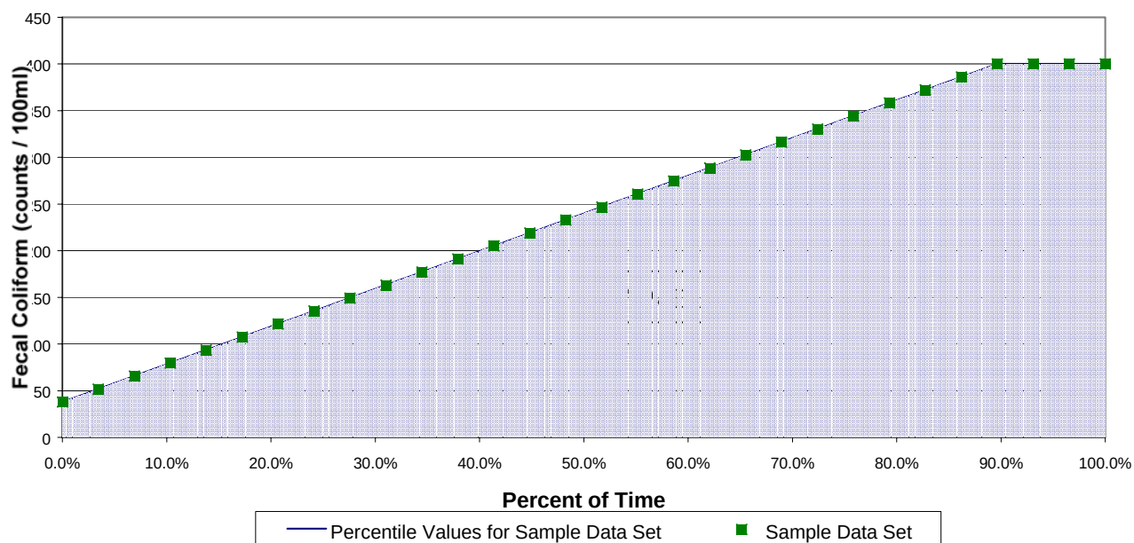
Figure 4. Theoretical Capacity Curve
