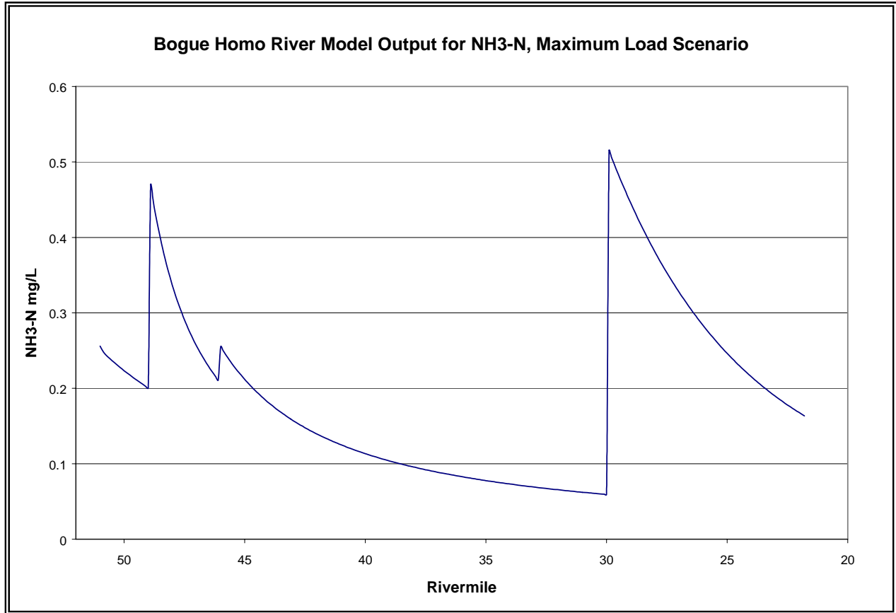
Figure 9. Model Output for \text{NH}_3\text{-N} in the Bogue Homo River, Maximum Load Scenario
