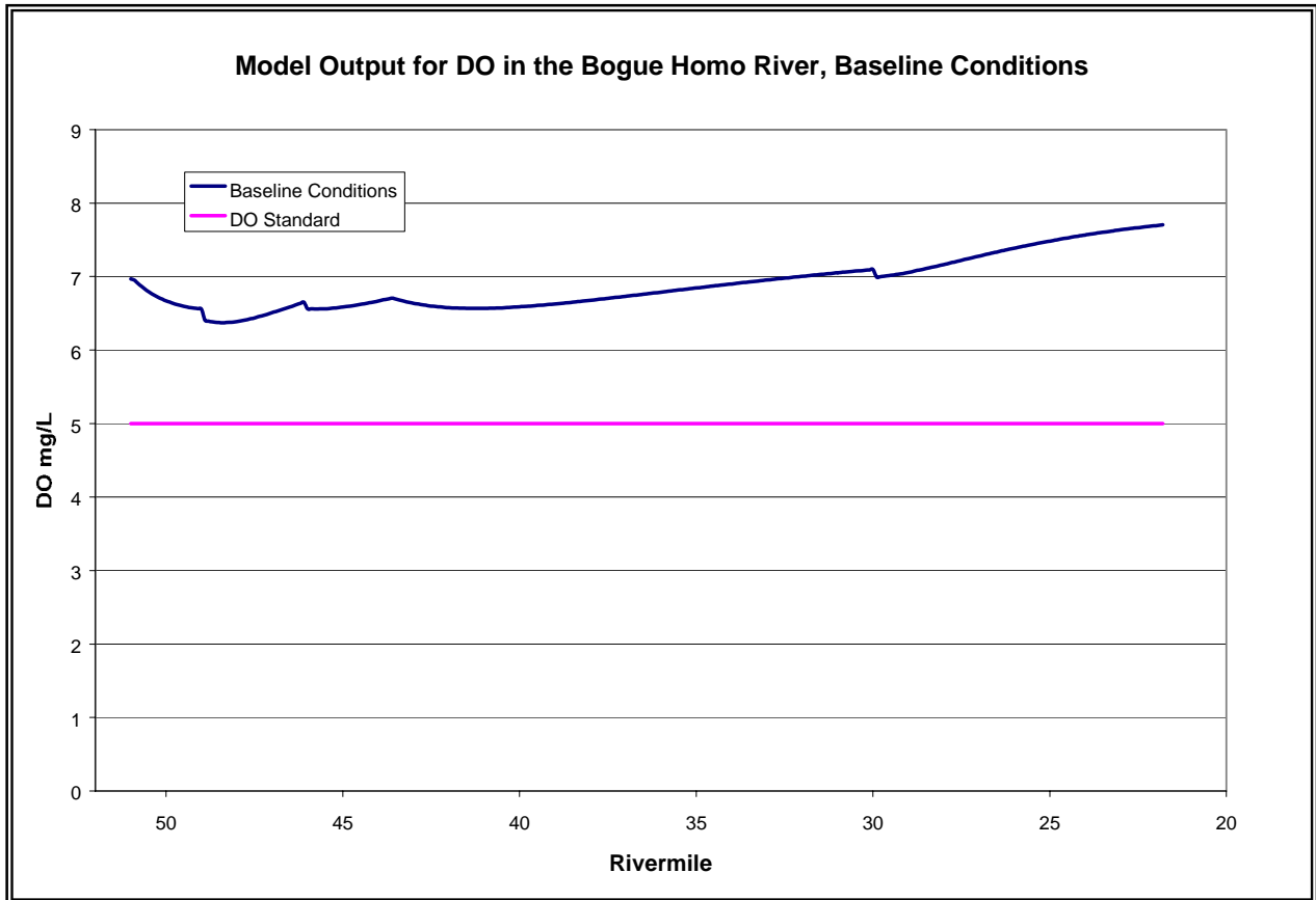
Figure 7. Model Output for DO in the Bogue Homo River, Baseline Conditions
