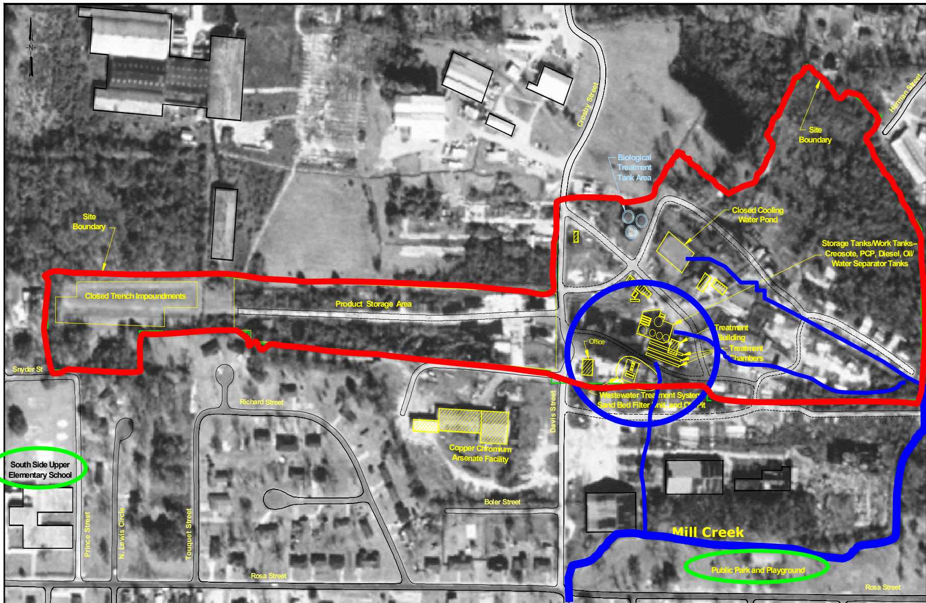
Figure 2-2 Site Layout Picayune Wood Treating, Inc. Picayune, Mississippi
