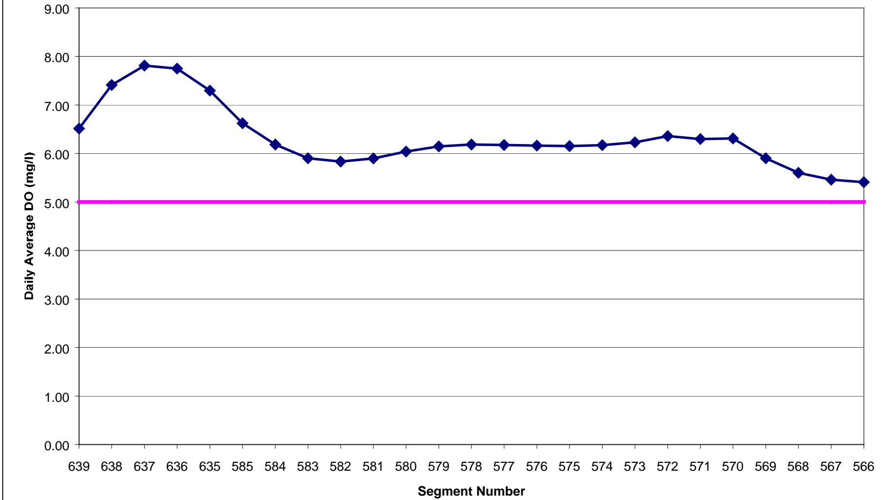
Graph A-1: Daily Average Dissolved Oxygen in Bernard Bayou segment 3 from WASP5 Model
