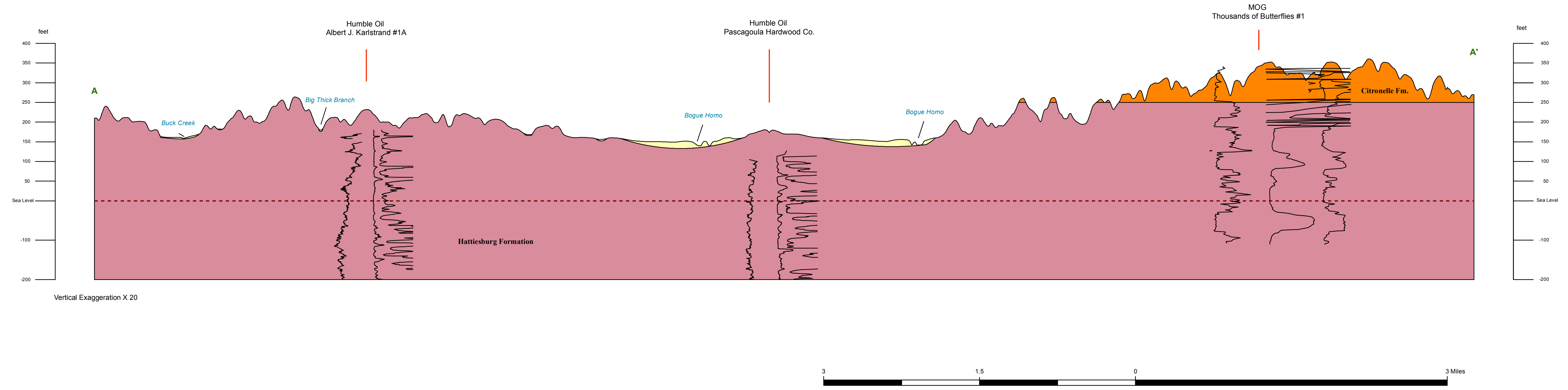
Structural Cross-Section of the Ovett 7.5-Minute Geologic Quadrangle
