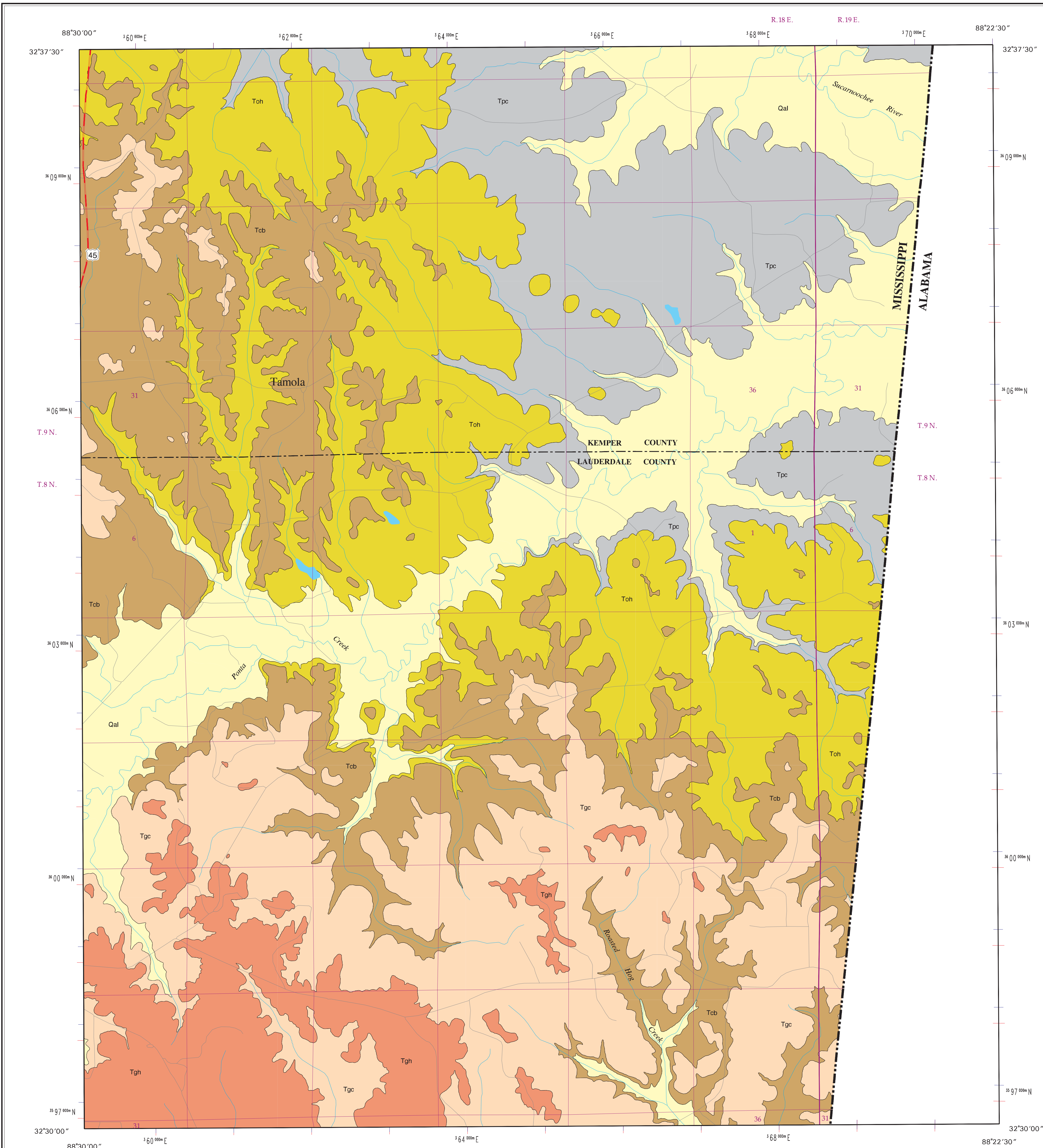
GEOLOGIC MAP TAMOLA QUADRANGLE
