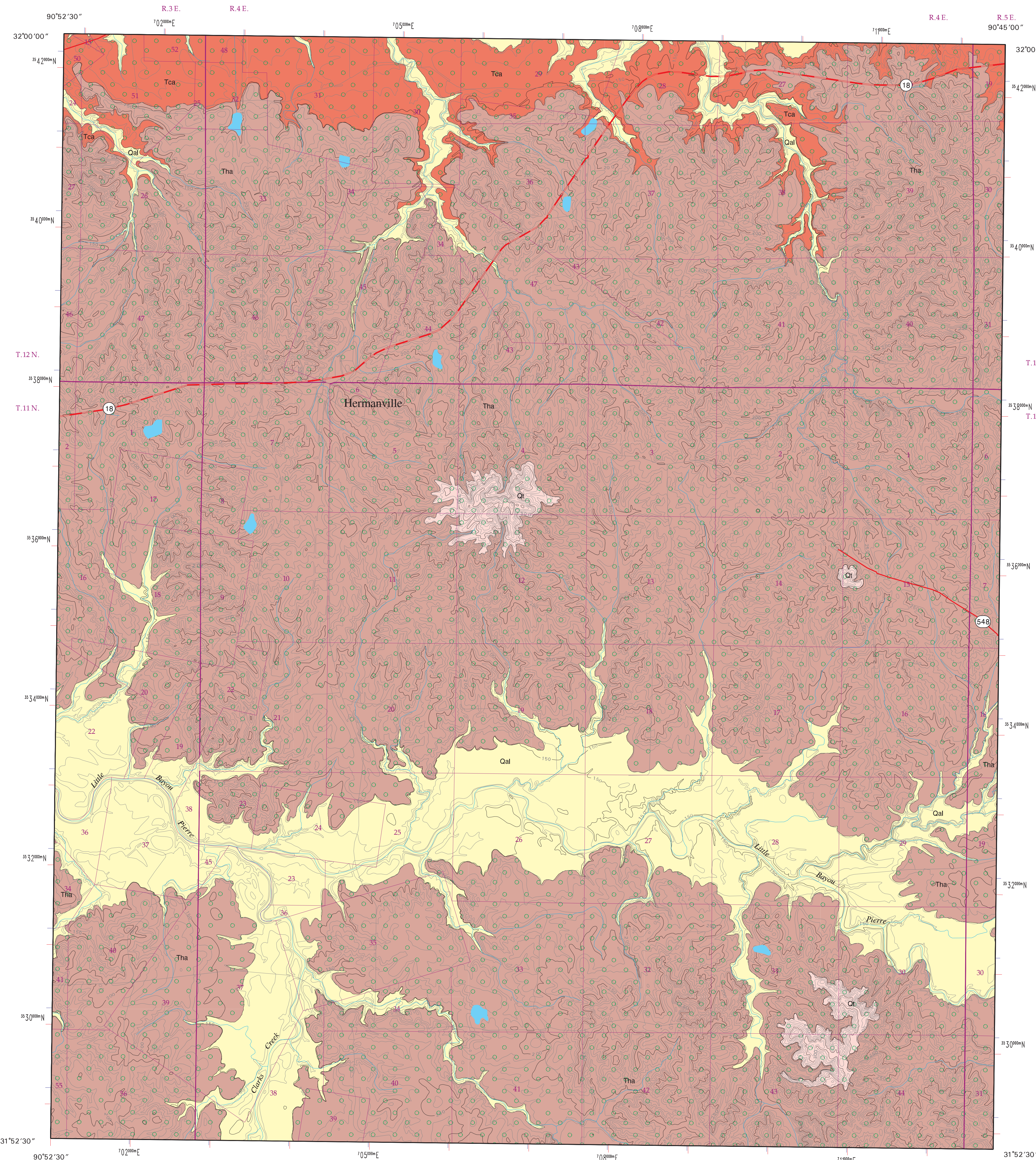
GEOLOGIC MAP HERMANVILLE QUADRANGLE Claiborne County, Mississippi
