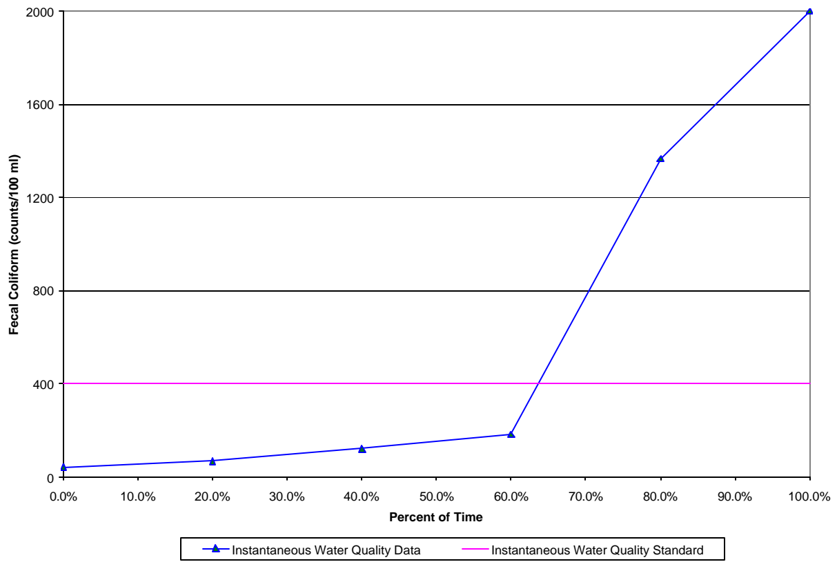
Figure 6. Existing Load Curve for Station 27, Summer 2004
