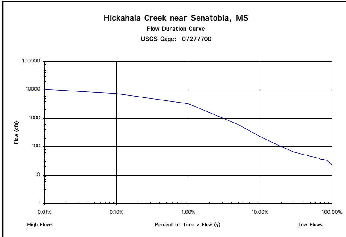
Figure 5. Flow Duration Curve for Hickahala Creek at Station 07277700
